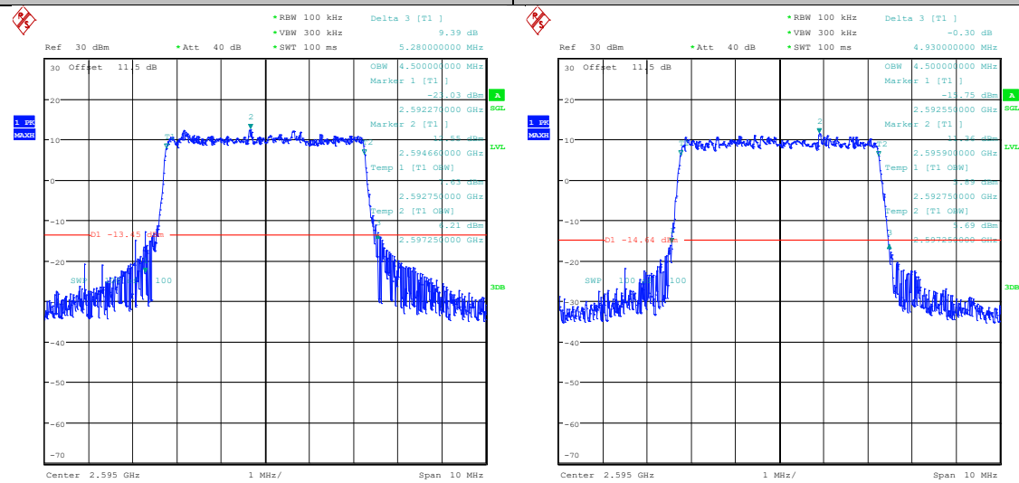
Band38-5MHz-QPSK-37775-25RB#0-PASS
