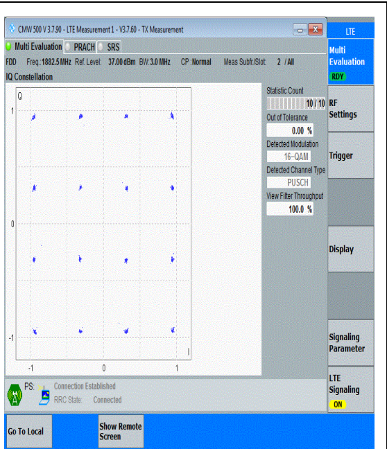
Band25-3MHz-16QAM-26365-15RB#0-PASS
