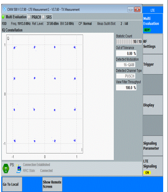
Band25-3MHz-16QAM-26675-15RB#0-PASS
