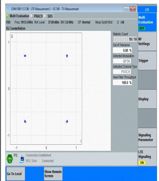
Band25-3MHz-QPSK-26675-15RB#0-PASS
