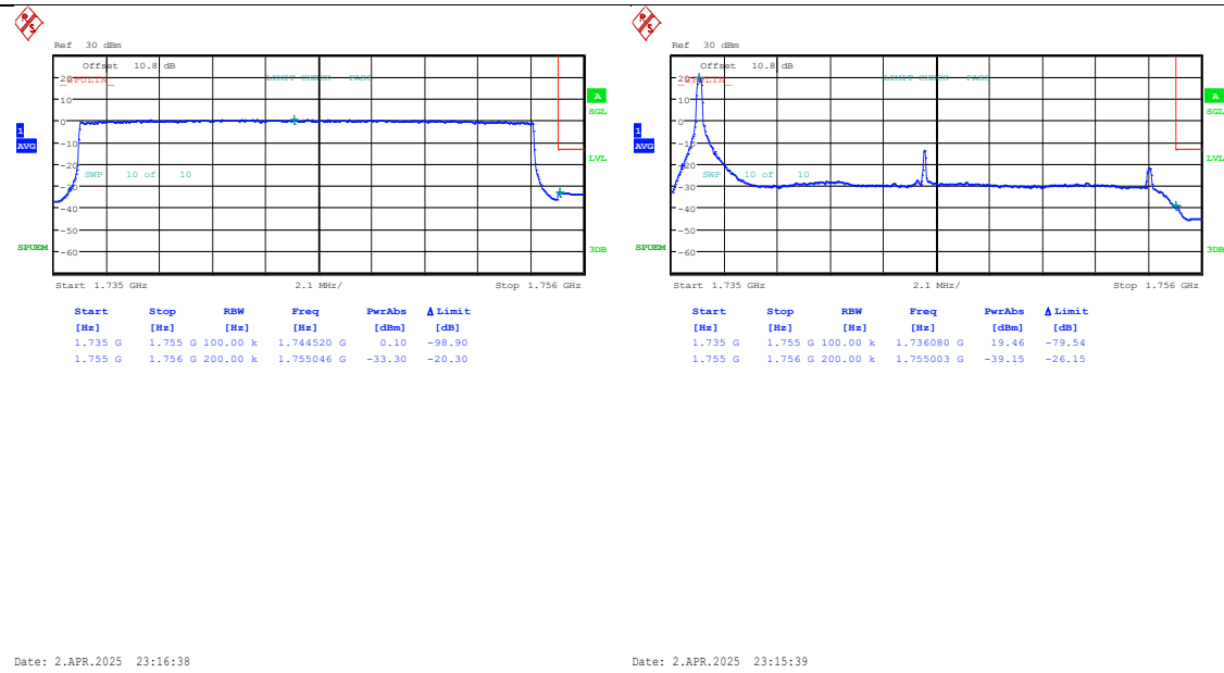
Band4-20MHz-QPSK-20300-100RB#0-PASS
