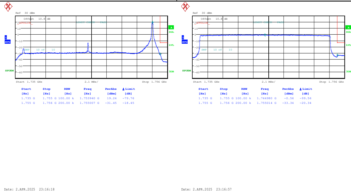
Band4-20MHz-16QAM-20300-1RB#99-PASS
