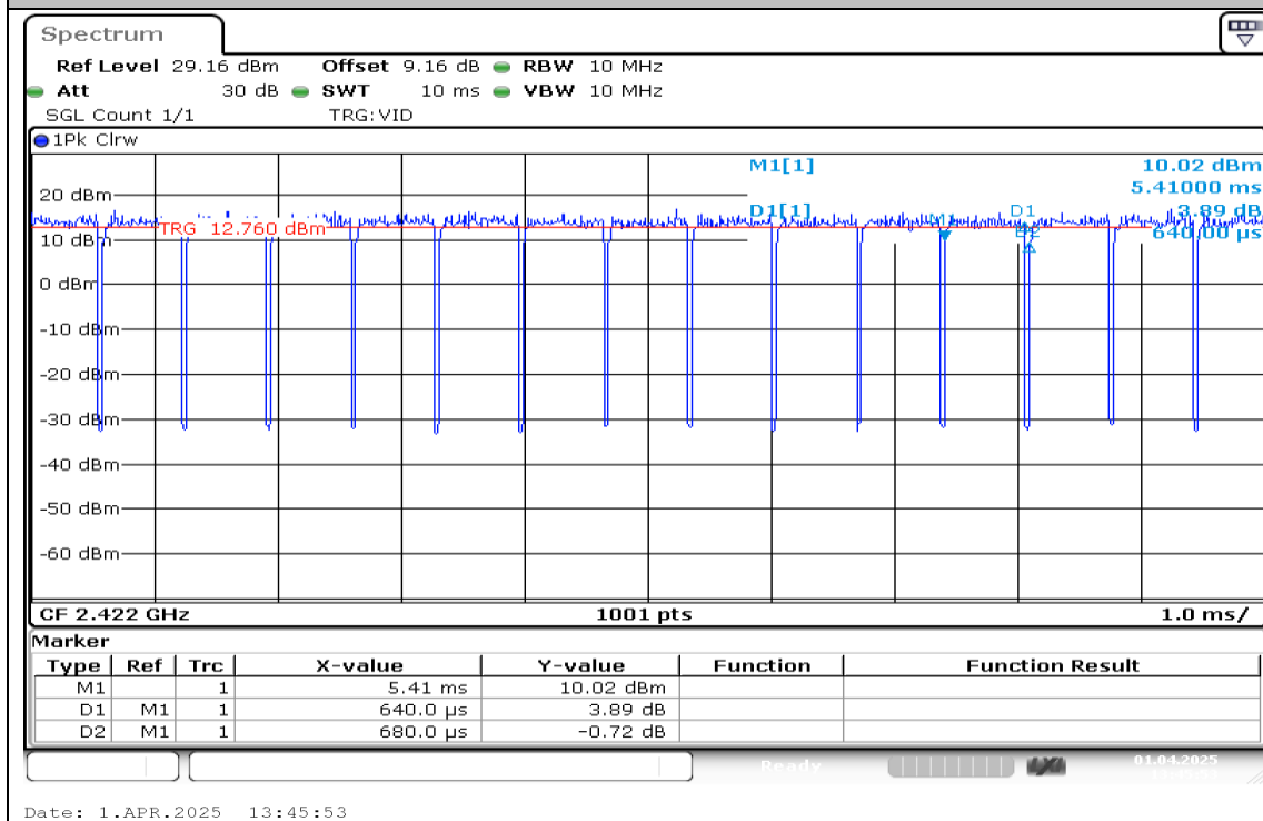
NTNV-11N40SISO-Ant1-2422
