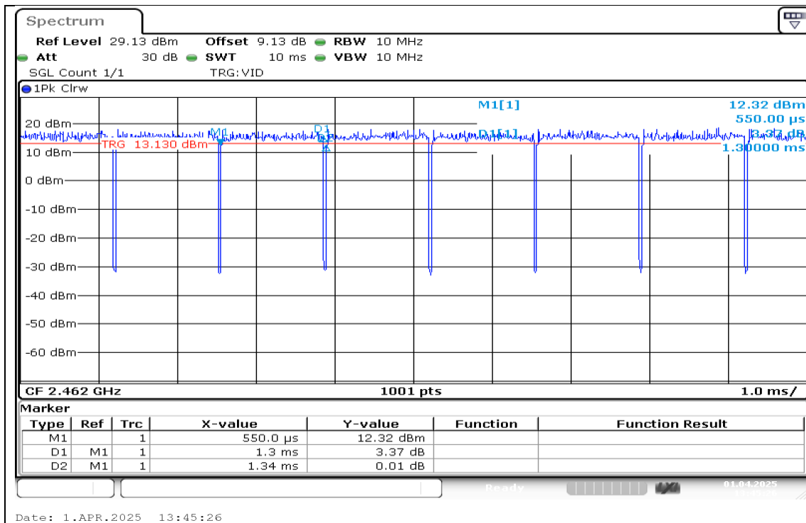
NTNV-11N20SISO-Ant1-2462
