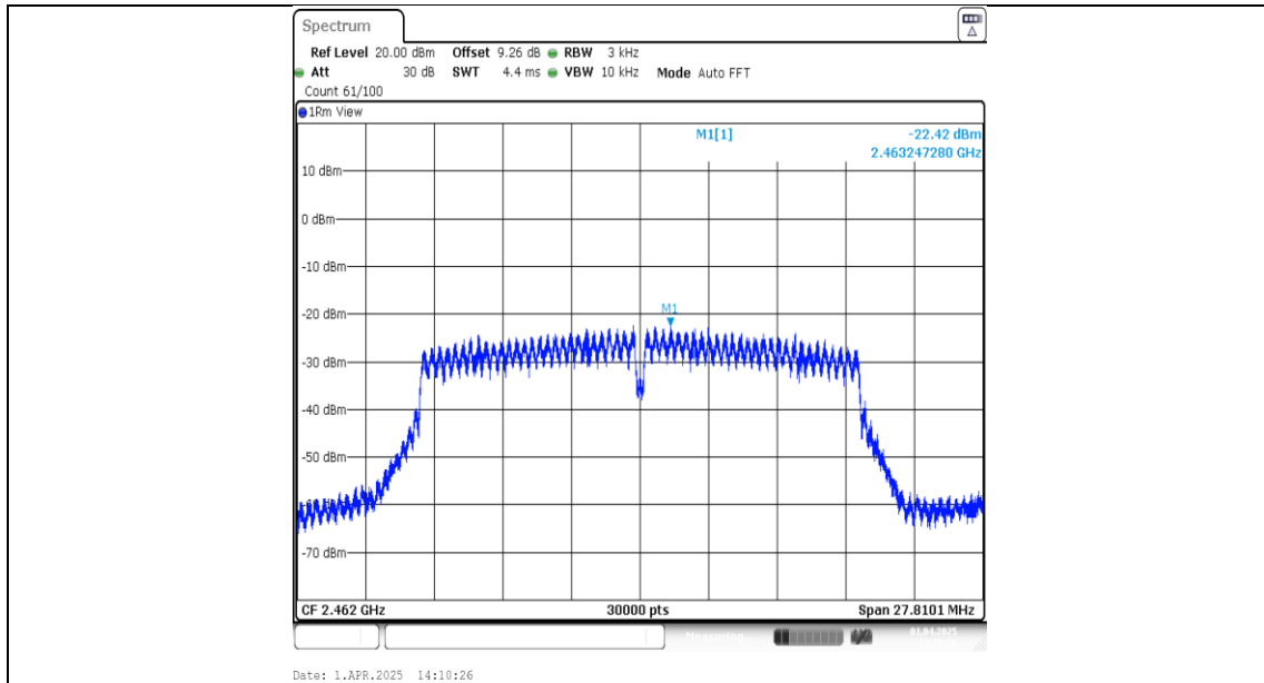
11N20SISO-Ant1-2462-PASS
