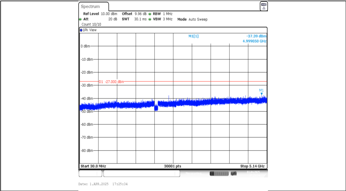
11AC40SISO-Ant1-5230-30~5140-PASS
