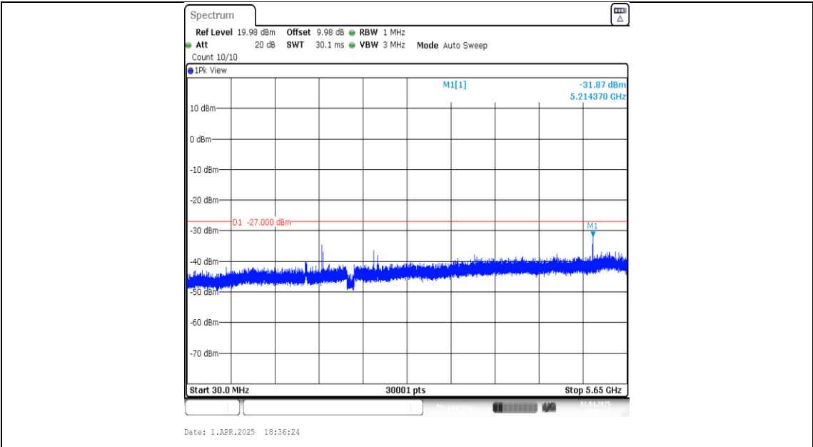
11AC40SISO-Ant1-5755-30~5650-PASS
