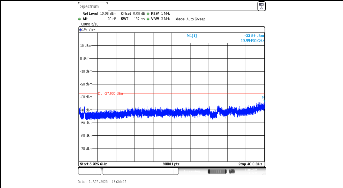
11AC40SISO-Ant1-5755-5925~40000-PASS
