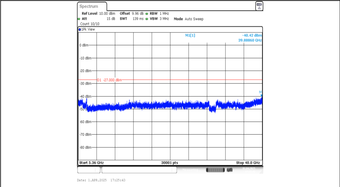
11AC40SISO-Ant1-5230-5360~40000-PASS
