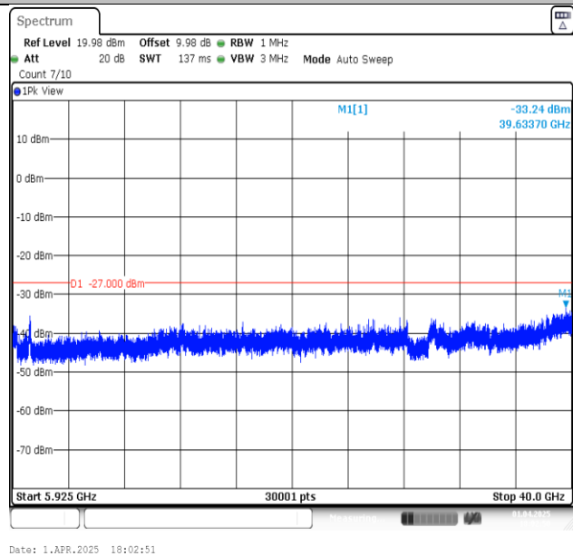
11N20SISO-Ant1-5825-5925~40000-PASS
