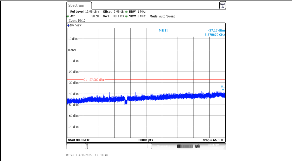
11A-Ant1-5745-30~5650-PASS
