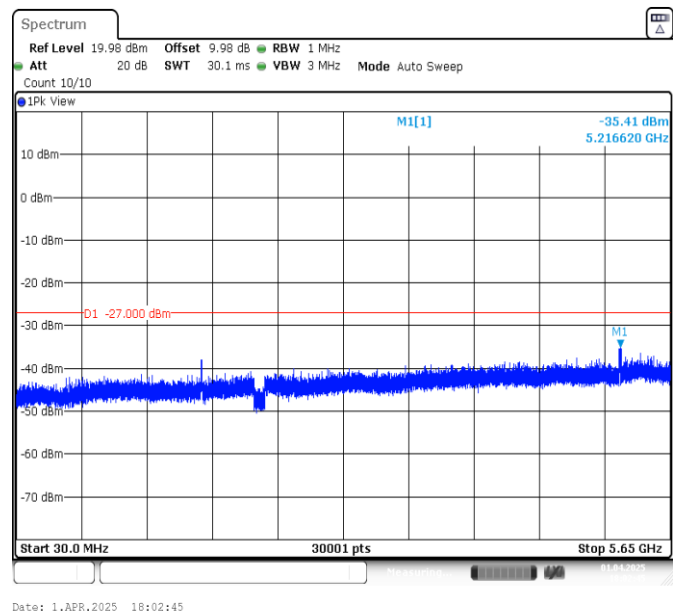
11N20SISO-Ant1-5825-30~5650-PASS
