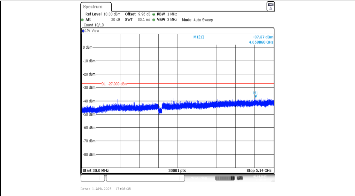
11AC20SISO-Ant1-5180-30~5140-PASS
