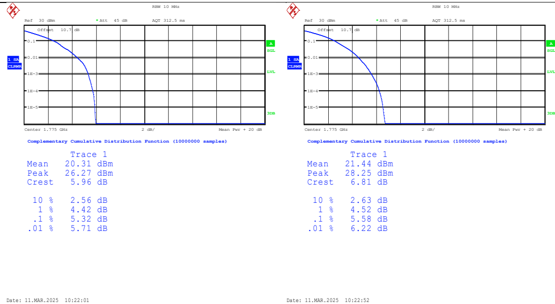
Band66-10MHz-QPSK-132622-1RB#0-PASS
