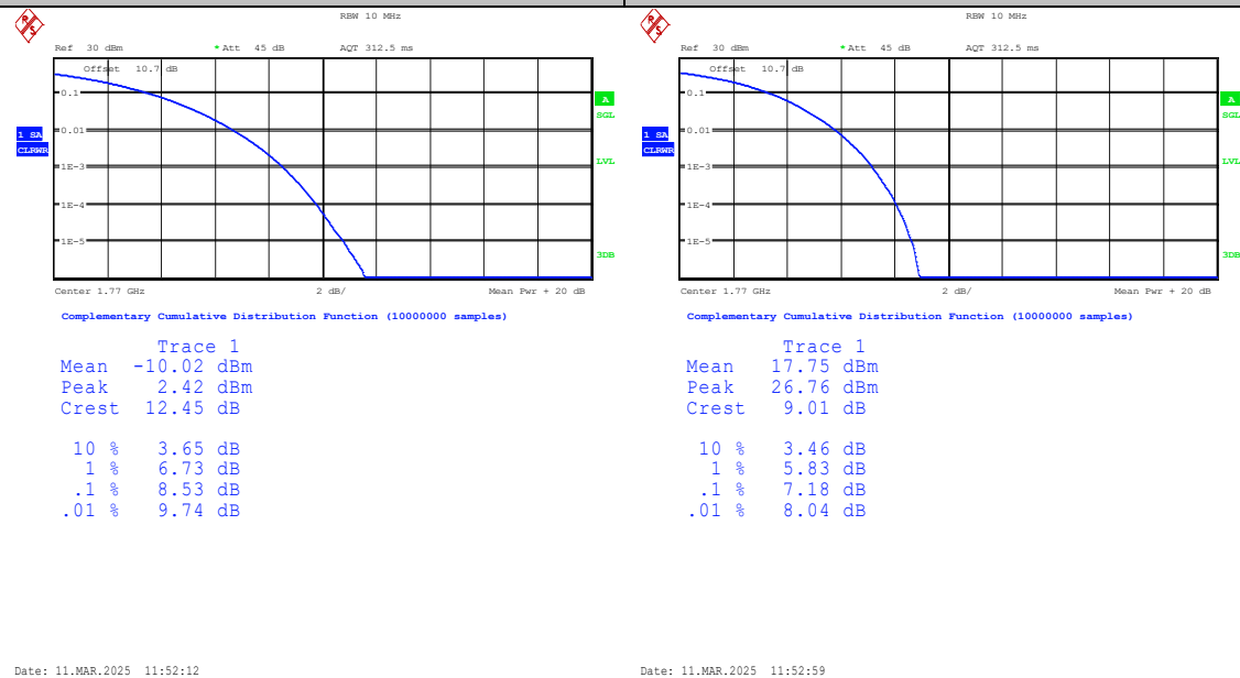
Band66-20MHz-16QAM-132572-1RB#0-PASS
