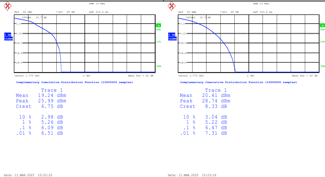
Band66-10MHz-16QAM-132622-1RB#0-PASS
