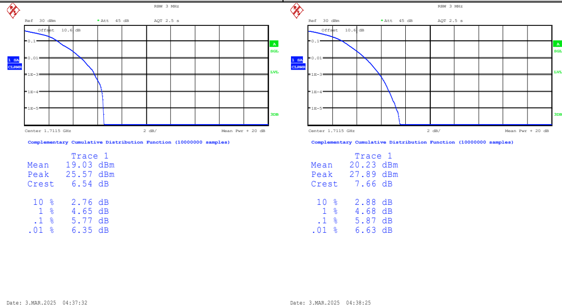
Band4-3MHz-16QAM-19965-1RB#0-PASS
