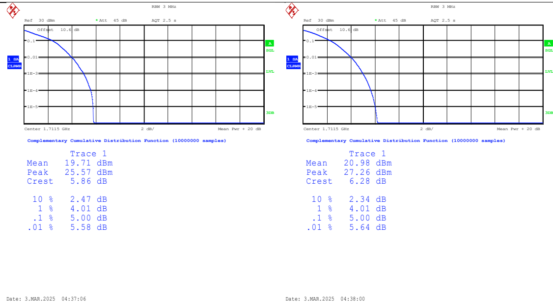
Band4-3MHz-QPSK-19965-1RB#0-PASS
