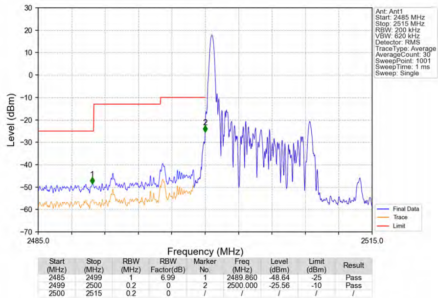
Band7_10MHz_16QAM_LCH_2505MHz_RB_1_0_NTNV
