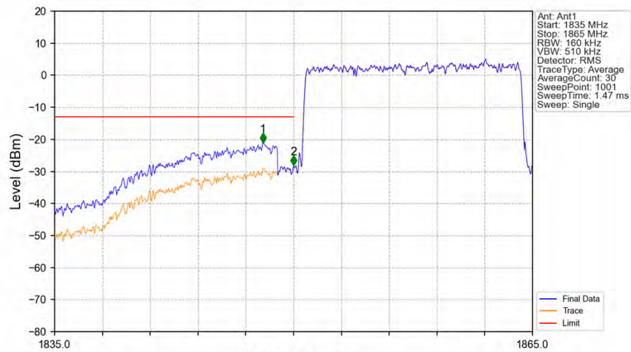
Band2_15MHz_16QAM_LCH_1857.5MHz_RB_75_0_NTNV
