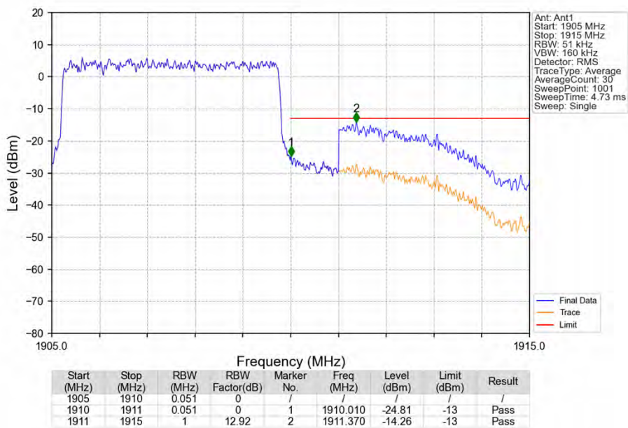
Band2_5MHz_QPSK_HCH_1907.5MHz_RB_25_0_NTNV
