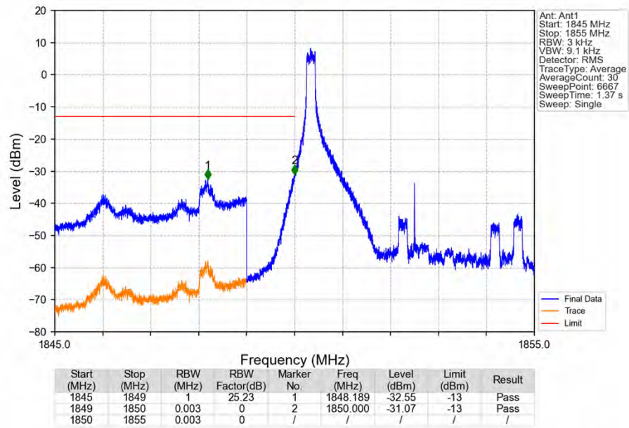
Band2_5MHz_16QAM_LCH_1852.5MHz_RB_1_0_NTNV
