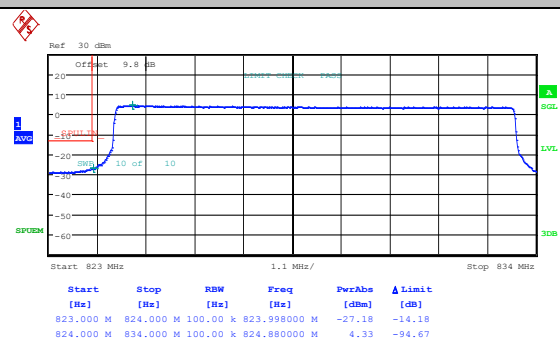
Band26_10MHz_16QAM_26840_1RB#49
