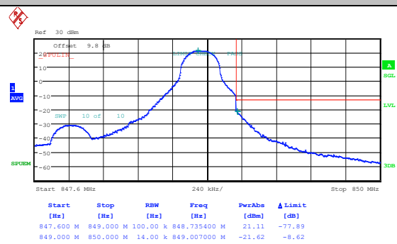
Band26_1.4MHz_16QAM_27033_1RB#0
