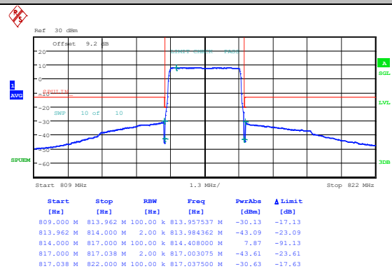
Band26_3MHz_16QAM_26705_1RB#14
