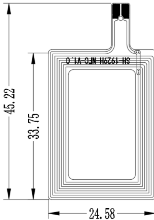
NFC:45.22*24.58mm PIFA
