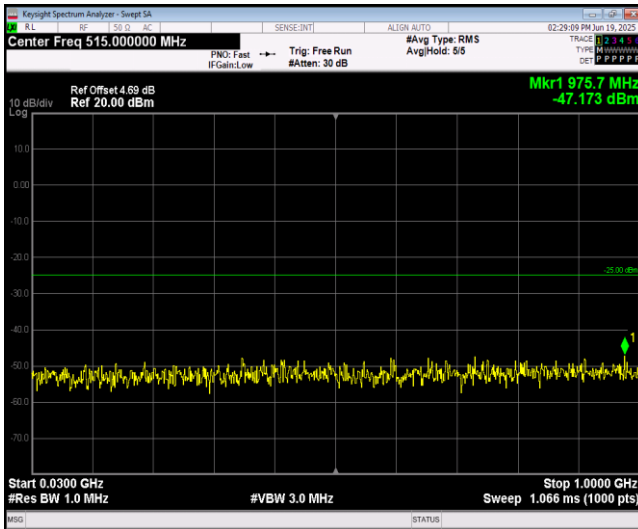
Band38-5MHz-16QAM-38225-1RB#0-Range1:30~1000MHz
