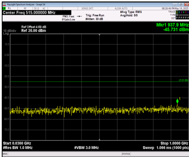
Band7-5MHz-QPSK-21100-1RB#0-Range1:30~1000 MHz
