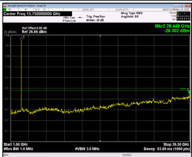
Band7-20MHz-64QAM-21350-1RB#0-Range2:1000~26500MHz
