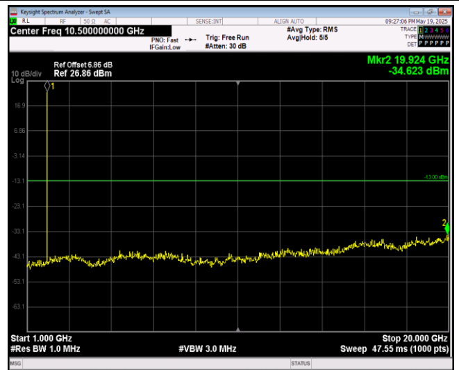
Band25-1.4MHz-16QAM-26047-1RB#0-Range2:1000~20000MHz
