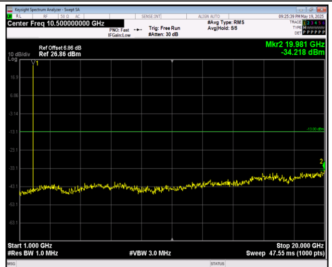
Band25-1.4MHz-16QAM-26365-1RB#0-Range2:1000~20000MHz
