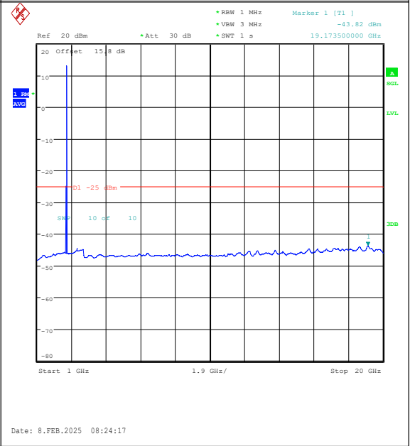
Band38-5MHz-QPSK-38225-1RB#0-1000~20000-PASS
