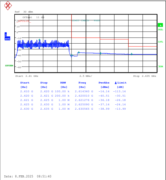
Band38-10MHz-16QAM-38200-50RB#0-PASS
