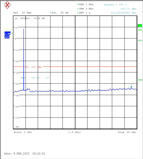
Band38-5MHz-16QAM-38000-1RB#0-1000~2000 0-PASS
