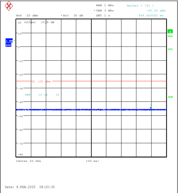
Band38-5MHz-16QAM-37775-1RB#0-20000~2700 0-PASS
