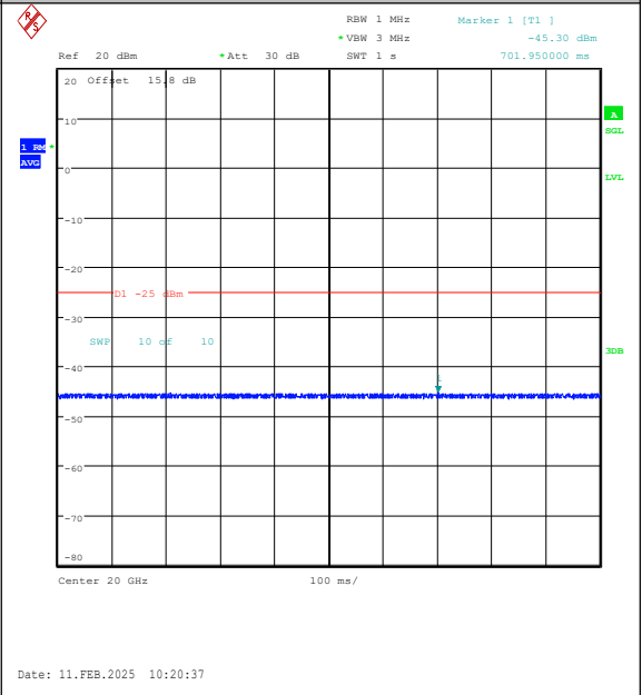
Band38-20MHz-16QAM-37850-1RB#0-20000~270 00-PASS
