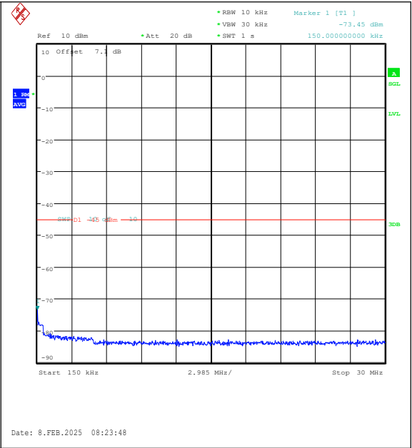
Band38-5MHz-QPSK-38225-1RB#0-0.15~30-PAS
