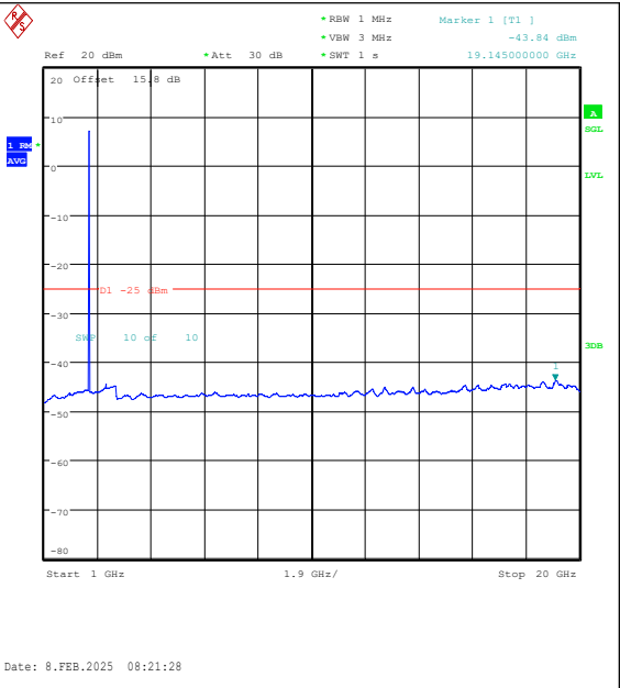
Band38-5MHz-QPSK-38000-1RB#0-1000~20000- PASS
