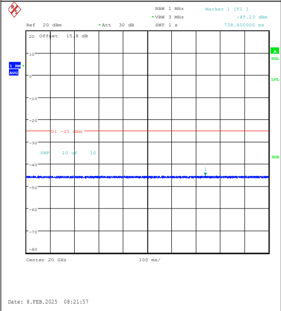
Band38-5MHz-QPSK-38000-1RB#0-20000~2700 0-PASS
