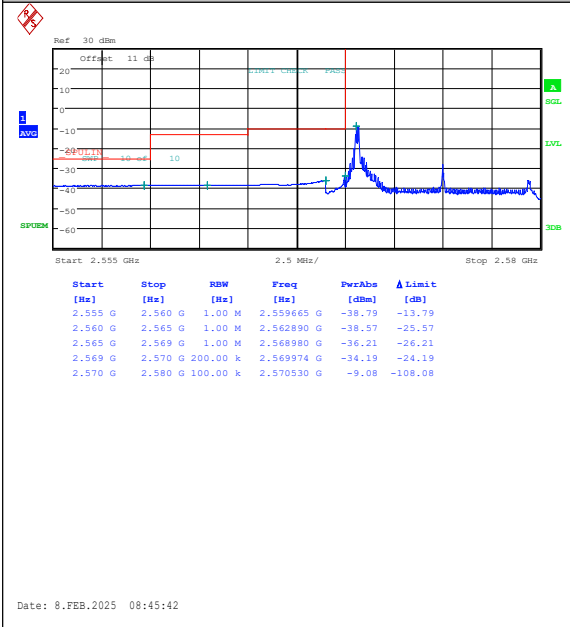
Band38-10MHz-QPSK-37800-1RB#0-PASS
