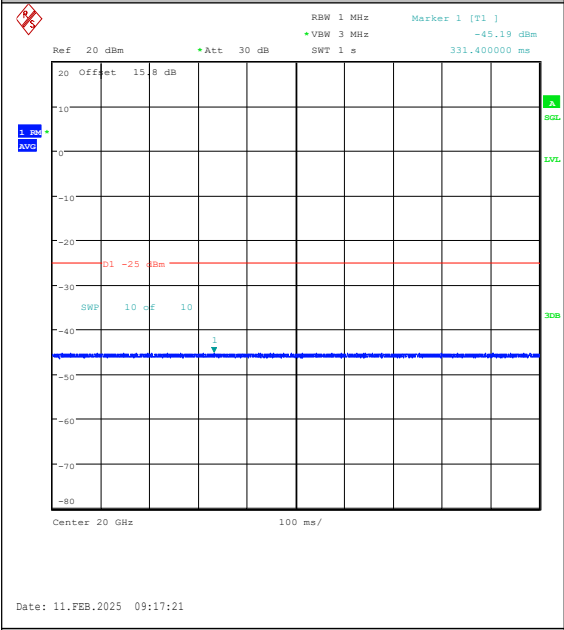
Band38-10MHz-QPSK-38200-1RB#0-20000~270 00-PASS
