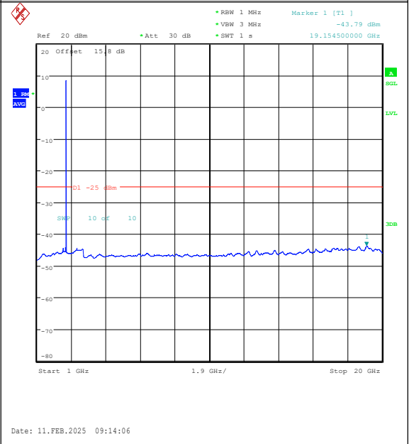
Band38-10MHz-QPSK-38000-1RB#0-1000~20000 -PASS
