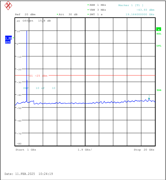
Band38-20MHz-QPSK-38150-1RB#0-1000~20000 -PASS
