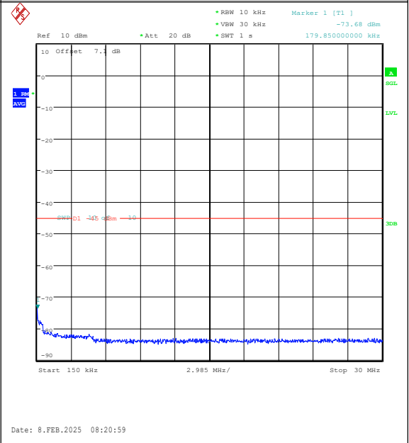
Band38-5MHz-QPSK-38000-1RB#0-0.15~30-PAS S
