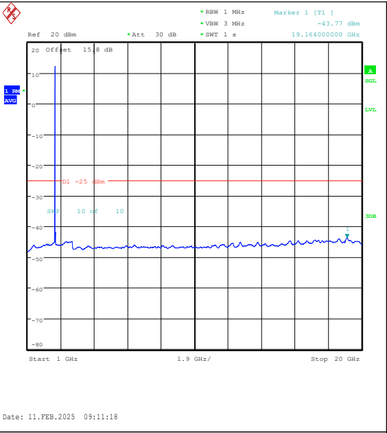
Band38-10MHz-QPSK-37800-1RB#0-1000~20000 -PASS
