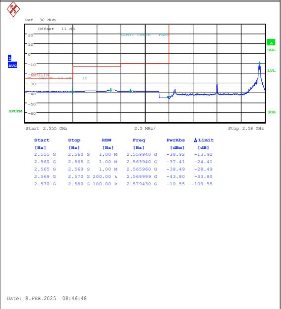
Band38-10MHz-QPSK-37800-1RB#49-PASS
