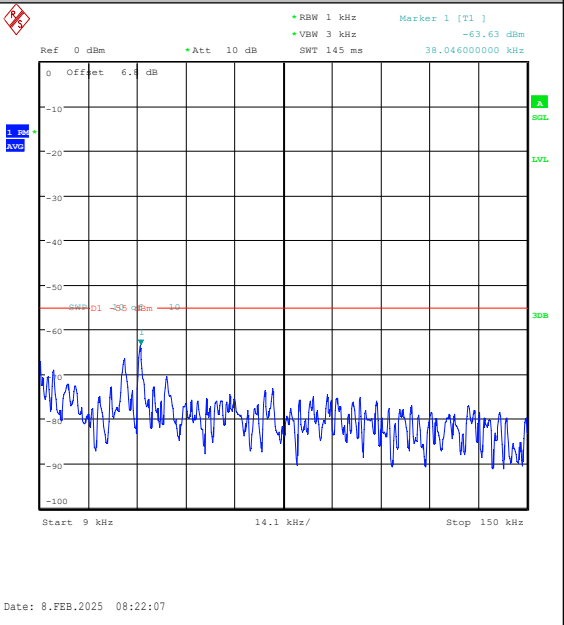
Band38-5MHz-16QAM-38000-1RB#0-0.009~0.15- PASS
