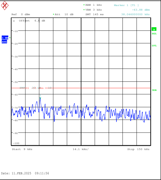
Band38-10MHz-16QAM-37800-1RB#0-0.009~0.15 -PASS
