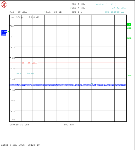
Band38-5MHz-16QAM-38000-1RB#0-20000~2700 0-PASS
