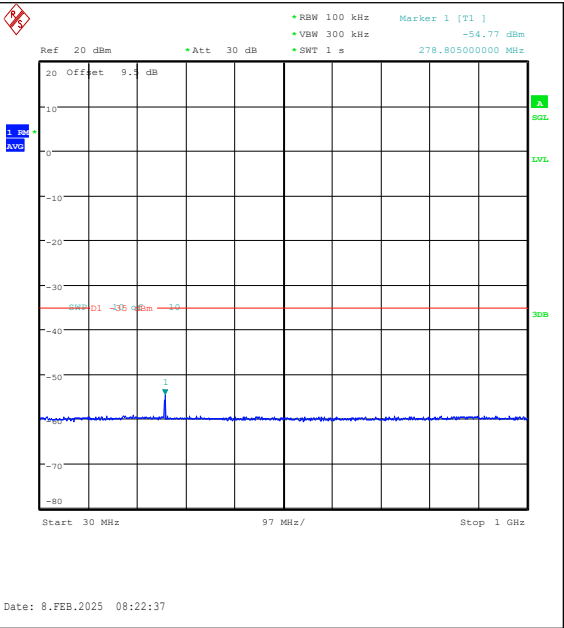
Band38-5MHz-16QAM-38000-1RB#0-30~1000-PA SS
