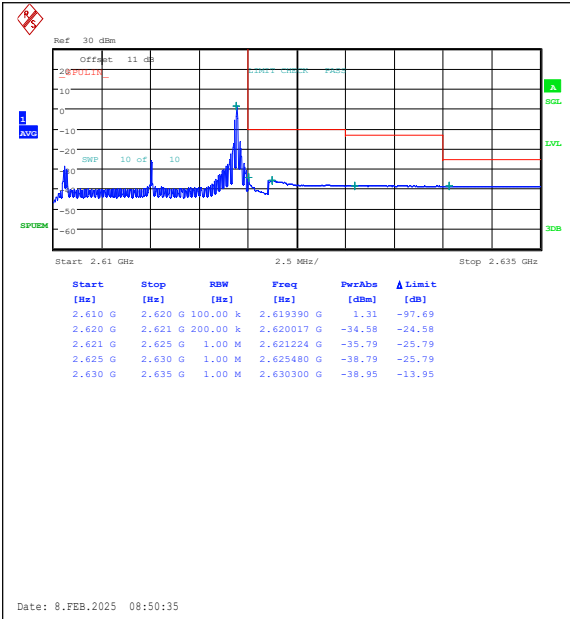
Band38-10MHz-16QAM-38200-1RB#49-PASS
