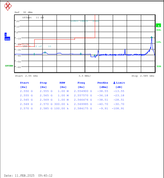
Band38-15MHz-QPSK-37825-1RB#74-PASS
