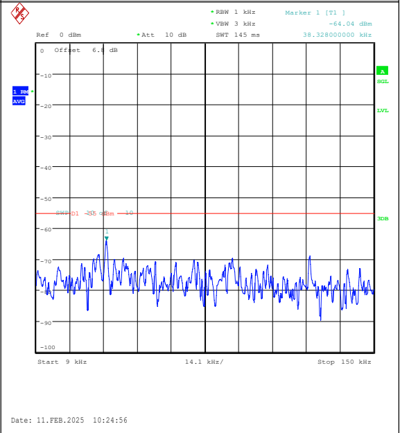
Band38-20MHz-16QAM-38150-1RB#0-0.009~0.15 -PASS
