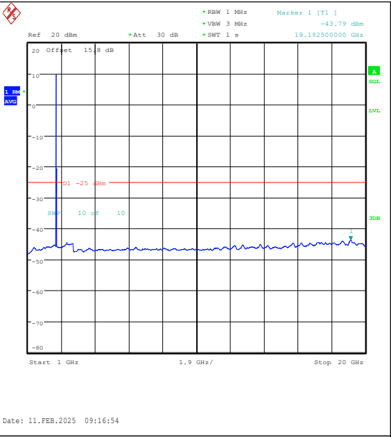
Band38-10MHz-QPSK-38200-1RB#0-1000~20000 -PASS
