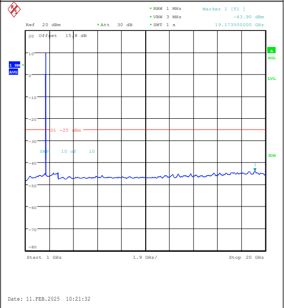
Band38-20MHz-QPSK-38000-1RB#0-1000~20000 -PASS
