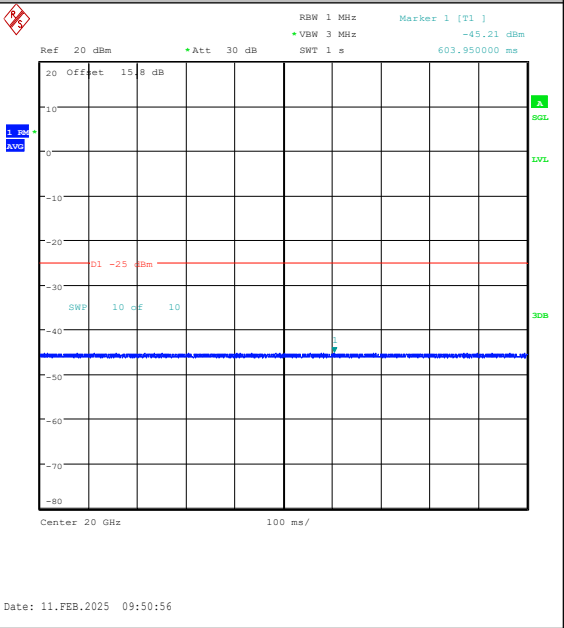
Band38-15MHz-16QAM-38000-1RB#0-20000~270 00-PASS
