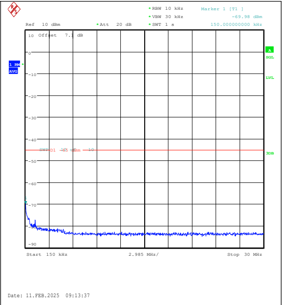
Band38-10MHz-QPSK-38000-1RB#0-0.15~30-PA SS
