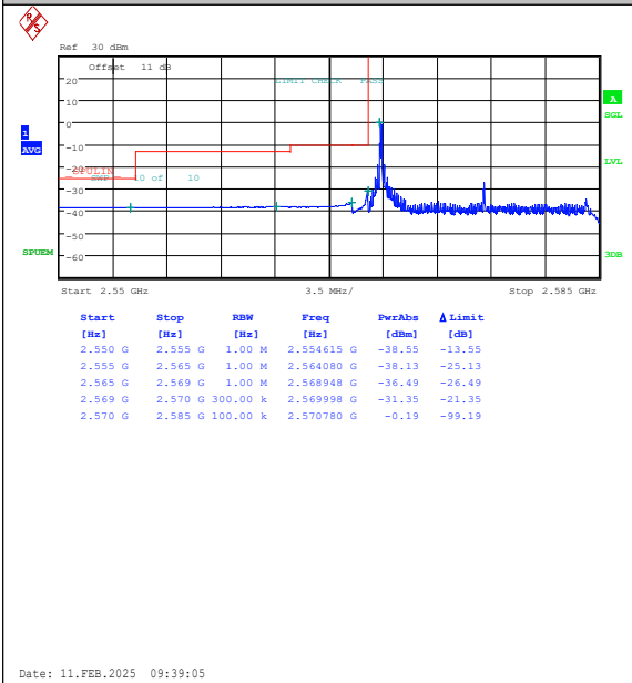
Band38-15MHz-QPSK-37825-1RB#0-PASS
