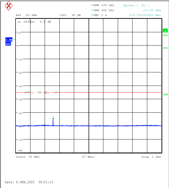
Band38-5MHz-QPSK-38000-1RB#0-30~1000-PA SS
