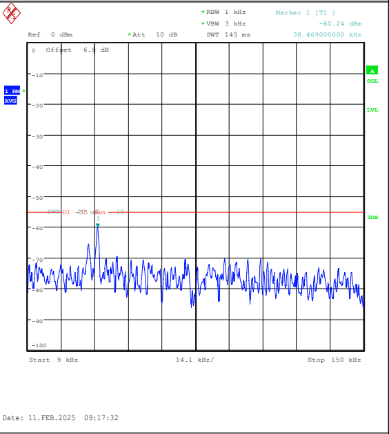
Band38-10MHz-16QAM-38200-1RB#0-0.009~0.15 -PASS
