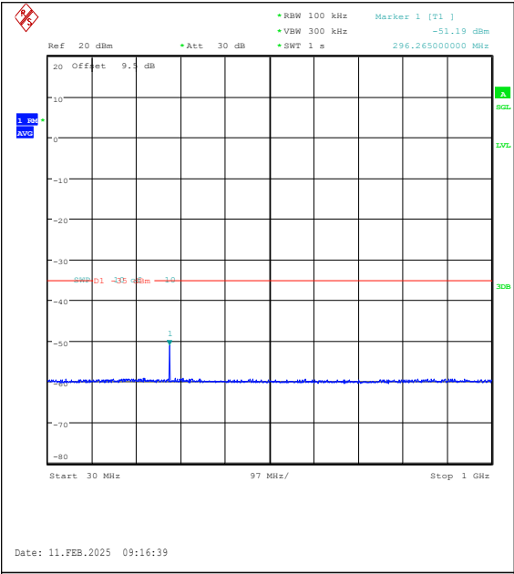
Band38-10MHz-QPSK-38200-1RB#0-30~1000-P ASS
