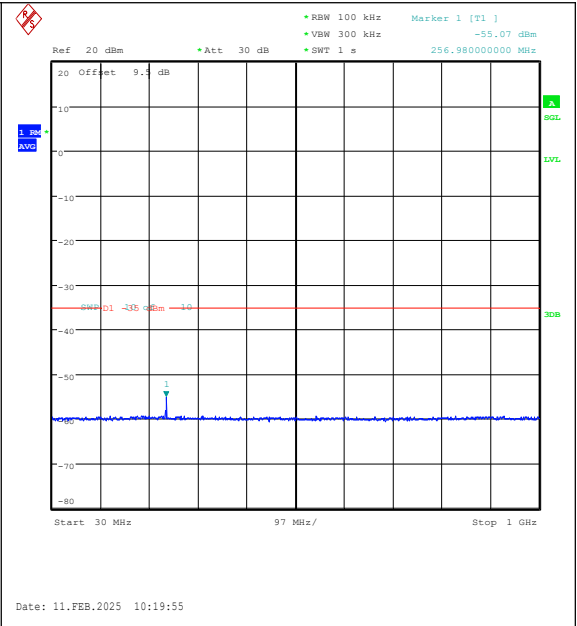
Band38-20MHz-16QAM-37850-1RB#0-30~1000-P ASS
