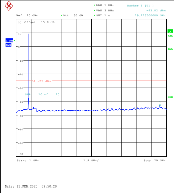
Band38-15MHz-16QAM-38000-1RB#0-1000~200 00-PASS
