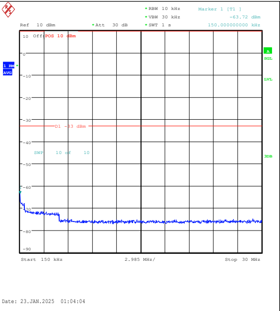
Band25-15MHz-QPSK-26115-1RB#0-0.15~30-PA-SS
