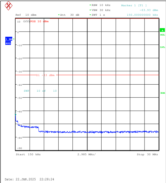
Band25-3MHz-16QAM-26675-15RB#0-0.15~30-P ASS
