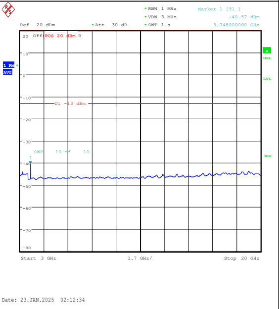
Band25-20MHz-16QAM-26365-1RB#0-3000~2000 0-PASS
