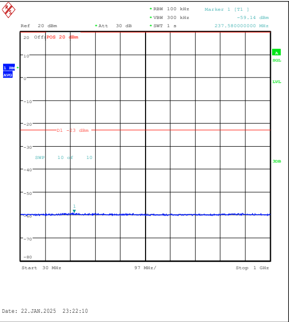
Band25-5MHz-16QAM-26665-1RB#0-30~1000-PA SS
