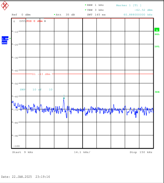
Band25-5MHz-16QAM-26365-25RB#0-0.009~0.15-PASS
