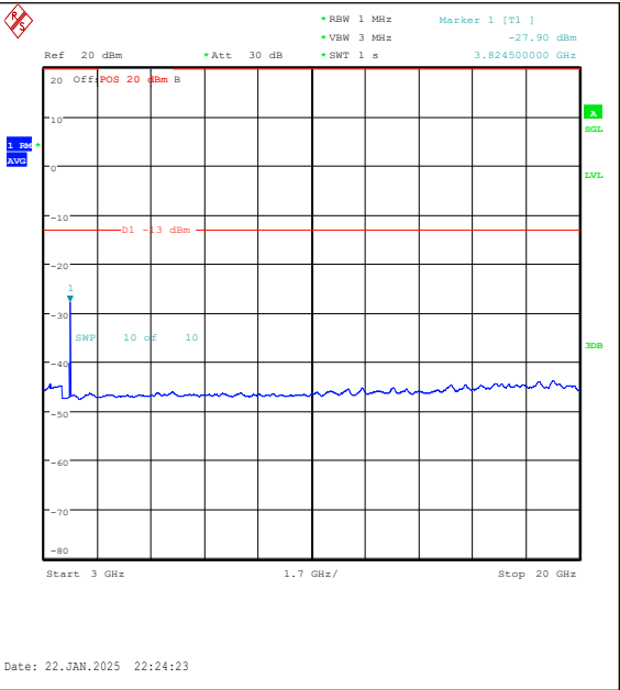
Band25-3MHz-16QAM-26675-1RB#0-3000~20000 -PASS
