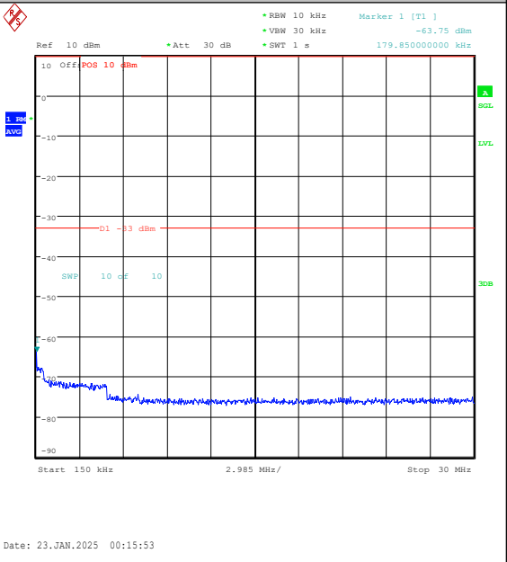
Band25-10MHz-QPSK-26365-50RB#0-0.15~30-PA SS
