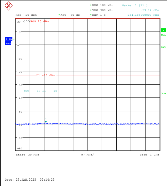
Band25-20MHz-16QAM-26365-1RB#99-30~1000-PASS
