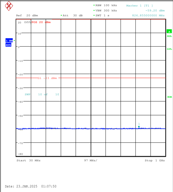
Band25-15MHz-16QAM-26115-1RB#74-30~1000-PASS
