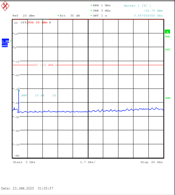
Band25-15MHz-16QAM-26115-1RB#0-3000~2000 0-PASS
