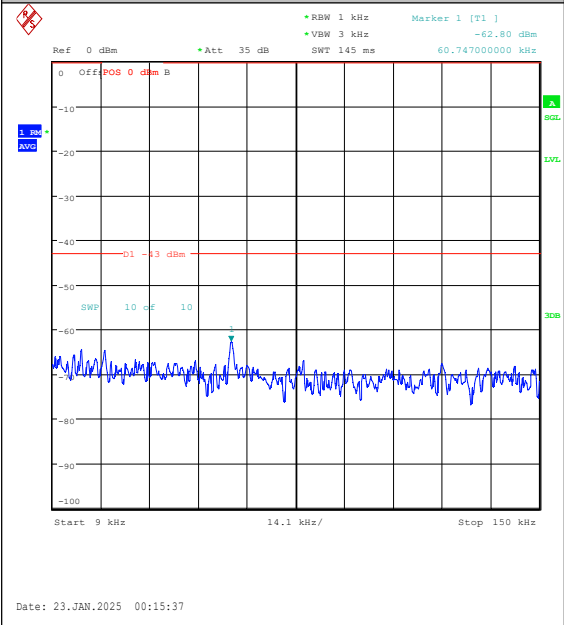
Band25-10MHz-QPSK-26365-50RB#0-0.009~0.1 5-PASS
