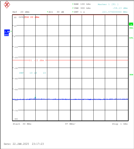
Band25-5MHz-16QAM-26365-1RB#24-30~1000-PASS
