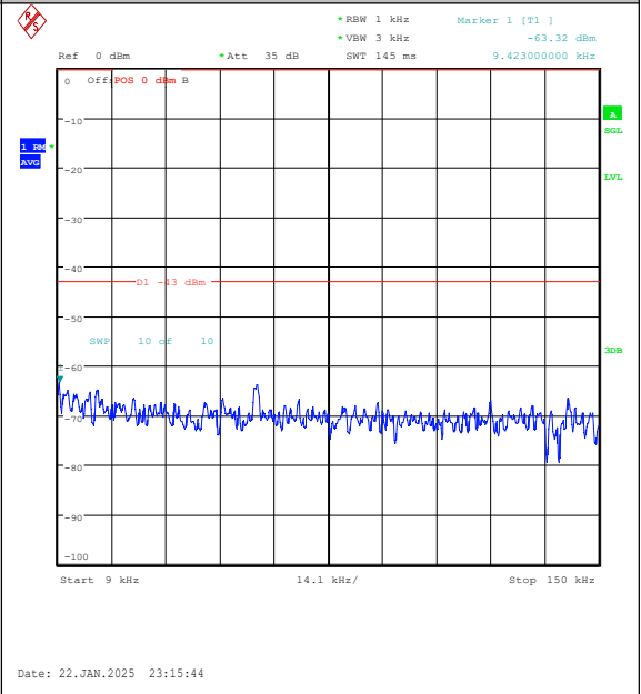
Band25-5MHz-QPSK-26365-1RB#24-0.009~0.15- PASS
