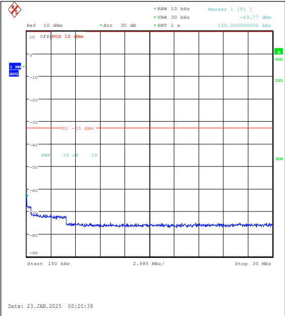
Band25-10MHz-QPSK-26640-1RB#49-0.15~30-P ASS
