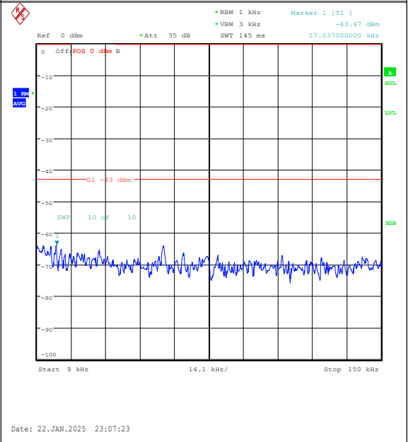
Band25-5MHz-16QAM-26065-1RB#0-0.009~0.15-P PASS
