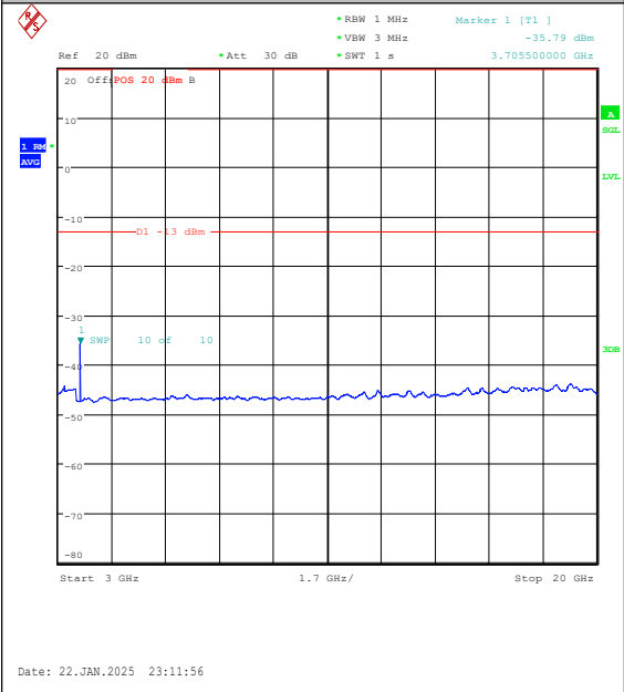
Band25-5MHz-QPSK-26065-25RB#0-3000~2000 0-PASS
