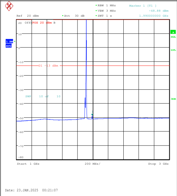
Band25-10MHz-QPSK-26640-1RB#49-1000~300 0-PASS
