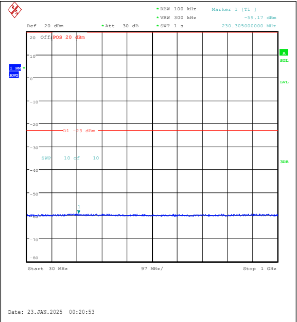
Band25-10MHz-QPSK-26640-1RB#49-30~1000-P ASS
