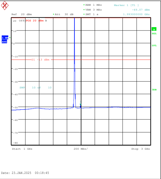
Band25-10MHz-QPSK-26640-1RB#0-1000~3000- PASS
