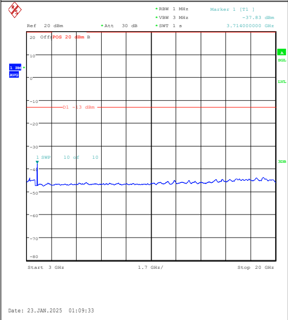
Band25-15MHz-QPSK-26115-75RB#0-3000~200 00-PASS
