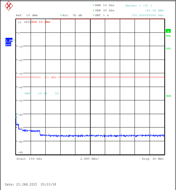
Band25-10MHz-QPSK-26090-1RB#0-0.15~30-PA SS
