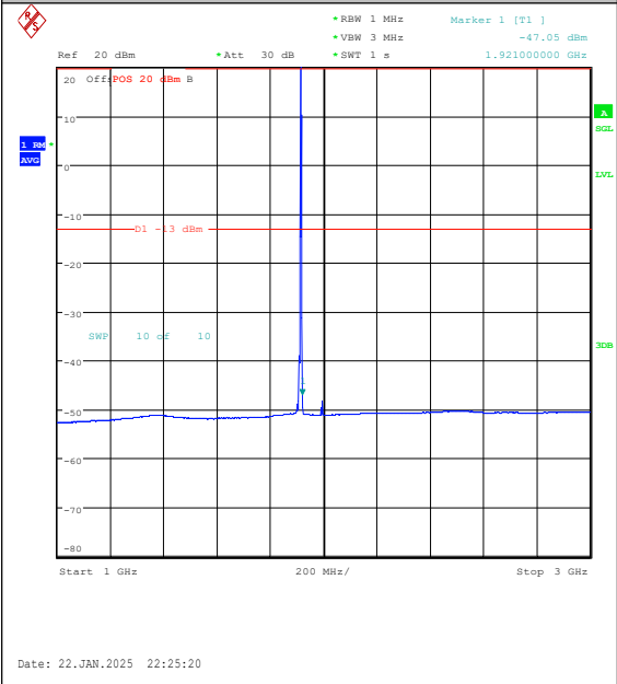
Band25-3MHz-QPSK-26675-1RB#14-1000~3000 -PASS
