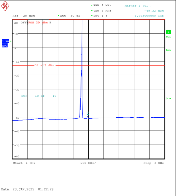
Band25-15MHz-16QAM-26615-1RB#74-1000~3000-PASS
