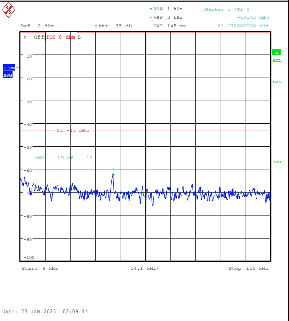
Band25-20MHz-16QAM-26140-100RB#0-0.009~0. 15-PASS
