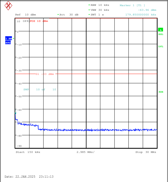
Band25-5MHz-QPSK-26065-25RB#0-0.15~30-PA SS
