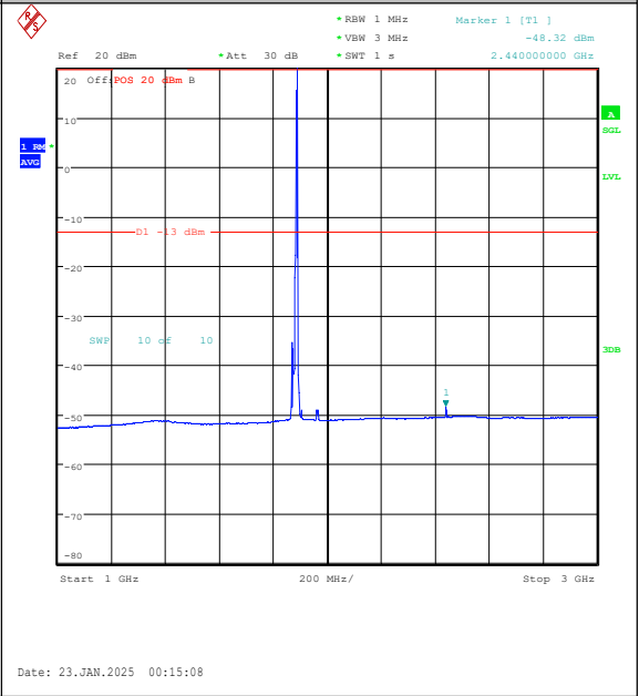
Band25-10MHz-16QAM-26365-1RB#49-1000~300 0-PASS
