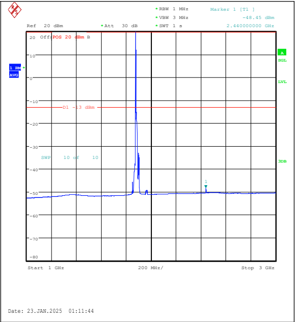
Band25-15MHz-QPSK-26365-1RB#0-1000~3000- PASS
