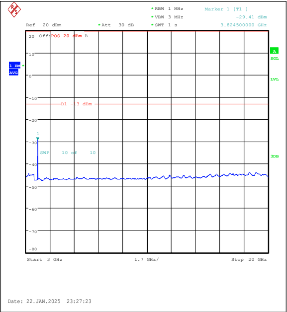
Band25-5MHz-16QAM-26665-25RB#0-3000~2000 0-PASS
