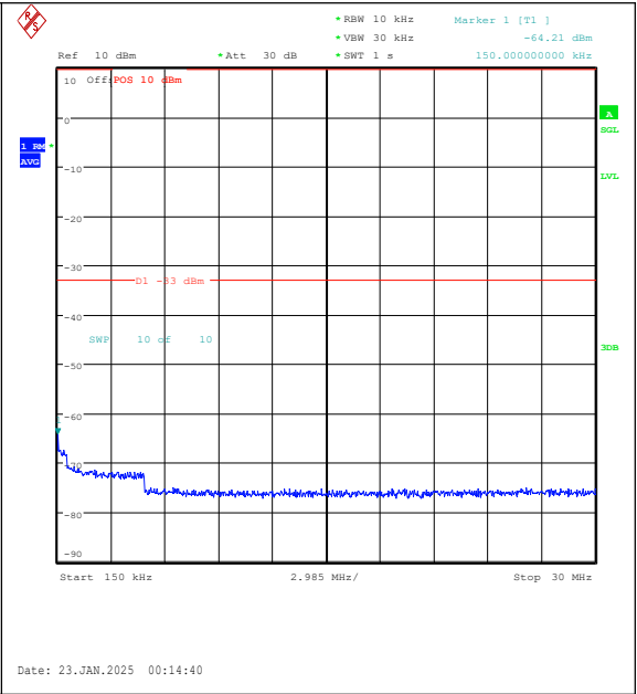
Band25-10MHz-16QAM-26365-1RB#49-0.15~30-P ASS
