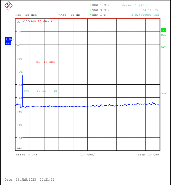
Band25-10MHz-QPSK-26640-1RB#49-3000~2000 0-PASS
