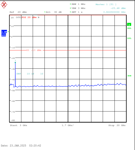
Band25-20MHz-QPSK-26590-1RB#99-3000~2000 0-PASS
