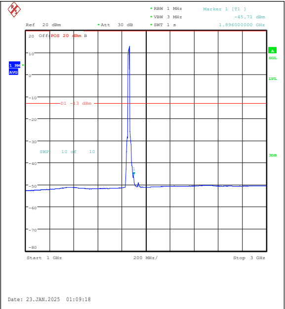
Band25-15MHz-QPSK-26115-75RB#0-1000~3000 -PASS
