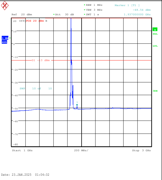
Band25-15MHz-QPSK-26115-1RB#0-1000~3000-PASS
