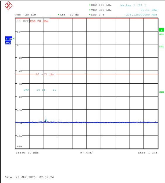
Band25-20MHz-16QAM-26140-1RB#99-30~1000 -PASS
