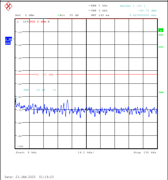
Band25-15MHz-16QAM-26615-1RB#0-0.009~0.15-PASS
