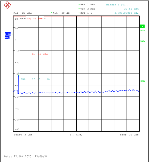
Band25-5MHz-QPSK-26065-1RB#24-3000~20000 -PASS
