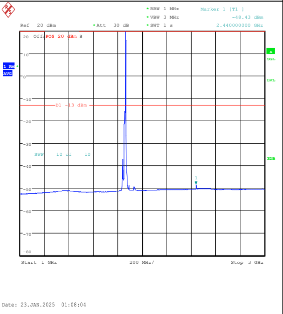
Band25-15MHz-16QAM-26115-1RB#74-1000~3000-PASS
