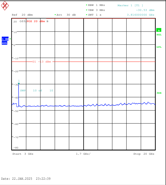
Band25-5MHz-16QAM-26665-1RB#0-3000~20000 -PASS
