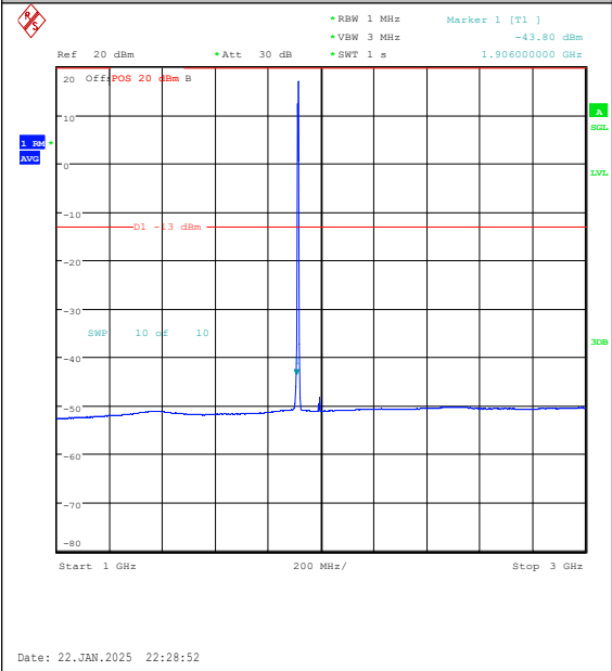
Band25-3MHz-16QAM-26675-15RB#0-1000~300 0-PASS
