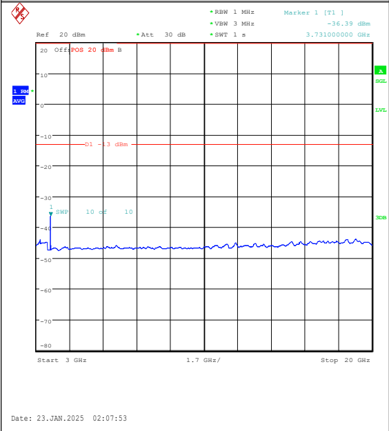
Band25-20MHz-16QAM-26140-1RB#99-3000~20 000-PASS
