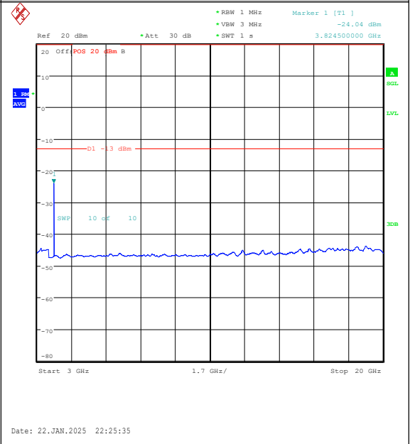
Band25-3MHz-QPSK-26675-1RB#14-3000~20000 -PASS
