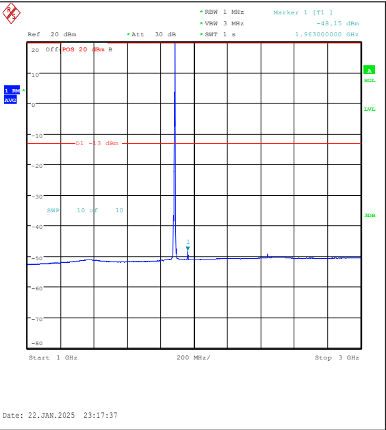
Band25-5MHz-16QAM-26365-1RB#24-1000~3000-PASS
