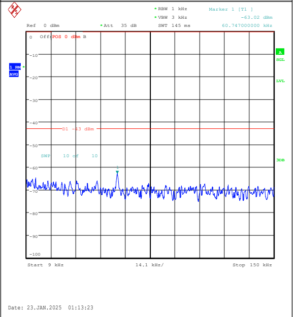
Band25-15MHz-QPSK-26365-1RB#74-0.009~0.15 -PASS
