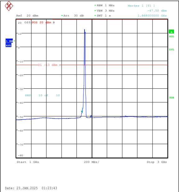
Band25-15MHz-QPSK-26615-75RB#0-1000~3000-PASS
