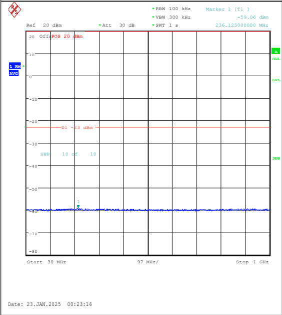
Band25-10MHz-QPSK-26640-50RB#0-30~1000- PASS
