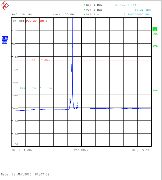
Band25-20MHz-16QAM-26140-1RB#99-1000~300 0-PASS
