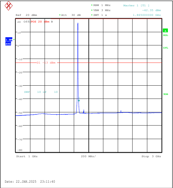
Band25-5MHz-QPSK-26065-25RB#0-1000~3000-P PASS
