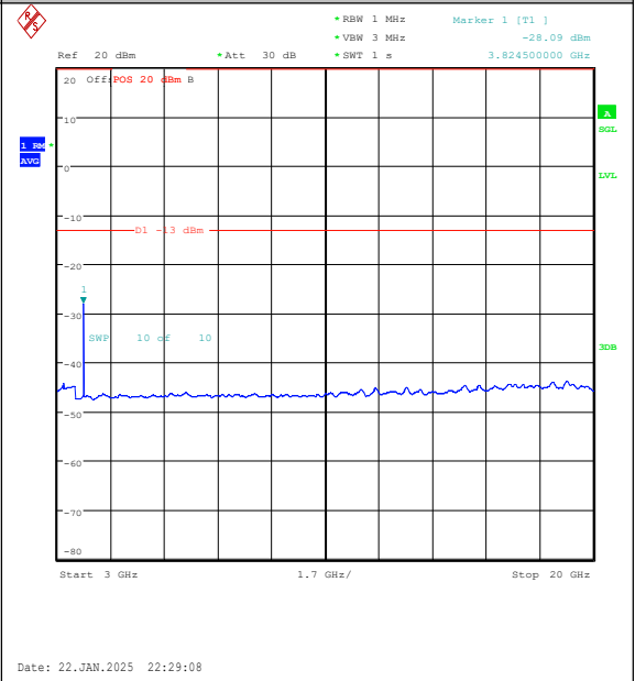
Band25-3MHz-16QAM-26675-15RB#0-3000~2000 0-PASS
