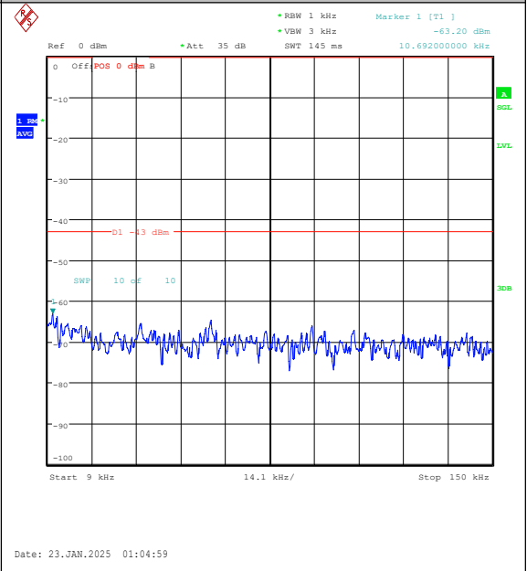
Band25-15MHz-16QAM-26115-1RB#0-0.009~0.15 -PASS
