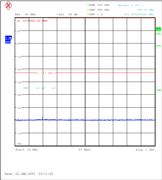
Band25-5MHz-QPSK-26065-25RB#0-30~1000-P ASS
