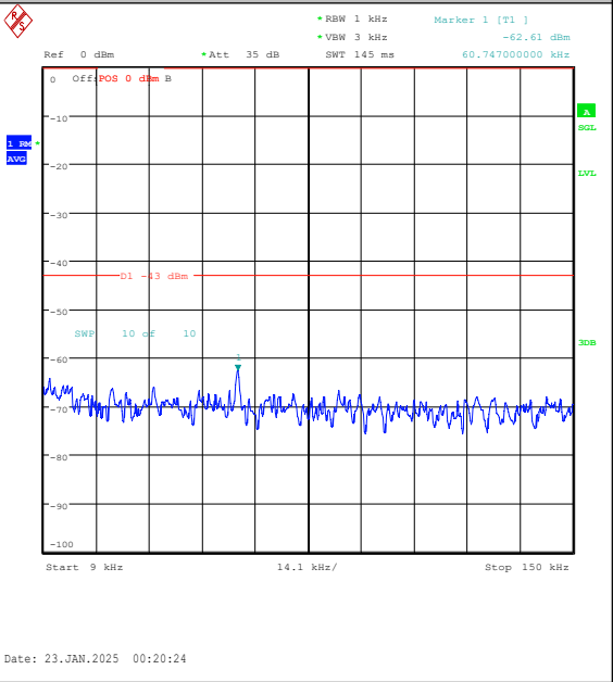
Band25-10MHz-QPSK-26640-1RB#49-0.009~0.15 -PASS
