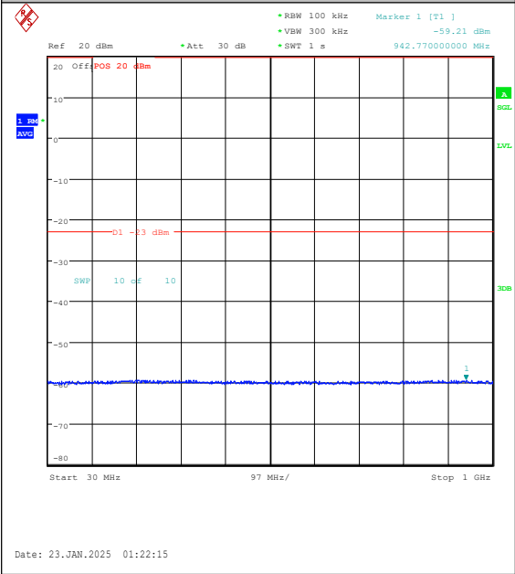
Band25-15MHz-16QAM-26615-1RB#74-30~1000-PASS
