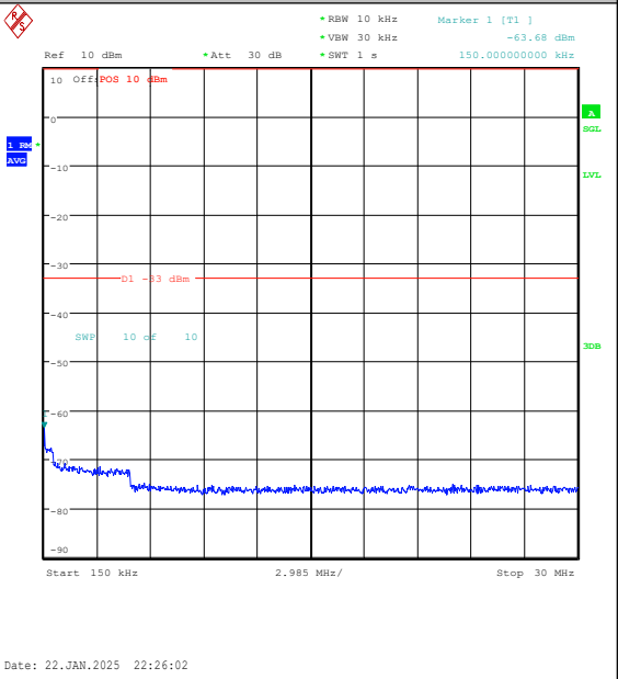
Band25-3MHz-16QAM-26675-1RB#14-0.15~30-P ASS
