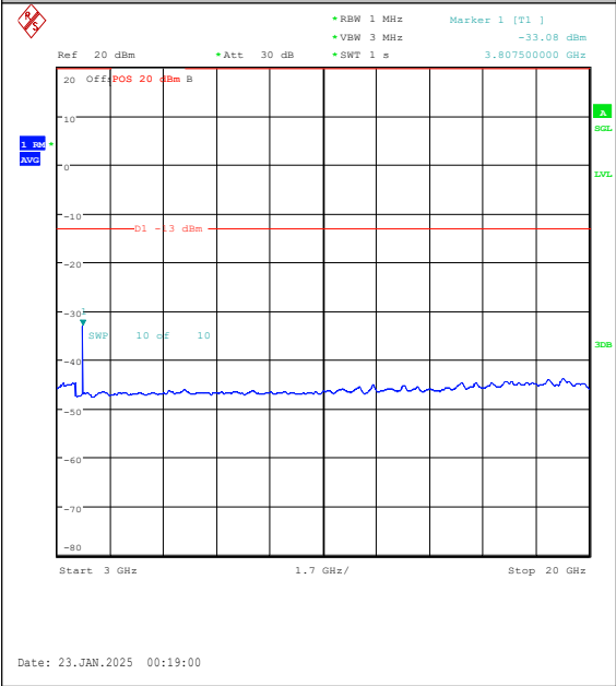
Band25-10MHz-QPSK-26640-1RB#0-3000~2000 0-PASS
