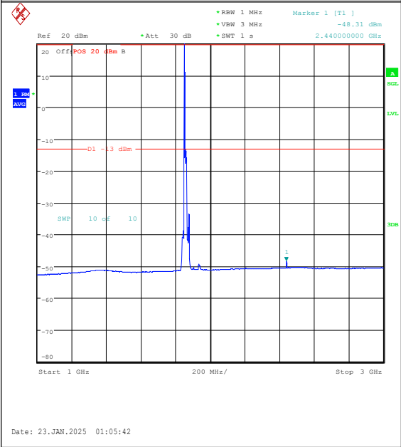
Band25-15MHz-16QAM-26115-1RB#0-1000~300 0-PASS
