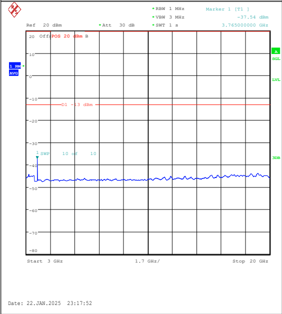
Band25-5MHz-16QAM-26365-1RB#24-3000~20000-PASS
