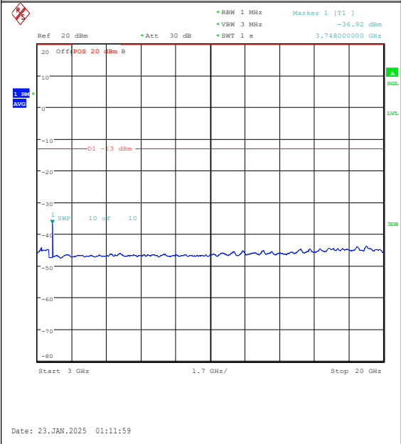
Band25-15MHz-QPSK-26365-1RB#0-3000~2000 0-PASS
