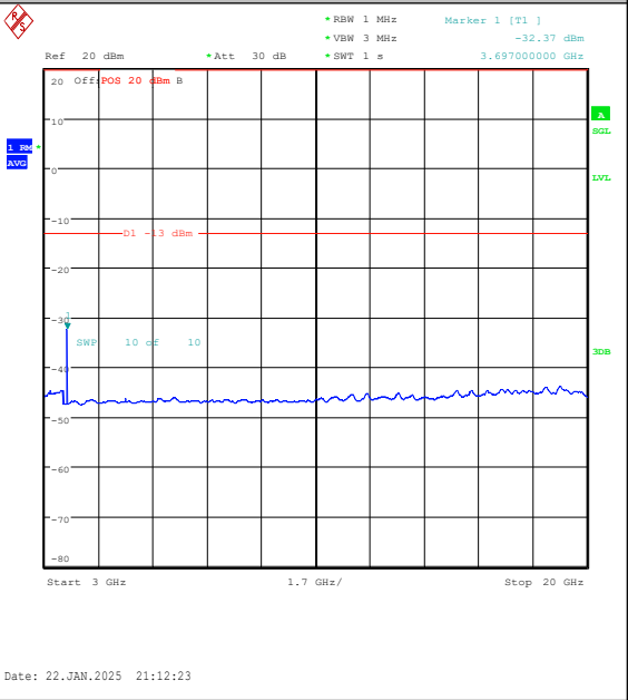
Band25-1.4MHz-16QAM-26047-1RB#0-3000~20000-PASS
