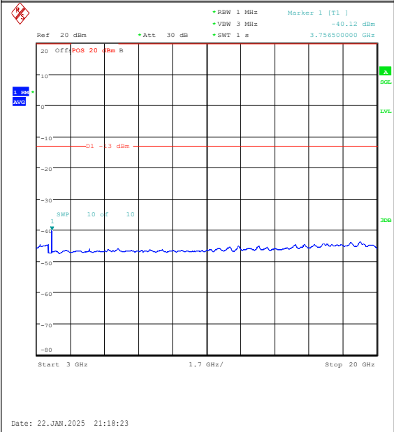
Band25-1.4MHz-QPSK-26365-1RB#0-3000~2000 0-PASS
