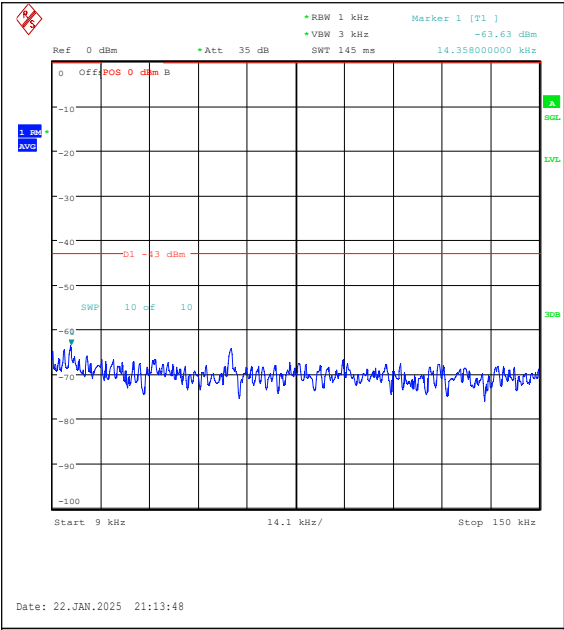
Band25-1.4MHz-16QAM-26047-1RB#5-0.009~0. 15-PASS
