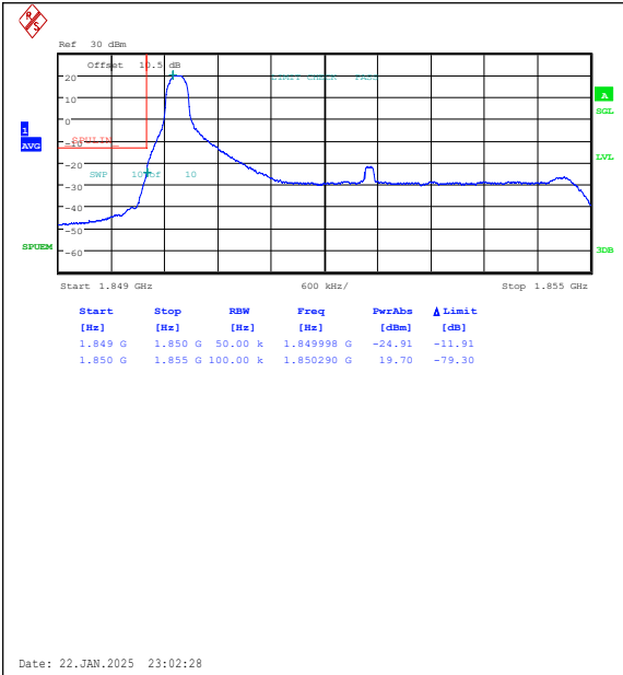
Band25-5MHz-QPSK-26065-1RB#0-PASS
