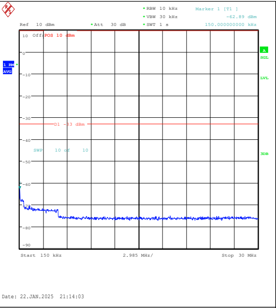
Band25-1.4MHz-16QAM-26047-1RB#5-0.15~30-P ASS
