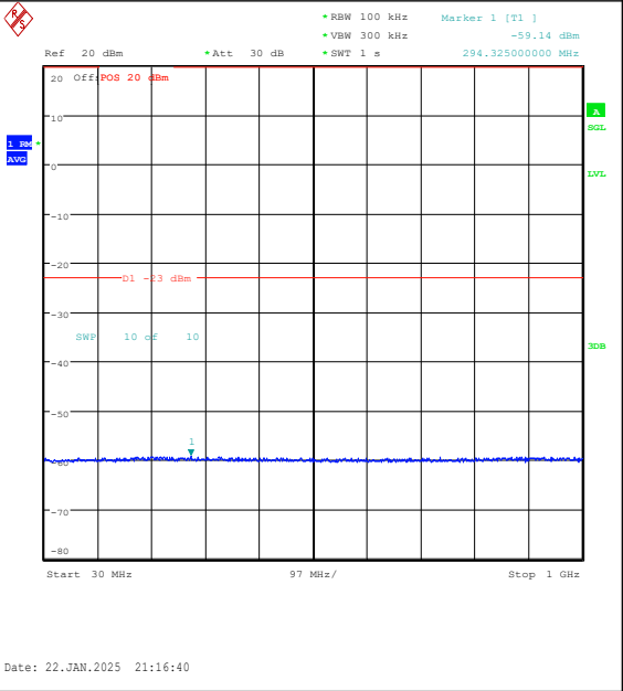
Band25-1.4MHz-16QAM-26047-6RB#0-30~1000-PASS
