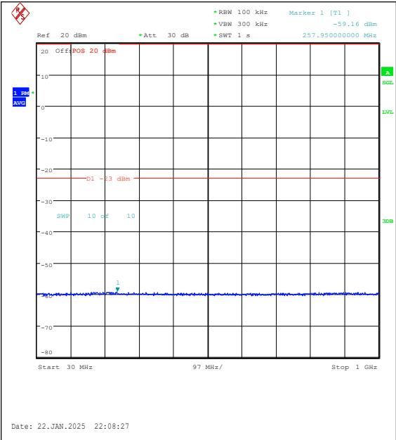
Band25-3MHz-QPSK-26055-1RB#0-30~1000-PA SS
