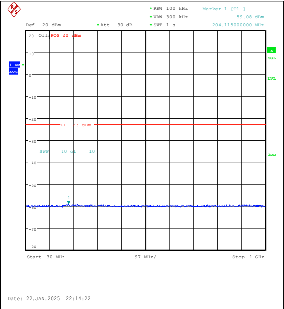
Band25-3MHz-16QAM-26055-15RB#0-30~1000-P ASS
