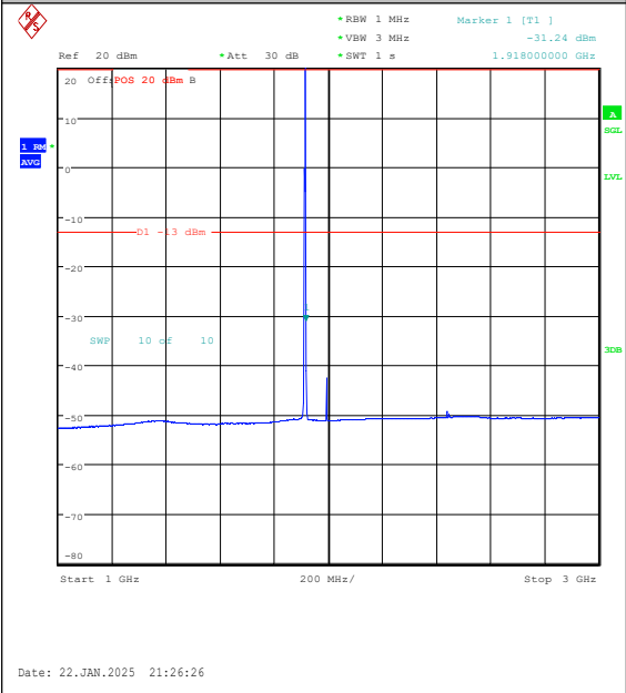
Band25-1.4MHz-16QAM-26683-1RB#0-1000~3000-PASS
