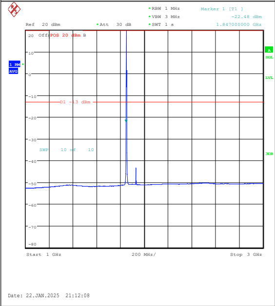
Band25-1.4MHz-16QAM-26047-1RB#0-1000~3000-PASS
