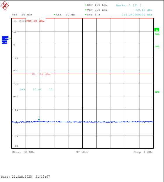
Band25-1.4MHz-QPSK-26047-1RB#5-30~1000-PA SS
