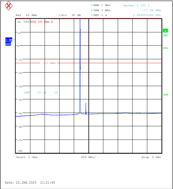
Band25-1.4MHz-16QAM-26365-1RB#5-1000~300 0-PASS
