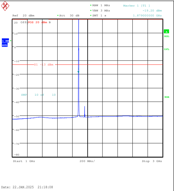
Band25-1.4MHz-QPSK-26365-1RB#0-1000~3000- PASS
