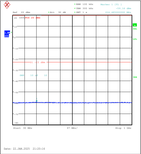
Band25-1.4MHz-QPSK-26365-1RB#5-30~1000-PA SS
