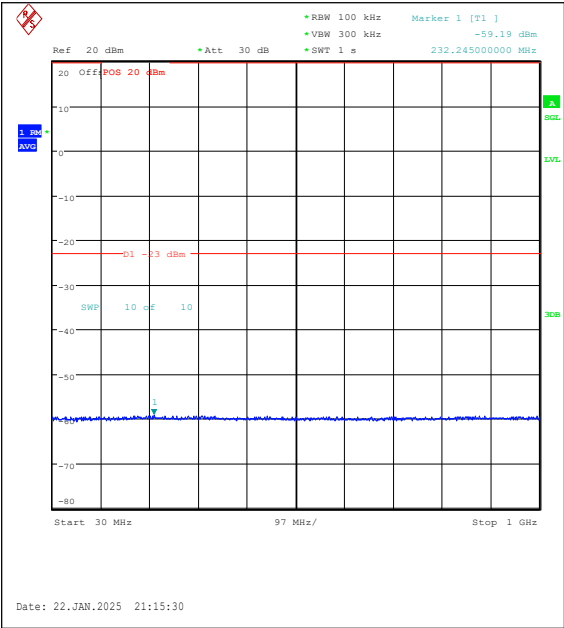
Band25-1.4MHz-QPSK-26047-6RB#0-30~1000-P ASS
