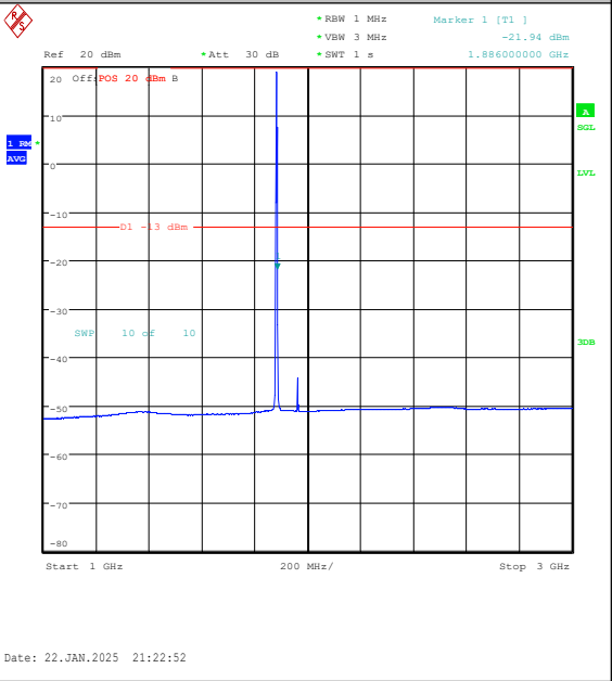
Band25-1.4MHz-QPSK-26365-6RB#0-1000~3000- PASS
