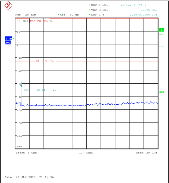
Band25-1.4MHz-QPSK-26047-1RB#5-3000~2000 0-PASS
