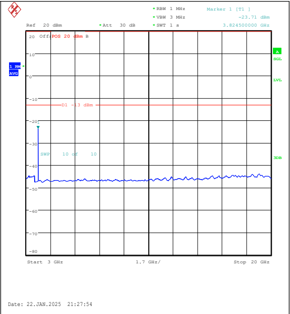
Band25-1.4MHz-QPSK-26683-1RB#5-3000~2000 0-PASS
