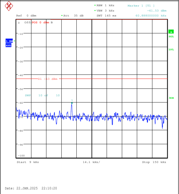
Band25-3MHz-QPSK-26055-1RB#14-0.009~0.15- PASS
