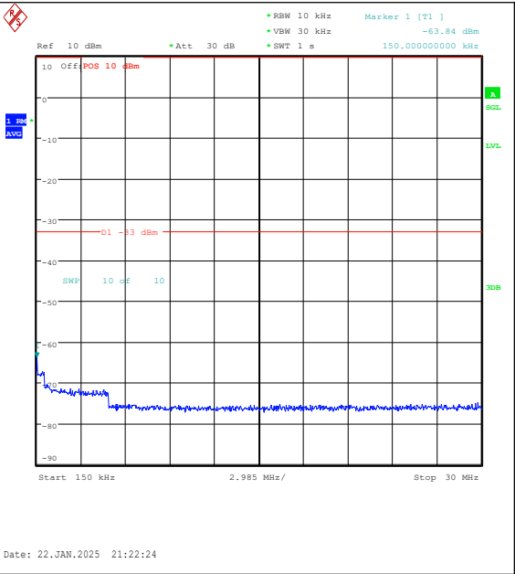
Band25-1.4MHz-QPSK-26365-6RB#0-0.15~30-PA SS
