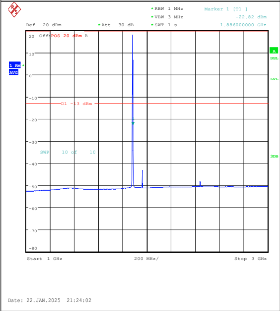
Band25-1.4MHz-16QAM-26365-6RB#0-1000~3000-PASS
