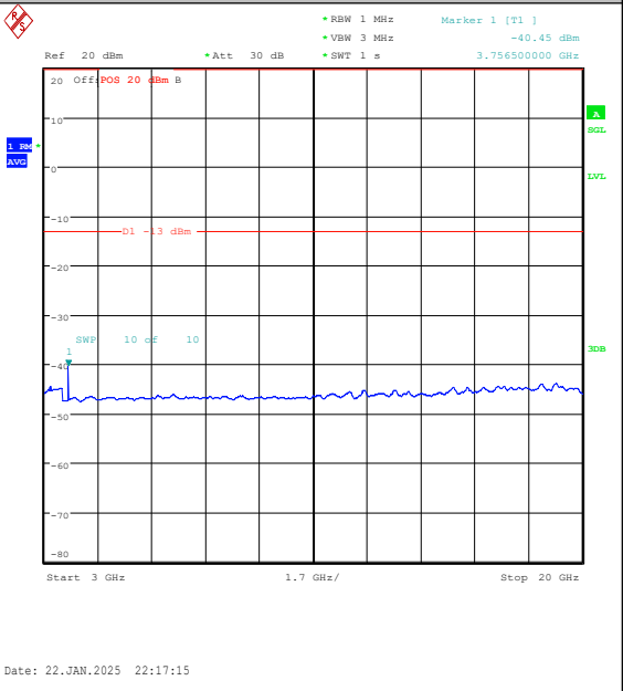
Band25-3MHz-16QAM-26365-1RB#0-3000~20000 -PASS
