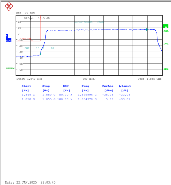
Band25-5MHz-QPSK-26065-25RB#0-PASS
