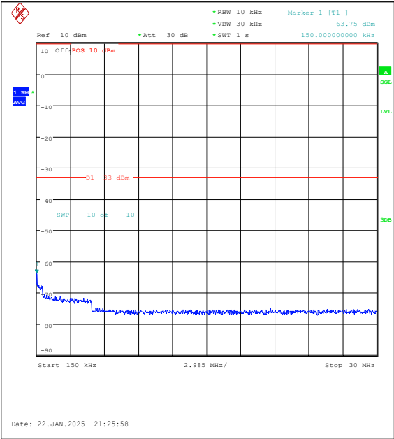
Band25-1.4MHz-16QAM-26683-1RB#0-0.15~30-PASS
