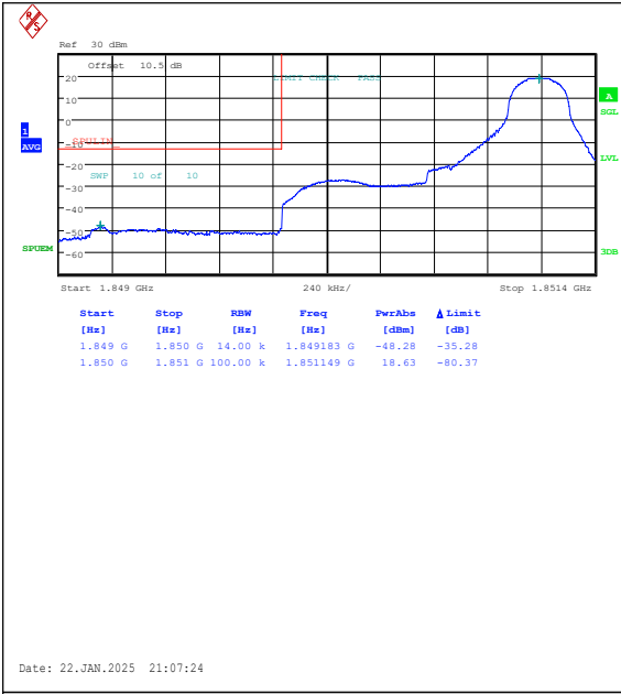
Band25-1.4MHz-16QAM-26047-1RB#5-PASS
