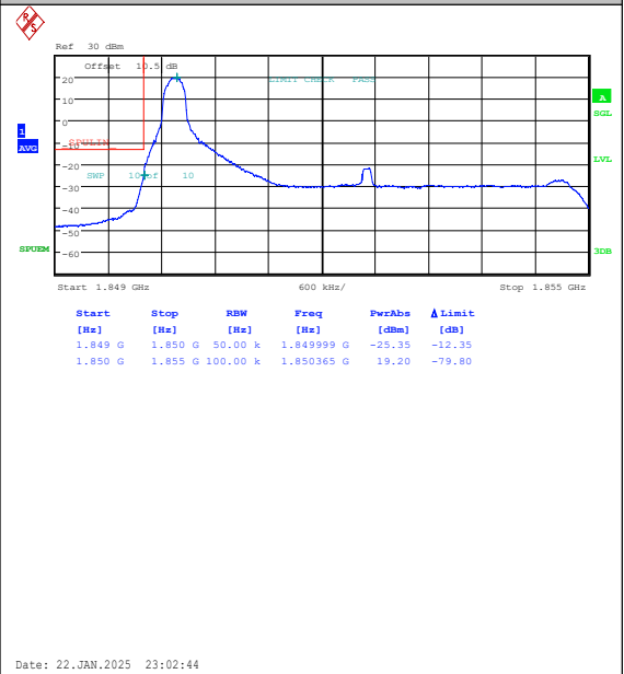
Band25-5MHz-16QAM-26065-1RB#0-PASS
