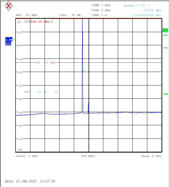
Band25-1.4MHz-QPSK-26683-1RB#5-1000~3000 -PASS
