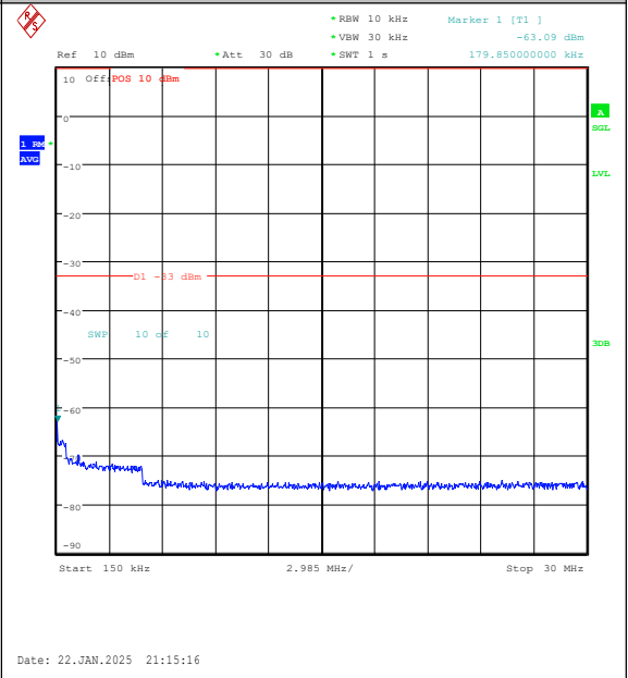
Band25-1.4MHz-QPSK-26047-6RB#0-0.15~30-PA SS
