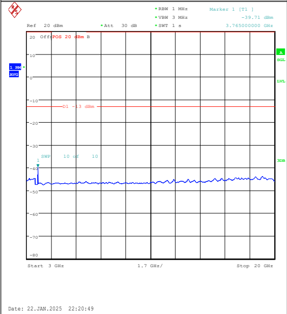
Band25-3MHz-QPSK-26365-15RB#0-3000~2000 0-PASS
