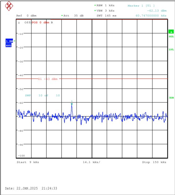
Band25-1.4MHz-QPSK-26683-1RB#0-0.009~0.15 -PASS
