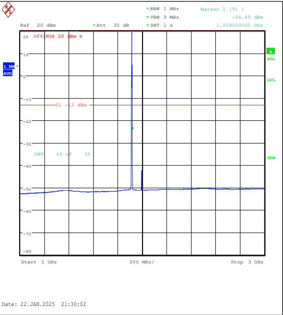
Band25-1.4MHz-QPSK-26683-6RB#0-1000~3000- PASS
