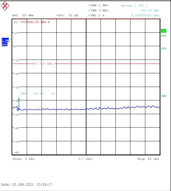
Band25-1.4MHz-16QAM-26365-6RB#0-3000~20000-PASS
