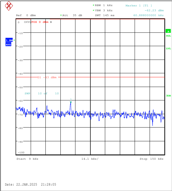
Band25-1.4MHz-16QAM-26683-1RB#5-0.009~0. 15-PASS
