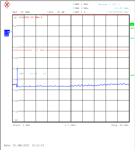
Band25-1.4MHz-QPSK-26047-1RB#0-3000~2000 0-PASS
