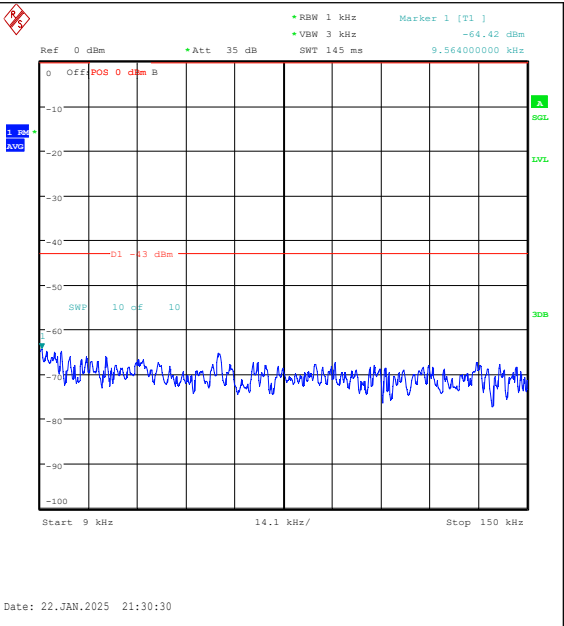
Band25-1.4MHz-16QAM-26683-6RB#0-0.009~0.15-PASS
