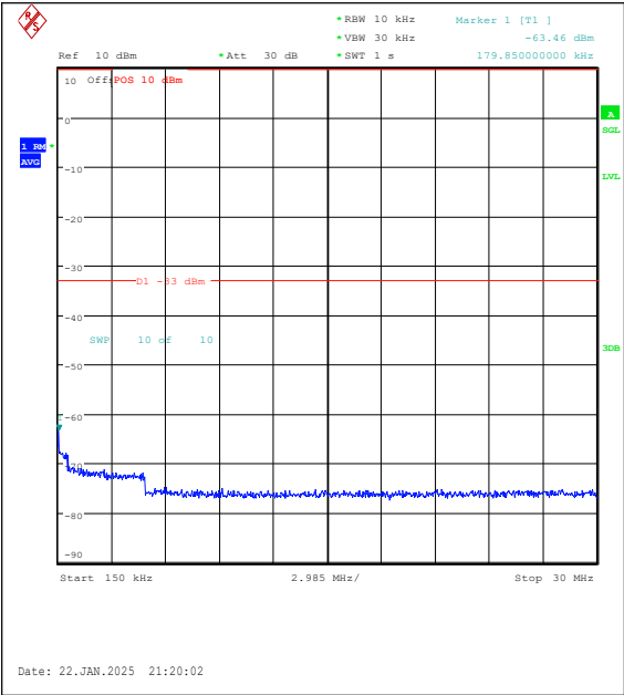
Band25-1.4MHz-QPSK-26365-1RB#5-0.15~30-P ASS
