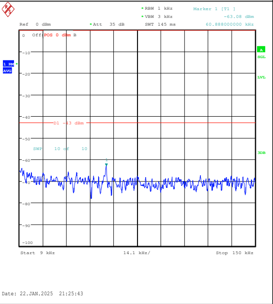
Band25-1.4MHz-16QAM-26683-1RB#0-0.009~0.1 5-PASS
