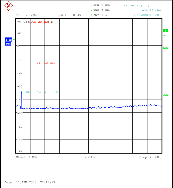
Band25-3MHz-16QAM-26055-15RB#0-3000~2000 0-PASS
