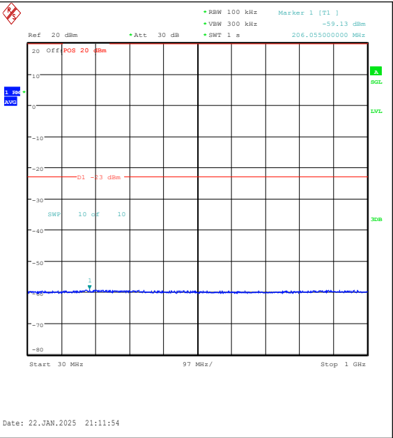
Band25-1.4MHz-16QAM-26047-1RB#0-30~1000-P ASS
