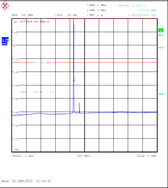
Band25-1.4MHz-16QAM-26047-1RB#5-1000~3000- PASS
