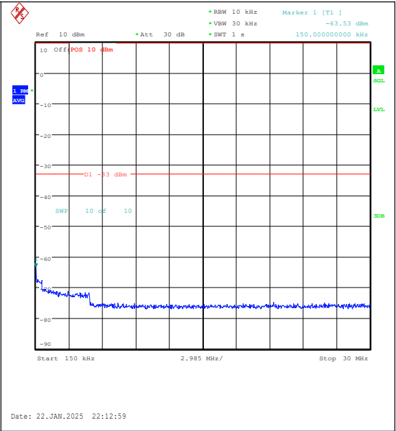
Band25-3MHz-QPSK-26055-15RB#0-0.15~30-PA SS
