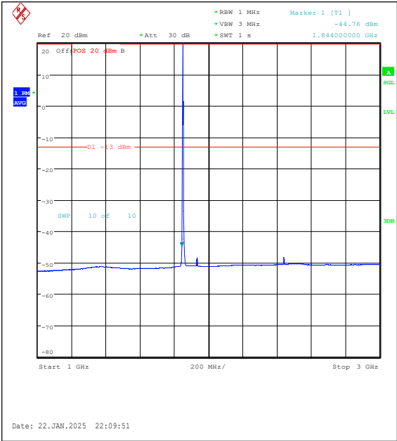
Band25-3MHz-16QAM-26055-1RB#0-1000~3000 -PASS
