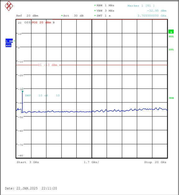
Band25-3MHz-QPSK-26055-1RB#14-3000~20000 -PASS
