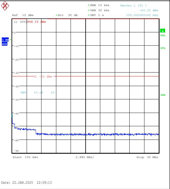
Band25-3MHz-QPSK-26055-1RB#0-0.15~30-PAS S
