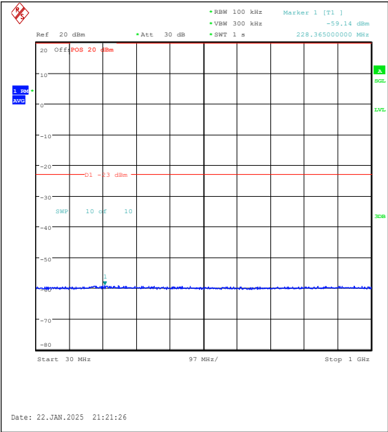
Band25-1.4MHz-16QAM-26365-1RB#5-30~1000-PASS
