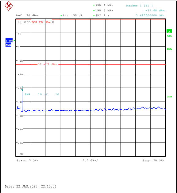
Band25-3MHz-16QAM-26055-1RB#0-3000~20000 -PASS
