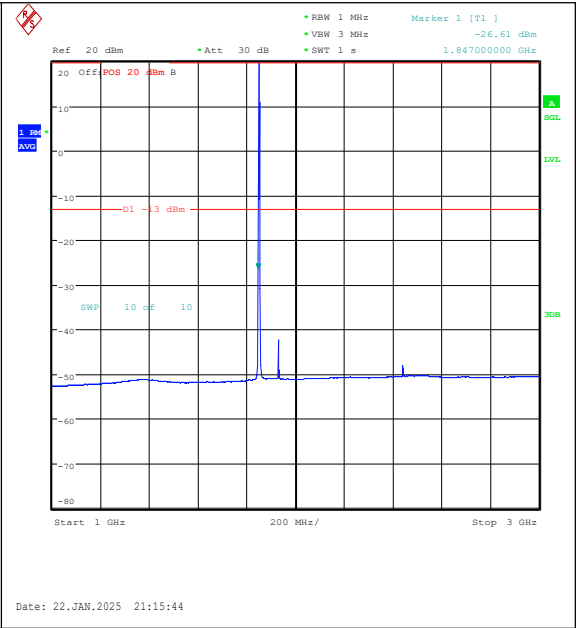
Band25-1.4MHz-QPSK-26047-6RB#0-1000~3000- PASS
