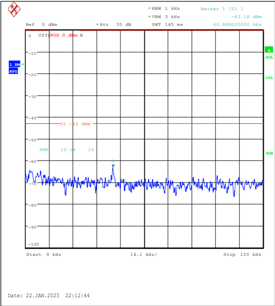
Band25-3MHz-QPSK-26055-15RB#0-0.009~0.15 -PASS
