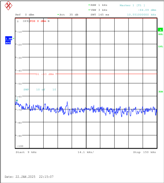
Band25-3MHz-QPSK-26365-1RB#0-0.009~0.15-PASS
