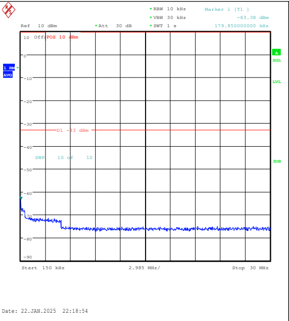
Band25-3MHz-16QAM-26365-1RB#14-0.15~30-P ASS
