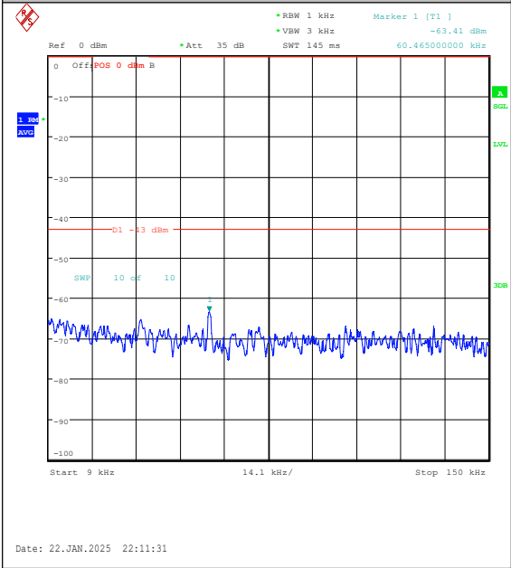
Band25-3MHz-16QAM-26055-1RB#14-0.009~0.1 5-PASS
