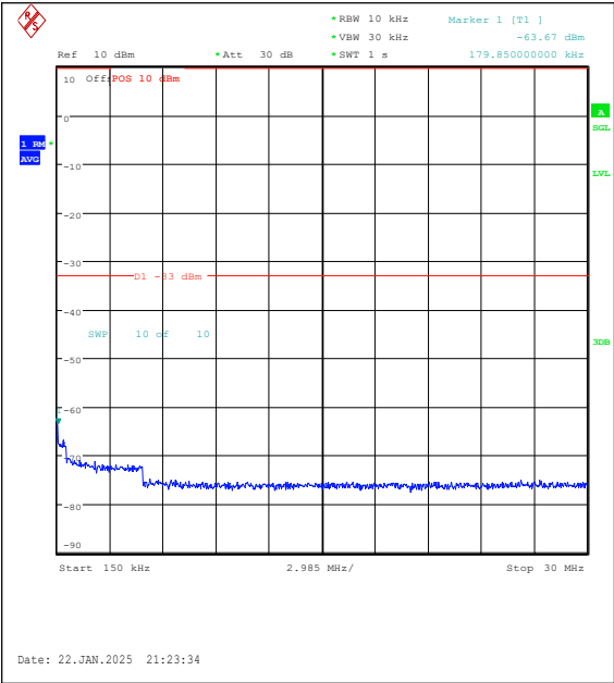
Band25-1.4MHz-16QAM-26365-6RB#0-0.15~30-PASS
