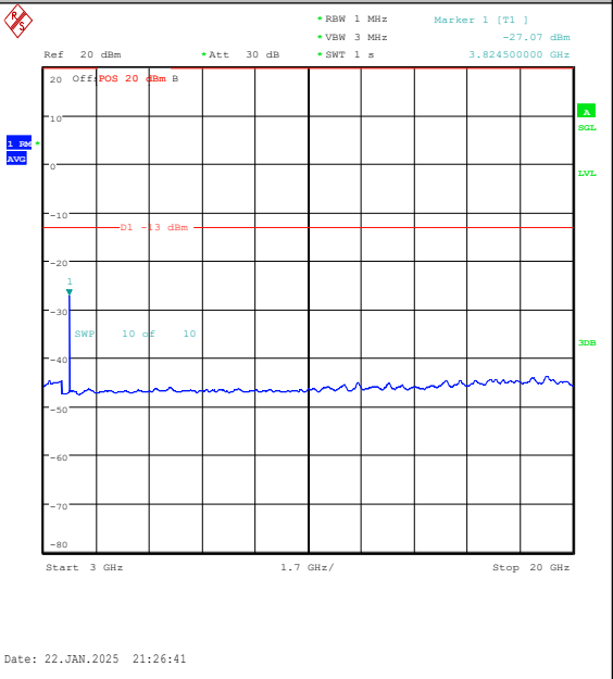
Band25-1.4MHz-16QAM-26683-1RB#0-3000~20000-PASS
