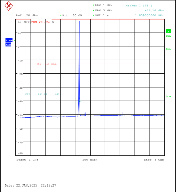
Band25-3MHz-QPSK-26055-15RB#0-1000~3000- PASS
