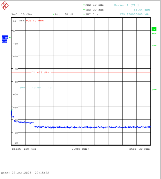
Band25-3MHz-QPSK-26365-1RB#0-0.15~30-PAS
