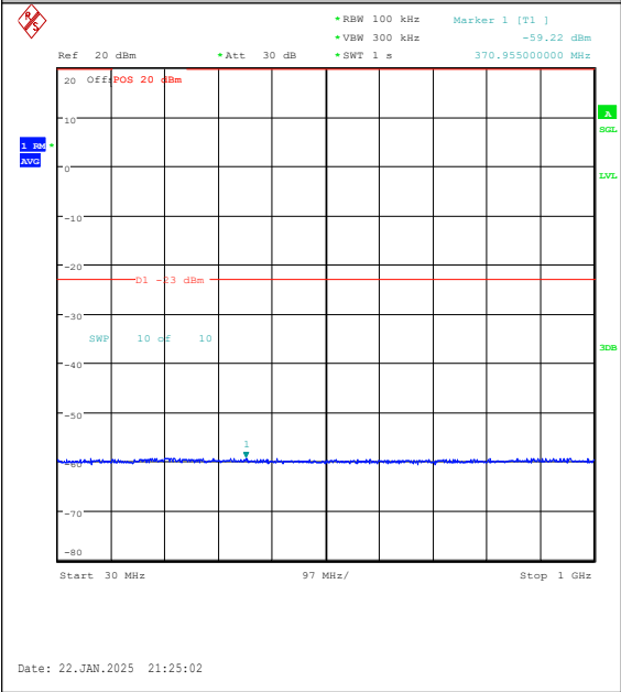
Band25-1.4MHz-QPSK-26683-1RB#0-30~1000-P ASS
