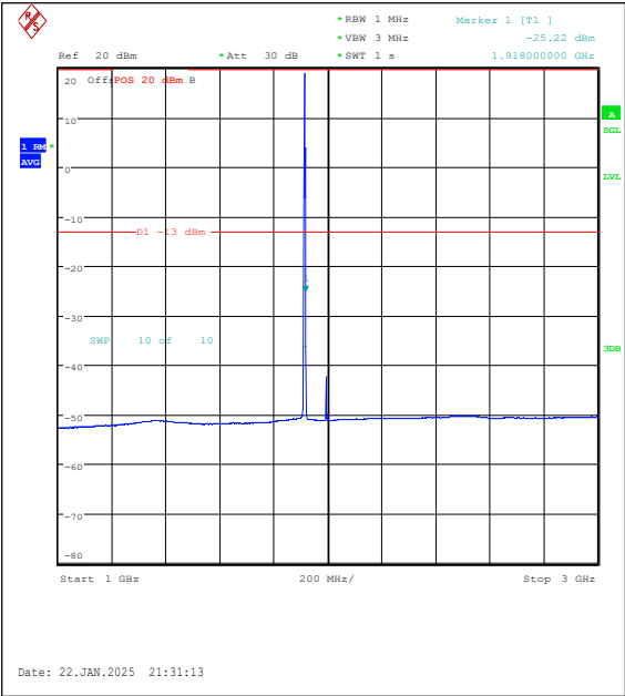
Band25-1.4MHz-16QAM-26683-6RB#0-1000~30 00-PASS
