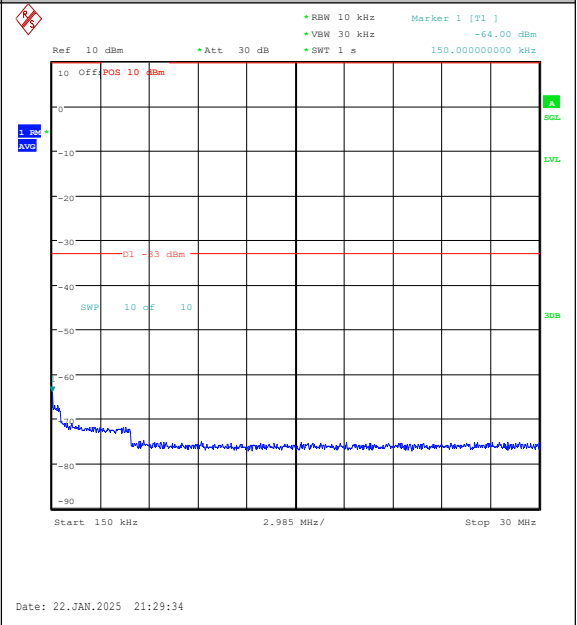
Band25-1.4MHz-QPSK-26683-6RB#0-0.15~30-PA SS
