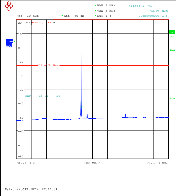
Band25-3MHz-QPSK-26055-1RB#14-1000~3000 -PASS
