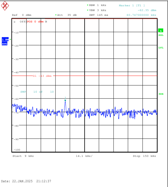
Band25-1.4MHz-QPSK-26047-1RB#5-0.009~0.15- PASS
