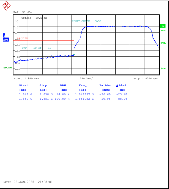
Band25-1.4MHz-16QAM-26047-6RB#0-PASS
