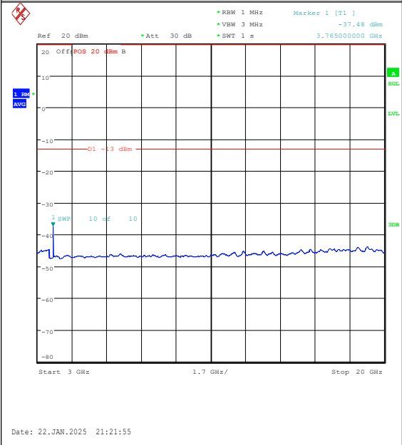
Band25-1.4MHz-16QAM-26365-1RB#5-3000~20 000-PASS
