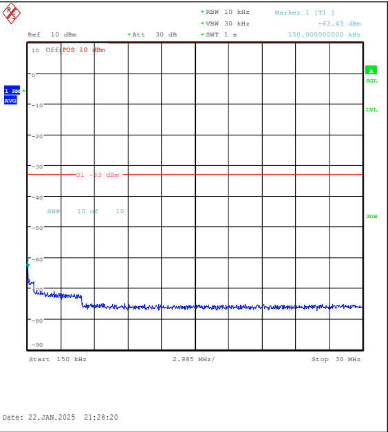
Band25-1.4MHz-16QAM-26683-1RB#5-0.15~30-P ASS
