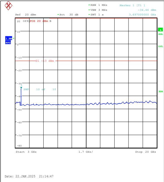
Band25-1.4MHz-16QAM-26047-1RB#5-3000~20000-PASS
