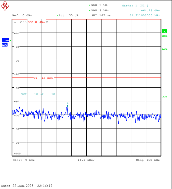
Band25-3MHz-16QAM-26365-1RB#0-0.009~0.15- PASS
