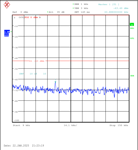
Band25-1.4MHz-16QAM-26365-6RB#0-0.009~0.1 5-PASS
