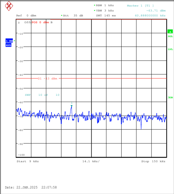
Band25-3MHz-QPSK-26055-1RB#0-0.009~0.15- PASS
