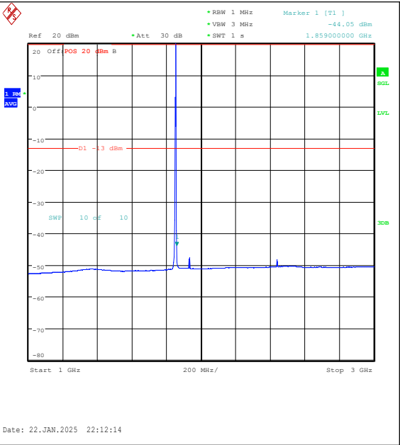
Band25-3MHz-16QAM-26055-1RB#14-1000~3000-PASS
