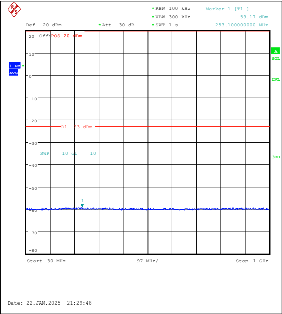
Band25-1.4MHz-QPSK-26683-6RB#0-30~1000-P ASS
