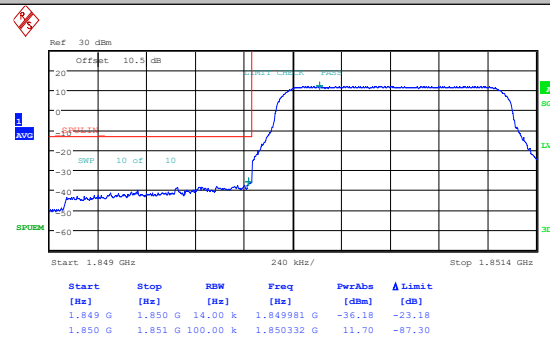
Band25-1.4MHz-QPSK-26047-1RB#0-PASS
