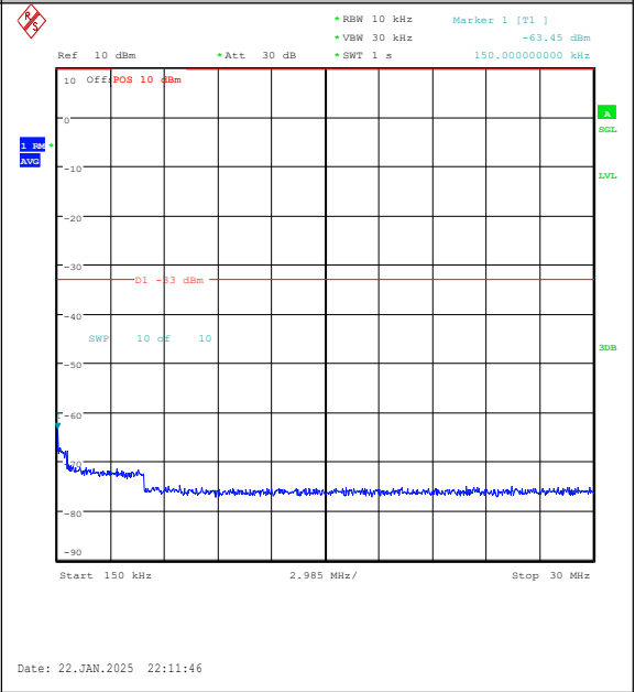
Band25-3MHz-16QAM-26055-1RB#14-0.15~30-P ASS
