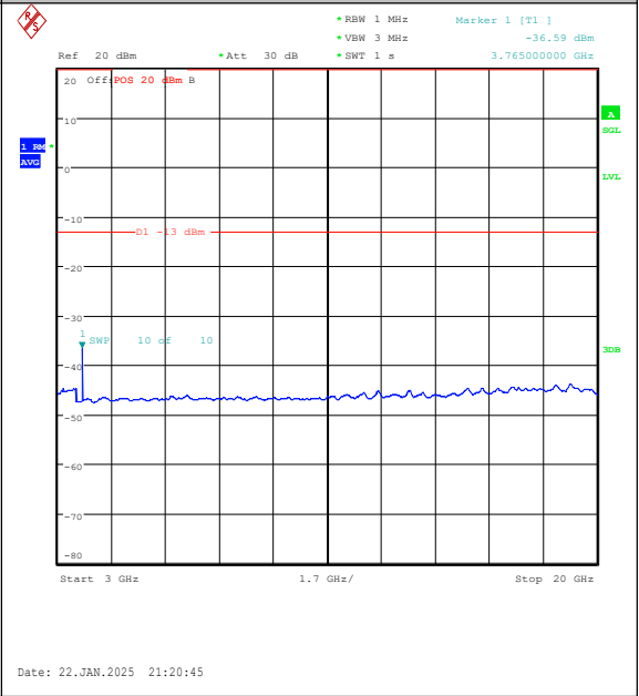
Band25-1.4MHz-QPSK-26365-1RB#5-3000~2000 0-PASS
