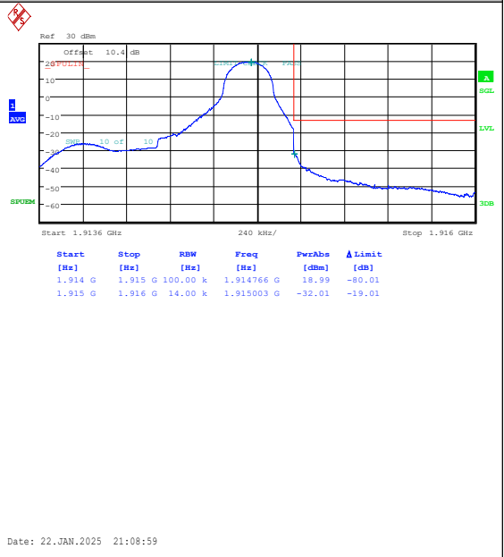
Band25-1.4MHz-QPSK-26683-1RB#5-PASS
