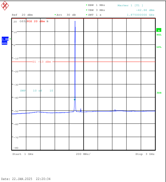
Band25-3MHz-QPSK-26365-15RB#0-1000~3000- PASS
