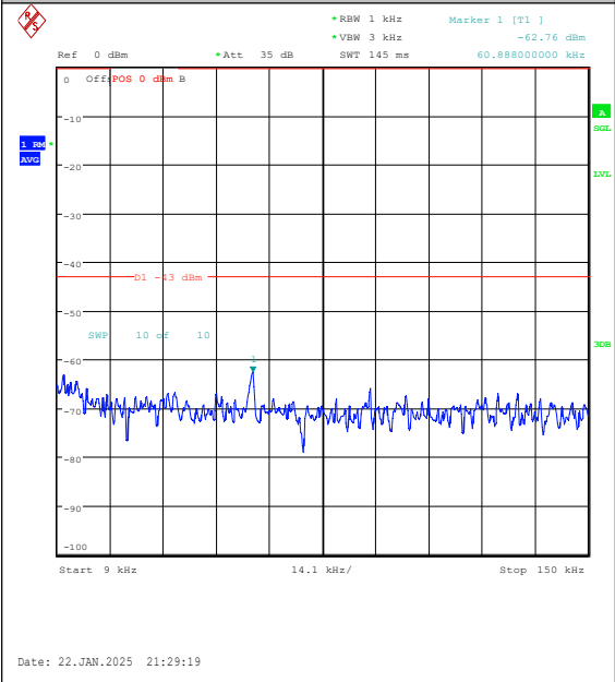
Band25-1.4MHz-QPSK-26683-6RB#0-0.009~0.15 -PASS
