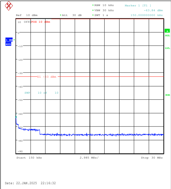
Band25-3MHz-16QAM-26365-1RB#0-0.15~30-PA SS
