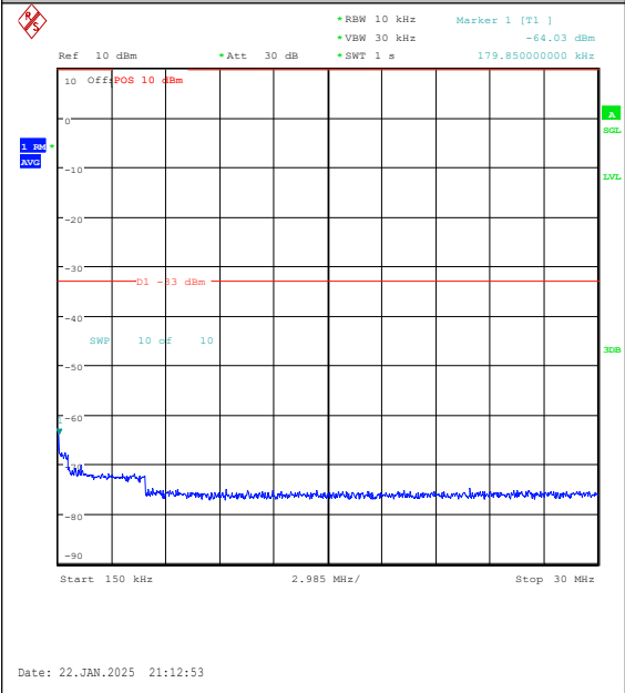
Band25-1.4MHz-QPSK-26047-1RB#5-0.15~30-P ASS
