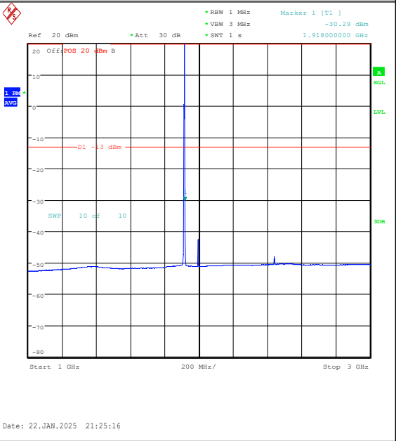
Band25-1.4MHz-QPSK-26683-1RB#0-1000~3000- PASS
