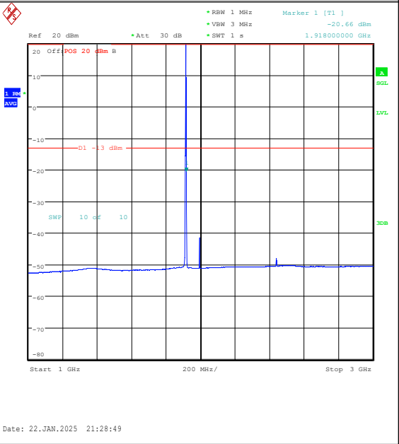
Band25-1.4MHz-16QAM-26683-1RB#5-1000~300 0-PASS
