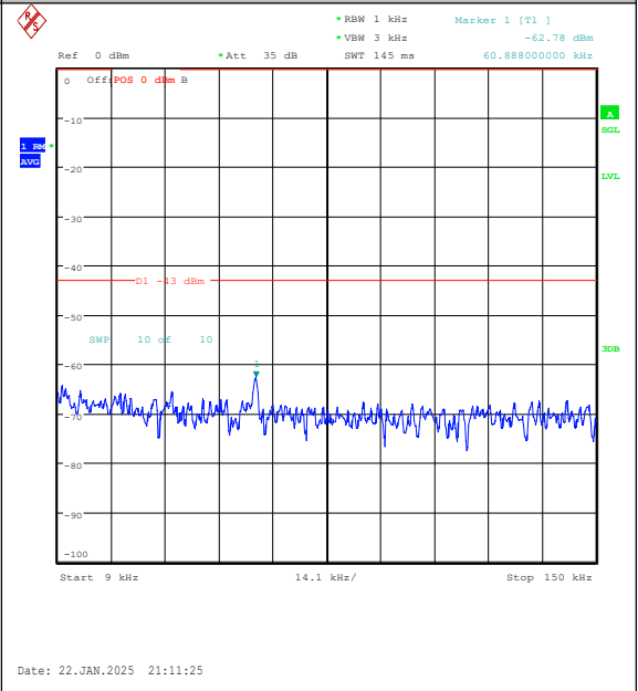
Band25-1.4MHz-16QAM-26047-1RB#0-0.009~0.1 5-PASS
