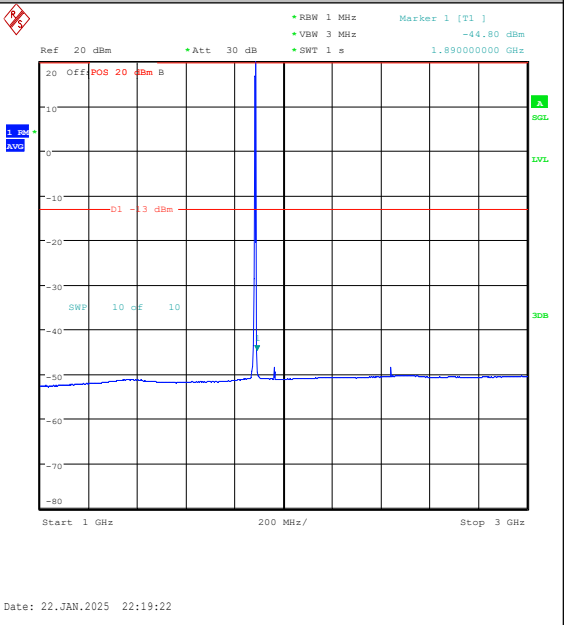
Band25-3MHz-16QAM-26365-1RB#14-1000~3000 -PASS
