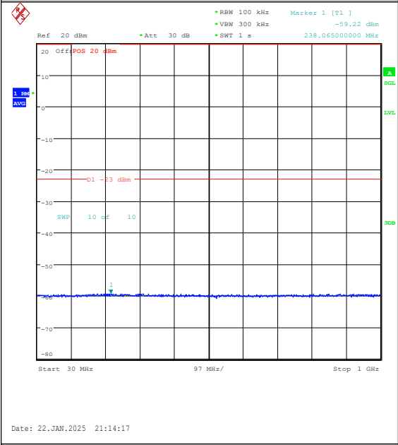
Band25-1.4MHz-16QAM-26047-1RB#5-30~1000- PASS
