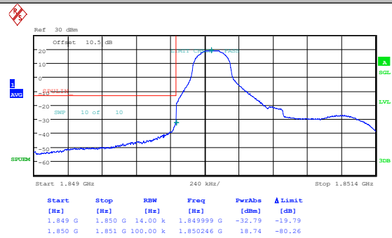
Band25-1.4MHz-QPSK-26047-1RB#5-PASS
