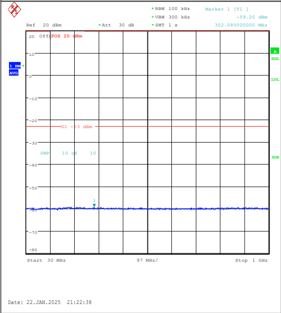
Band25-1.4MHz-QPSK-26365-6RB#0-30~1000-P ASS
