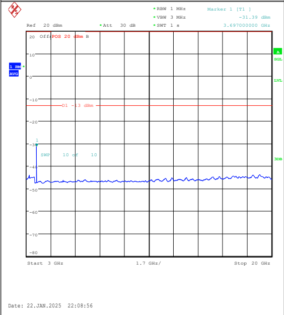
Band25-3MHz-QPSK-26055-1RB#0-3000~20000 -PASS
