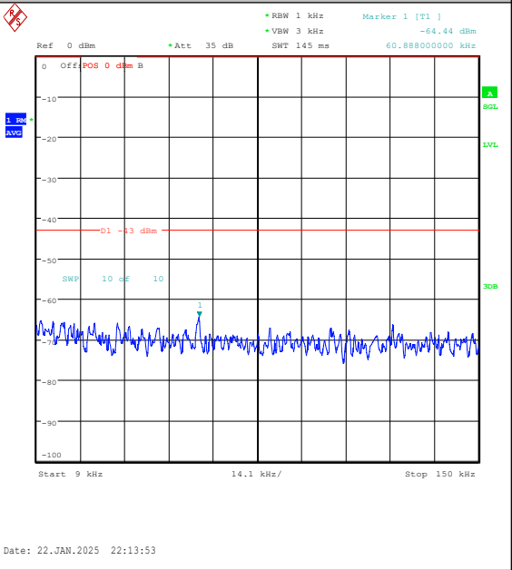
Band25-3MHz-16QAM-26055-15RB#0-0.009~0.15-PASS
