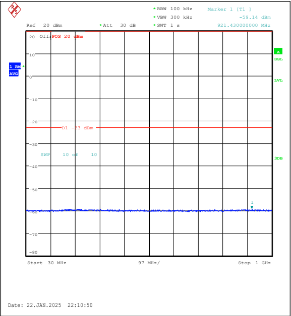
Band25-3MHz-QPSK-26055-1RB#14-30~1000-PA SS
