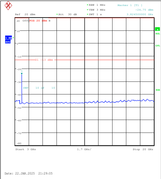
Band25-1.4MHz-16QAM-26683-1RB#5-3000~20000-PASS
