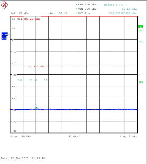
Band25-1.4MHz-16QAM-26365-6RB#0-30~1000-P ASS
