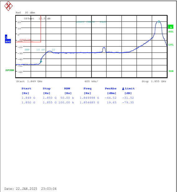
Band25-5MHz-QPSK-26065-1RB#24-PASS
