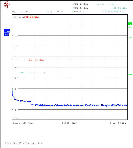
Band25-3MHz-16QAM-26055-15RB#0-0.15~30-P ASS
