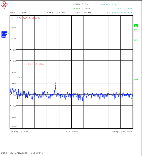
Band25-1.4MHz-QPSK-26365-1RB#5-0.009~0.15- PASS
