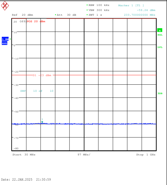
Band25-1.4MHz-16QAM-26683-6RB#0-30~1000-PASS
