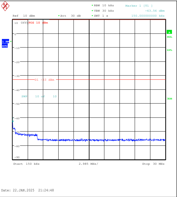
Band25-1.4MHz-QPSK-26683-1RB#0-0.15~30-PA SS
