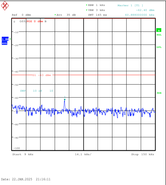
Band25-1.4MHz-16QAM-26047-6RB#0-0.009~0.15-PASS
