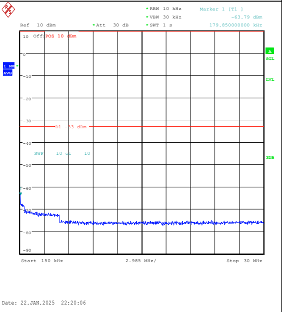
Band25-3MHz-QPSK-26365-15RB#0-0.15~30-PA SS
