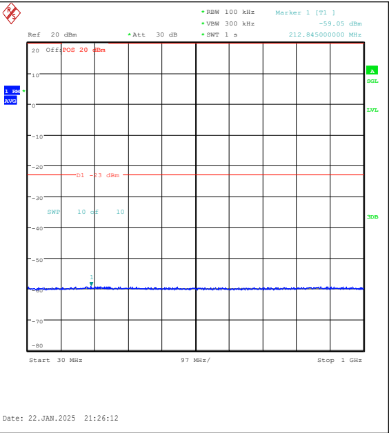
Band25-1.4MHz-16QAM-26683-1RB#0-30~1000-P ASS
