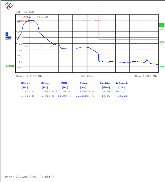
Band25-1.4MHz-QPSK-26683-1RB#0-PASS
