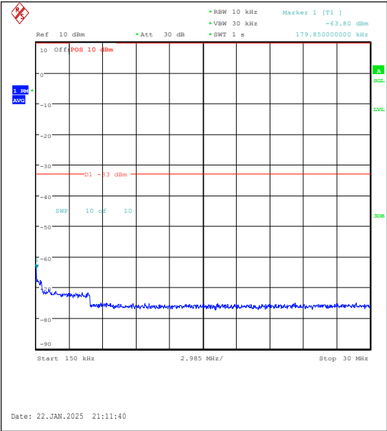
Band25-1.4MHz-16QAM-26047-1RB#0-0.15~30-PASS
