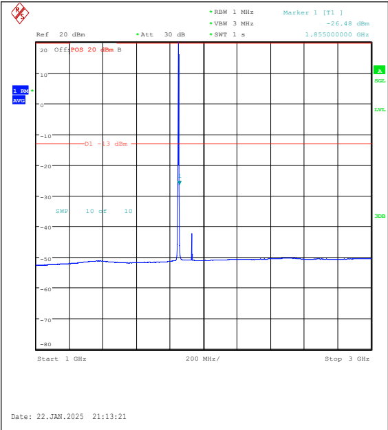
Band25-1.4MHz-QPSK-26047-1RB#5-1000~3000 -PASS
