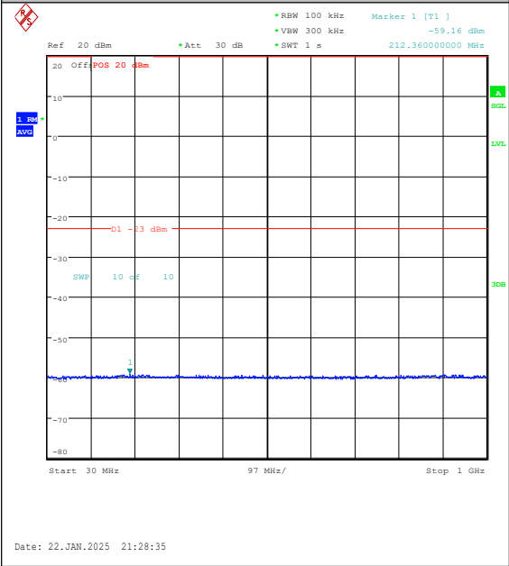
Band25-1.4MHz-16QAM-26683-1RB#5-30~1000- PASS
