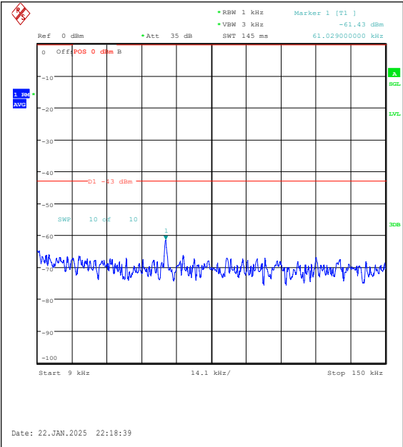
Band25-3MHz-16QAM-26365-1RB#14-0.009~0.1 5-PASS
