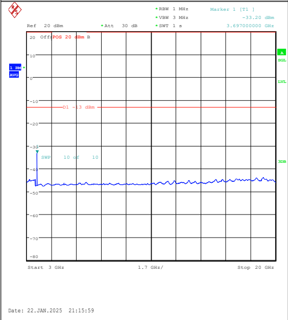
Band25-1.4MHz-QPSK-26047-6RB#0-3000~2000 0-PASS
