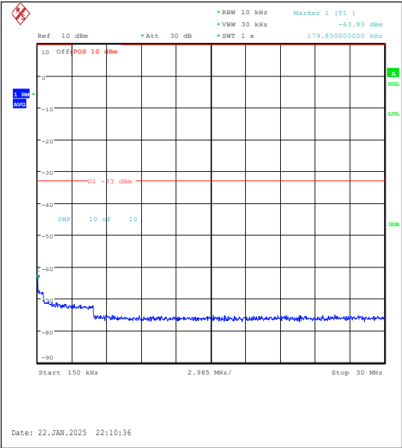
Band25-3MHz-QPSK-26055-1RB#14-0.15~30-PA SS
