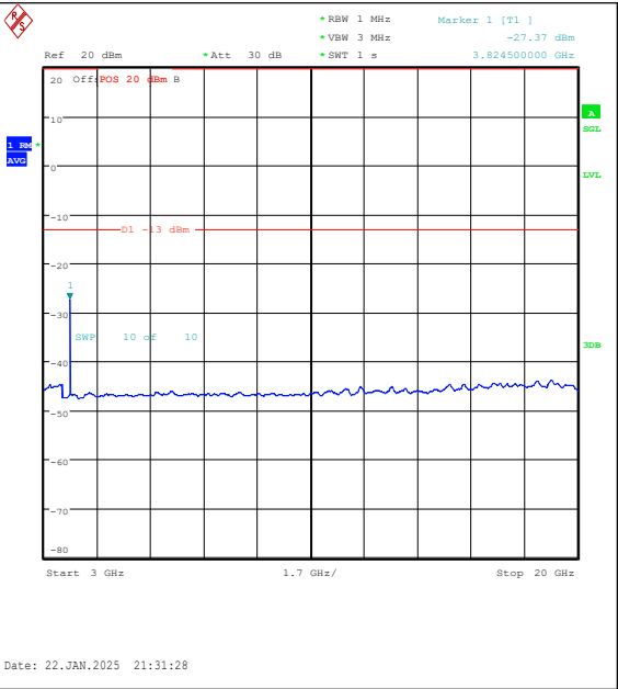
Band25-1.4MHz-16QAM-26683-6RB#0-3000~200 00-PASS
