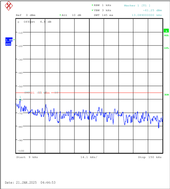
Band7-20MHz-16QAM-20850-1RB#99-0.009~0.1 5-PASS
