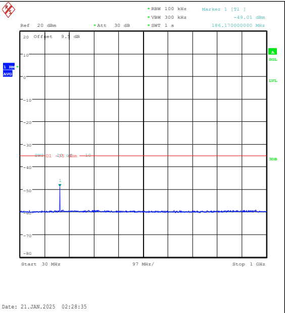
Band7-10MHz-16QAM-20800-1RB#0-30~1000-PA SS
