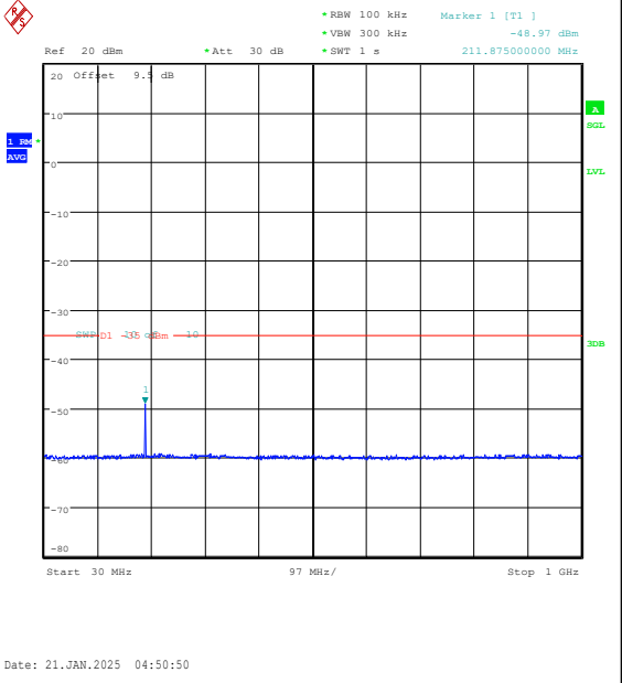
Band7-20MHz-16QAM-21100-1RB#0-30~1000-PA SS
