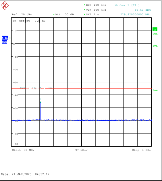
Band7-20MHz-QPSK-21100-1RB#99-30~1000-PA SS
