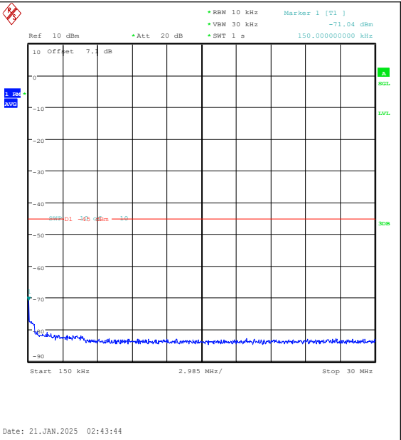
Band7-10MHz-QPSK-21400-1RB#0-0.15~30-PAS
