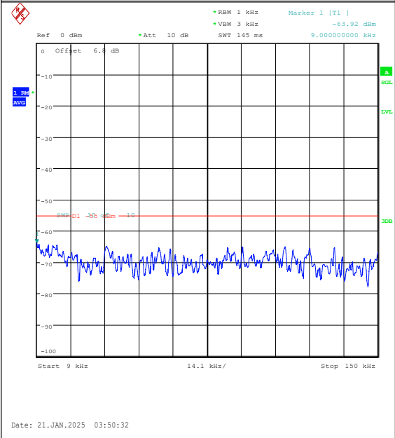
Band7-15MHz-QPSK-21375-1RB#0-0.009~0.15- PASS
