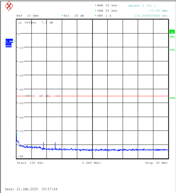
Band7-15MHz-16QAM-21375-75RB#0-0.15~30-P ASS
