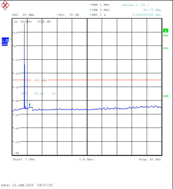
Band7-20MHz-QPSK-21350-1RB#0-1000~20000-PASS
