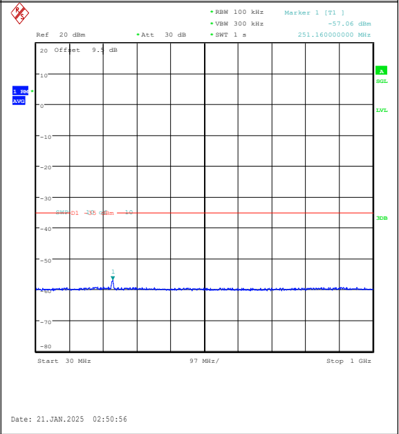
Band7-10MHz-16QAM-21400-50RB#0-30~1000-PASS
