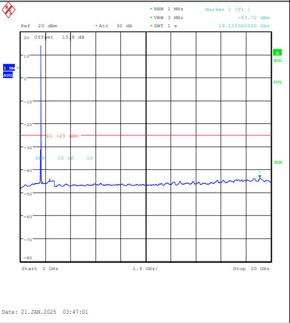
Band7-15MHz-16QAM-21100-1RB#74-1000~2000 0-PASS
