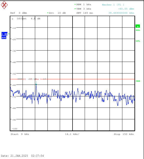
Band7-10MHz-QPSK-21100-1RB#49-0.009~0.15- PASS
