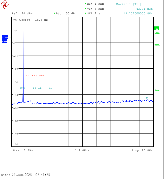
Band7-10MHz-QPSK-21100-50RB#0-1000~20000-PASS
