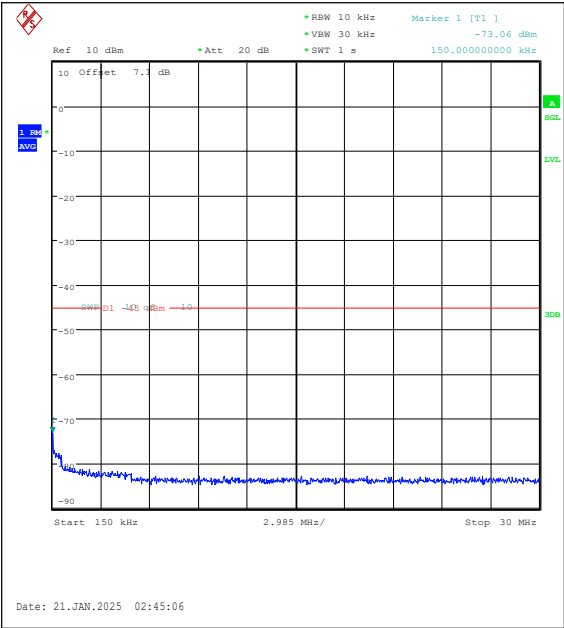
Band7-10MHz-16QAM-21400-1RB#0-0.15~30-PA SS
