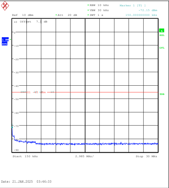
Band7-15MHz-16QAM-21100-1RB#74-0.15~30-PA SS
