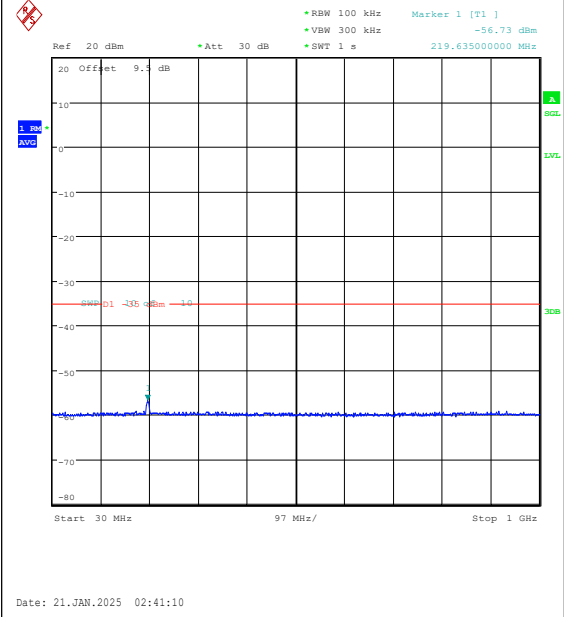
Band7-10MHz-QPSK-21100-50RB#0-30~1000-PASS
