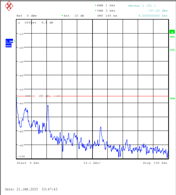
Band7-15MHz-QPSK-21100-75RB#0-0.009~0.15-PASS PASS
