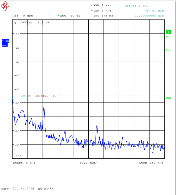
Band7-20MHz-16QAM-21350-100RB#0-0.009~0.15-PASS
