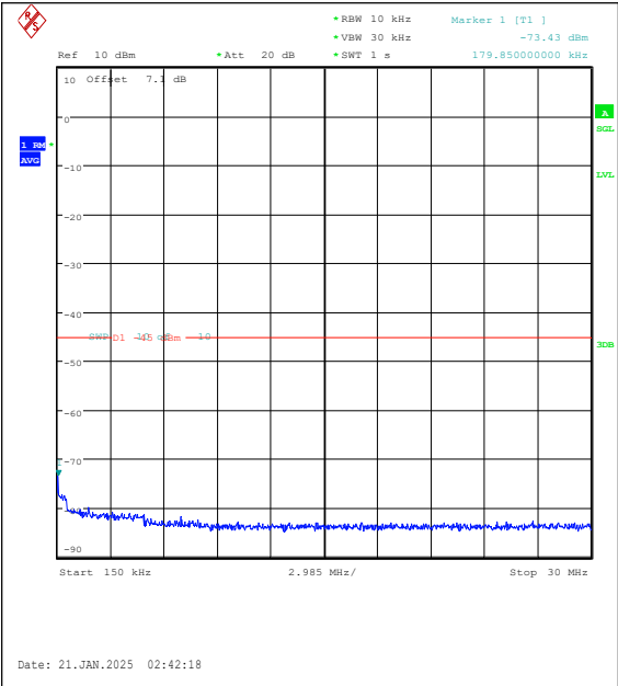
Band7-10MHz-16QAM-21100-50RB#0-0.15~30-P ASS
