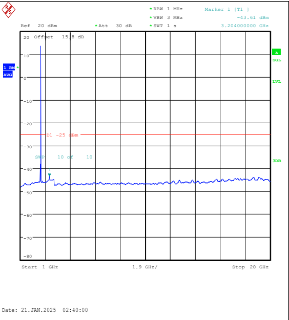
Band7-10MHz-16QAM-21100-1RB#49-1000~2000-0-PASS
