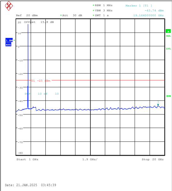
Band7-15MHz-QPSK-21100-1RB#74-1000~2000 0-PASS
