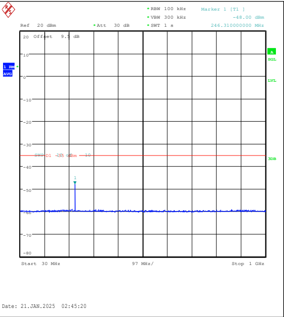
Band7-10MHz-16QAM-21400-1RB#0-30~1000-PA SS
