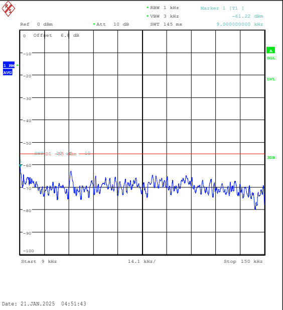
Band7-20MHz-QPSK-21100-1RB#99-0.009~0.15- PASS
