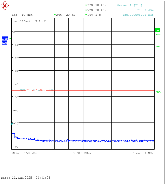
Band7-20MHz-QPSK-20850-1RB#0-0.15~30-PAS
