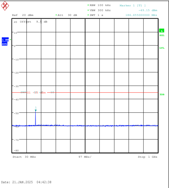
Band7-20MHz-16QAM-20850-1RB#0-30~1000-PA SS
