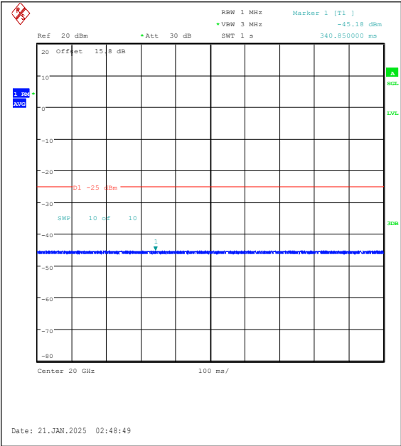
Band7-10MHz-16QAM-21400-1RB#49-20000~27000-PASS
