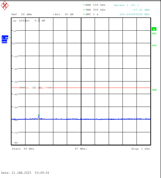
Band7-15MHz-16QAM-21100-75RB#0-30~1000-PASS
