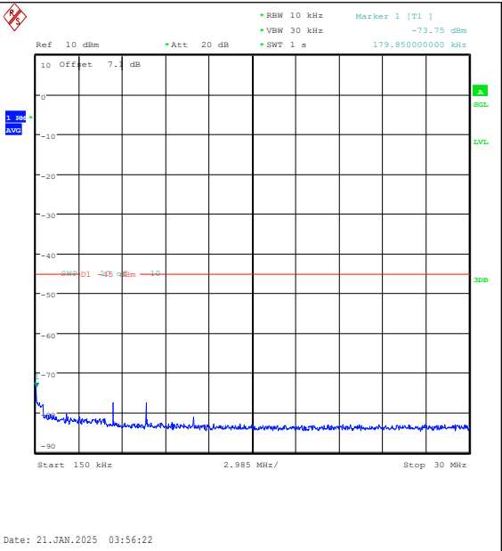
Band7-15MHz-QPSK-21375-75RB#0-0.15~30-PA SS
