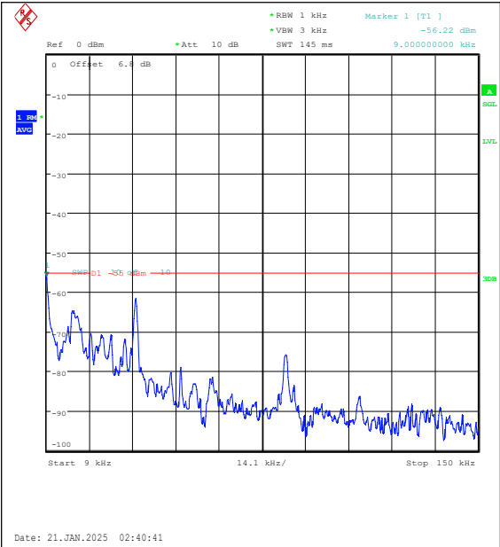
Band7-10MHz-QPSK-21100-50RB#0-0.009~0.15-PASS
