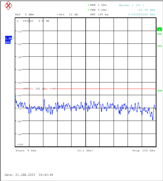
Band7-20MHz-QPSK-20850-1RB#0-0.009~0.15-PASS
