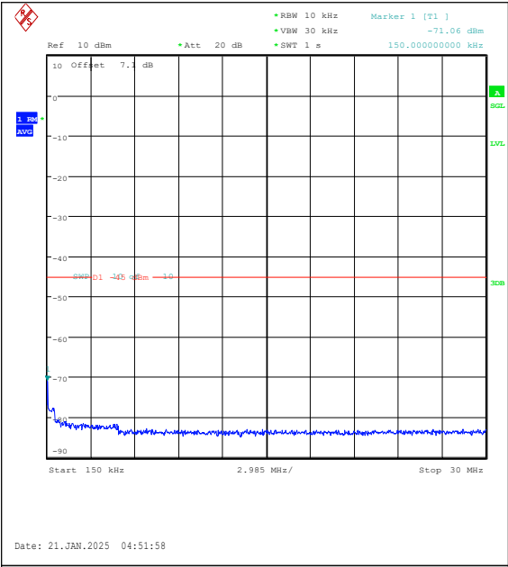
Band7-20MHz-QPSK-21100-1RB#99-0.15~30-PA SS
