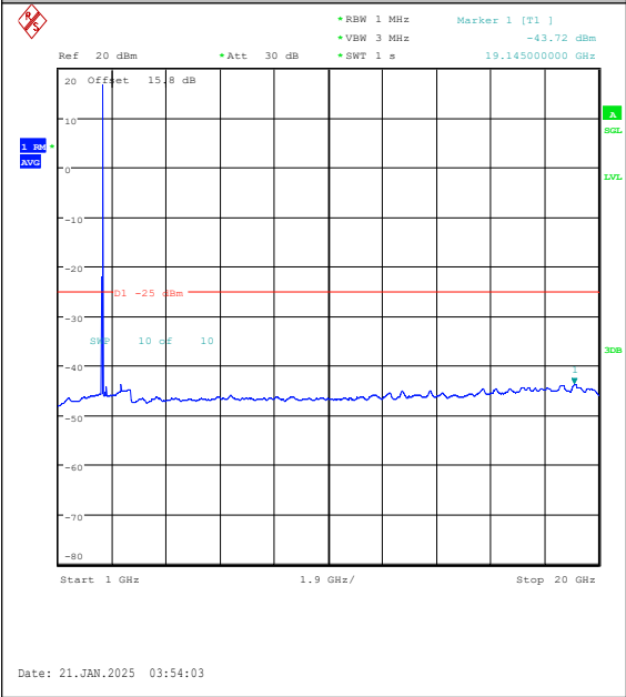
Band7-15MHz-QPSK-21375-1RB#74-1000~2000 0-PASS
