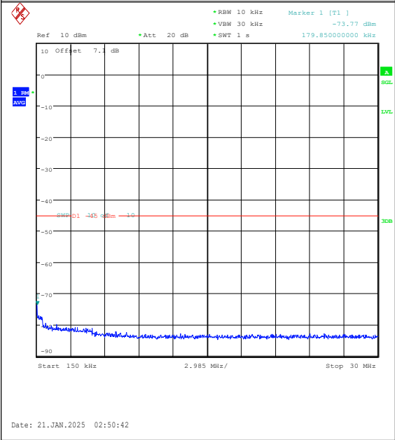
Band7-10MHz-16QAM-21400-50RB#0-0.15~30-PASS
