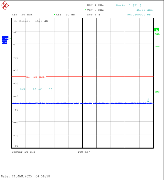
Band7-20MHz-16QAM-21100-100RB#0-20000~27000-PASS
