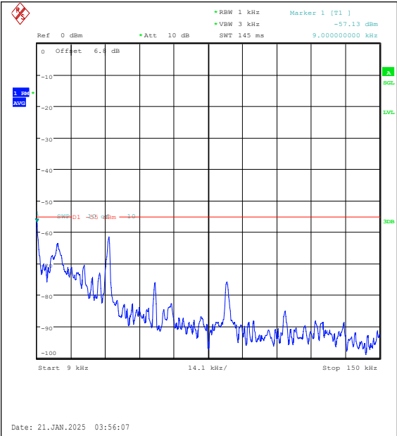
Band7-15MHz-QPSK-21375-75RB#0-0.009~0.15 -PASS
