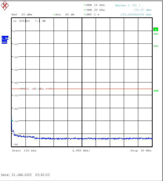
Band7-15MHz-QPSK-21100-1RB#0-0.15~30-PAS S
