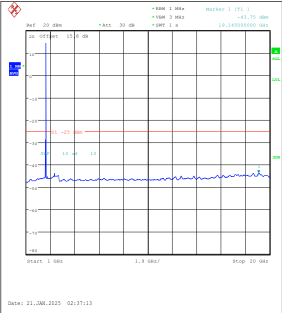
Band7-10MHz-16QAM-21100-1RB#0-1000~2000 0-PASS
