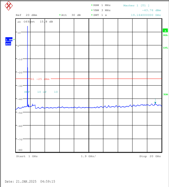
Band7-20MHz-16QAM-21350-1RB#0-1000~2000 0-PASS
