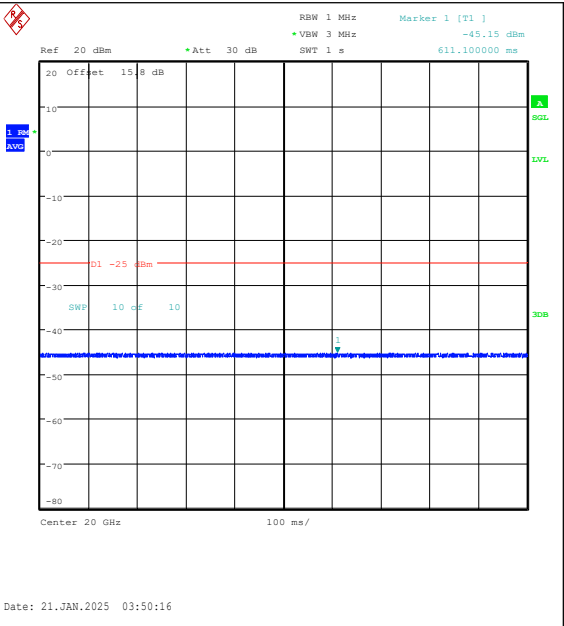
Band7-15MHz-16QAM-21100-75RB#0-20000~270 00-PASS
