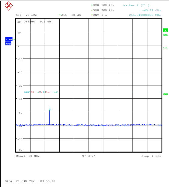
Band7-15MHz-16QAM-21375-1RB#74-30~1000-PASS
