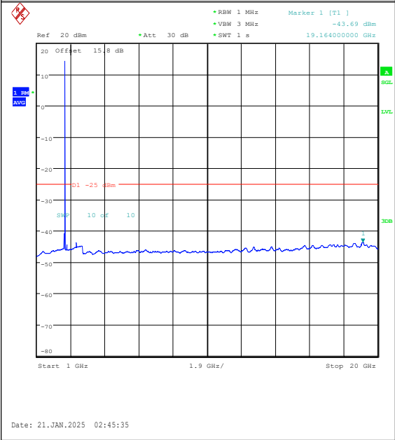
Band7-10MHz-16QAM-21400-1RB#0-1000~2000 0-PASS
