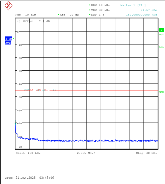
Band7-15MHz-16QAM-21100-1RB#0-0.15~30-PA SS
