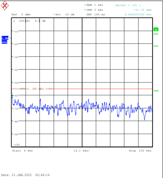
Band7-10MHz-QPSK-21400-1RB#49-0.009~0.15- PASS
