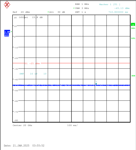
Band7-15MHz-16QAM-21375-1RB#74-20000~27000-PASS
