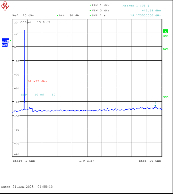
Band7-20MHz-QPSK-21100-100RB#0-1000~2000 0-PASS
