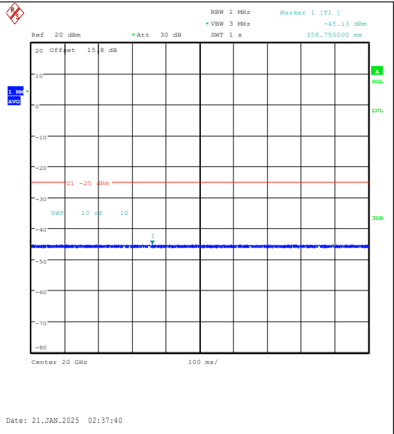
Band7-10MHz-16QAM-21100-1RB#0-20000~2700 0-PASS
