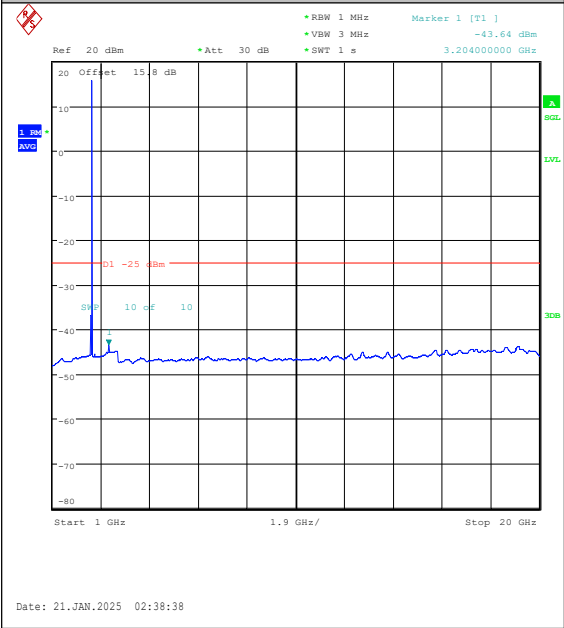
Band7-10MHz-QPSK-21100-1RB#49-1000~2000 0-PASS
