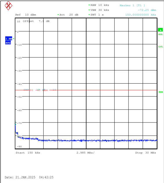
Band7-20MHz-16QAM-20850-1RB#0-0.15~30-PA SS
