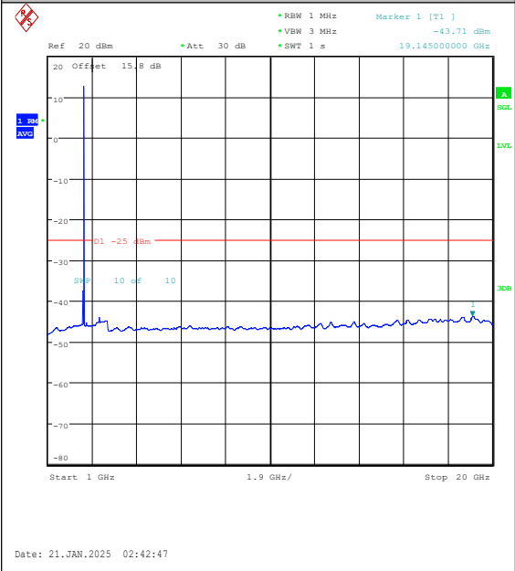
Band7-10MHz-16QAM-21100-50RB#0-1000~200 00-PASS
