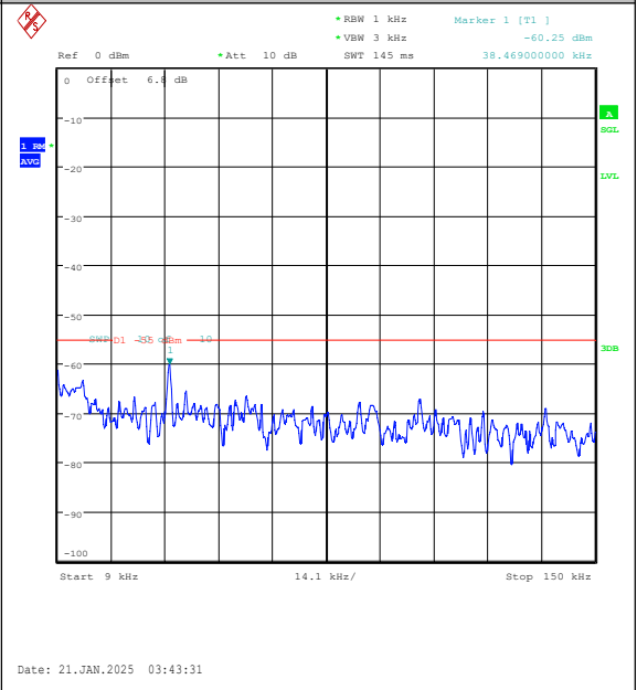
Band7-15MHz-16QAM-21100-1RB#0-0.009~0.15- PASS
