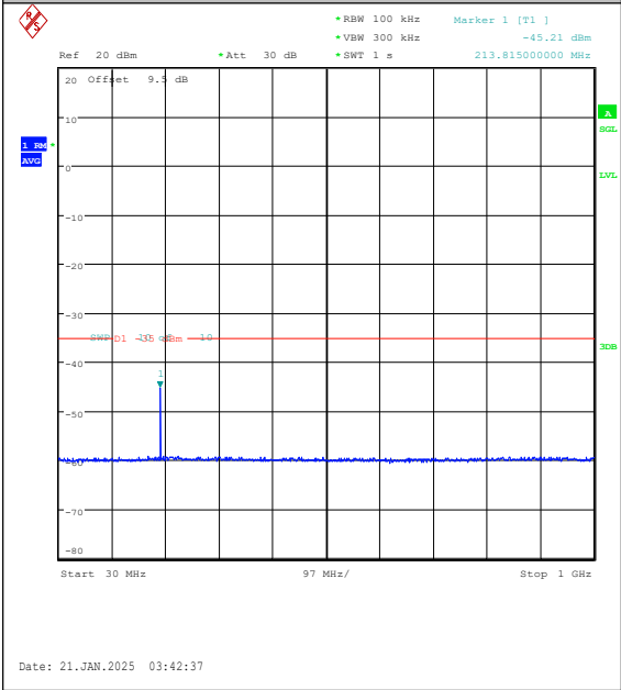
Band7-15MHz-QPSK-21100-1RB#0-30~1000-PA SS
