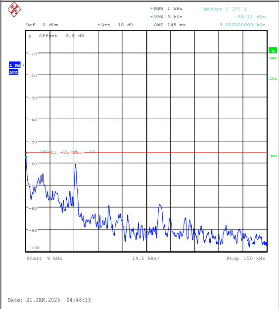
Band7-20MHz-QPSK-20850-100RB#0-0.009~0.1 5-PASS
