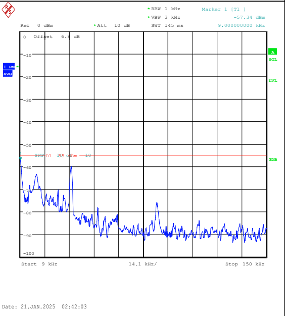
Band7-10MHz-16QAM-21100-50RB#0-0.009~0.15-PASS
