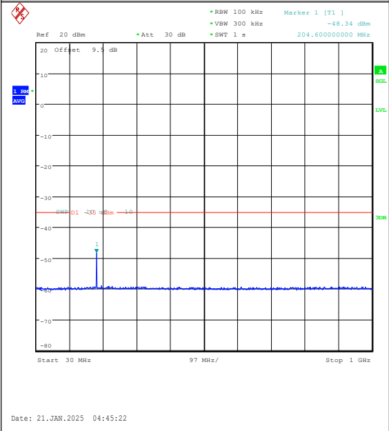
Band7-20MHz-16QAM-20850-1RB#99-30~1000- PASS
