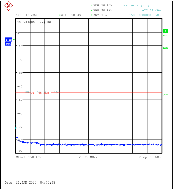
Band7-20MHz-16QAM-20850-1RB#99-0.15~30-P ASS
