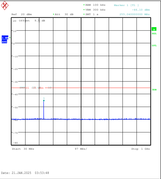
Band7-15MHz-QPSK-21375-1RB#74-30~1000-PA SS
