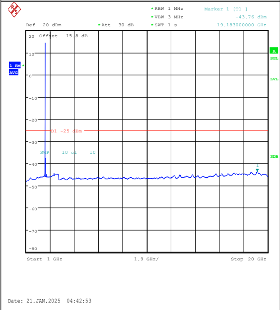
Band7-20MHz-16QAM-20850-1RB#0-1000~2000 0-PASS
