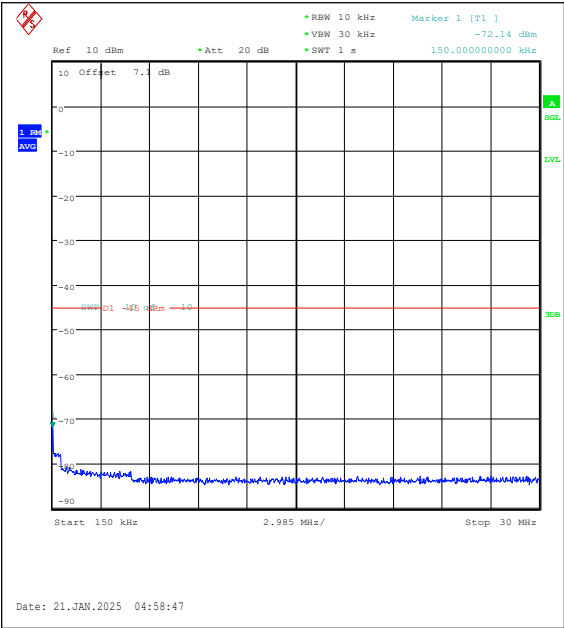
Band7-20MHz-16QAM-21350-1RB#0-0.15~30-PA SS
