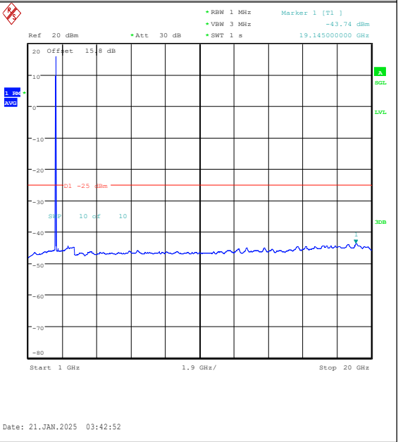
Band7-15MHz-QPSK-21100-1RB#0-1000~20000-PASS PASS
