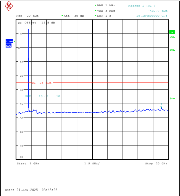
Band7-15MHz-QPSK-21100-75RB#0-1000~20000 -PASS
