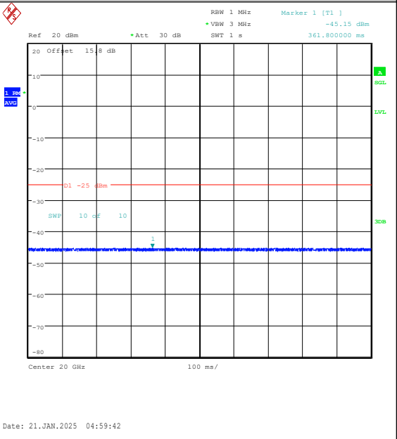
Band7-20MHz-16QAM-21350-1RB#0-20000~2700 0-PASS
