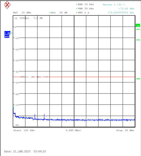
Band7-15MHz-16QAM-21100-75RB#0-0.15~30-PASS
