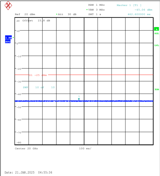
Band7-20MHz-QPSK-21100-100RB#0-20000~27000-PASS
