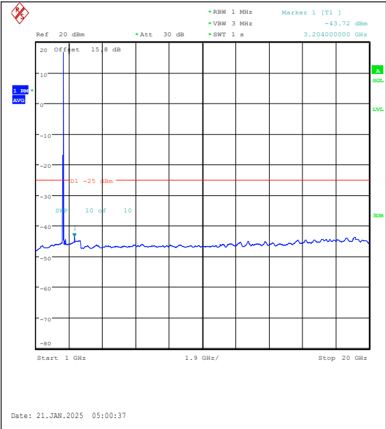
Band7-20MHz-QPSK-21350-1RB#99-1000~2000 0-PASS
