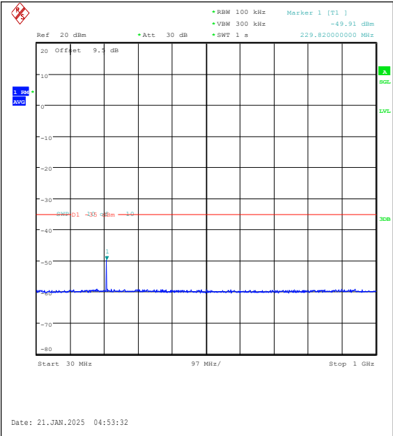
Band7-20MHz-16QAM-21100-1RB#99-30~1000-PASS
