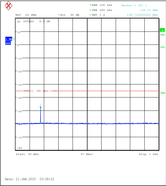
Band7-15MHz-16QAM-20825-1RB#74-30~1000-PASS
