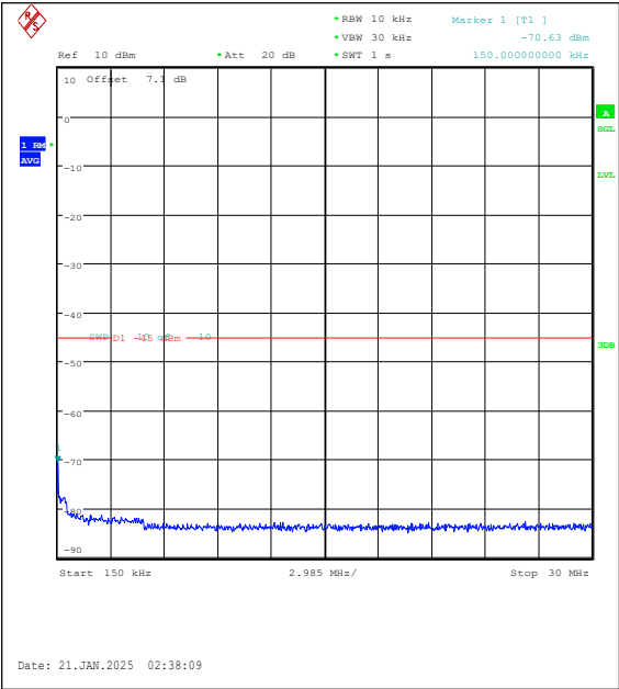
Band7-10MHz-QPSK-21100-1RB#49-0.15~30-PA SS
