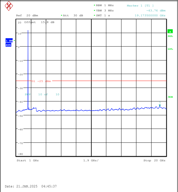
Band7-20MHz-16QAM-20850-1RB#99-1000~2000 0-PASS
