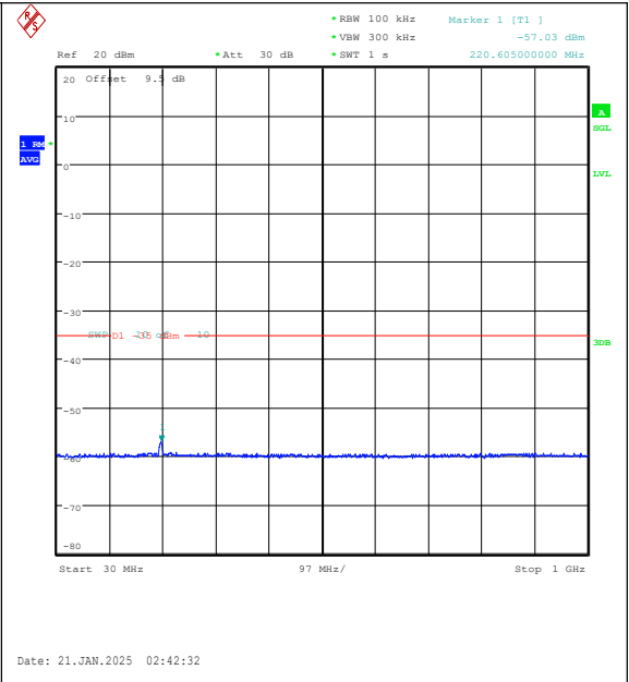
Band7-10MHz-16QAM-21100-50RB#0-30~1000-P ASS
