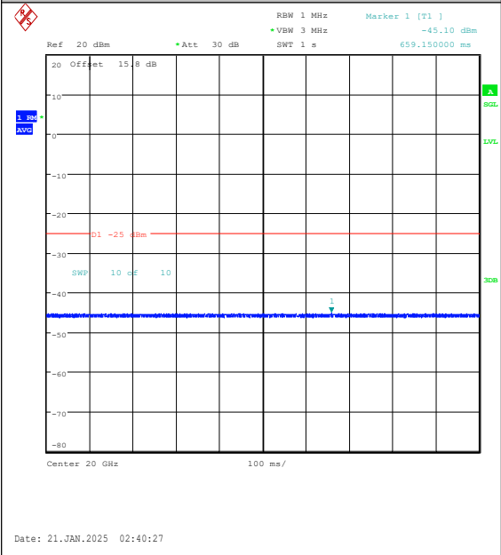
Band7-10MHz-16QAM-21100-1RB#49-20000~27000-PASS
