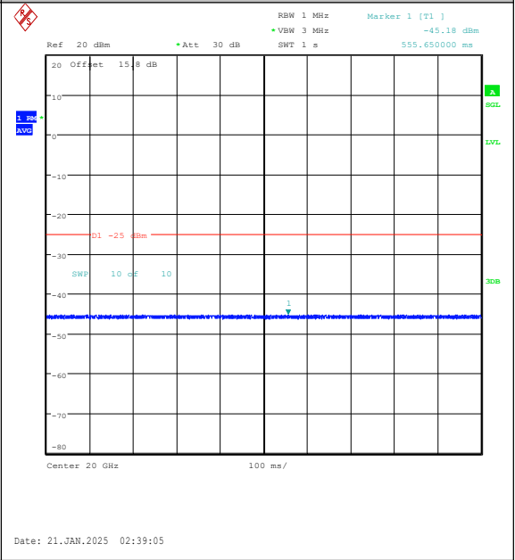
Band7-10MHz-QPSK-21100-1RB#49-20000~2700 0-PASS
