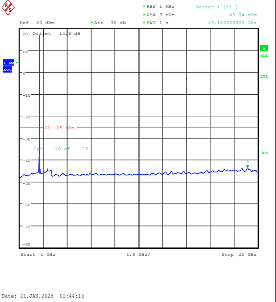
Band7-10MHz-QPSK-21400-1RB#0-1000~20000-PASS
