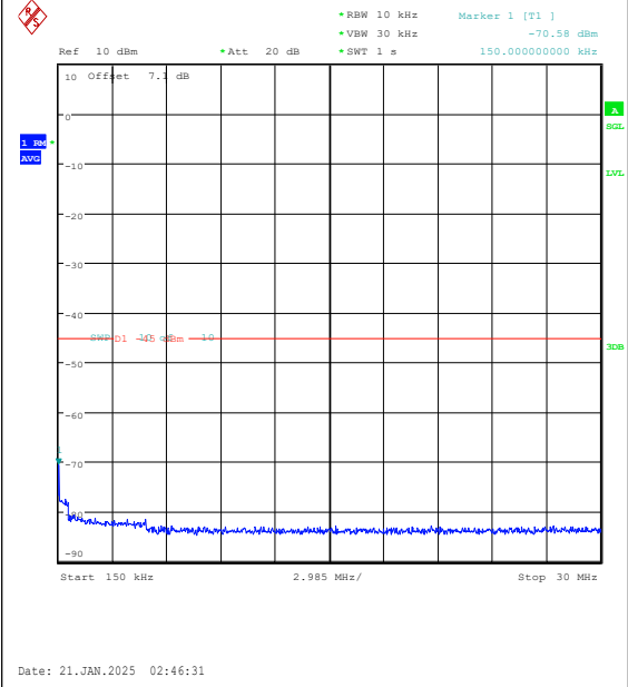
Band7-10MHz-QPSK-21400-1RB#49-0.15~30-PA SS
