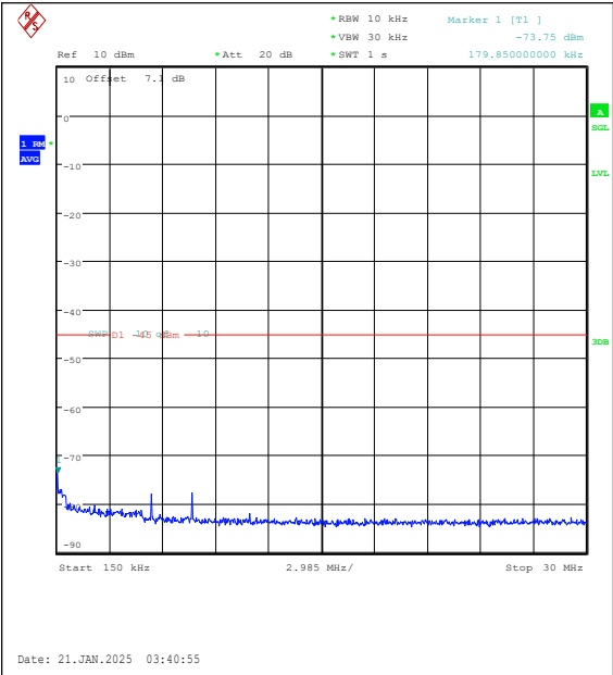
Band7-15MHz-16QAM-20825-75RB#0-0.15~30-P ASS
