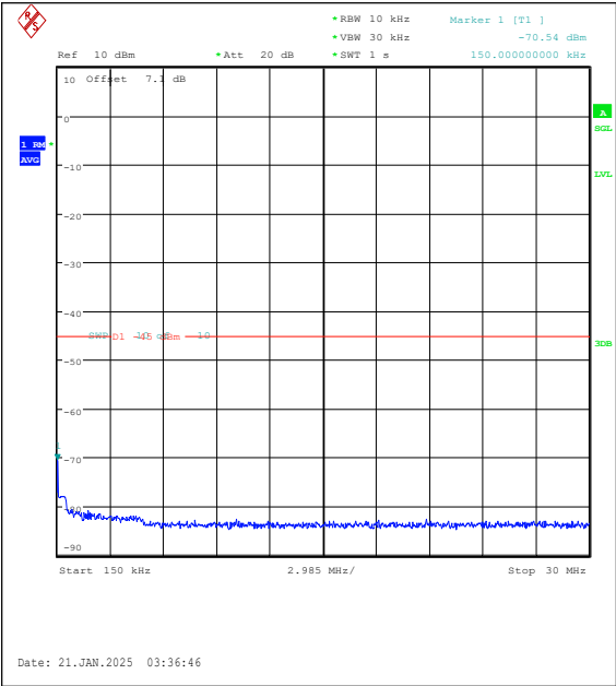
Band7-15MHz-QPSK-20825-1RB#74-0.15~30-PA SS
