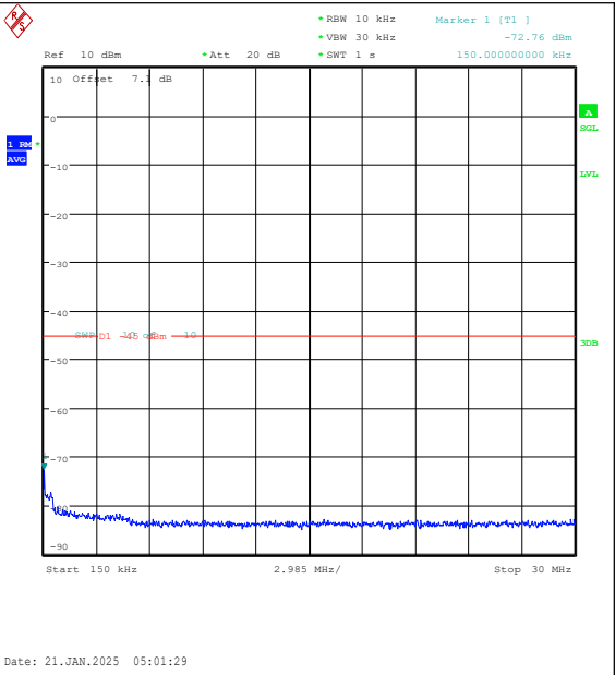
Band7-20MHz-16QAM-21350-1RB#99-0.15~30-P ASS
