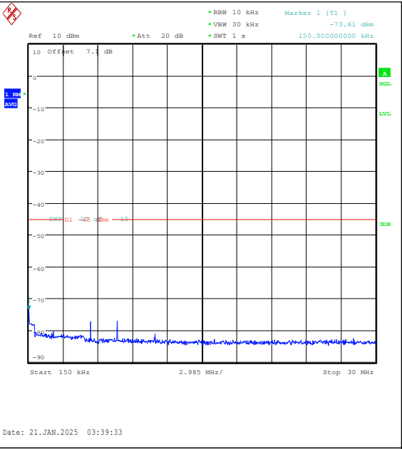
Band7-15MHz-QPSK-20825-75RB#0-0.15~30-PA SS
