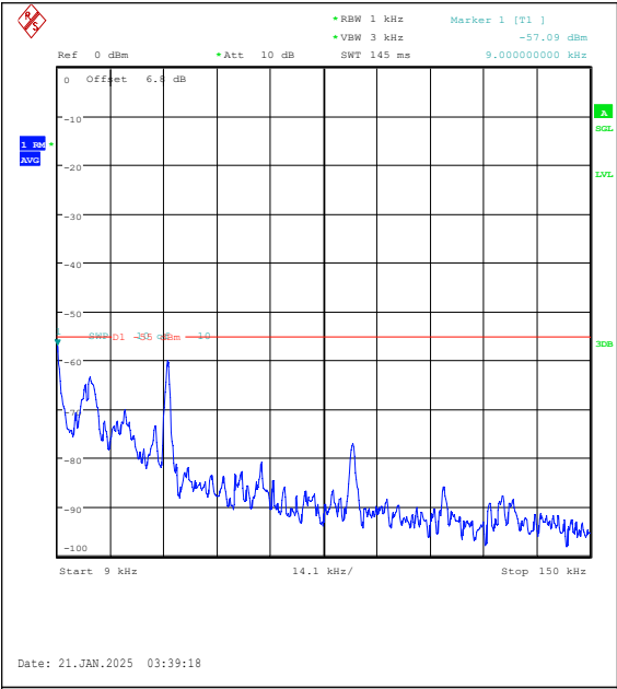
Band7-15MHz-QPSK-20825-75RB#0-0.009~0.15 -PASS
