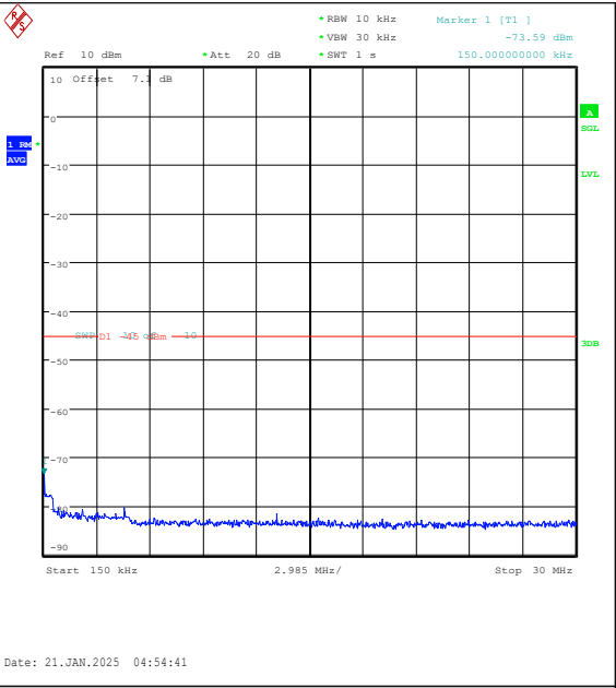
Band7-20MHz-QPSK-21100-100RB#0-0.15~30-PA SS
