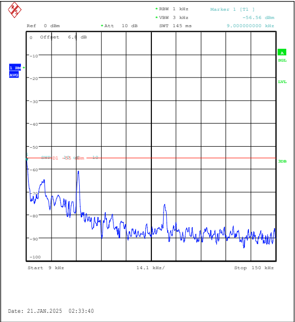
Band7-10MHz-16QAM-20800-50RB#0-0.009~0.15-PASS
