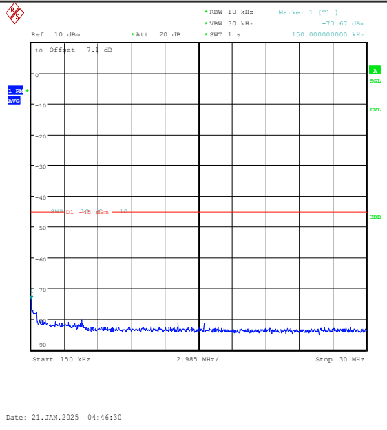
Band7-20MHz-QPSK-20850-100RB#0-0.15~30-PA SS
