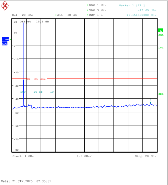
Band7-10MHz-QPSK-21100-1RB#0-1000~20000- PASS
