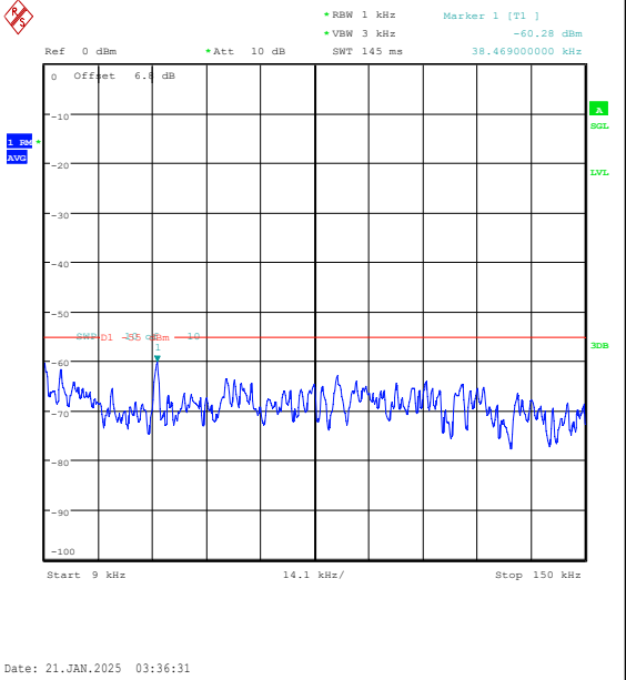
Band7-15MHz-QPSK-20825-1RB#74-0.009~0.15- PASS
