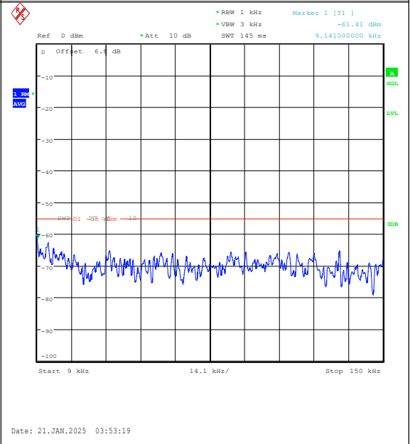
Band7-15MHz-QPSK-21375-1RB#74-0.009~0.15- PASS
