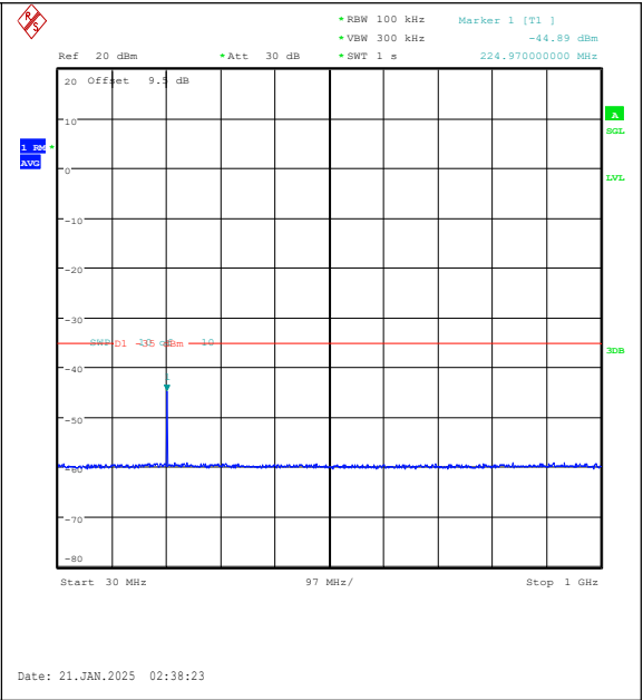
Band7-10MHz-QPSK-21100-1RB#49-30~1000-PA SS
