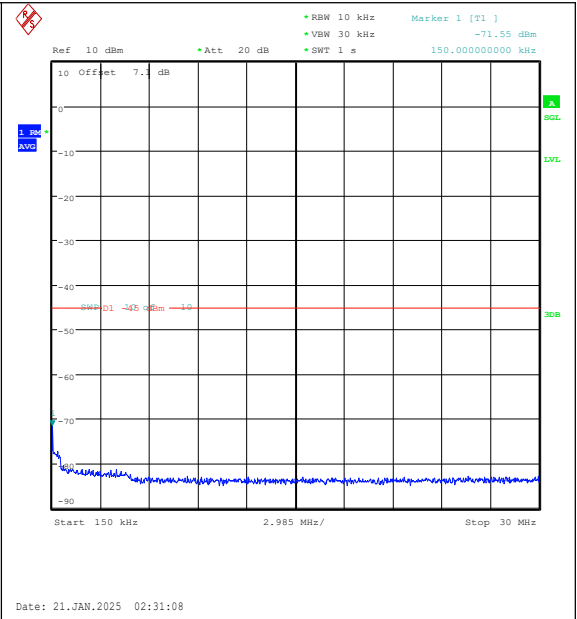
Band7-10MHz-16QAM-20800-1RB#49-0.15~30-P ASS
