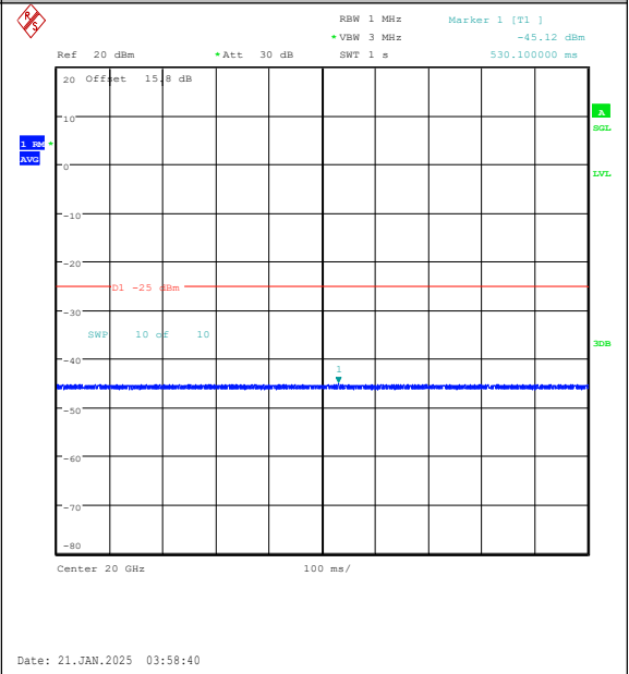
Band7-15MHz-16QAM-21375-75RB#0-20000~270 00-PASS
