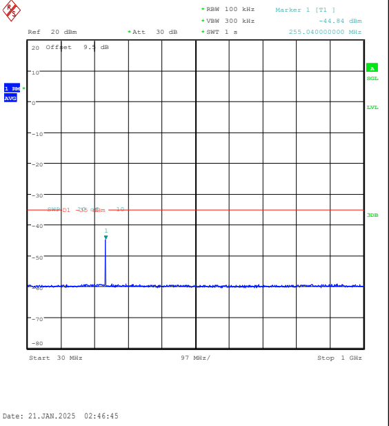
Band7-10MHz-QPSK-21400-1RB#49-30~1000-PA SS
