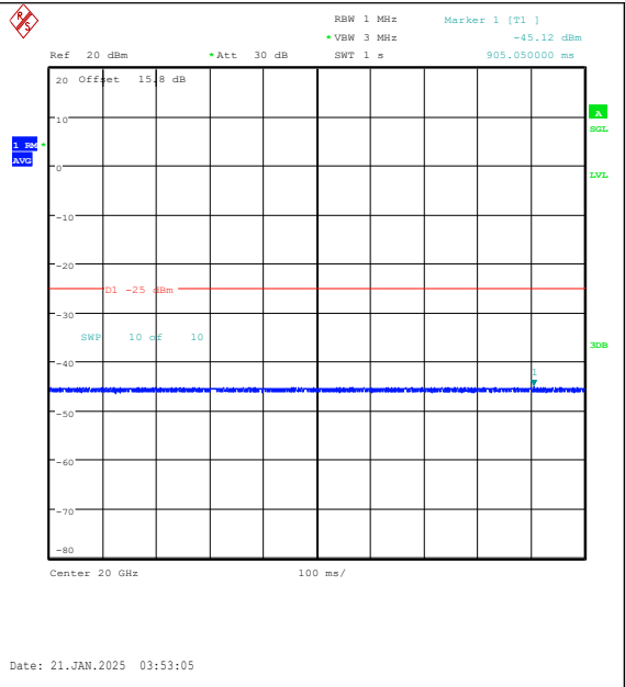
Band7-15MHz-16QAM-21375-1RB#0-20000~2700 0-PASS
