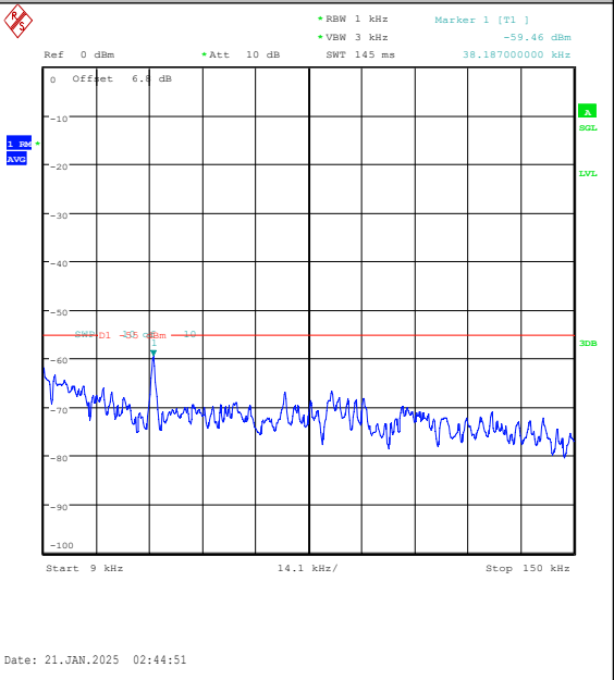
Band7-10MHz-16QAM-21400-1RB#0-0.009~0.15- PASS
