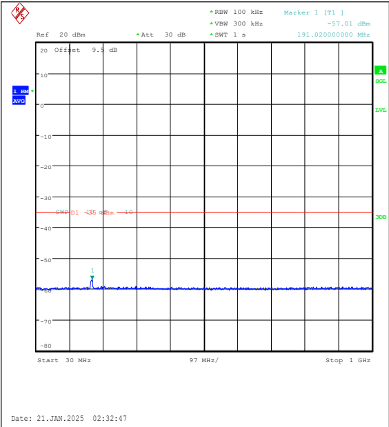
Band7-10MHz-QPSK-20800-50RB#0-30~1000-P ASS
