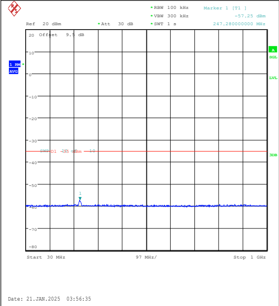
Band7-15MHz-QPSK-21375-75RB#0-30~1000-P ASS
