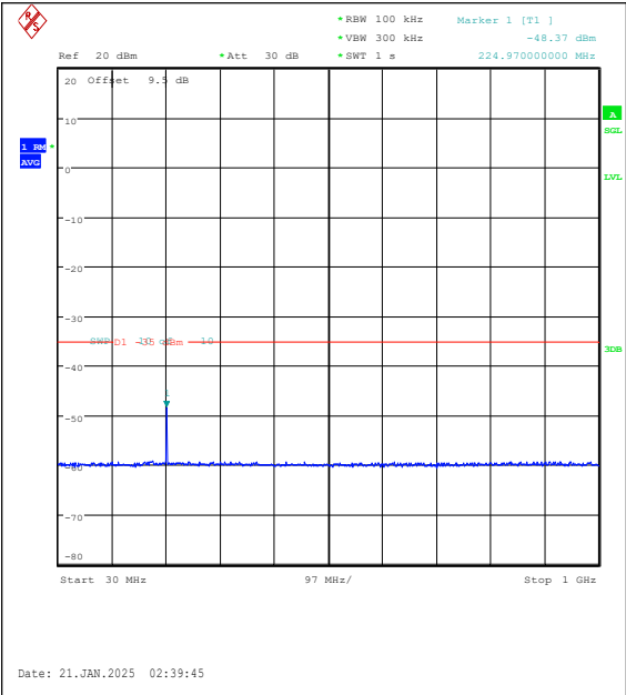
Band7-10MHz-16QAM-21100-1RB#49-30~1000-PASS
