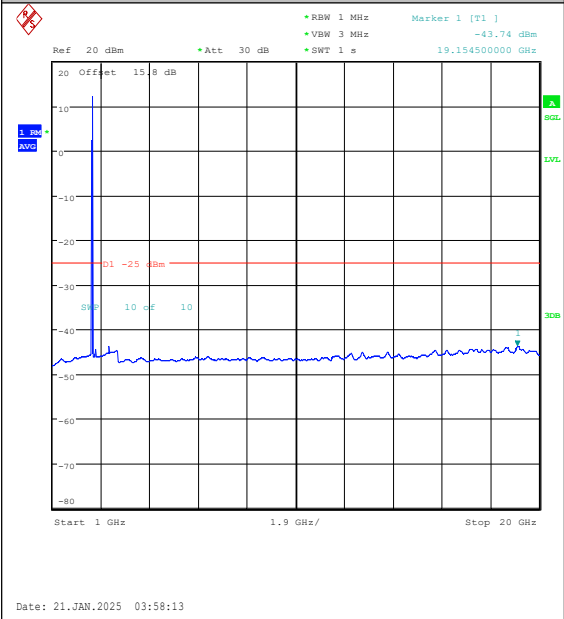
Band7-15MHz-16QAM-21375-75RB#0-1000~200 00-PASS
