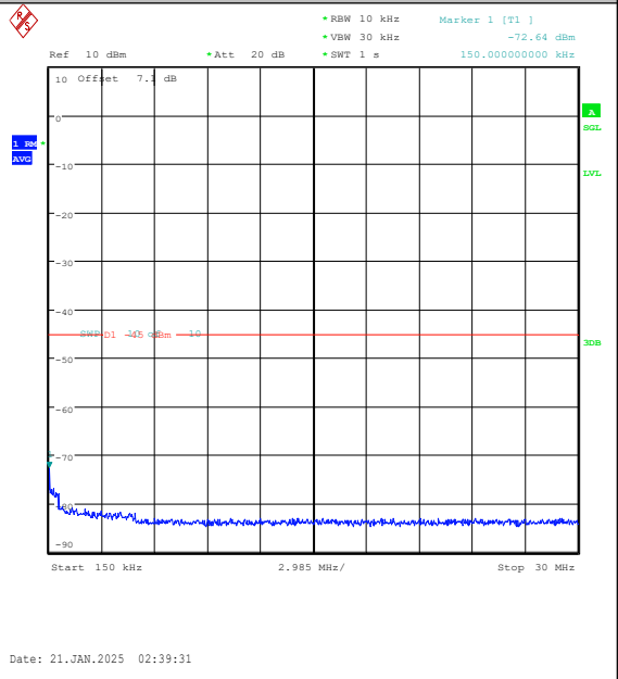
Band7-10MHz-16QAM-21100-1RB#49-0.15~30-PA SS
