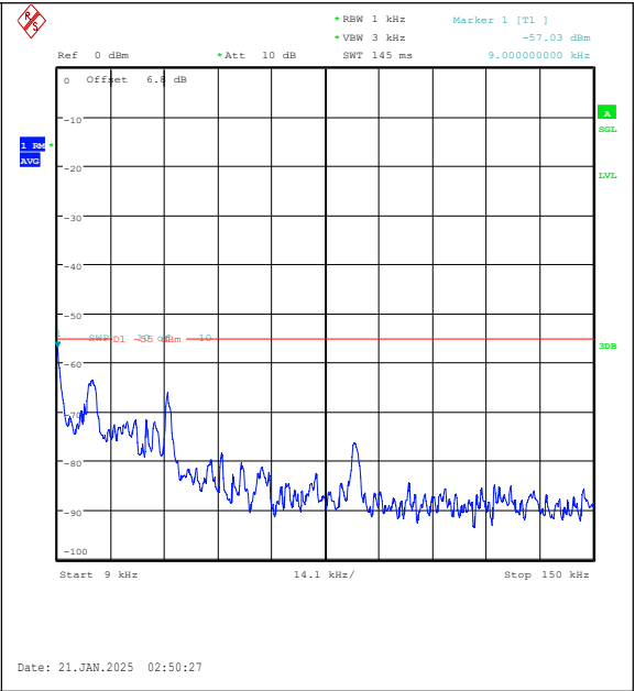
Band7-10MHz-16QAM-21400-50RB#0-0.009~0.15-PASS
