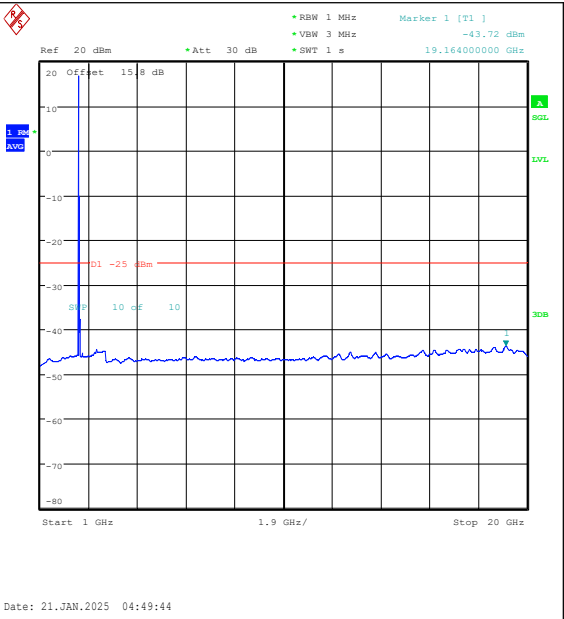
Band7-20MHz-QPSK-21100-1RB#0-1000~20000- PASS
