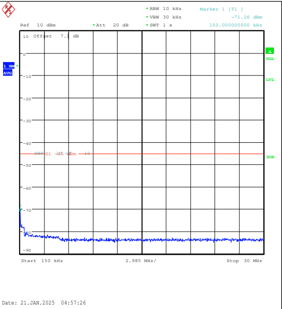
Band7-20MHz-QPSK-21350-1RB#0-0.15~30-PAS
