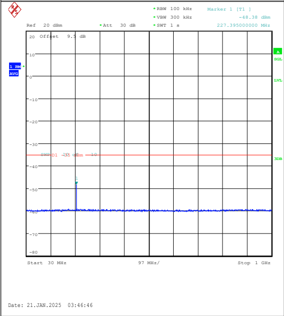
Band7-15MHz-16QAM-21100-1RB#74-30~1000- PASS
