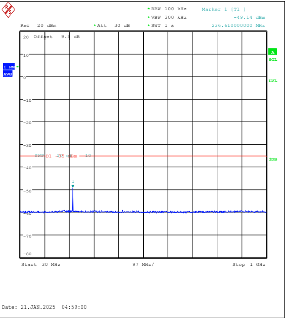
Band7-20MHz-16QAM-21350-1RB#0-30~1000-PA SS
