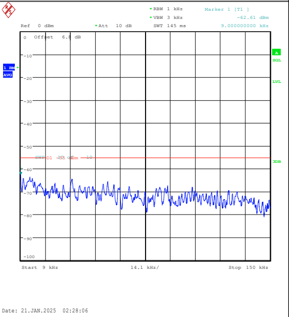
Band7-10MHz-16QAM-20800-1RB#0-0.009~0.15- PASS
