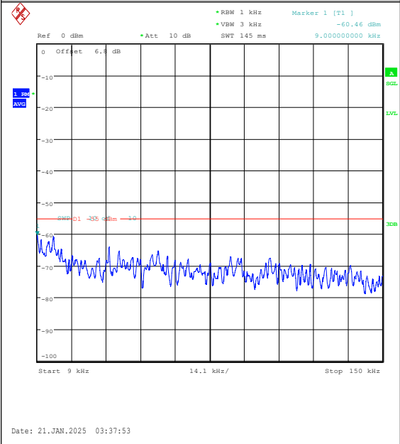
Band7-15MHz-16QAM-20825-1RB#74-0.009~0.1 5-PASS
