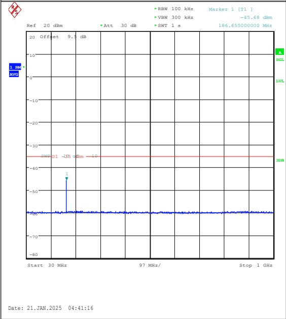
Band7-20MHz-QPSK-20850-1RB#0-30~1000-PA
