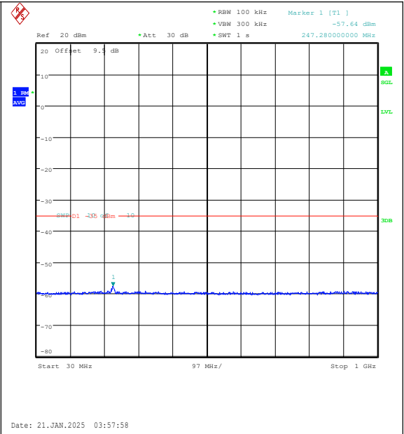
Band7-15MHz-16QAM-21375-75RB#0-30~1000-P ASS
