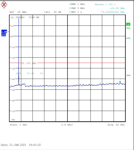
Band7-20MHz-QPSK-20850-1RB#0-1000~20000-PASS
