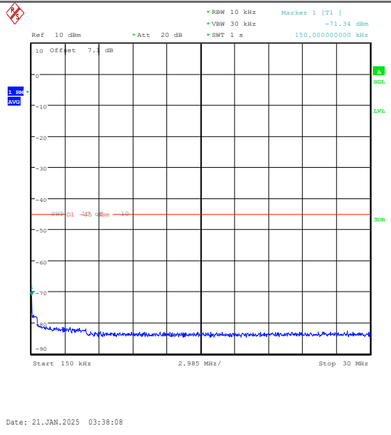
Band7-15MHz-16QAM-20825-1RB#74-0.15~30-P ASS
