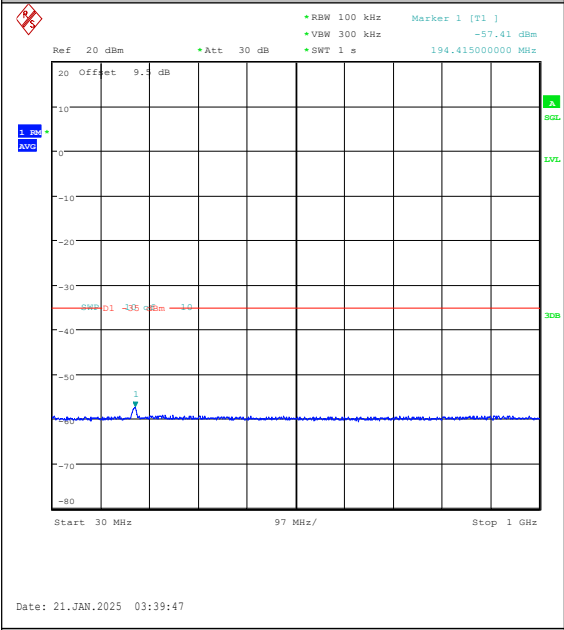
Band7-15MHz-QPSK-20825-75RB#0-30~1000-P ASS
