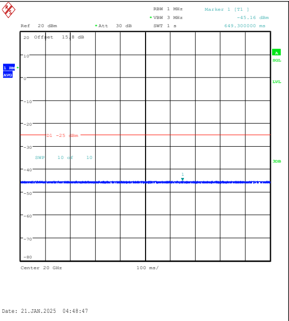
Band7-20MHz-16QAM-20850-100RB#0-20000~27000-PASS
