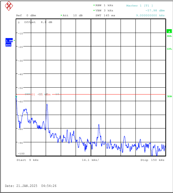
Band7-20MHz-QPSK-21100-100RB#0-0.009~0.1 5-PASS
