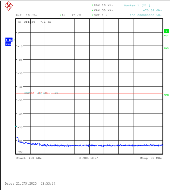
Band7-15MHz-QPSK-21375-1RB#74-0.15~30-PA SS
