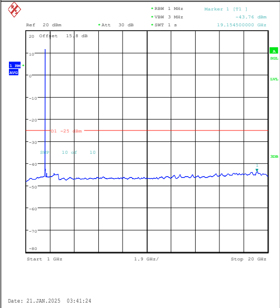
Band7-15MHz-16QAM-20825-75RB#0-1000~200 00-PASS
