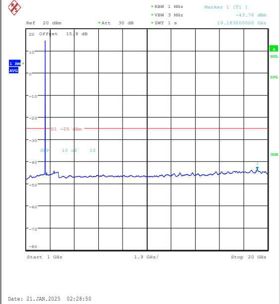
Band7-10MHz-16QAM-20800-1RB#0-1000~2000 0-PASS
