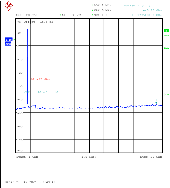
Band7-15MHz-16QAM-21100-75RB#0-1000~200 00-PASS
