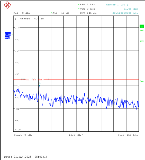
Band7-20MHz-16QAM-21350-1RB#99-0.009~0.1 5-PASS
