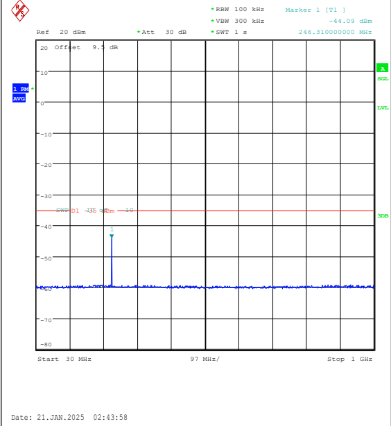
Band7-10MHz-QPSK-21400-1RB#0-30~1000-PA
