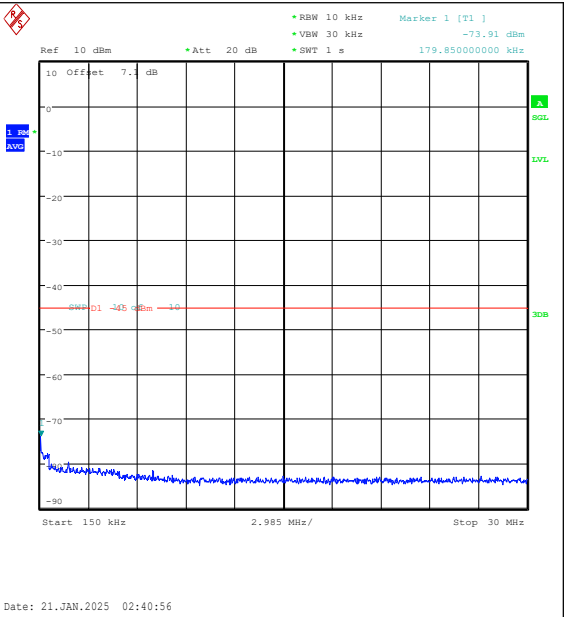
Band7-10MHz-QPSK-21100-50RB#0-0.15~30-PA-SS
