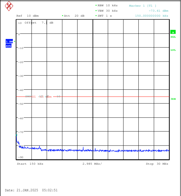
Band7-20MHz-QPSK-21350-100RB#0-0.15~30-PA SS
