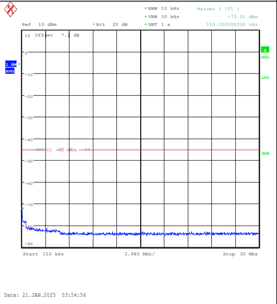
Band7-15MHz-16QAM-21375-1RB#74-0.15~30-P ASS
