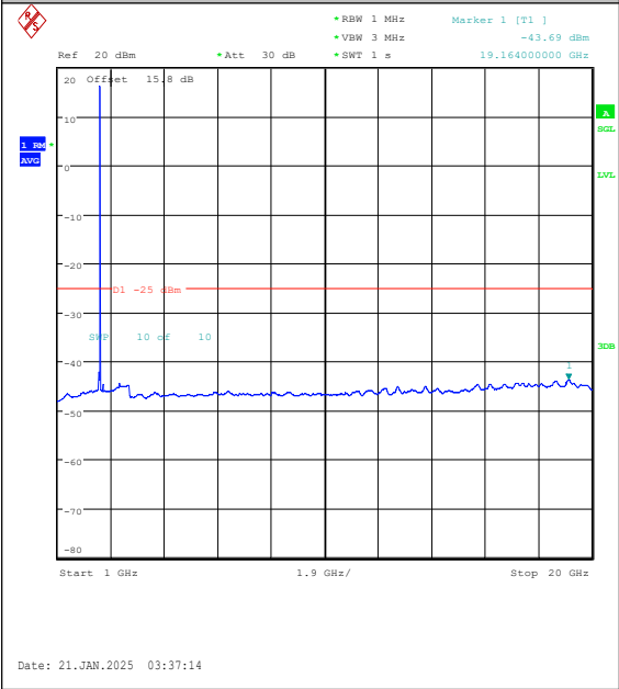
Band7-15MHz-QPSK-20825-1RB#74-1000~2000 0-PASS
