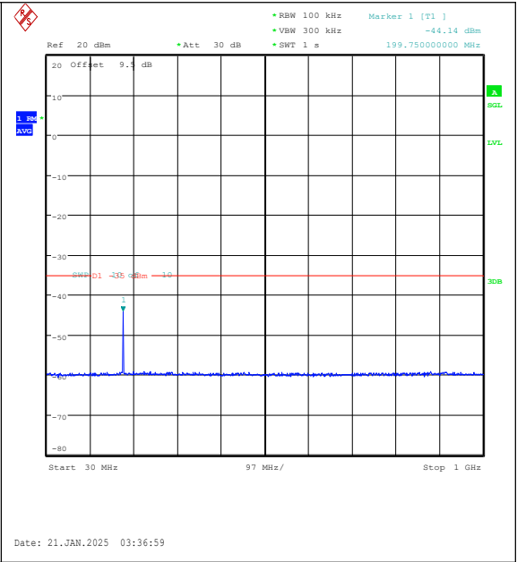
Band7-15MHz-QPSK-20825-1RB#74-30~1000-PA SS
