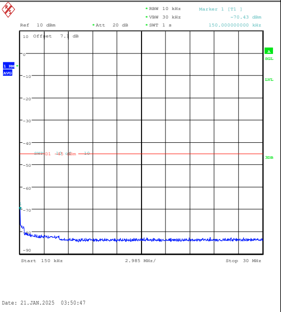
Band7-15MHz-QPSK-21375-1RB#0-0.15~30-PAS S
