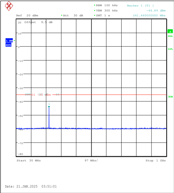
Band7-15MHz-QPSK-21375-1RB#0-30~1000-PA SS
