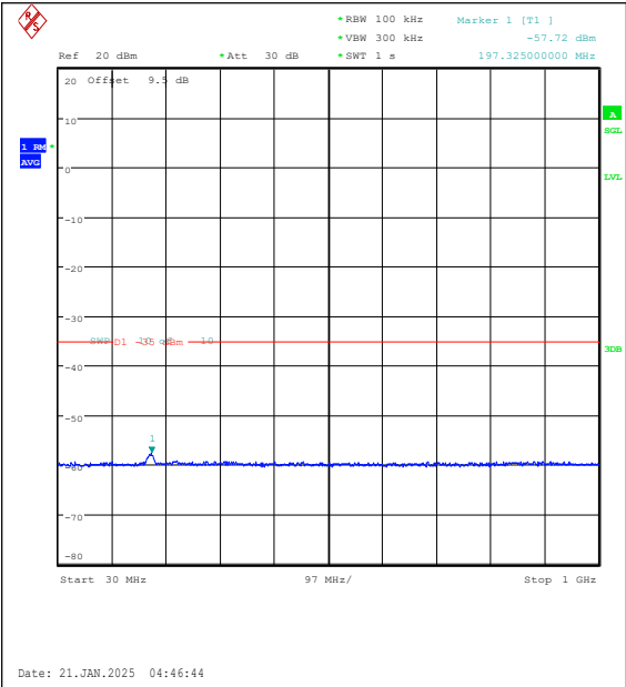
Band7-20MHz-QPSK-20850-100RB#0-30~1000-PASS
