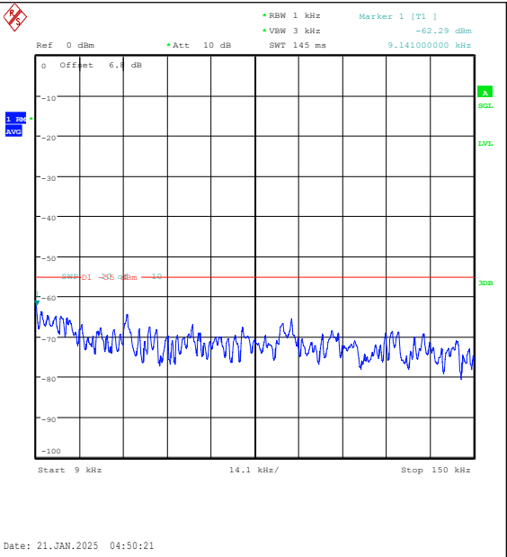
Band7-20MHz-16QAM-21100-1RB#0-0.009~0.15PASS
