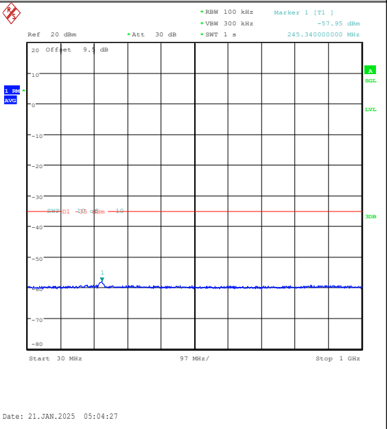
Band7-20MHz-16QAM-21350-100RB#0-30~1000-PASS
