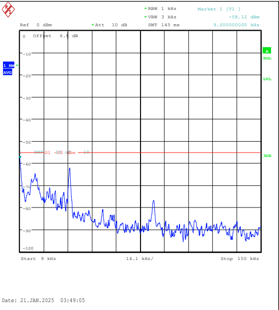
Band7-15MHz-16QAM-21100-75RB#0-0.009~0.15-PASS
