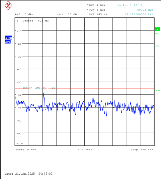
Band7-20MHz-QPSK-21100-1RB#0-0.009~0.15-PASS
