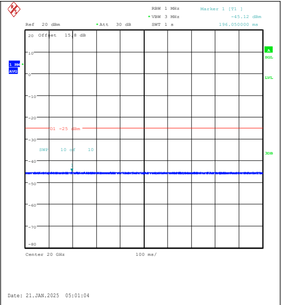
Band7-20MHz-QPSK-21350-1RB#99-20000~2700 0-PASS
