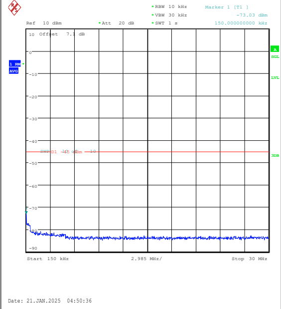
Band7-20MHz-16QAM-21100-1RB#0-0.15~30-PA SS
