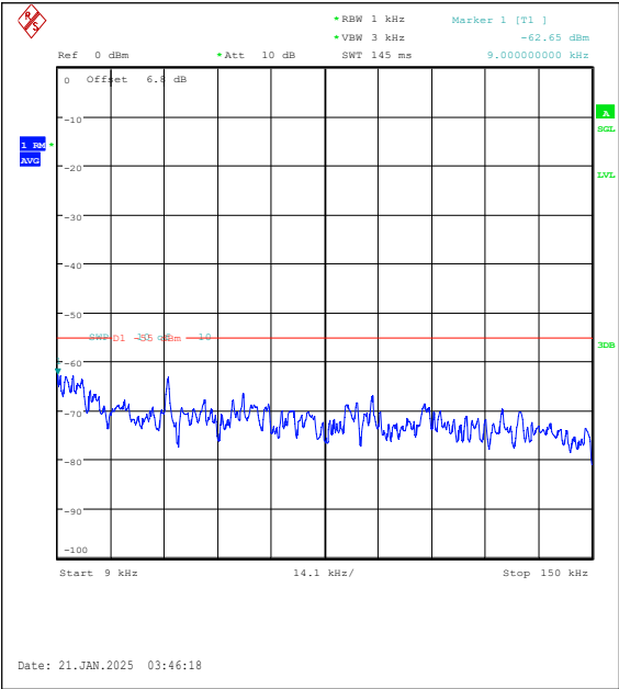
Band7-15MHz-16QAM-21100-1RB#74-0.009~0.1 5-PASS
