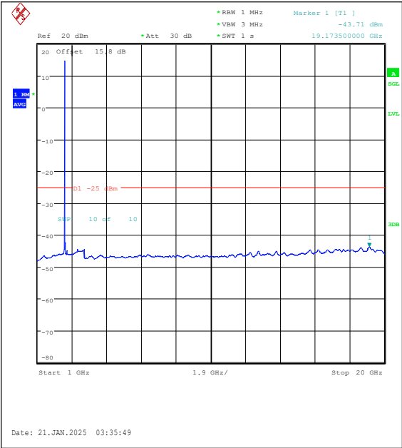
Band7-15MHz-16QAM-20825-1RB#0-1000~2000 0-PASS
