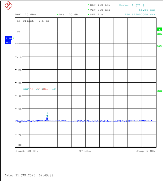
Band7-10MHz-QPSK-21400-50RB#0-30~1000-P ASS
