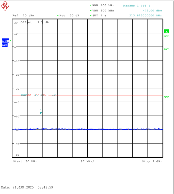
Band7-15MHz-16QAM-21100-1RB#0-30~1000-PA SS
