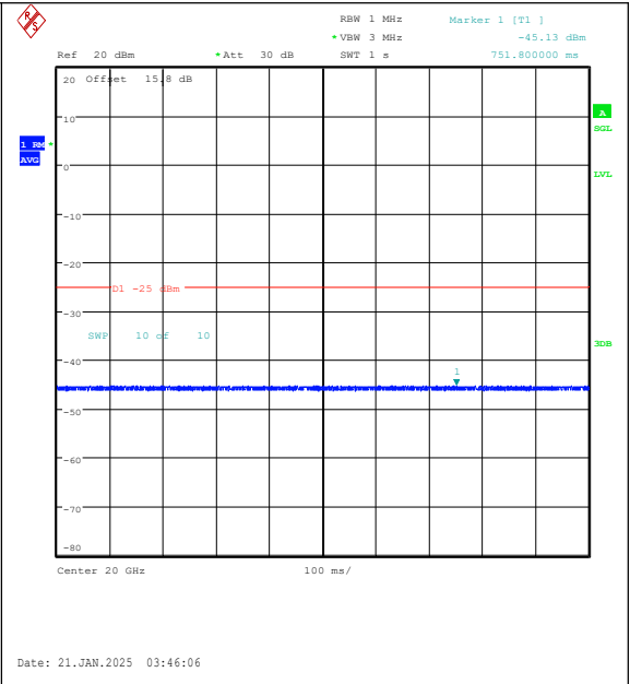
Band7-15MHz-QPSK-21100-1RB#74-20000~2700 0-PASS
