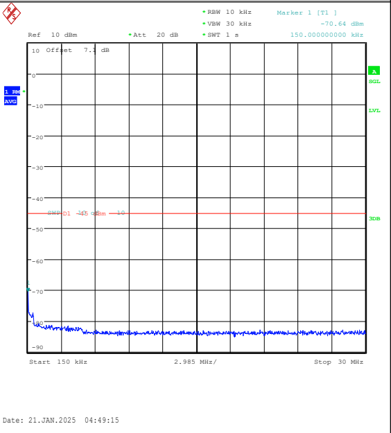
Band7-20MHz-QPSK-21100-1RB#0-0.15~30-PASS
