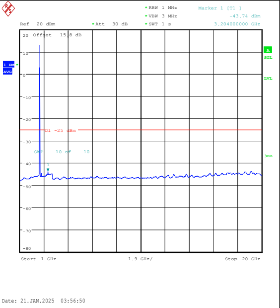
Band7-15MHz-QPSK-21375-75RB#0-1000~20000 -PASS
