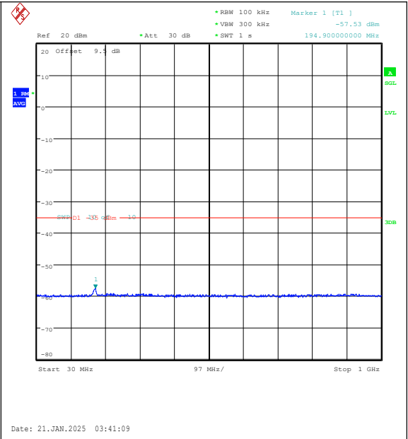
Band7-15MHz-16QAM-20825-75RB#0-30~1000-P ASS
