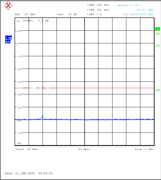
Band7-20MHz-QPSK-21100-100RB#0-30~1000-P ASS
