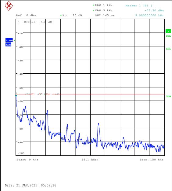
Band7-20MHz-QPSK-21350-100RB#0-0.009~0.1 5-PASS
