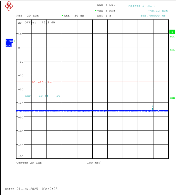
Band7-15MHz-16QAM-21100-1RB#74-20000~27000-PASS
