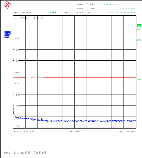
Band7-10MHz-16QAM-20800-50RB#0-0.15~30-PASS
