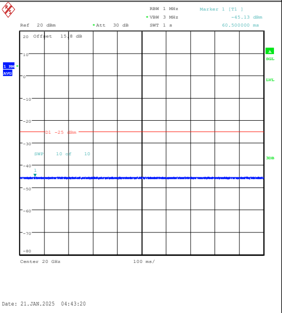
Band7-20MHz-16QAM-20850-1RB#0-20000~2700 0-PASS
