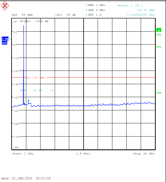
Band7-20MHz-16QAM-21350-1RB#99-1000~2000 0-PASS
