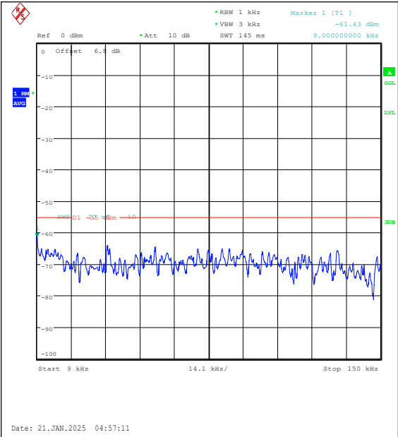
Band7-20MHz-QPSK-21350-1RB#0-0.009~0.15-PASS
