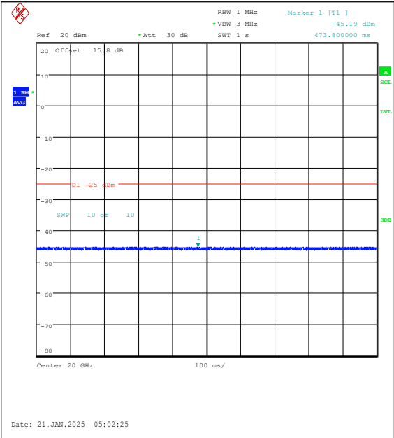
Band7-20MHz-16QAM-21350-1RB#99-20000~27000-PASS
