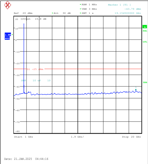
Band7-20MHz-QPSK-20850-1RB#99-1000~2000 0-PASS
