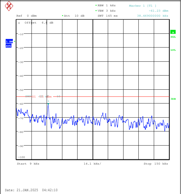
Band7-20MHz-16QAM-20850-1RB#0-0.009~0.15-PASS
