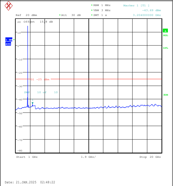
Band7-10MHz-16QAM-21400-1RB#49-1000~2000 0-PASS
