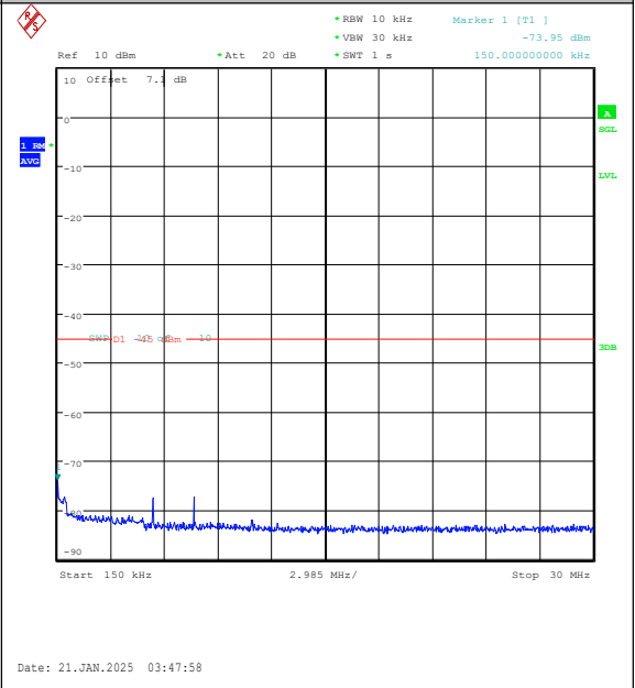
Band7-15MHz-QPSK-21100-75RB#0-0.15~30-PA SS
