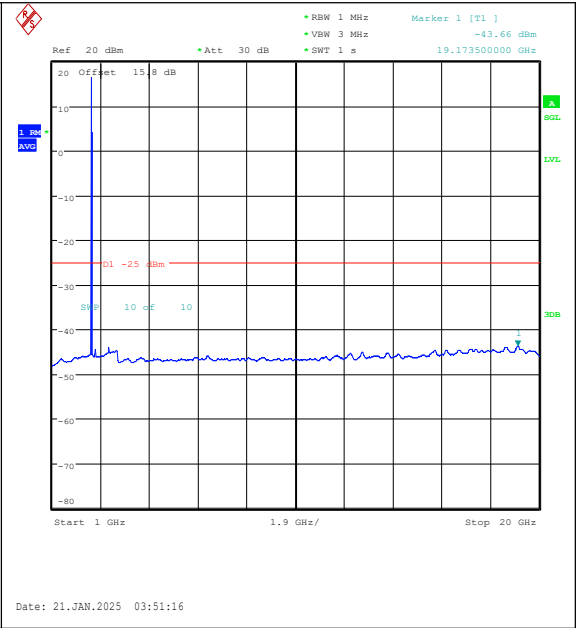
Band7-15MHz-QPSK-21375-1RB#0-1000~20000- PASS
