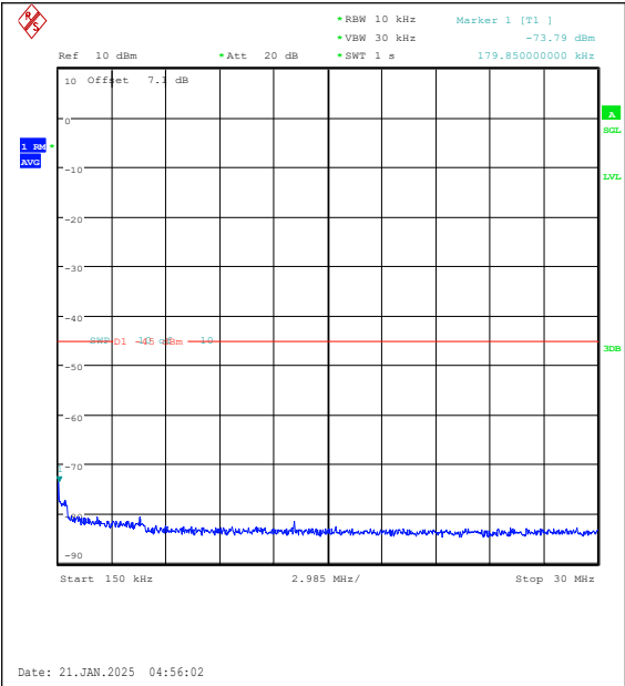
Band7-20MHz-16QAM-21100-100RB#0-0.15~30-PASS
