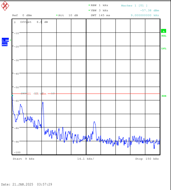
Band7-15MHz-16QAM-21375-75RB#0-0.009~0.15-PASS
