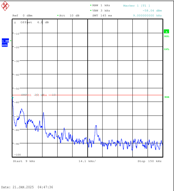
Band7-20MHz-16QAM-20850-100RB#0-0.009~0.15-PASS
