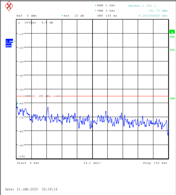
Band7-10MHz-16QAM-21100-1RB#49-0.009~0.1 5-PASS
