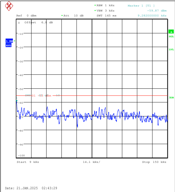
Band7-10MHz-QPSK-21400-1RB#0-0.009~0.15-PASS
