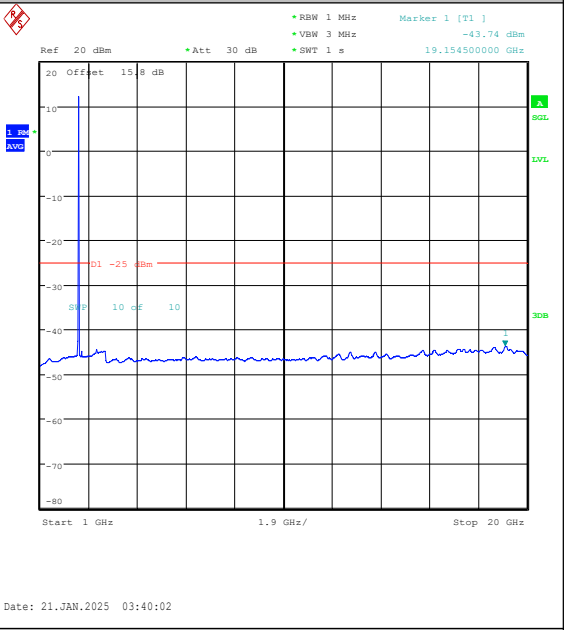
Band7-15MHz-QPSK-20825-75RB#0-1000~20000 -PASS
