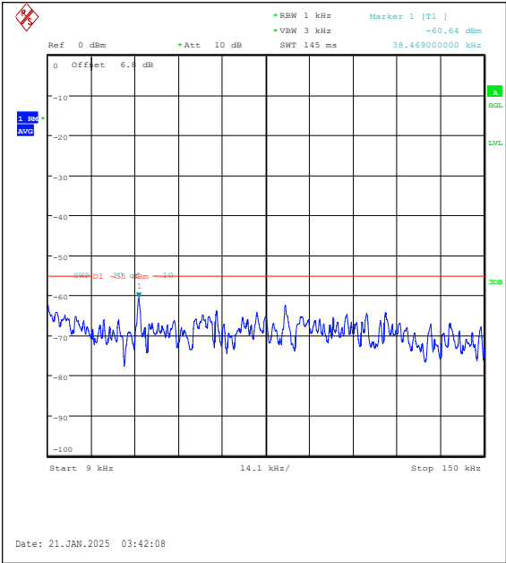
Band7-15MHz-QPSK-21100-1RB#0-0.009~0.15-P ASS
