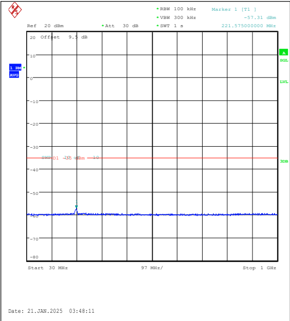
Band7-15MHz-QPSK-21100-75RB#0-30~1000-P ASS
