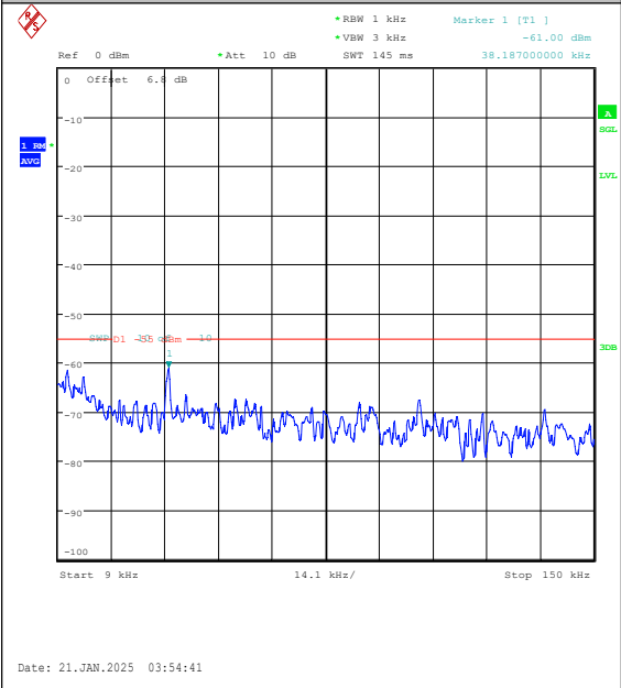
Band7-15MHz-16QAM-21375-1RB#74-0.009~0.1 5-PASS
