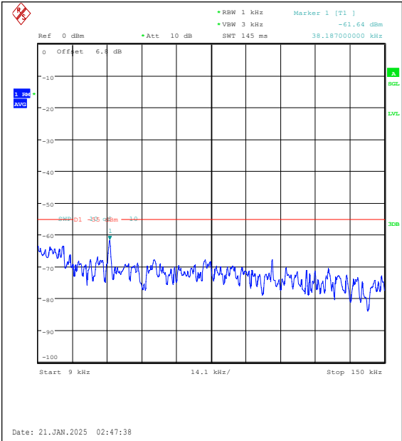
Band7-10MHz-16QAM-21400-1RB#49-0.009~0.1 5-PASS
