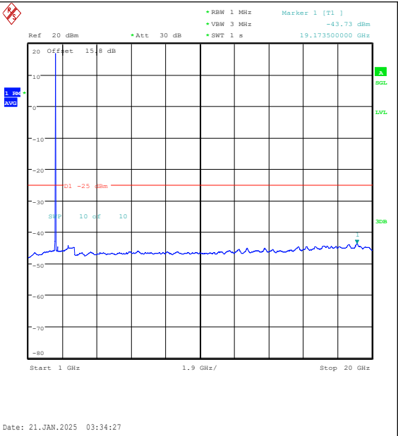
Band7-15MHz-QPSK-20825-1RB#0-1000~20000- PASS
