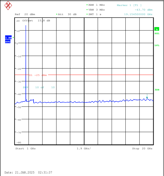
Band7-10MHz-16QAM-20800-1RB#49-1000~2000 0-PASS
