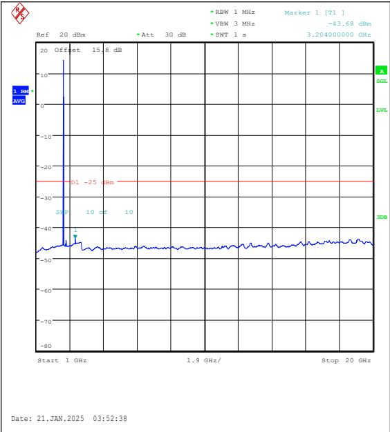
Band7-15MHz-16QAM-21375-1RB#0-1000~2000 0-PASS
