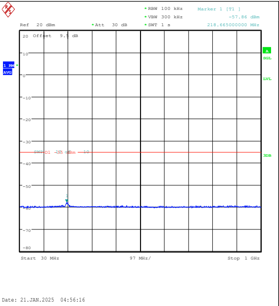
Band7-20MHz-16QAM-21100-100RB#0-30~1000-PASS
