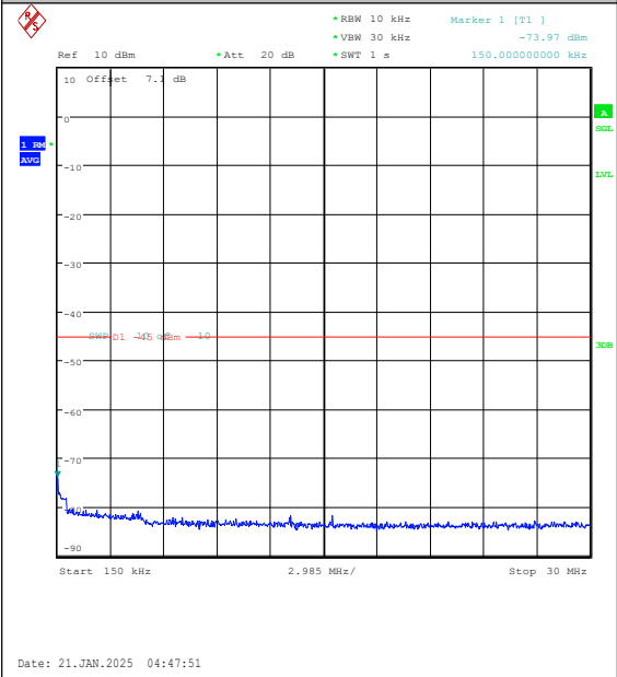
Band7-20MHz-16QAM-20850-100RB#0-0.15~30-PASS
