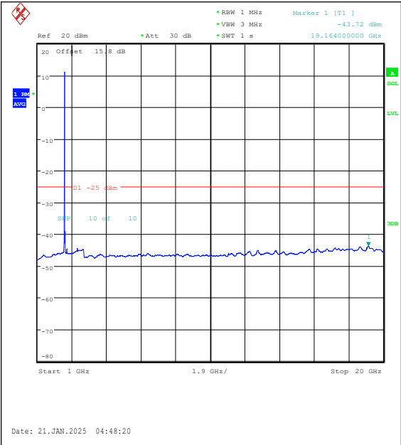
Band7-20MHz-16QAM-20850-100RB#0-1000~20000-PASS
