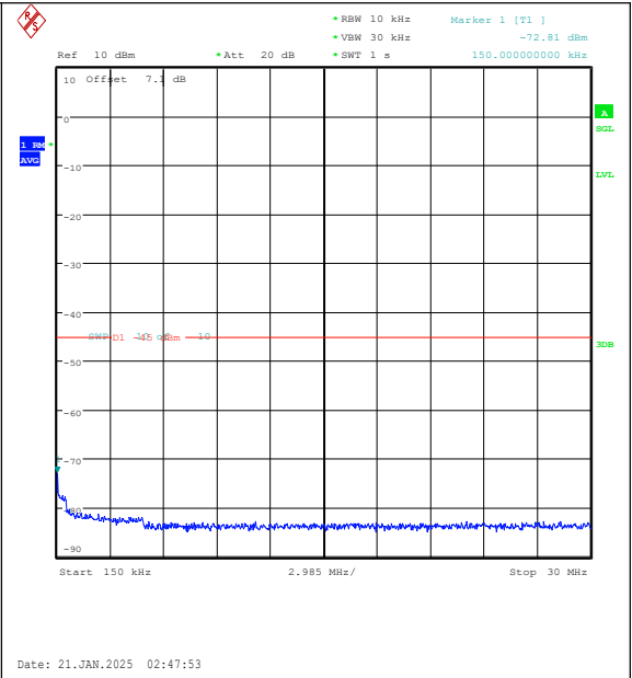
Band7-10MHz-16QAM-21400-1RB#49-0.15~30-P ASS
