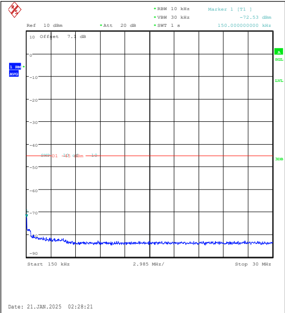
Band7-10MHz-16QAM-20800-1RB#0-0.15~30-PA SS
