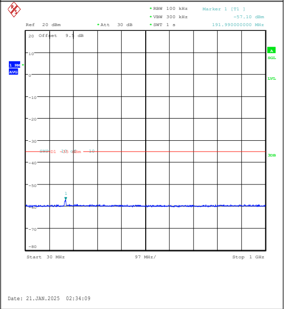
Band7-10MHz-16QAM-20800-50RB#0-30~1000-PASS
