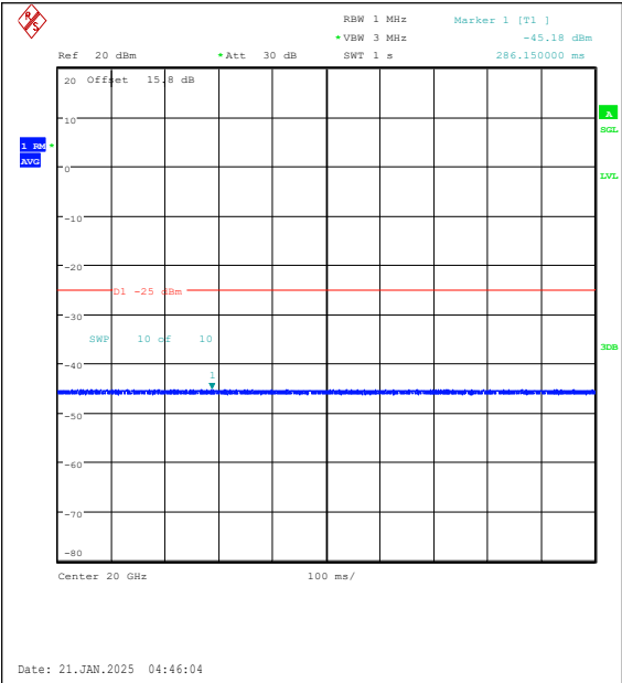
Band7-20MHz-16QAM-20850-1RB#99-20000~27000-PASS
