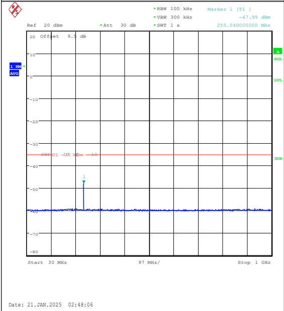
Band7-10MHz-16QAM-21400-1RB#49-30~1000- PASS
