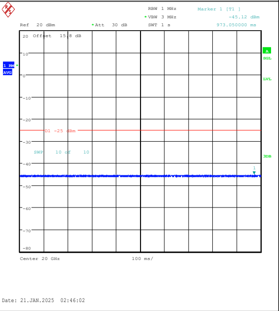
Band7-10MHz-16QAM-21400-1RB#0-20000~2700 0-PASS
