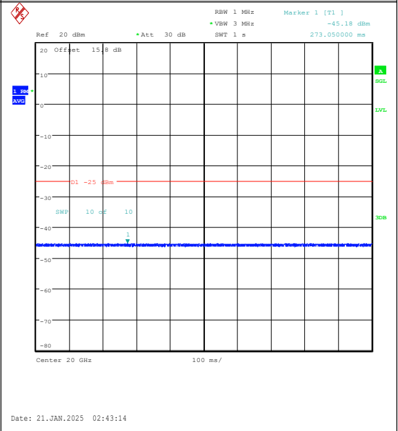
Band7-10MHz-16QAM-21100-50RB#0-20000~270 00-PASS
