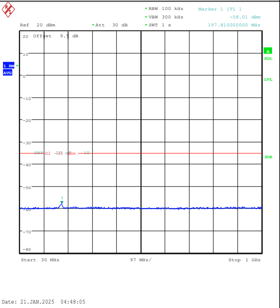
Band7-20MHz-16QAM-20850-100RB#0-30~1000-PASS
