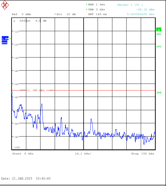
Band7-15MHz-16QAM-20825-75RB#0-0.009~0.15-PASS
