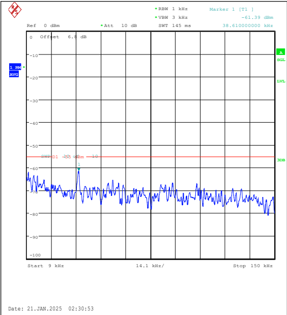
Band7-10MHz-16QAM-20800-1RB#49-0.009~0.1 5-PASS
