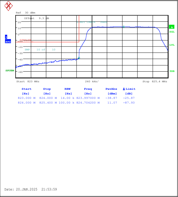
Band5-1.4MHz-16QAM-20407-6RB#0-PASS
