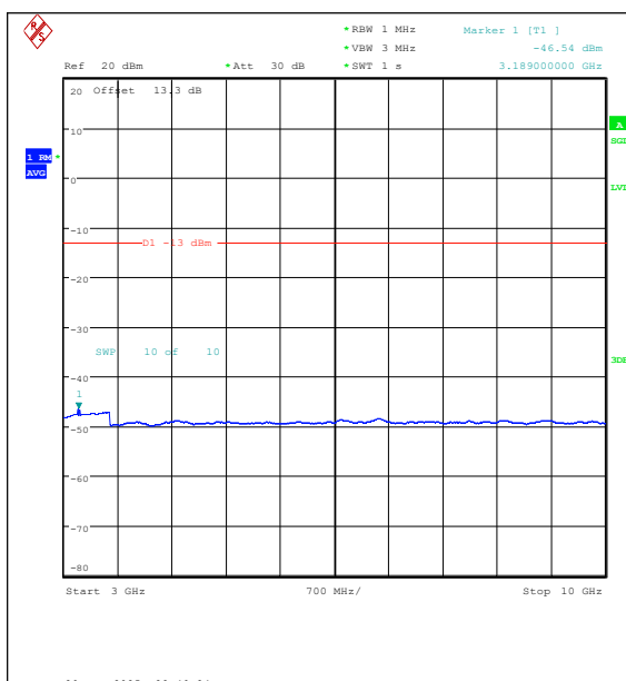
Band5-3MHz-QPSK-20415-1RB#0-3000~10000-P ASS
