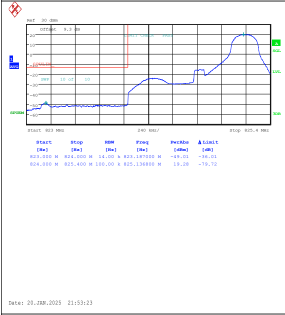
Band5-1.4MHz-16QAM-20407-1RB#5-PASS
