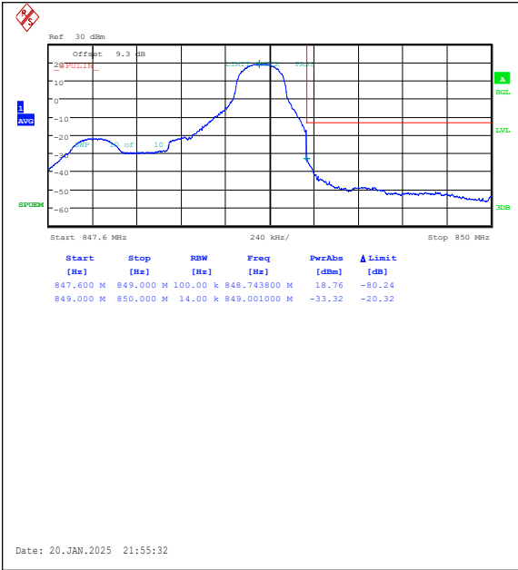
Band5-1.4MHz-16QAM-20643-1RB#5-PASS
