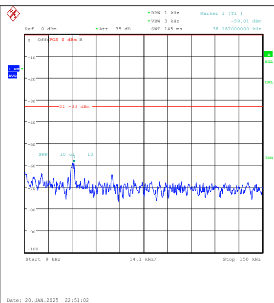
Band5-3MHz-QPSK-20415-1RB#14-0.009~0.15-P ASS
