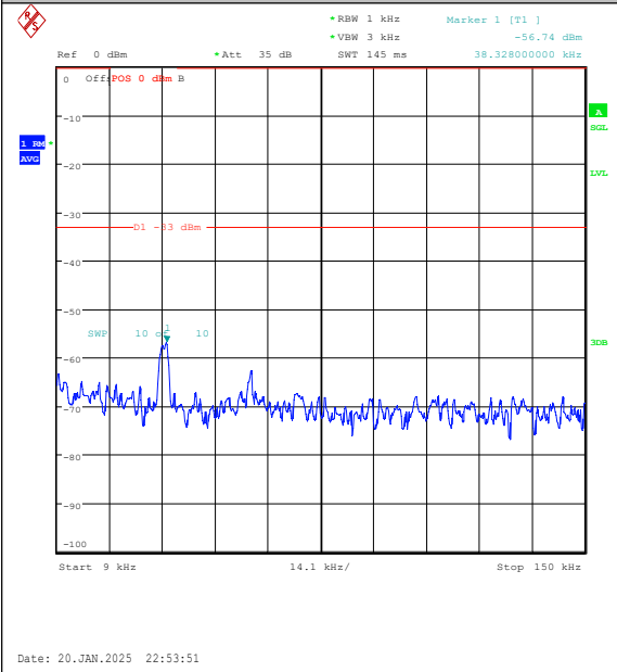
Band5-3MHz-QPSK-20415-15RB#0-0.009~0.15-P ASS
