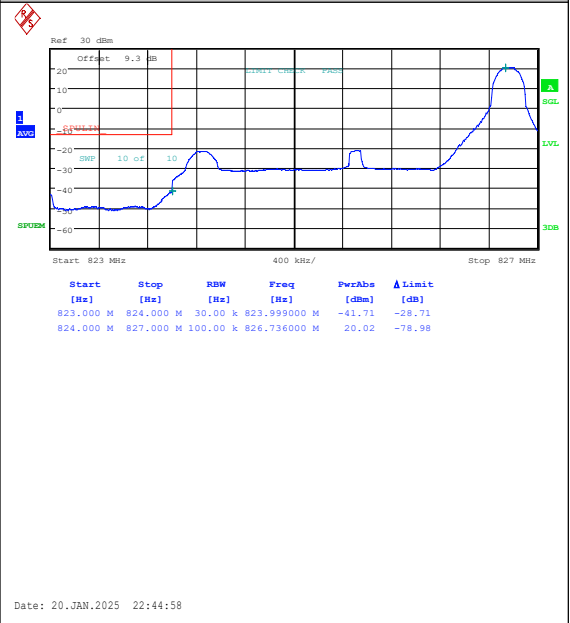
Band5-3MHz-QPSK-20415-1RB#14-PASS
