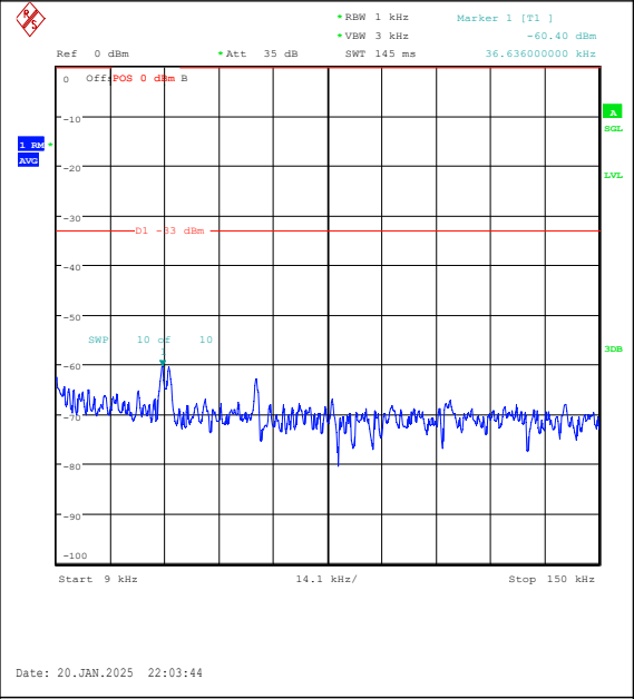
Band5-1.4MHz-16QAM-20407-6RB#0-0.009~0.15 -PASS
