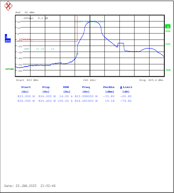
Band5-1.4MHz-16QAM-20407-1RB#0-PASS
