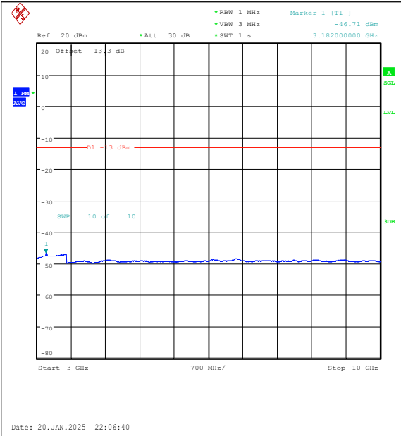
Band5-1.4MHz-QPSK-20525-1RB#0-3000~10000 -PASS
