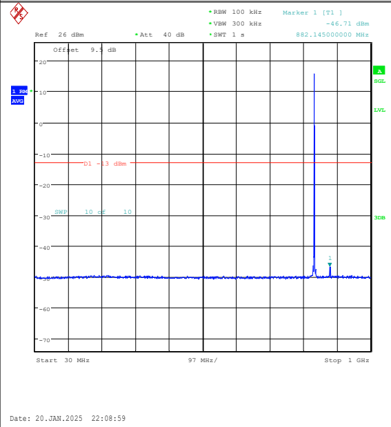
Band5-1.4MHz-QPSK-20525-1RB#5-30~1000-PA SS
