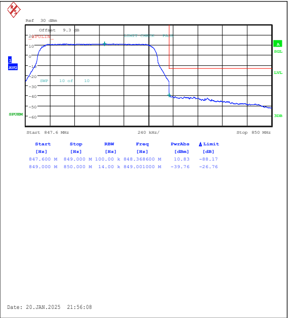
Band5-1.4MHz-16QAM-20643-6RB#0-PASS
