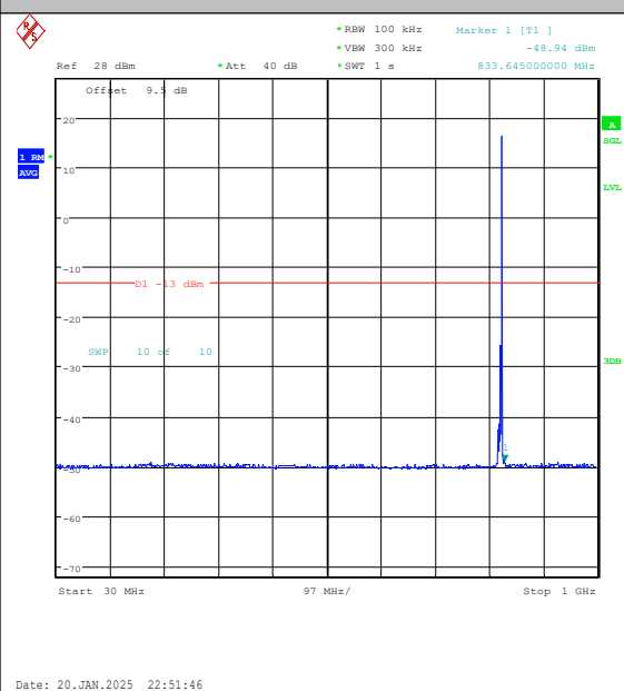
Band5-3MHz-QPSK-20415-1RB#14-30~1000-PA SS
