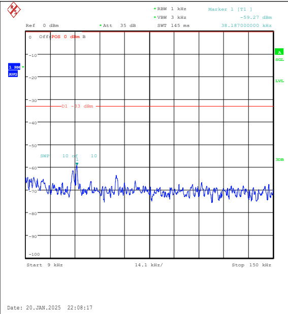
Band5-1.4MHz-QPSK-20525-1RB#5-0.009~0.15- PASS
