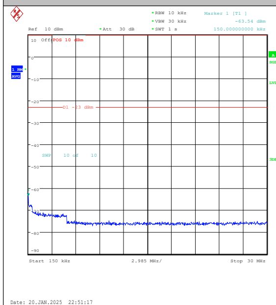
Band5-3MHz-QPSK-20415-1RB#14-0.15~30-PAS S
