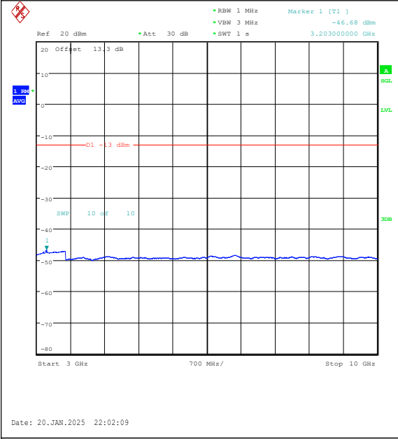
Band5-1.4MHz-16QAM-20407-1RB#5-3000~1000 0-PASS
