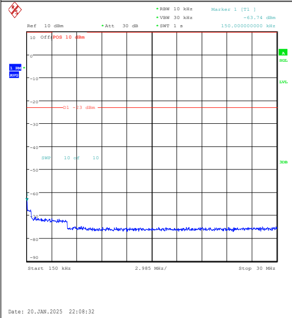
Band5-1.4MHz-QPSK-20525-1RB#5-0.15~30-PA SS
