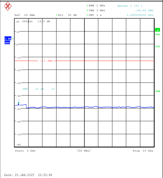
Band5-3MHz-16QAM-20415-1RB#0-3000~10000- PASS
