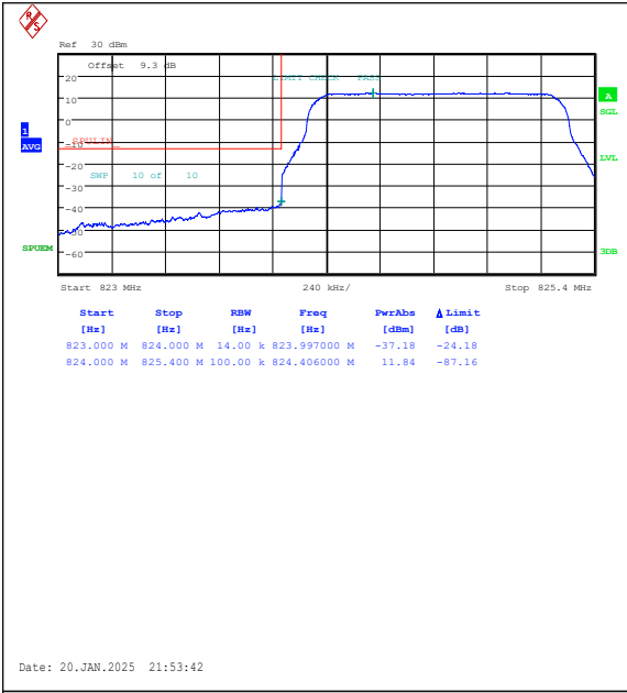
Band5-1.4MHz-QPSK-20407-6RB#0-PASS
