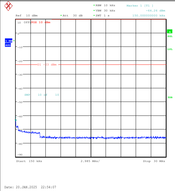
Band5-3MHz-QPSK-20415-15RB#0-0.15~30-PAS S
