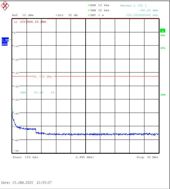
Band2-1.4MHz-QPSK-18900-6RB#0-0.15~30-PAS
