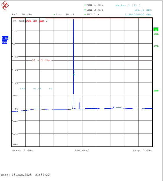
Band2-1.4MHz-16QAM-18900-1RB#5-1000~3000- PASS
