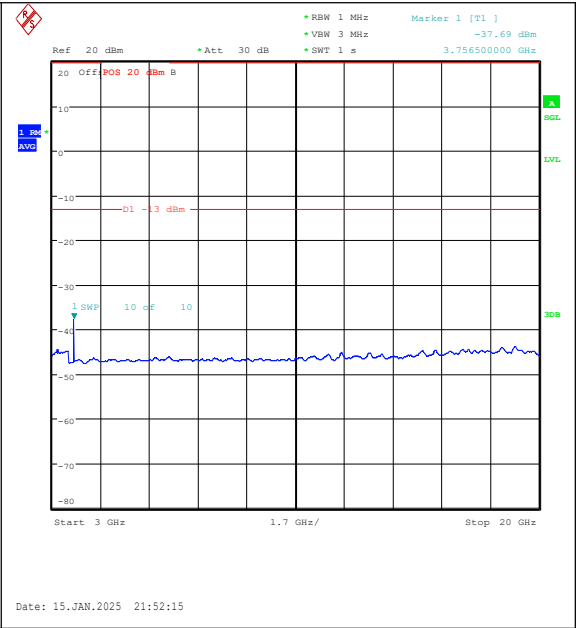
Band2-1.4MHz-16QAM-18900-1RB#0-3000~2000 0-PASS
