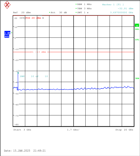
Band2-1.4MHz-QPSK-18607-6RB#0-3000~20000 -PASS
