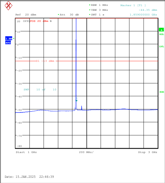
Band2-3MHz-QPSK-18615-1RB#14-1000~3000- PASS
