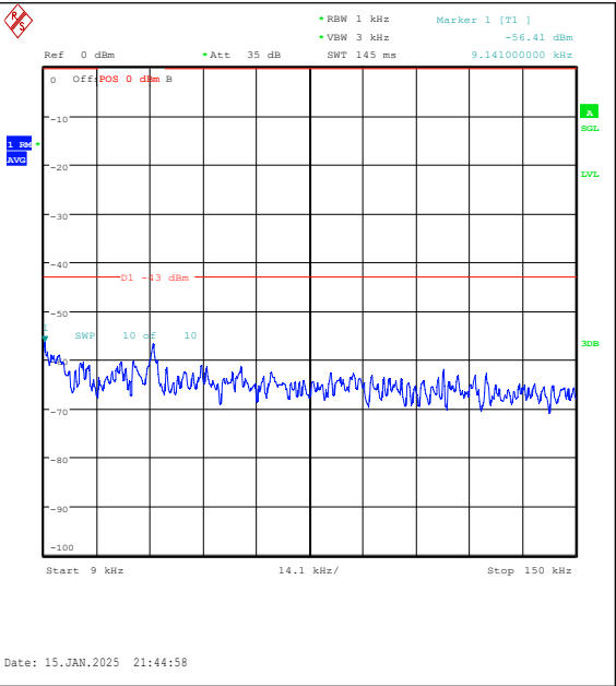
Band2-1.4MHz-QPSK-18607-1RB#5-0.009~0.15-P ASS
