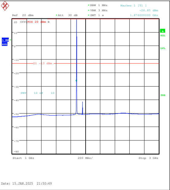
Band2-1.4MHz-QPSK-18900-1RB#0-1000~3000-P ASS
