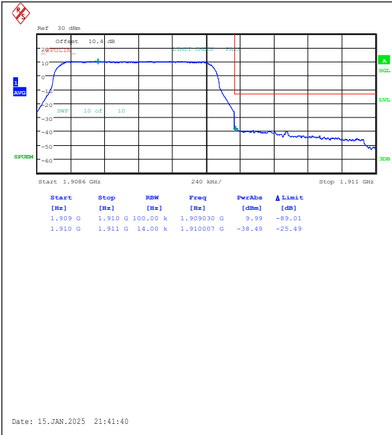
Band2-1.4MHz-QPSK-19193-6RB#0-PASS
