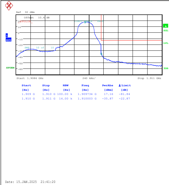
Band2-1.4MHz-16QAM-19193-1RB#5-PASS
