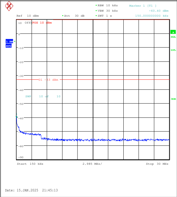
Band2-1.4MHz-QPSK-18607-1RB#5-0.15~30-PA SS
