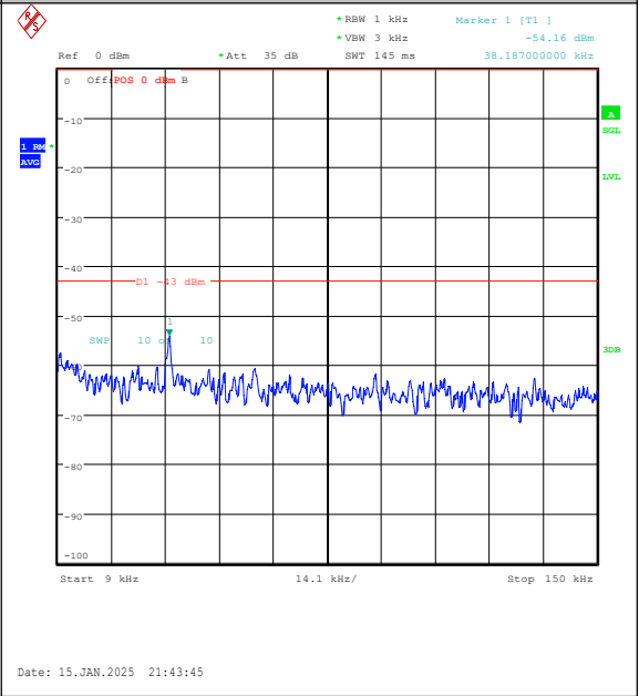
Band2-1.4MHz-16QAM-18607-1RB#0-0.009~0.15- PASS
