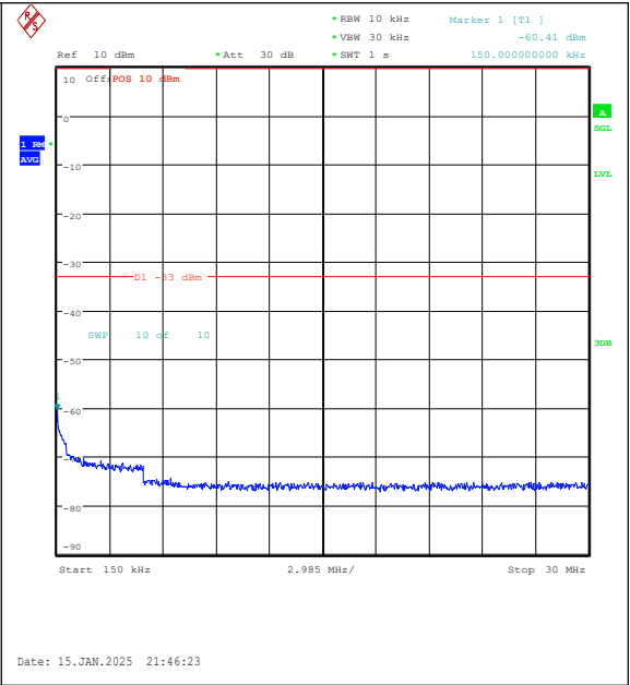
Band2-1.4MHz-16QAM-18607-1RB#5-0.15~30-PA SS
