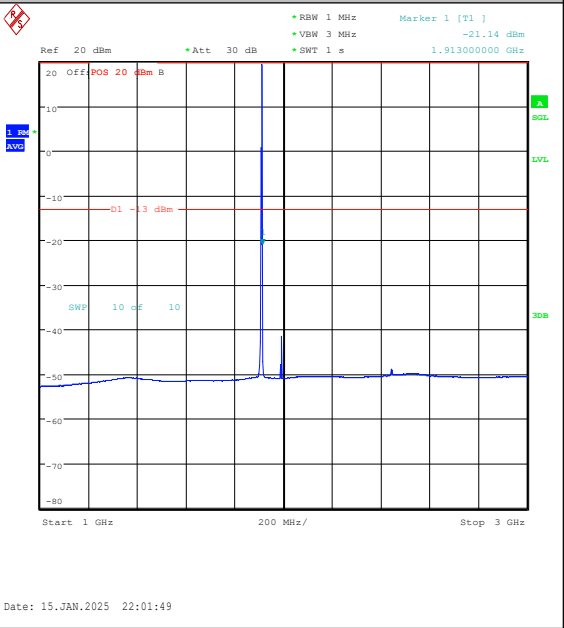
Band2-1.4MHz-16QAM-19193-1RB#5-1000~3000- PASS
