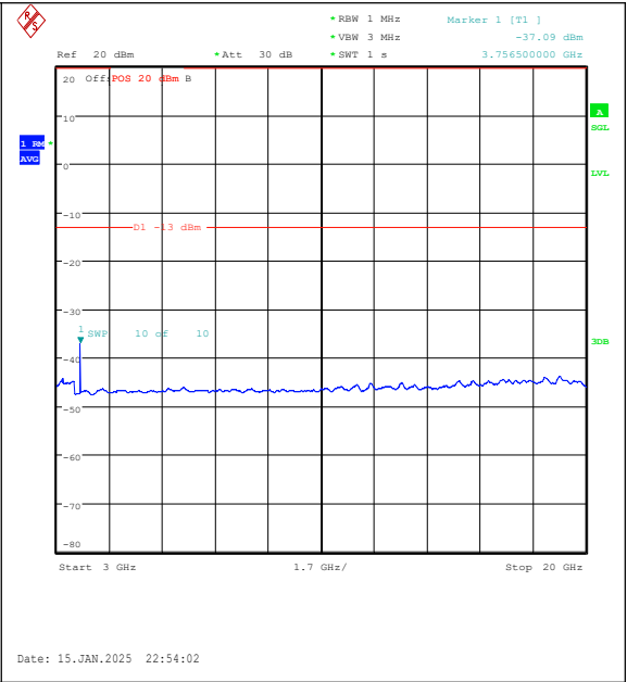
Band2-3MHz-QPSK-18900-1RB#14-3000~20000-PASS
