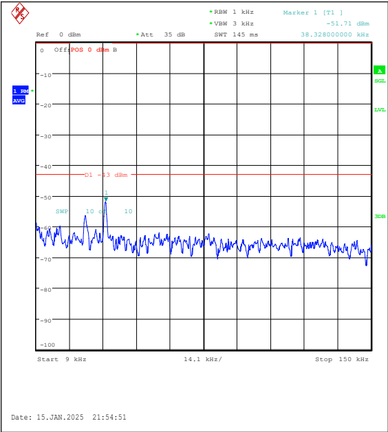
Band2-1.4MHz-QPSK-18900-6RB#0-0.009~0.15-PASS
