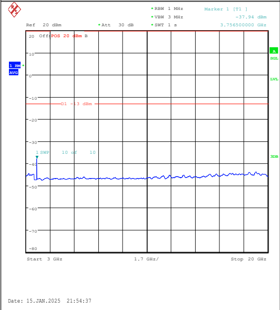
Band2-1.4MHz-16QAM-18900-1RB#5-3000~200 00-PASS
