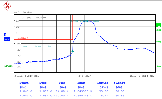
Band2-1.4MHz-QPSK-18607-1RB#5-PASS
