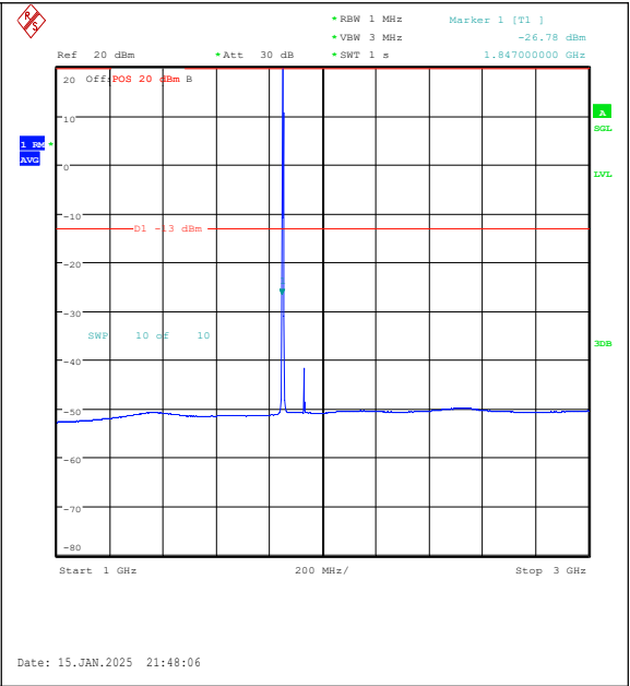
Band2-1.4MHz-QPSK-18607-6RB#0-1000~3000-P ASS
