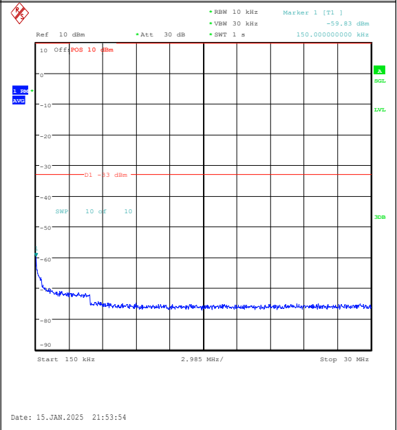
Band2-1.4MHz-16QAM-18900-1RB#5-0.15~30-PA SS
