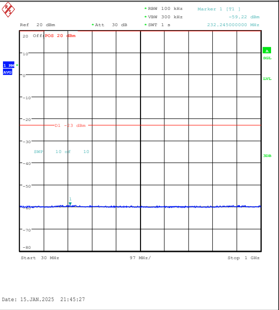
Band2-1.4MHz-QPSK-18607-1RB#5-30~1000-PA SS
