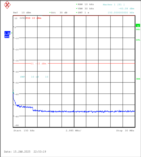
Band2-3MHz-QPSK-18900-1RB#14-0.15~30-PA SS
