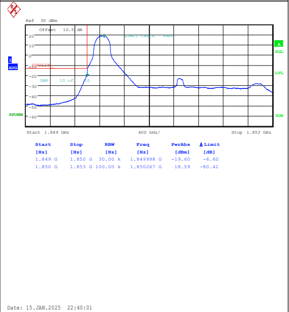
Band2-3MHz-16QAM-18615-1RB#0-PASS
