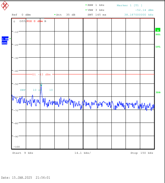
Band2-1.4MHz-16QAM-18900-6RB#0-0.009~0.15- PASS
