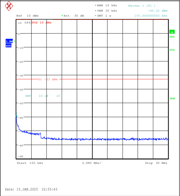
Band2-3MHz-QPSK-18900-15RB#0-0.15~30-PAS S
