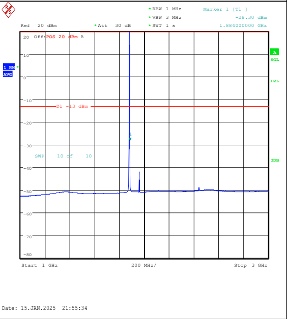
Band2-1.4MHz-QPSK-18900-6RB#0-1000~3000-P
