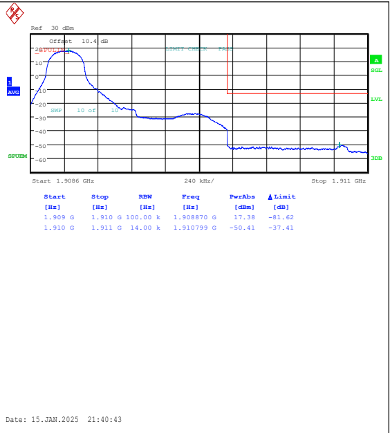
Band2-1.4MHz-16QAM-19193-1RB#0-PASS
