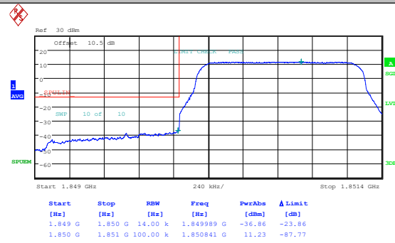
Band2-1.4MHz-QPSK-18607-1RB#0-PASS
