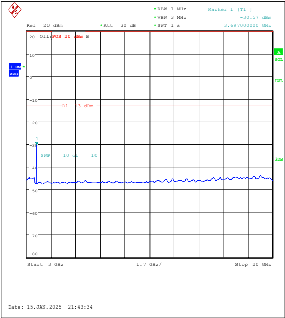
Band2-1.4MHz-QPSK-18607-1RB#0-3000~20000 -PASS
