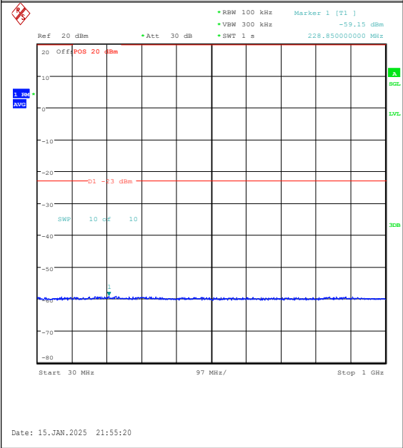
Band2-1.4MHz-QPSK-18900-6RB#0-30~1000-PA
