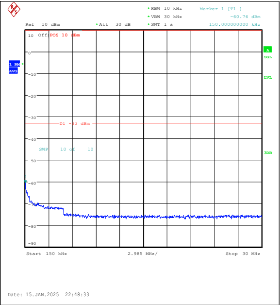
Band2-3MHz-QPSK-18615-15RB#0-0.15~30-PAS
