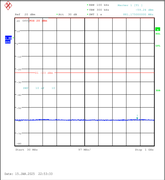
Band2-3MHz-QPSK-18900-1RB#14-30~1000-PAS S
