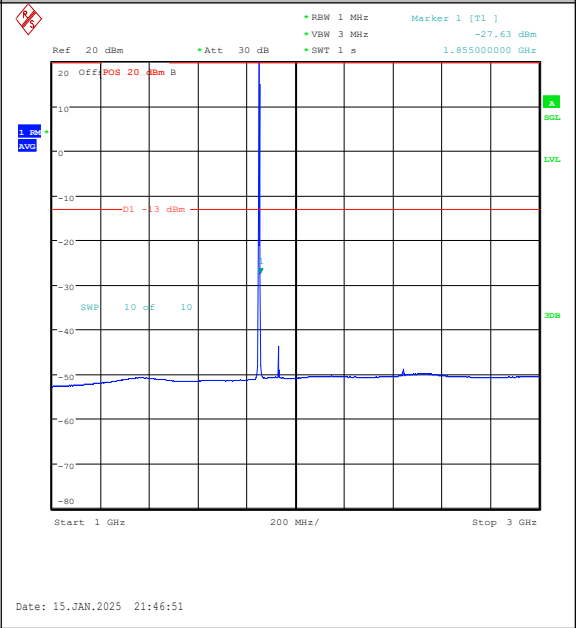
Band2-1.4MHz-16QAM-18607-1RB#5-1000~3000-P PASS
