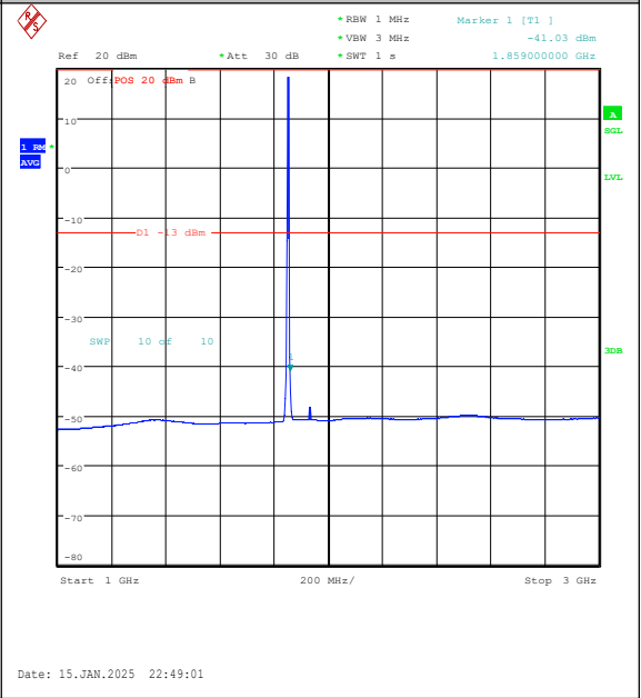
Band2-3MHz-QPSK-18615-15RB#0-1000~3000-P
