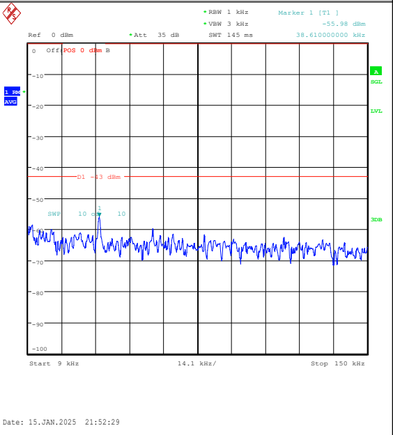
Band2-1.4MHz-QPSK-18900-1RB#5-0.009~0.15-P ASS
