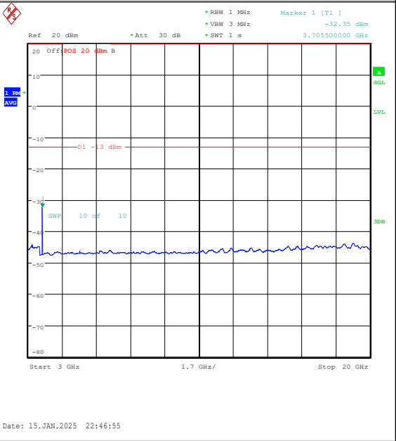
Band2-3MHz-QPSK-18615-1RB#14-3000~20000- PASS
