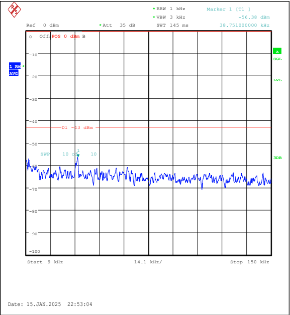
Band2-3MHz-QPSK-18900-1RB#14-0.009~0.15-P ASS
