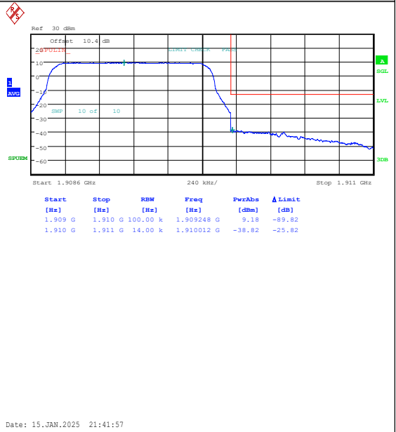
Band2-1.4MHz-16QAM-19193-6RB#0-PASS
