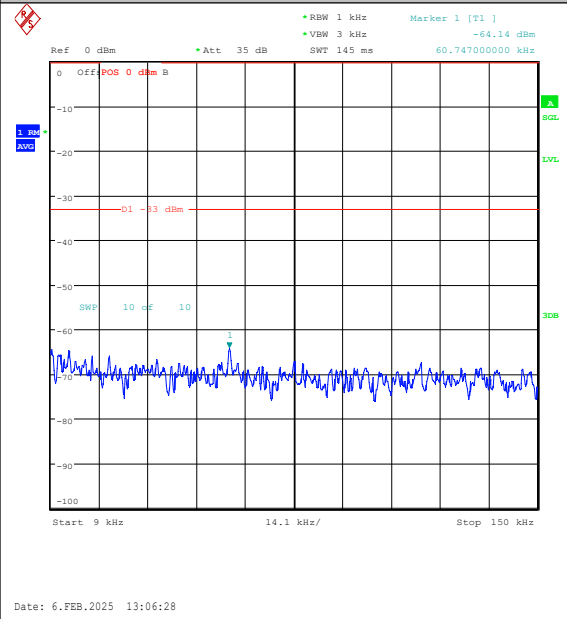
Band26(824-849)-15MHz-16QAM-26965-75RB#0- 0.009~0.15-PASS
