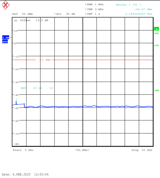
Band26(824-849)-10MHz-QPSK-26915-1RB#49-3 000~10000-PASS
