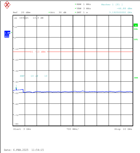
Band26(824-849)-10MHz-QPSK-26840-1RB#0-30 00~10000-PASS
