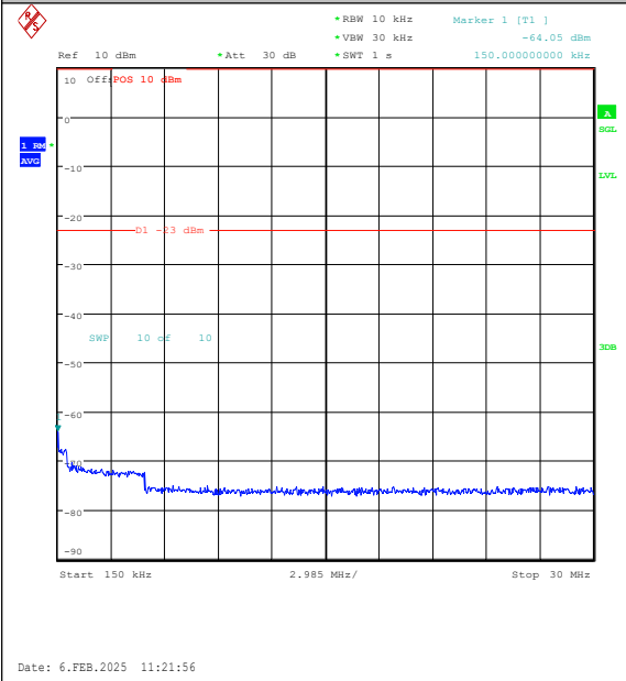
Band26(824-849)-5MHz-16QAM-27015-1RB#0-0. 15~30-PASS
