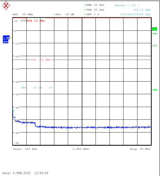
Band26(824-849)-10MHz-QPSK-26915-50RB#0-0 .15~30-PASS
