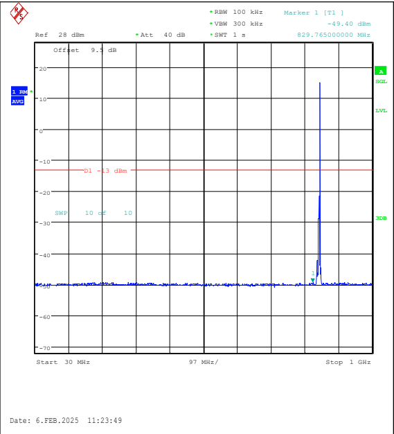
Band26(824-849)-5MHz-QPSK-27015-1RB#24-30 ~1000-PASS
