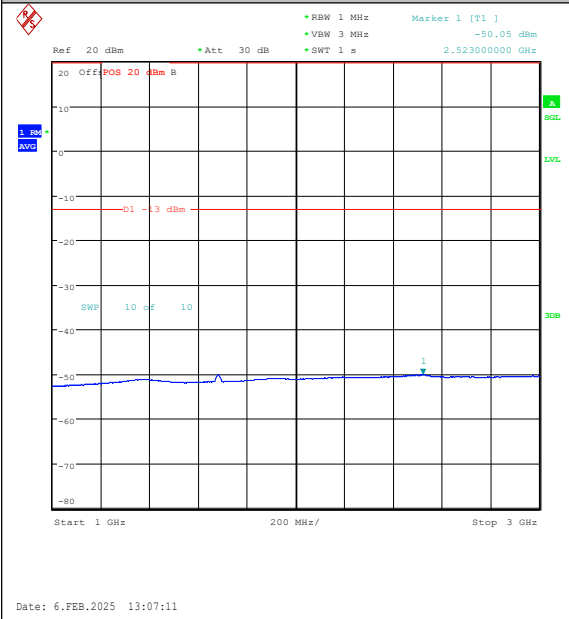
Band26(824-849)-15MHz-16QAM-26965-75RB#0-1000~3000-PASS
