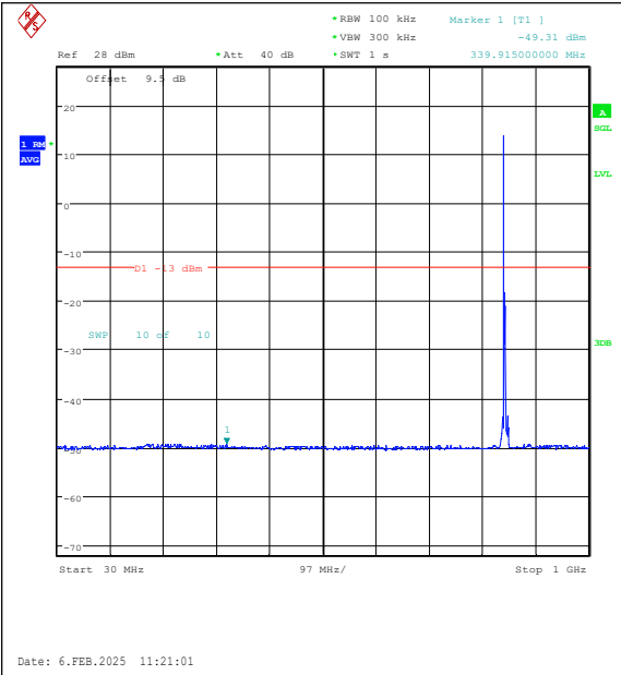
Band26(824-849)-5MHz-QPSK-27015-1RB#0-30~1000-PASS
