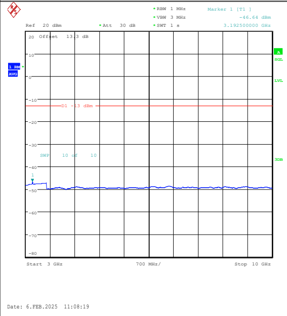
Band26(824-849)-5MHz-QPSK-26815-1RB#24-30 00~10000-PASS
