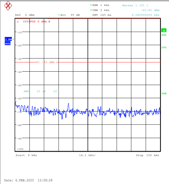
Band26(824-849)-15MHz-16QAM-26915-75RB#0-0.009~0.15-PASS
