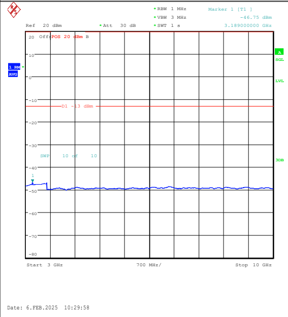
Band26(824-849)-3MHz-16QAM-26915-15RB#0-3 000~10000-PASS
