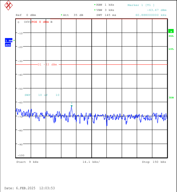
Band26(824-849)-10MHz-QPSK-26915-1RB#49-0 .009~0.15-PASS
