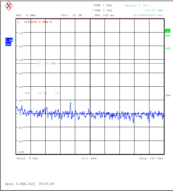
Band26(824-849)-1.4MHz-QPSK-27033-6RB#0-0. 009~0.15-PASS
