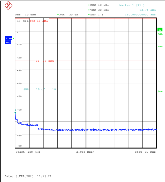
Band26(824-849)-5MHz-QPSK-27015-1RB#24-0. 15~30-PASS
