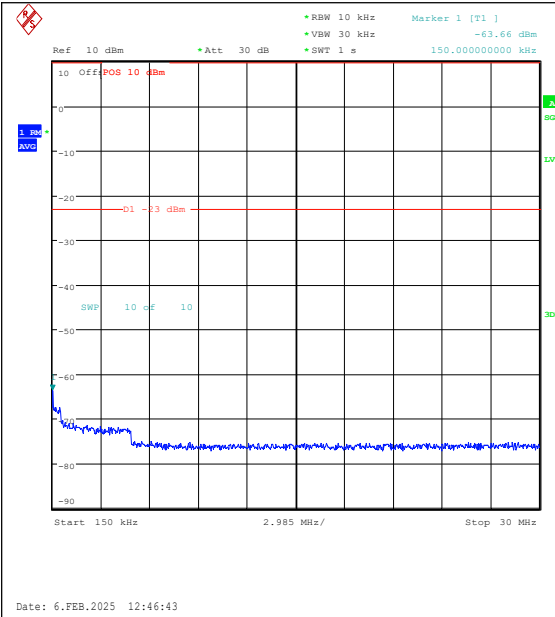
Band26(824-849)-15MHz-QPSK-26865-1RB#74-0 .15~30-PASS
