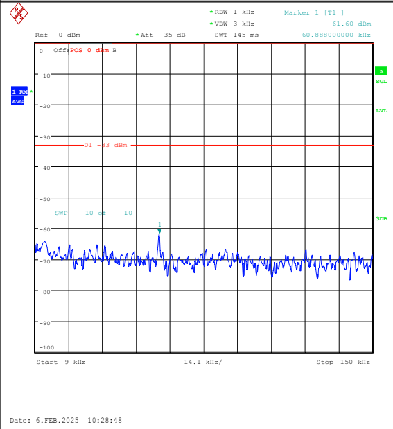
Band26(824-849)-3MHz-16QAM-26915-15RB#0-0 .009~0.15-PASS
