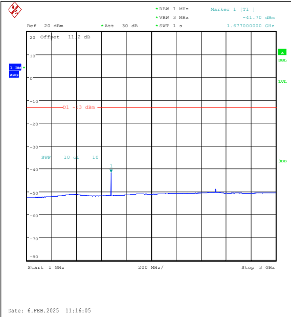
Band26(824-849)-5MHz-QPSK-26915-1RB#24-10 00~3000-PASS
