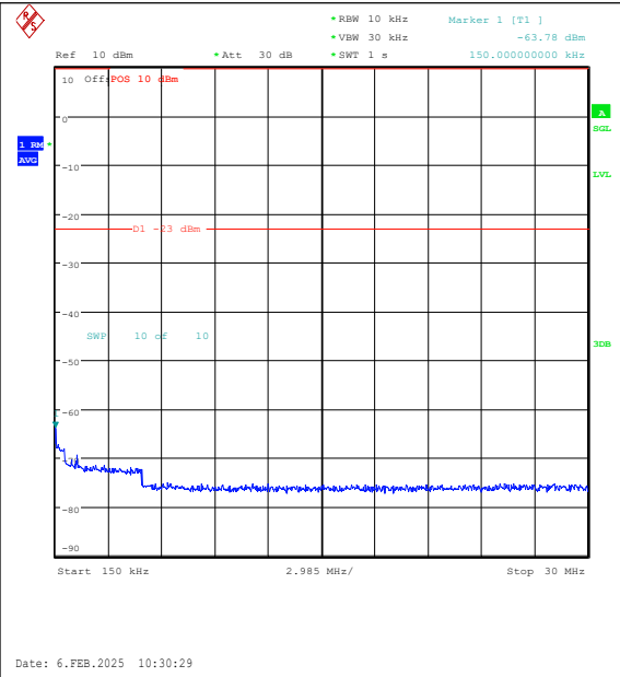
Band26(824-849)-3MHz-QPSK-27025-1RB#0-0.1 5~30-PASS
