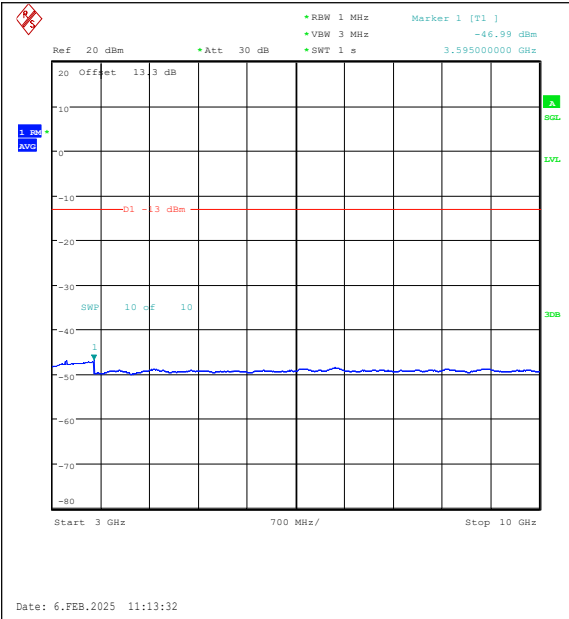
Band26(824-849)-5MHz-QPSK-26915-1RB#0-300 0~10000-PASS
