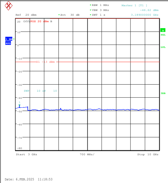
Band26(824-849)-5MHz-QPSK-26915-25RB#0-30 00~10000-PASS
