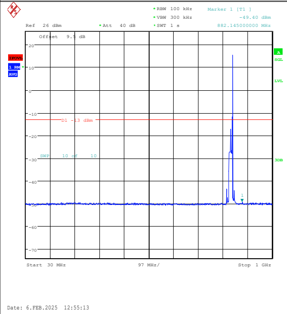
Band26(824-849)-15MHz-QPSK-26915-1RB#74-3 0~1000-PASS
