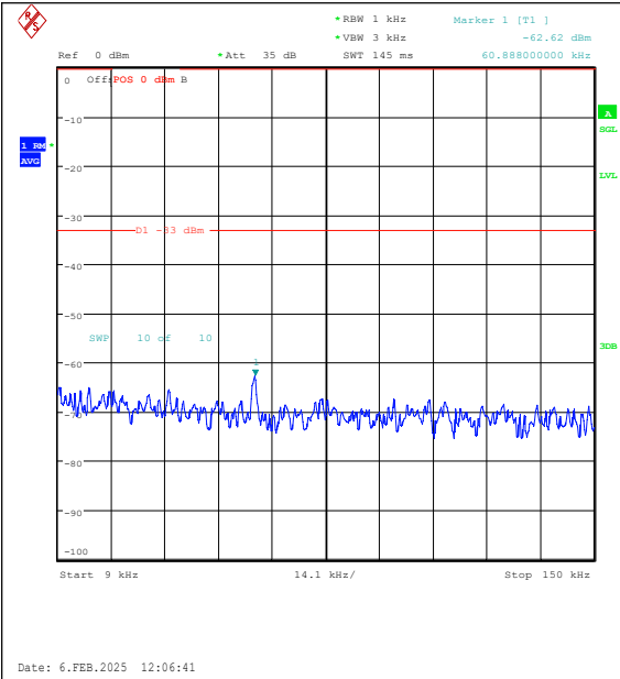
Band26(824-849)-10MHz-QPSK-26915-50RB#0-0 .009~0.15-PASS
