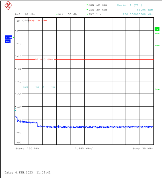
Band26(824-849)-10MHz-16QAM-26840-1RB#0-0 .15~30-PASS
