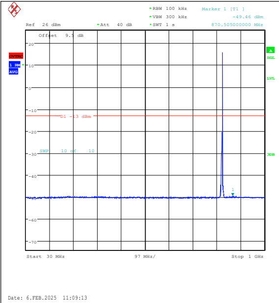
Band26(824-849)-5MHz-16QAM-26815-1RB#24-3 0~1000-PASS
