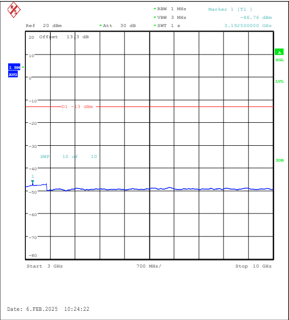
Band26(824-849)-3MHz-16QAM-26915-1RB#0-30 00~10000-PASS
