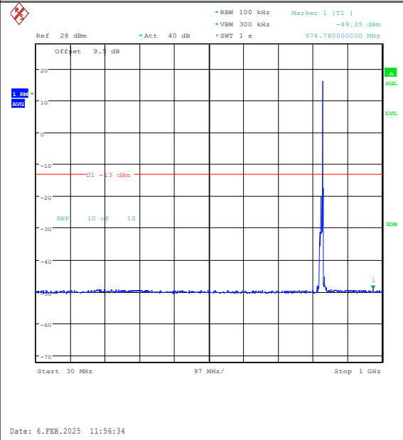
Band26(824-849)-10MHz-QPSK-26840-1RB#49-3 0~1000-PASS
