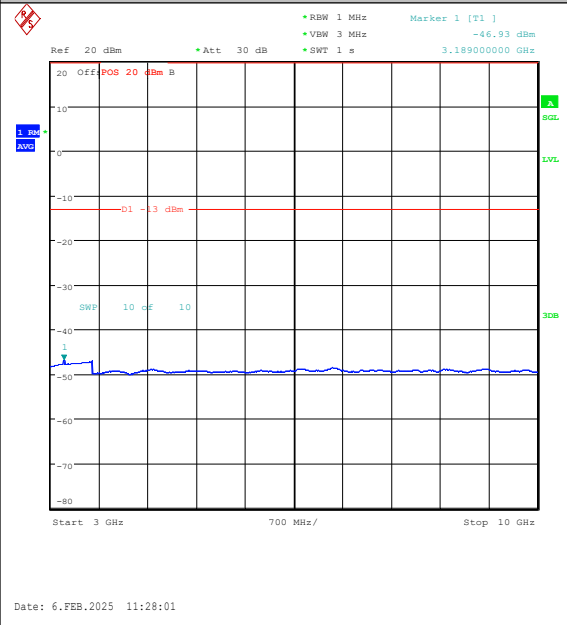
Band26(824-849)-5MHz-16QAM-27015-25RB#0-3 000~10000-PASS
