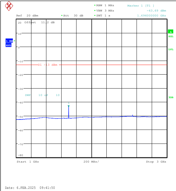
Band26(824-849)-1.4MHz-16QAM-27033-1RB#0- 1000~3000-PASS
