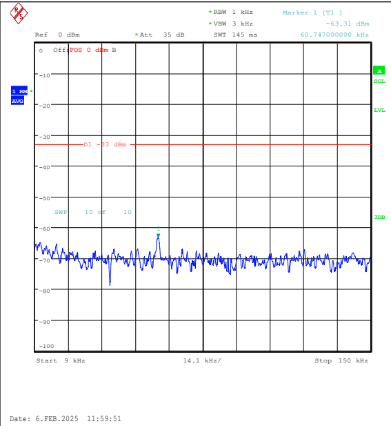
Band26(824-849)-10MHz-16QAM-26840-50RB#0-0.009~0.15-PASS
