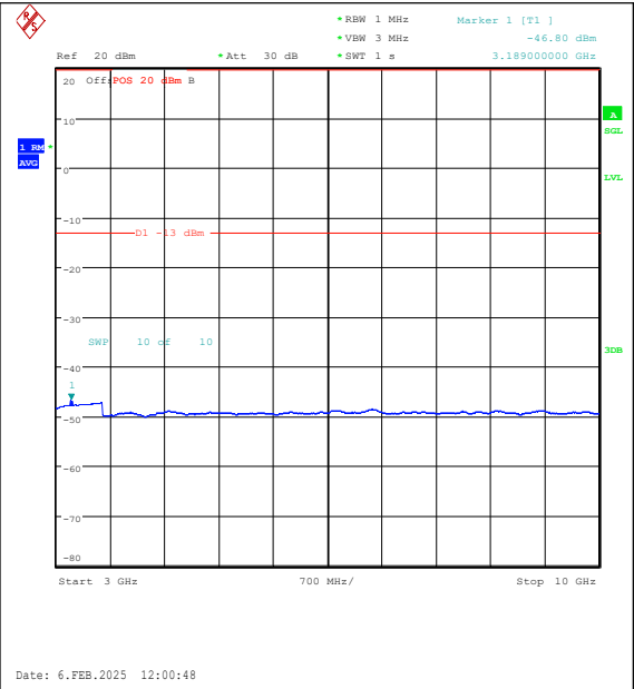
Band26(824-849)-10MHz-16QAM-26840-50RB#0-3000~10000-PASS
