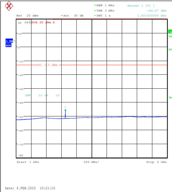
Band26(824-849)-3MHz-16QAM-26805-15RB#0-1 000~3000-PASS
