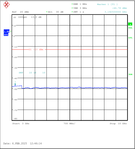
Band26(824-849)-15MHz-16QAM-26865-1RB#0-3 000~10000-PASS
