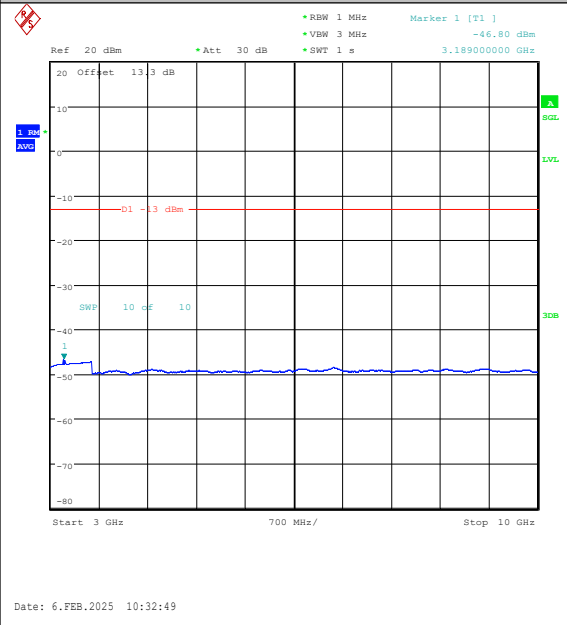
Band26(824-849)-3MHz-16QAM-27025-1RB#0-30 00~10000-PASS
