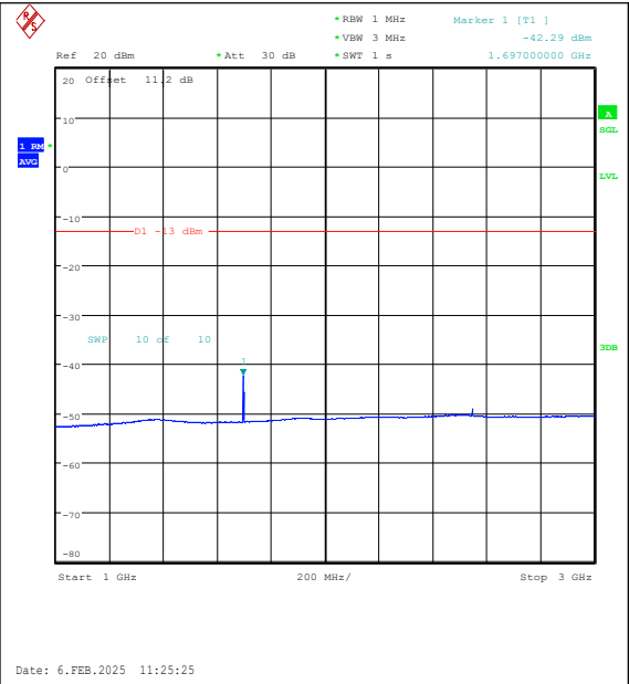
Band26(824-849)-5MHz-16QAM-27015-1RB#24-1 000~3000-PASS
