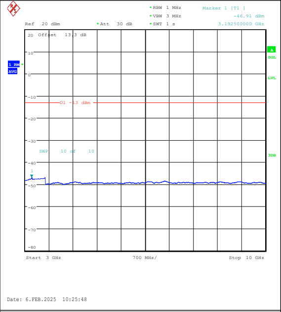
Band26(824-849)-3MHz-QPSK-26915-1RB#14-30 00~10000-PASS
