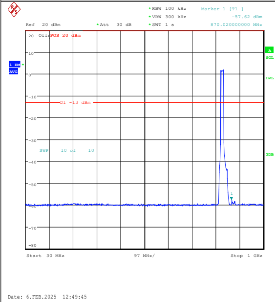
Band26(824-849)-15MHz-QPSK-26865-75RB#0-3 0~1000-PASS
