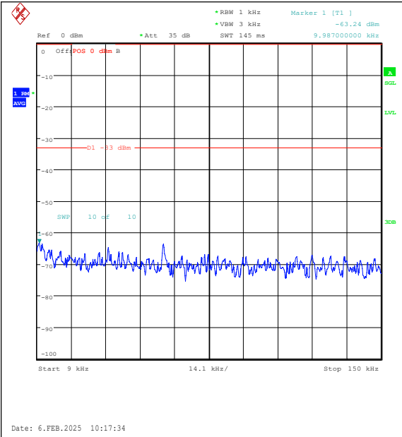
Band26(824-849)-3MHz-16QAM-26805-1RB#14-0 .009~0.15-PASS
