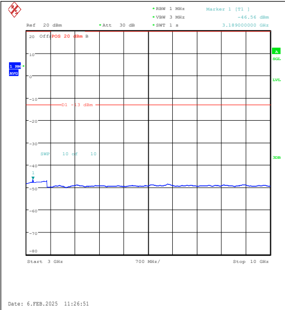
Band26(824-849)-5MHz-QPSK-27015-25RB#0-30 00~10000-PASS
