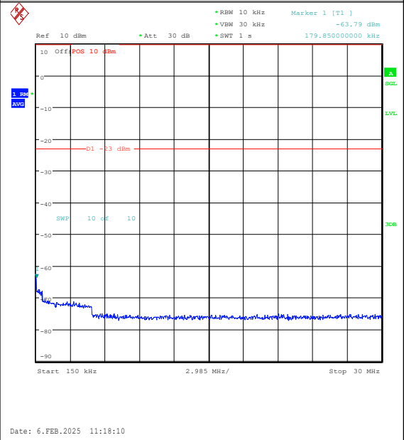
Band26(824-849)-5MHz-QPSK-26915-25RB#0-0. 15~30-PASS
