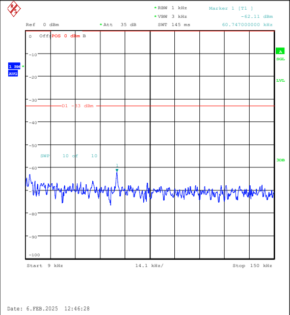
Band26(824-849)-15MHz-QPSK-26865-1RB#74-0 .009~0.15-PASS
