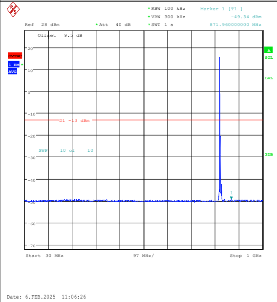
Band26(824-849)-5MHz-16QAM-26815-1RB#0-30 ~1000-PASS
