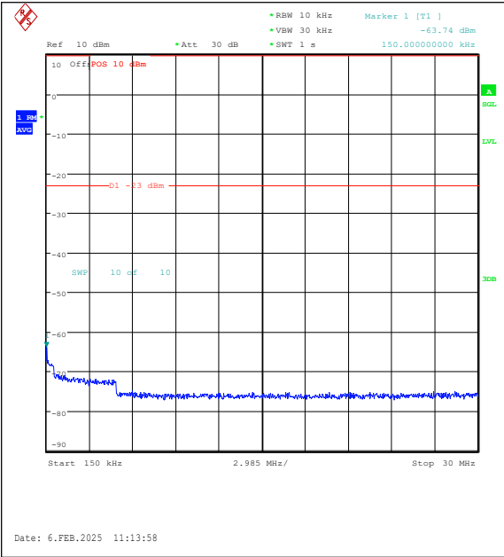
Band26(824-849)-5MHz-16QAM-26915-1RB#0-0. 15~30-PASS
