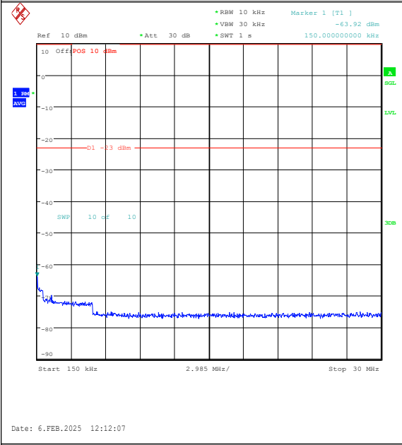
Band26(824-849)-10MHz-QPSK-26990-1RB#49-0 .15~30-PASS
