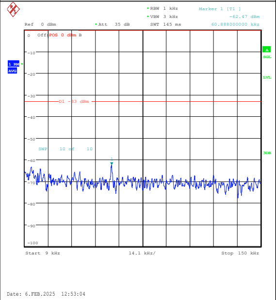
Band26(824-849)-15MHz-16QAM-26915-1RB#0-0 .009~0.15-PASS
