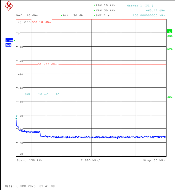
Band26(824-849)-1.4MHz-16QAM-27033-1RB#0- 0.15~30-PASS
