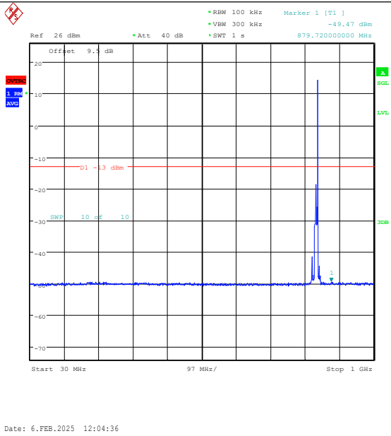
Band26(824-849)-10MHz-QPSK-26915-1RB#49-3 0~1000-PASS
