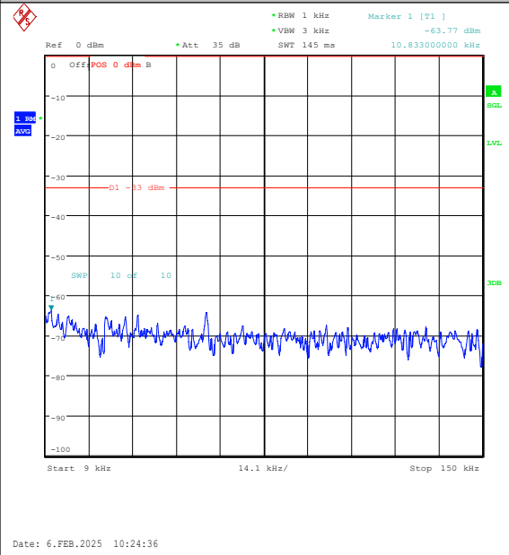
Band26(824-849)-3MHz-QPSK-26915-1RB#14-0.009~0.15-PASS
