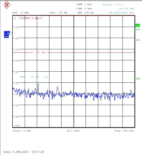
Band26(824-849)-1.4MHz-16QAM-26915-6RB#0-0.009~0.15-PASS
