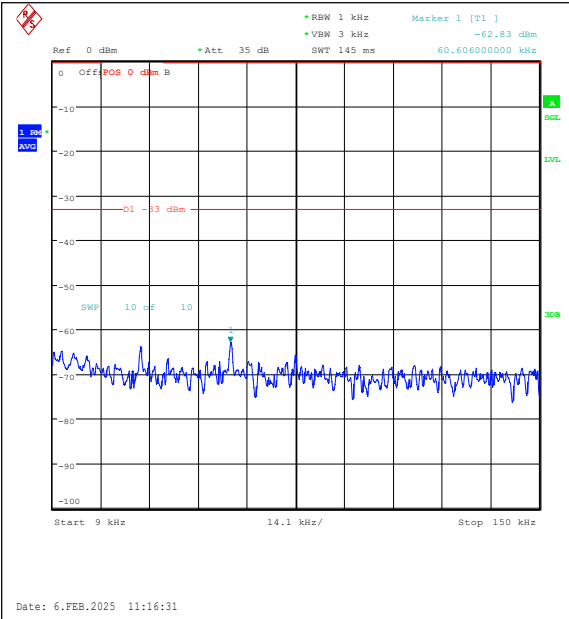
Band26(824-849)-5MHz-16QAM-26915-1RB#24-0 .009~0.15-PASS
