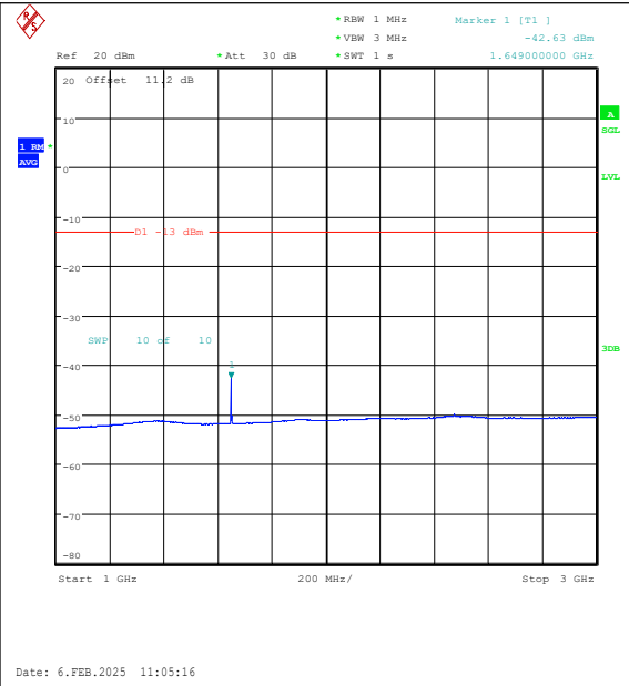
Band26(824-849)-5MHz-QPSK-26815-1RB#0-1000~3000-PASS
