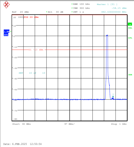
Band26(824-849)-15MHz-16QAM-26865-75RB#0-30~1000-PASS
