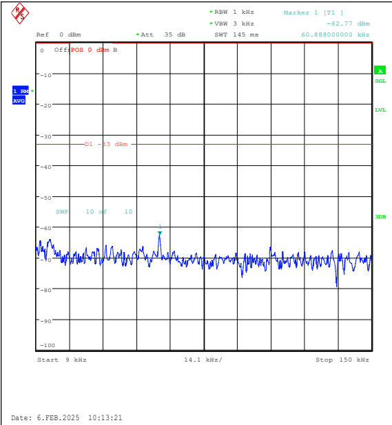
Band26(824-849)-3MHz-QPSK-26805-1RB#0-0.0 09~0.15-PASS
