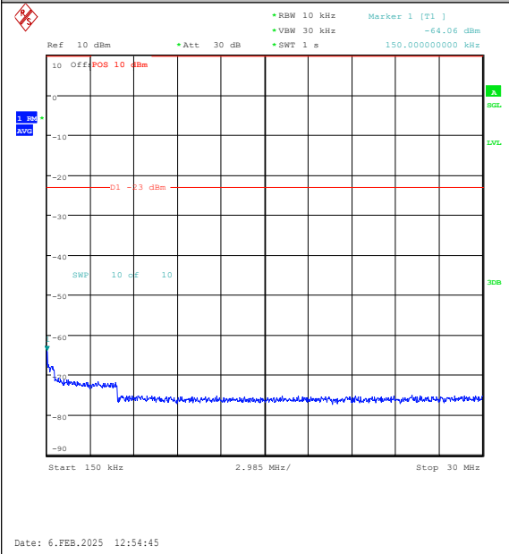
Band26(824-849)-15MHz-QPSK-26915-1RB#74-0 .15~30-PASS
