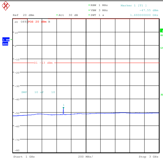
Band26(824-849)-5MHz-QPSK-27015-25RB#0-0. 15~30-PASS
