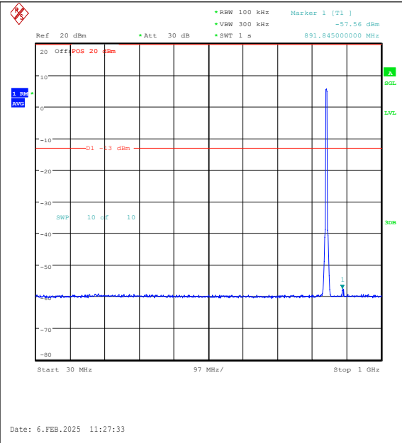
Band26(824-849)-5MHz-16QAM-27015-25RB#0-3 0~1000-PASS
