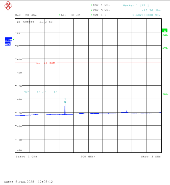
Band26(824-849)-10MHz-16QAM-26915-1RB#49-1000~3000-PASS
