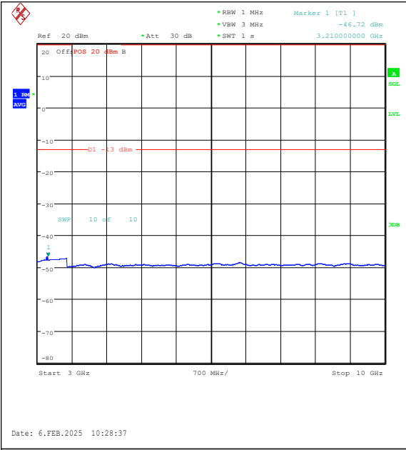
Band26(824-849)-3MHz-QPSK-26915-15RB#0-30 00~10000-PASS
