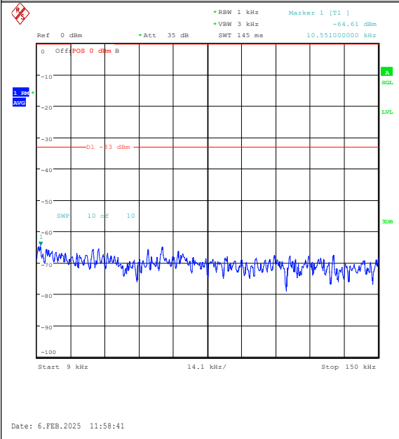
Band26(824-849)-10MHz-QPSK-26840-50RB#0-0 .009~0.15-PASS
