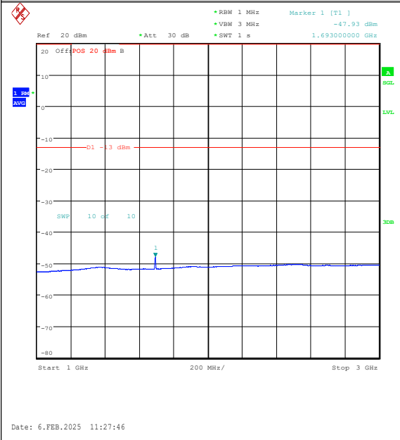
Band26(824-849)-5MHz-16QAM-27015-25RB#0-1 000~3000-PASS
