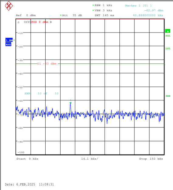
Band26(824-849)-5MHz-16QAM-26815-1RB#24-0 .009~0.15-PASS
