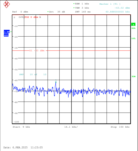
Band26(824-849)-5MHz-QPSK-27015-1RB#24-0.009~0.15-PASS
