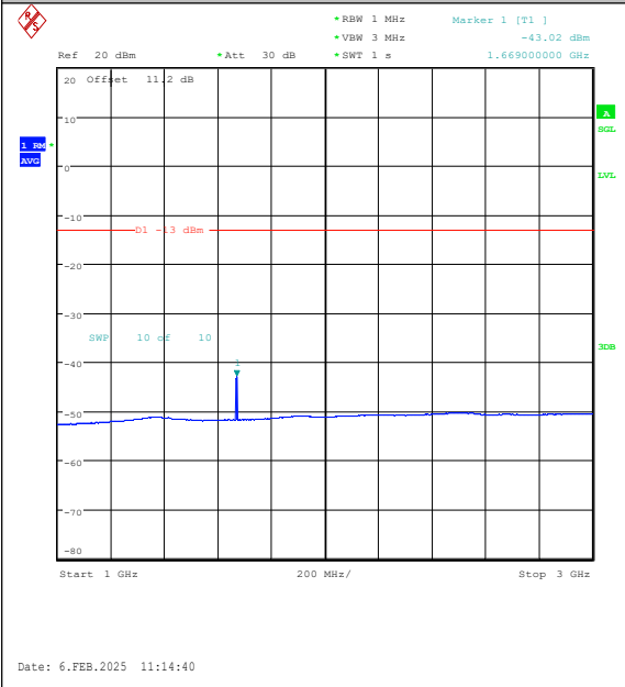
Band26(824-849)-5MHz-16QAM-26915-1RB#0-10 00~3000-PASS
