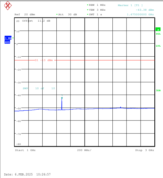
Band26(824-849)-3MHz-16QAM-26915-1RB#14-1 000~3000-PASS
