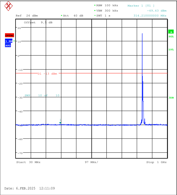
Band26(824-849)-10MHz-16QAM-26990-1RB#0-3 0~1000-PASS
