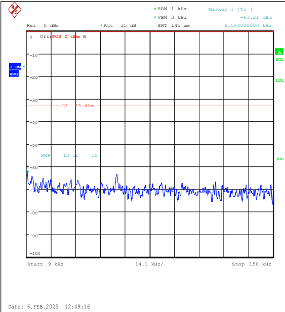
Band26(824-849)-15MHz-QPSK-26865-75RB#0-0 .009~0.15-PASS
