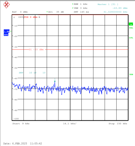
Band26(824-849)-5MHz-16QAM-26815-1RB#0-0. 009~0.15-PASS
