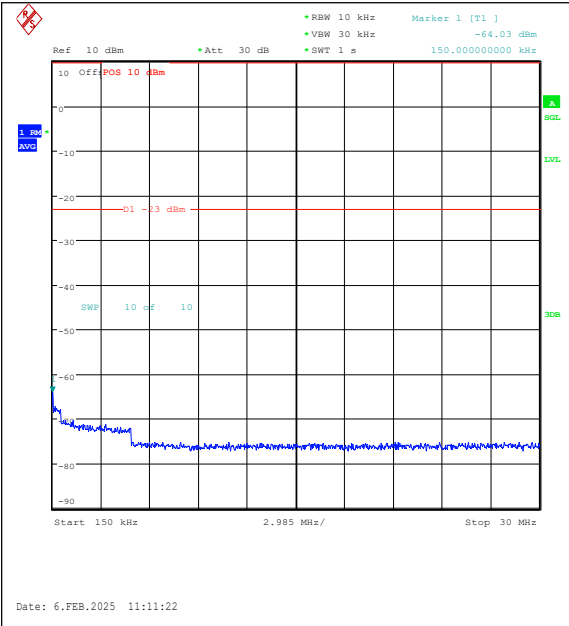
Band26(824-849)-5MHz-16QAM-26815-25RB#0-0 .15~30-PASS
