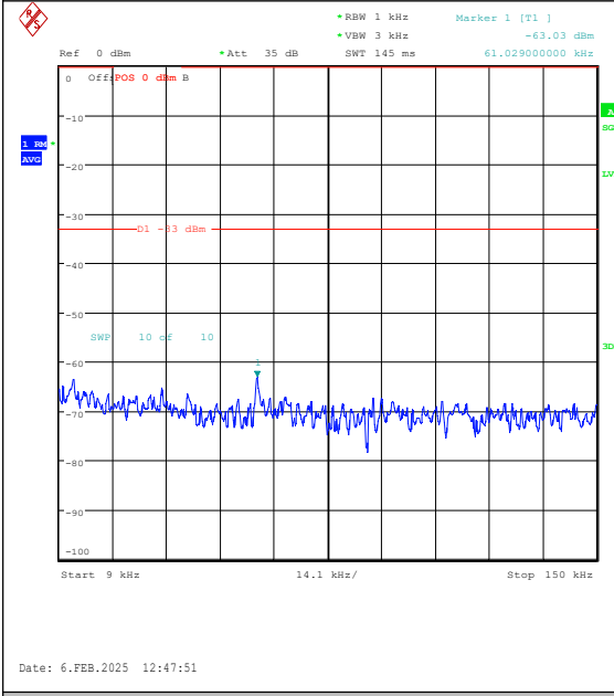
Band26(824-849)-15MHz-16QAM-26865-1RB#74- 0.009~0.15-PASS
