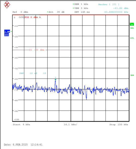
Band26(824-849)-10MHz-QPSK-26990-50RB#0-0 .009~0.15-PASS
