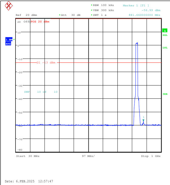
Band26(824-849)-15MHz-QPSK-26915-75RB#0-3 0~1000-PASS
