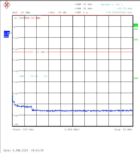
Band26(824-849)-1.4MHz-16QAM-27033-1RB#5- 0.15~30-PASS
