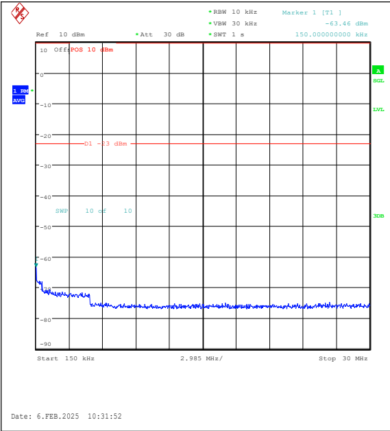
Band26(824-849)-3MHz-16QAM-27025-1RB#0-0. 15~30-PASS
