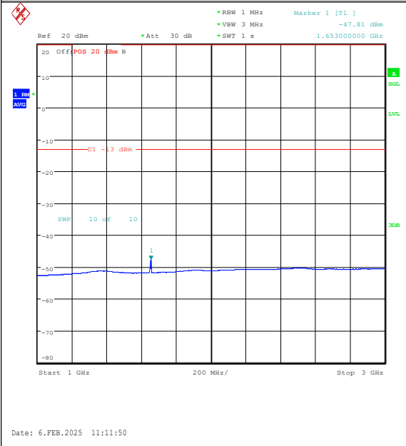
Band26(824-849)-5MHz-16QAM-26815-25RB#0-1 000~3000-PASS
