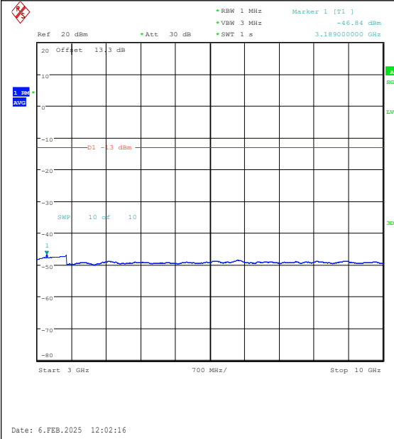
Band26(824-849)-10MHz-QPSK-26915-1RB#0-30 00~10000-PASS
