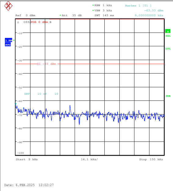
Band26(824-849)-10MHz-16QAM-26915-1RB#0-0 .009~0.15-PASS
