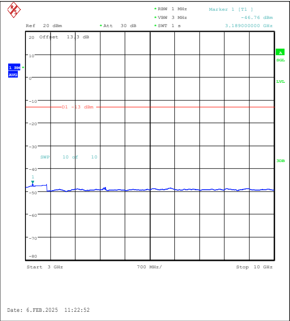
Band26(824-849)-5MHz-16QAM-27015-1RB#0-30 00~10000-PASS
