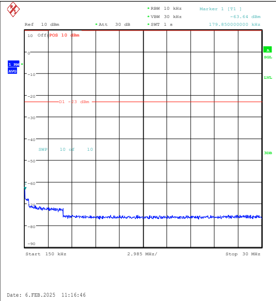
Band26(824-849)-5MHz-16QAM-26915-1RB#24-0 .15~30-PASS
