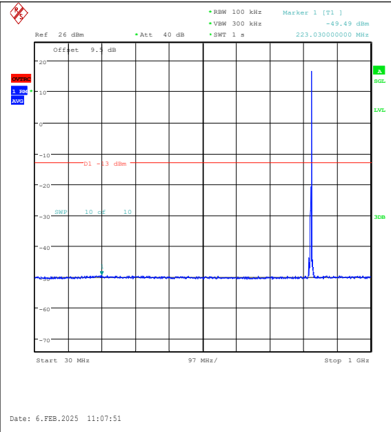
Band26(824-849)-5MHz-QPSK-26815-1RB#24-30 ~1000-PASS
