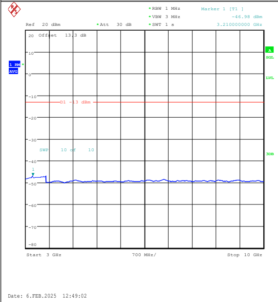
Band26(824-849)-15MHz-16QAM-26865-1RB#74-3000~10000-PASS
