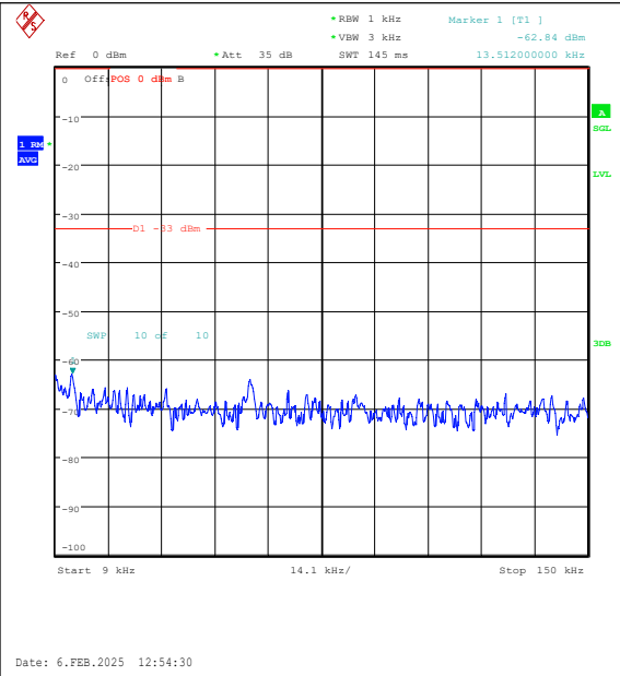
Band26(824-849)-15MHz-QPSK-26915-1RB#74-0 .009~0.15-PASS
