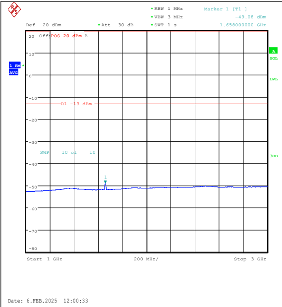
Band26(824-849)-10MHz-16QAM-26840-50RB#0-1000~3000-PASS
