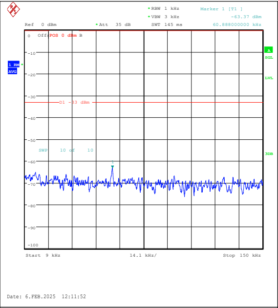
Band26(824-849)-10MHz-QPSK-26990-1RB#49-0 .009~0.15-PASS
