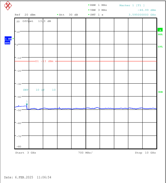
Band26(824-849)-5MHz-16QAM-26815-1RB#0-30 00~10000-PASS
