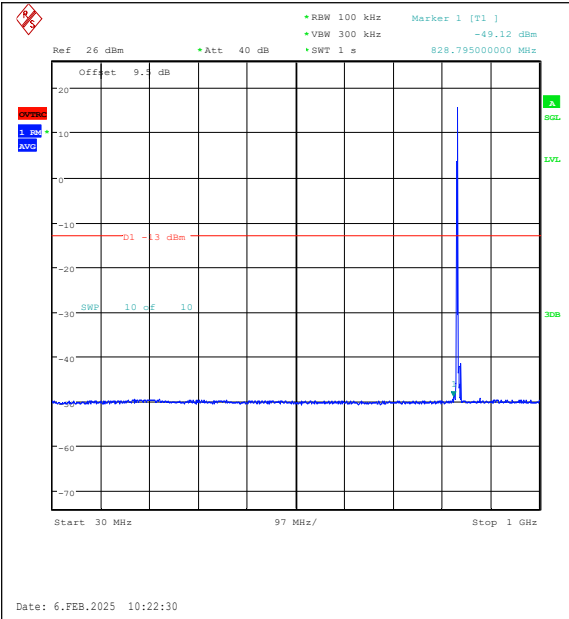
Band26(824-849)-3MHz-QPSK-26915-1RB#0-30~1000-PASS
