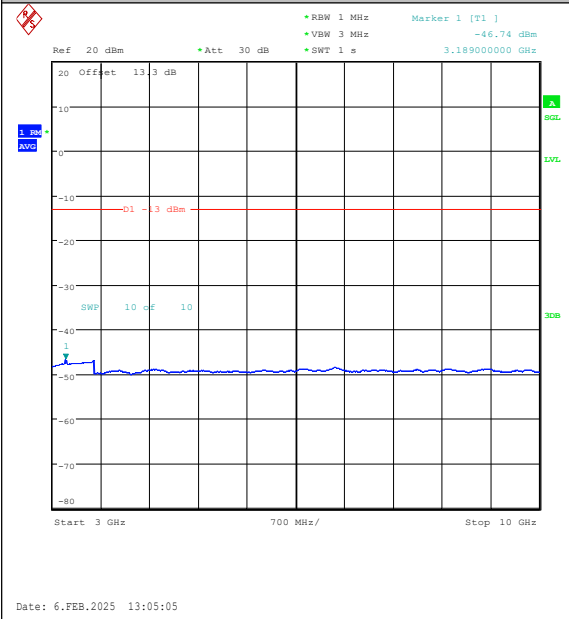
Band26(824-849)-15MHz-16QAM-26965-1RB#74- 3000~10000-PASS
