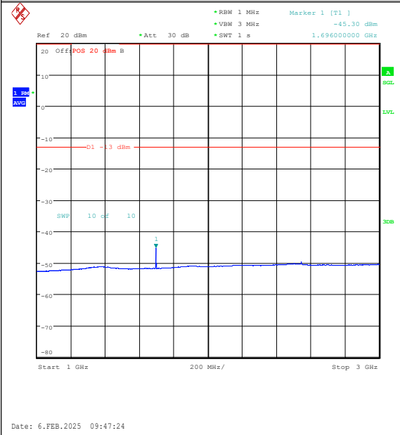
Band26(824-849)-1.4MHz-16QAM-27033-6RB#0-1000~3000-PASS
