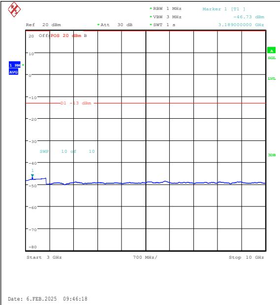
Band26(824-849)-1.4MHz-QPSK-27033-6RB#0-3 000~10000-PASS
