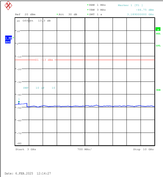
Band26(824-849)-10MHz-16QAM-26990-1RB#49-3000~10000-PASS
