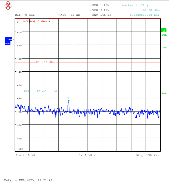
Band26(824-849)-5MHz-16QAM-27015-1RB#0-0. 009~0.15-PASS
