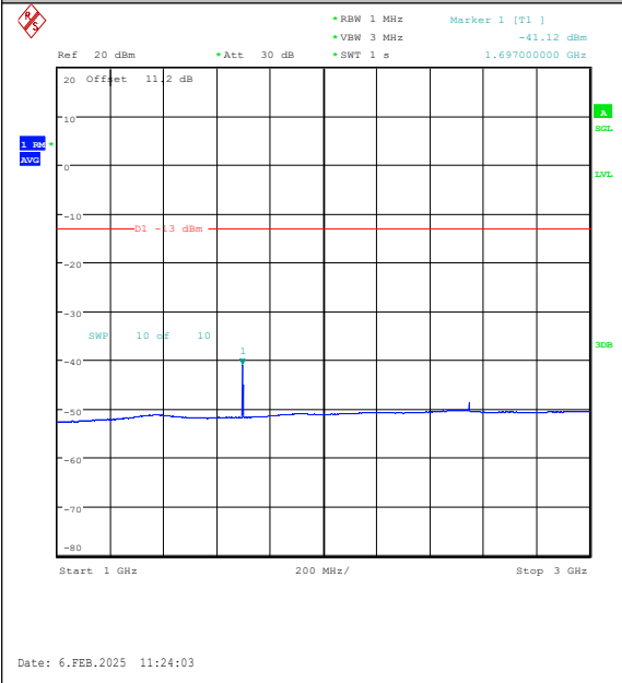
Band26(824-849)-5MHz-QPSK-27015-1RB#24-10 00~3000-PASS
