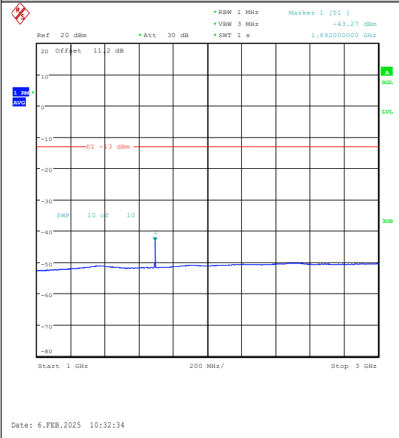
Band26(824-849)-3MHz-16QAM-27025-1RB#0-10 00~3000-PASS
