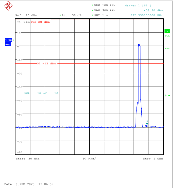
Band26(824-849)-15MHz-16QAM-26965-75RB#0-30~1000-PASS
