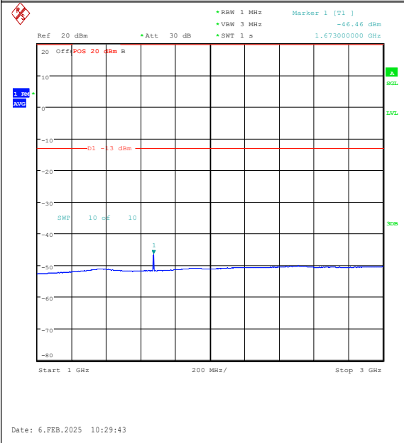
Band26(824-849)-3MHz-16QAM-26915-15RB#0-1 000~3000-PASS
