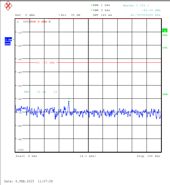
Band26(824-849)-5MHz-QPSK-26815-1RB#24-0.009~0.15-PASS
