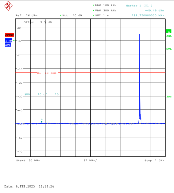
Band26(824-849)-5MHz-16QAM-26915-1RB#0-30 ~1000-PASS
