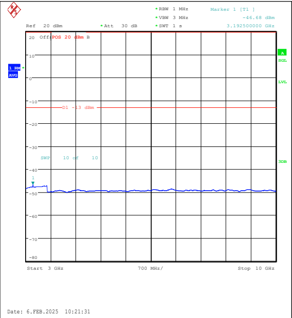
Band26(824-849)-3MHz-16QAM-26805-15RB#0-3 000~10000-PASS
