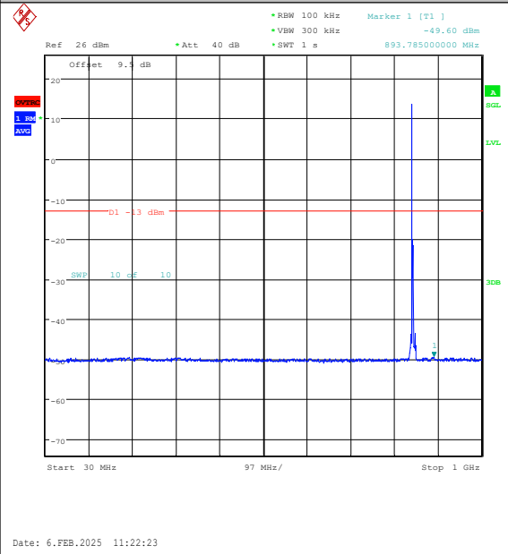
Band26(824-849)-5MHz-16QAM-27015-1RB#0-30 ~1000-PASS
