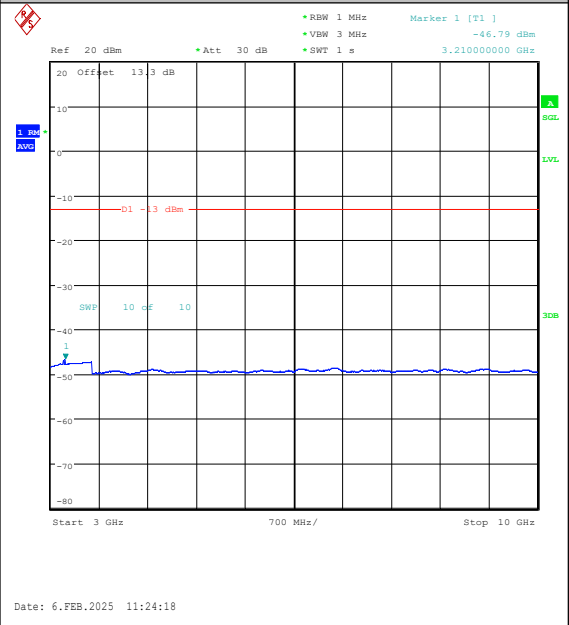
Band26(824-849)-5MHz-QPSK-27015-1RB#24-30 00~10000-PASS
