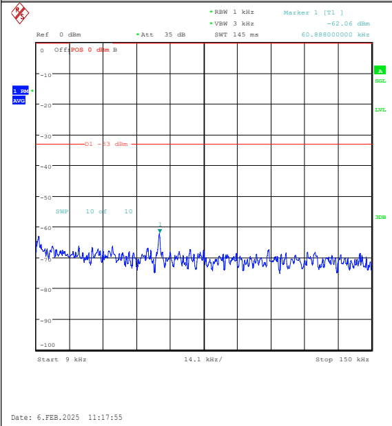
Band26(824-849)-5MHz-QPSK-26915-25RB#0-0. 009~0.15-PASS
