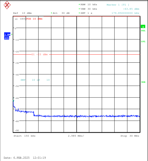
Band26(824-849)-10MHz-QPSK-26915-1RB#0-0.15~30-PASS
