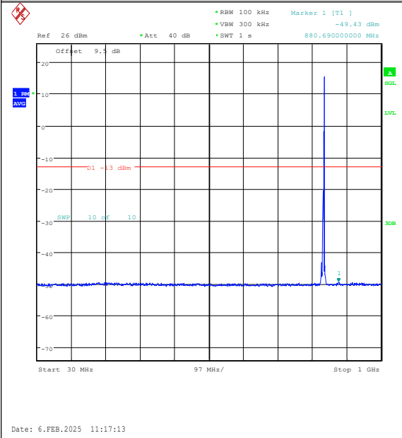
Band26(824-849)-5MHz-16QAM-26915-1RB#24-3 0~1000-PASS
