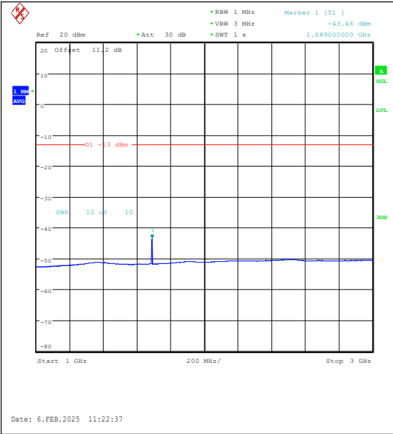
Band26(824-849)-5MHz-16QAM-27015-1RB#0-10 00~3000-PASS
