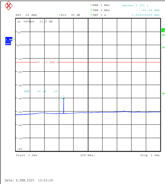
Band26(824-849)-10MHz-16QAM-26915-1RB#0-1 000~3000-PASS
