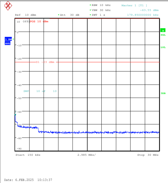
Band26(824-849)-3MHz-QPSK-26805-1RB#0-0.1 5~30-PASS
