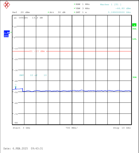
Band26(824-849)-1.4MHz-QPSK-27033-1RB#5-3 000~10000-PASS
