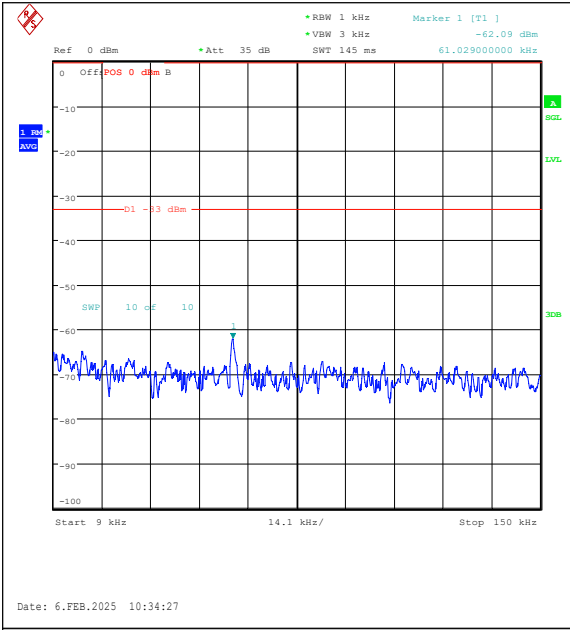
Band26(824-849)-3MHz-16QAM-27025-1RB#14-0 .009~0.15-PASS
