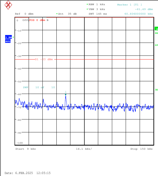
Band26(824-849)-10MHz-16QAM-26915-1RB#49- 0.009~0.15-PASS
