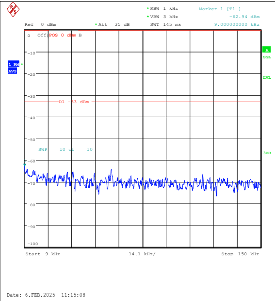
Band26(824-849)-5MHz-QPSK-26915-1RB#24-0. 009~0.15-PASS
