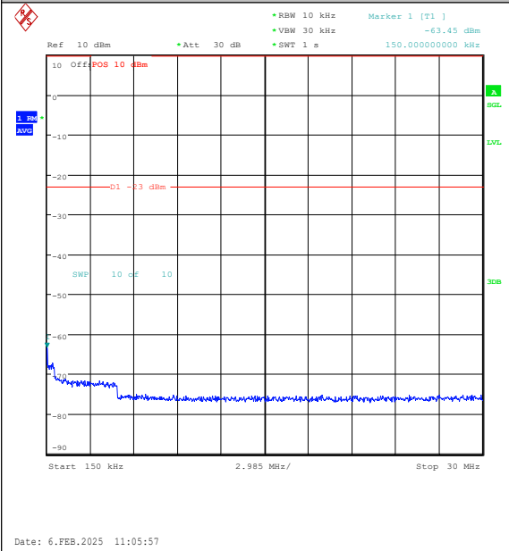
Band26(824-849)-5MHz-16QAM-26815-1RB#0-0. 15~30-PASS
