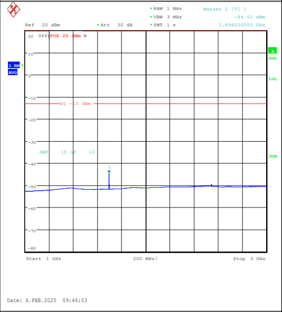
Band26(824-849)-1.4MHz-QPSK-27033-6RB#0-1 000~3000-PASS
