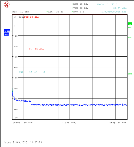
Band26(824-849)-5MHz-QPSK-26815-1RB#24-0. 15~30-PASS
