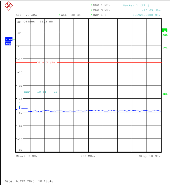
Band26(824-849)-3MHz-16QAM-26805-1RB#14-3 000~10000-PASS
