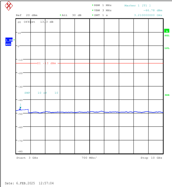
Band26(824-849)-15MHz-16QAM-26915-1RB#74-3000~10000-PASS
