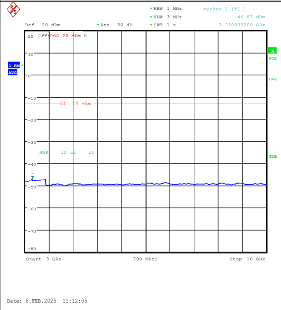
Band26(824-849)-5MHz-16QAM-26815-25RB#0-3 000~10000-PASS
