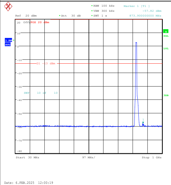
Band26(824-849)-10MHz-16QAM-26840-50RB#0-30~1000-PASS
