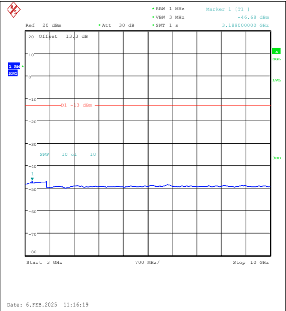
Band26(824-849)-5MHz-QPSK-26915-1RB#24-30 00~10000-PASS
