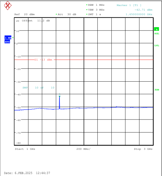
Band26(824-849)-15MHz-QPSK-26865-1RB#0-10 00~3000-PASS
