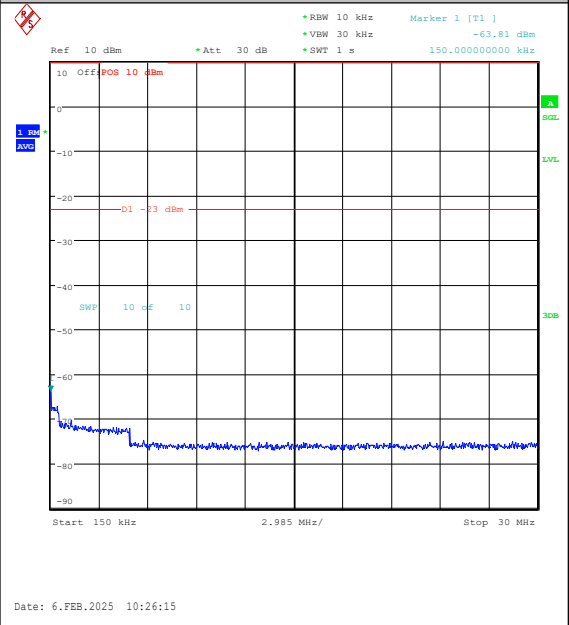
Band26(824-849)-3MHz-16QAM-26915-1RB#14-0 .15~30-PASS
