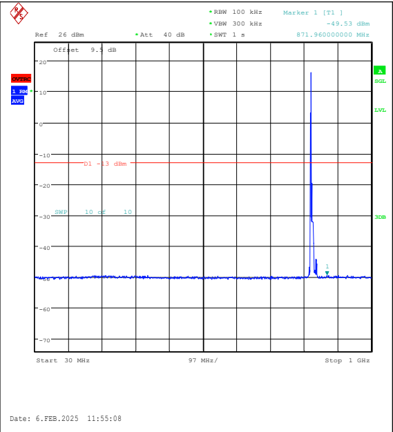
Band26(824-849)-10MHz-16QAM-26840-1RB#0-3 0~1000-PASS
