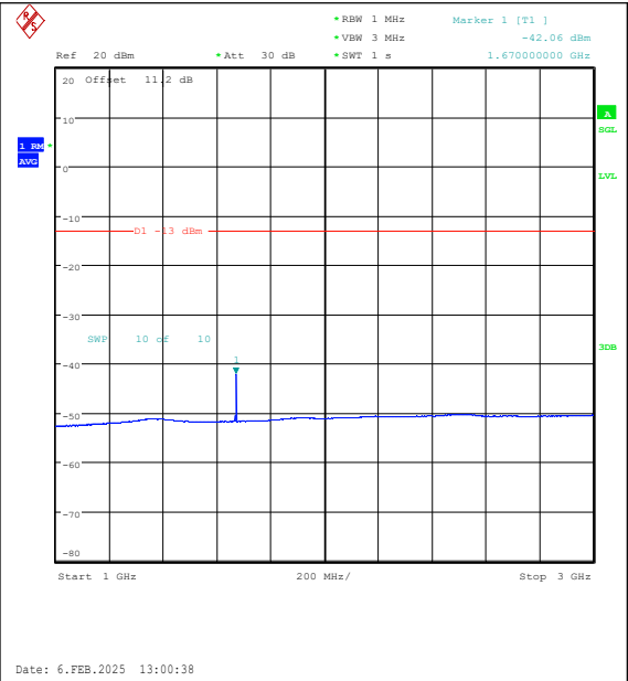
Band26(824-849)-15MHz-QPSK-26965-1RB#0-10 00~3000-PASS
