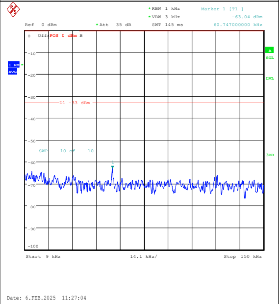
Band26(824-849)-5MHz-16QAM-27015-25RB#0-0 .009~0.15-PASS
