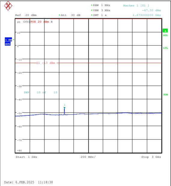
Band26(824-849)-5MHz-QPSK-26915-25RB#0-10 00~3000-PASS
