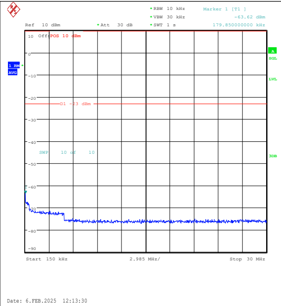
Band26(824-849)-10MHz-16QAM-26990-1RB#49- 0.15~30-PASS
