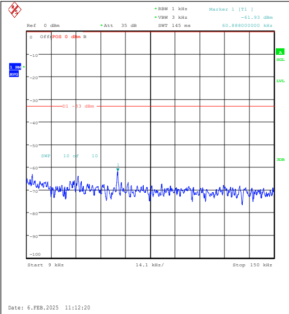
Band26(824-849)-5MHz-QPSK-26915-1RB#0-0.0 09~0.15-PASS
