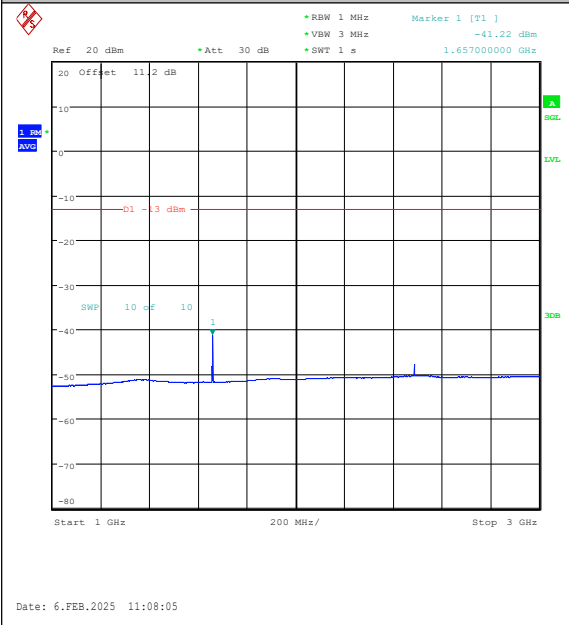
Band26(824-849)-5MHz-QPSK-26815-1RB#24-10 00~3000-PASS
