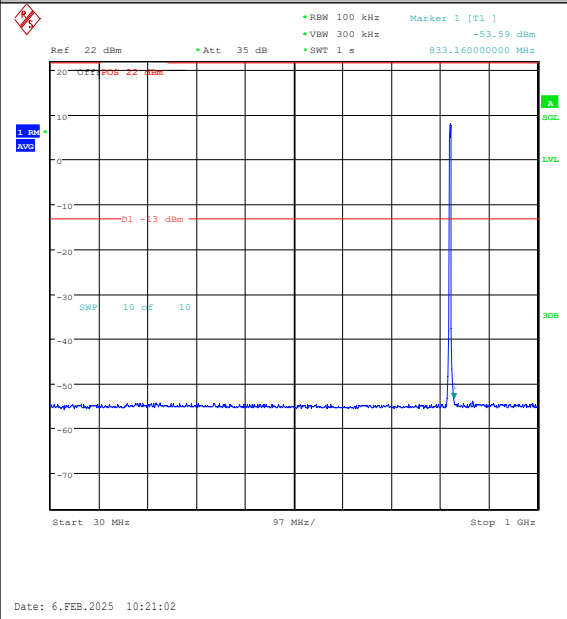
Band26(824-849)-3MHz-16QAM-26805-15RB#0-3 0~1000-PASS
