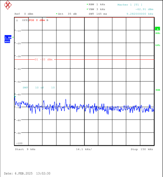
Band26(824-849)-15MHz-QPSK-26965-1RB#74-0 .009~0.15-PASS
