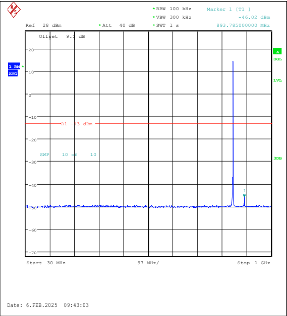
Band26(824-849)-1.4MHz-QPSK-27033-1RB#5-3 0~1000-PASS
