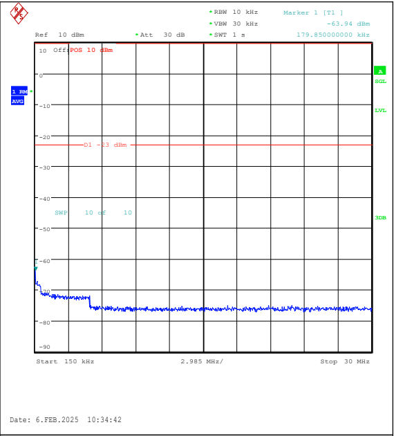
Band26(824-849)-3MHz-16QAM-27025-1RB#14-0 .15~30-PASS
