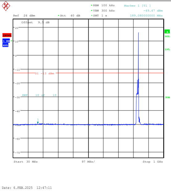
Band26(824-849)-15MHz-QPSK-26865-1RB#74-3 0~1000-PASS
