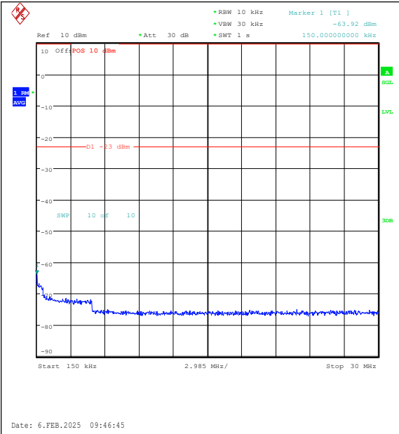
Band26(824-849)-1.4MHz-16QAM-27033-6RB#0-0.15~30-PASS
