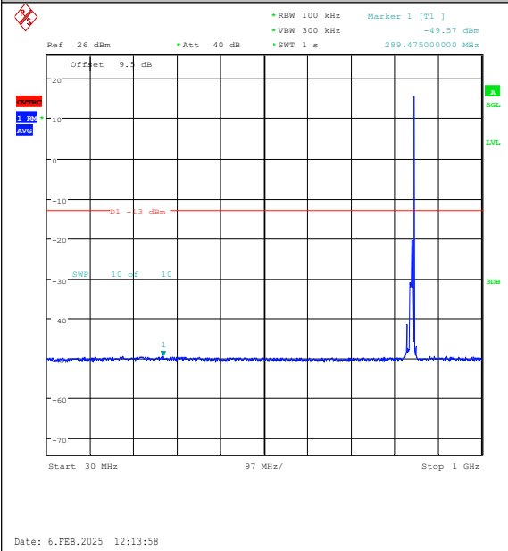
Band26(824-849)-10MHz-16QAM-26990-1RB#49- 30~1000-PASS
