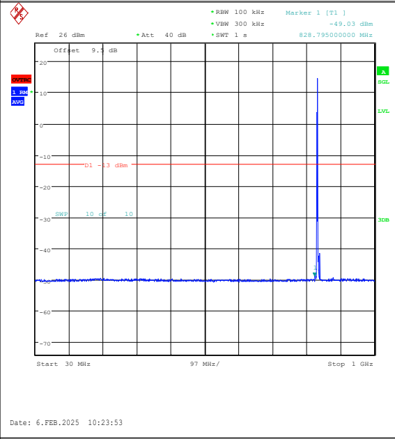
Band26(824-849)-3MHz-16QAM-26915-1RB#0-30 ~1000-PASS
