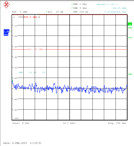
Band26(824-849)-10MHz-QPSK-26840-1RB#49-0 .009~0.15-PASS
