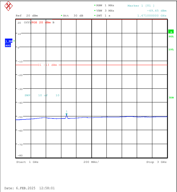
Band26(824-849)-15MHz-QPSK-26915-75RB#0-1 000~3000-PASS
