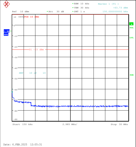
Band26(824-849)-10MHz-16QAM-26915-1RB#49- 0.15~30-PASS
