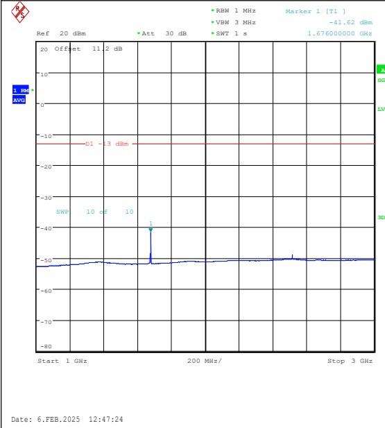
Band26(824-849)-15MHz-QPSK-26865-1RB#74-1 000~3000-PASS
