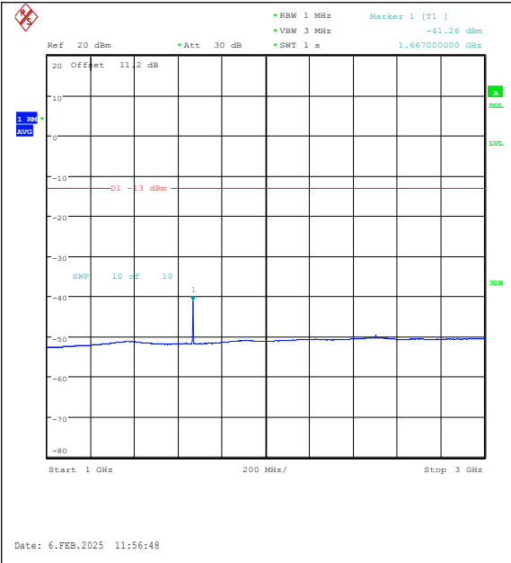
Band26(824-849)-10MHz-QPSK-26840-1RB#49-1 000~3000-PASS
