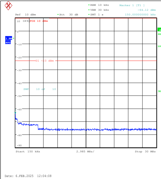
Band26(824-849)-10MHz-QPSK-26915-1RB#49-0 .15~30-PASS
