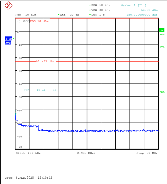
Band26(824-849)-10MHz-16QAM-26990-1RB#0-0 .15~30-PASS
