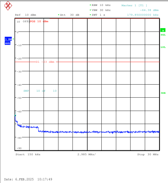
Band26(824-849)-3MHz-16QAM-26805-1RB#14-0 .15~30-PASS
