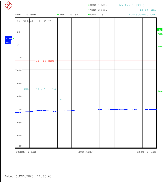
Band26(824-849)-5MHz-16QAM-26815-1RB#0-10 00~3000-PASS
