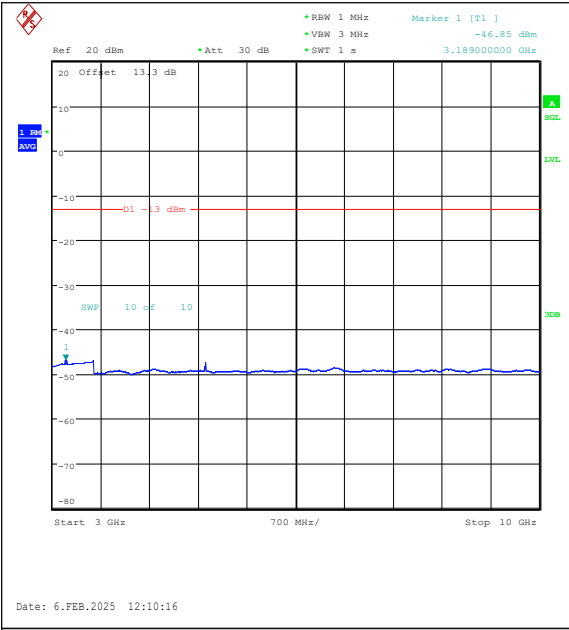
Band26(824-849)-10MHz-QPSK-26990-1RB#0-30 00~10000-PASS
