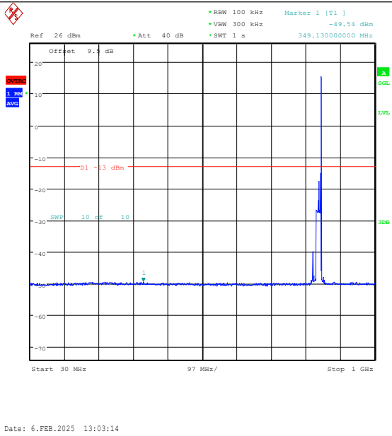
Band26(824-849)-15MHz-QPSK-26965-1RB#74-3 0~1000-PASS
