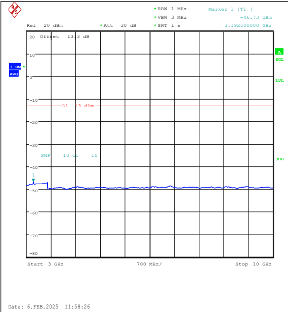
Band26(824-849)-10MHz-16QAM-26840-1RB#49-3000~10000-PASS
