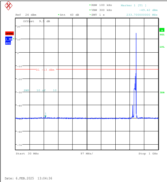
Band26(824-849)-15MHz-16QAM-26965-1RB#74- 30~1000-PASS
