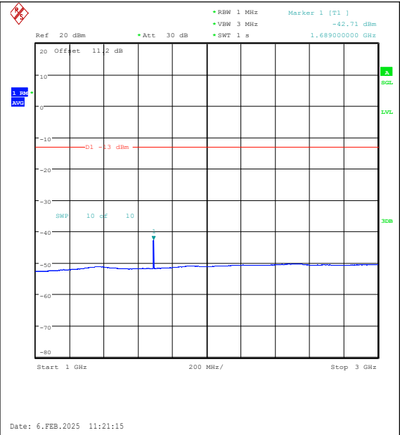
Band26(824-849)-5MHz-QPSK-27015-1RB#0-1000~3000-PASS
