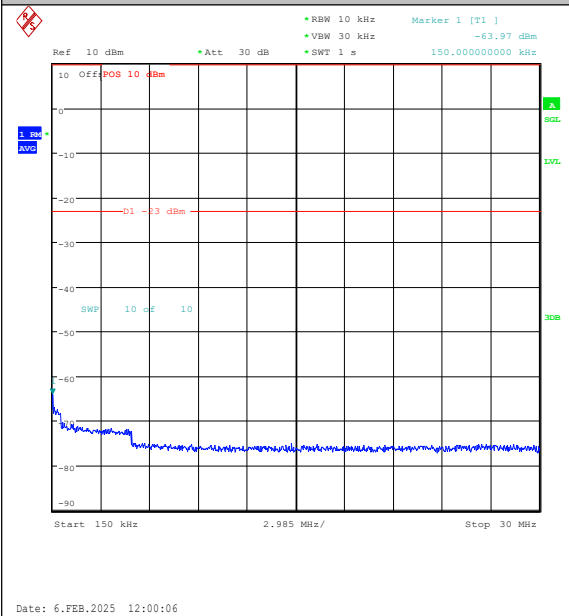
Band26(824-849)-10MHz-16QAM-26840-50RB#0-0.15~30-PASS
