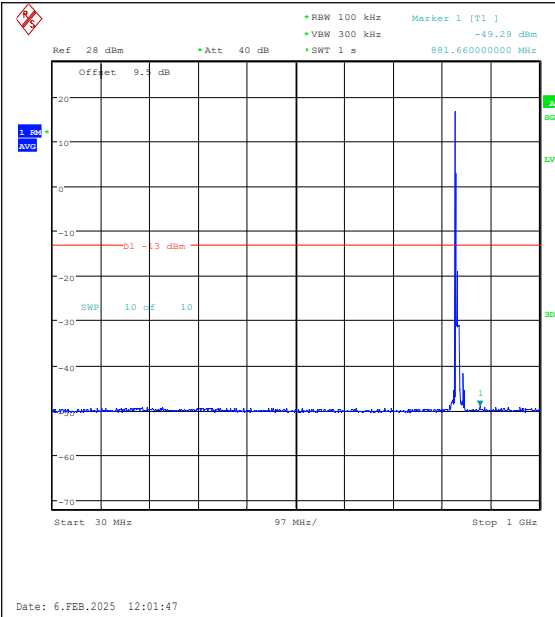
Band26(824-849)-10MHz-QPSK-26915-1RB#0-30 ~1000-PASS
