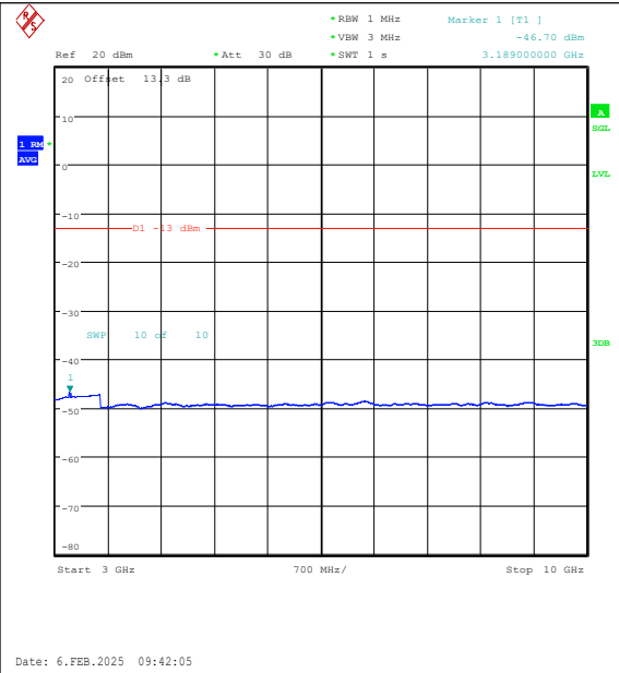
Band26(824-849)-1.4MHz-16QAM-27033-1RB#0- 3000~10000-PASS
