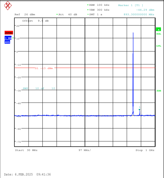
Band26(824-849)-1.4MHz-16QAM-27033-1RB#0- 30~1000-PASS
