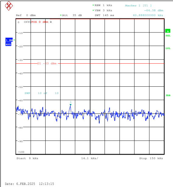
Band26(824-849)-10MHz-16QAM-26990-1RB#49- 0.009~0.15-PASS
