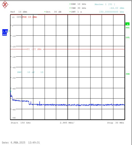
Band26(824-849)-15MHz-QPSK-26865-75RB#0-0 .15~30-PASS
