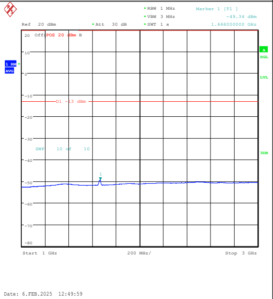
Band26(824-849)-15MHz-QPSK-26865-75RB#0-1 000~3000-PASS
