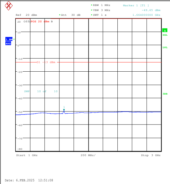
Band26(824-849)-15MHz-16QAM-26865-75RB#0-1000~3000-PASS
