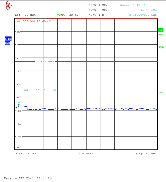
Band26(824-849)-15MHz-16QAM-26865-75RB#0-3000~10000-PASS
