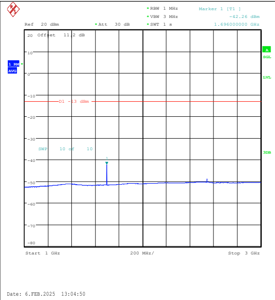
Band26(824-849)-15MHz-16QAM-26965-1RB#74- 1000~3000-PASS
