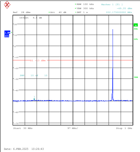
Band26(824-849)-3MHz-16QAM-26915-1RB#14-3 0~1000-PASS
