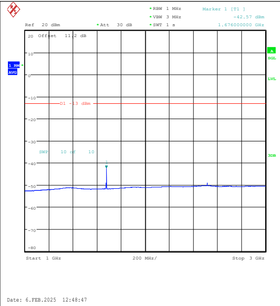
Band26(824-849)-15MHz-16QAM-26865-1RB#74-1000~3000-PASS
