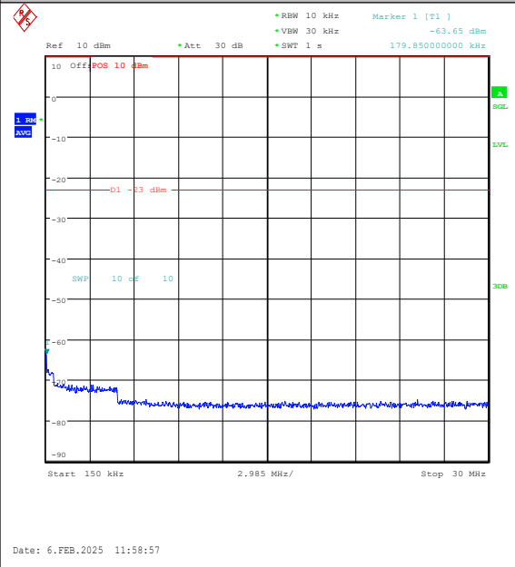
Band26(824-849)-10MHz-QPSK-26840-50RB#0-0 .15~30-PASS
