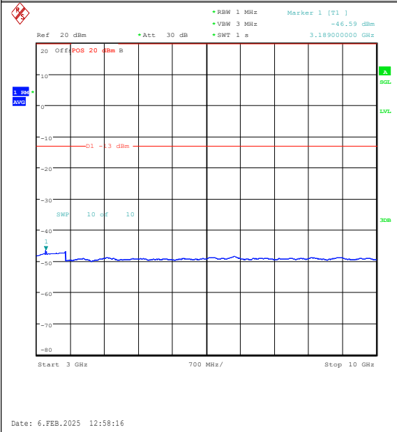
Band26(824-849)-15MHz-QPSK-26915-75RB#0-3 000~10000-PASS
