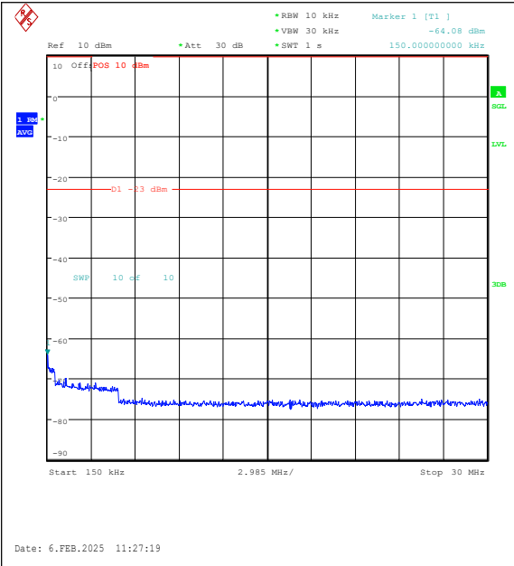
Band26(824-849)-5MHz-16QAM-27015-25RB#0-0 .15~30-PASS
