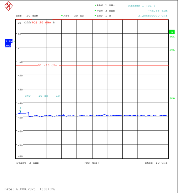
Band26(824-849)-15MHz-16QAM-26965-75RB#0-3000~10000-PASS
