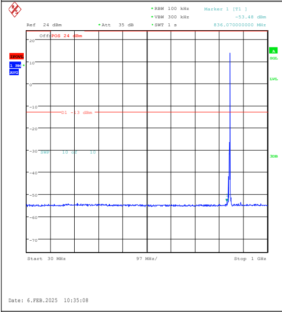
Band26(824-849)-3MHz-16QAM-27025-1RB#14-3 0~1000-PASS
