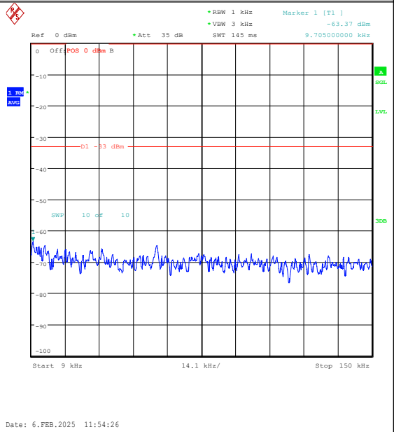
Band26(824-849)-10MHz-16QAM-26840-1RB#0-0 .009~0.15-PASS
