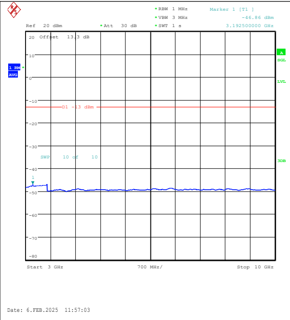
Band26(824-849)-10MHz-QPSK-26840-1RB#49-3 000~10000-PASS
