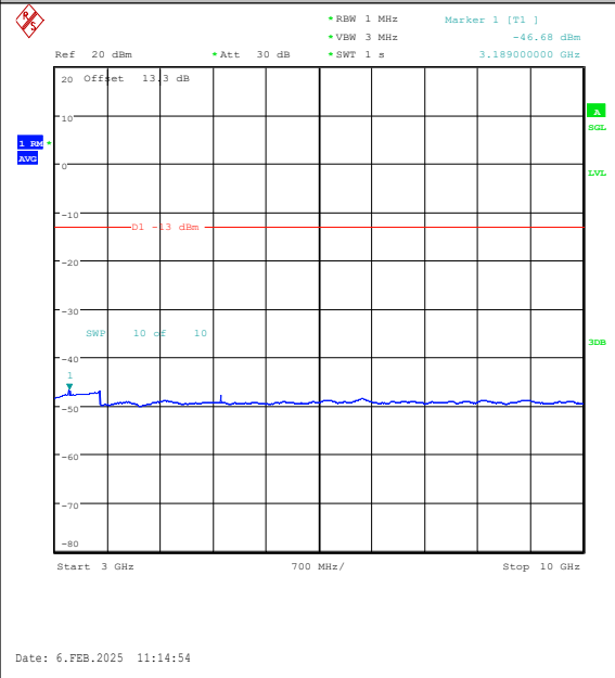
Band26(824-849)-5MHz-16QAM-26915-1RB#0-30 00~10000-PASS
