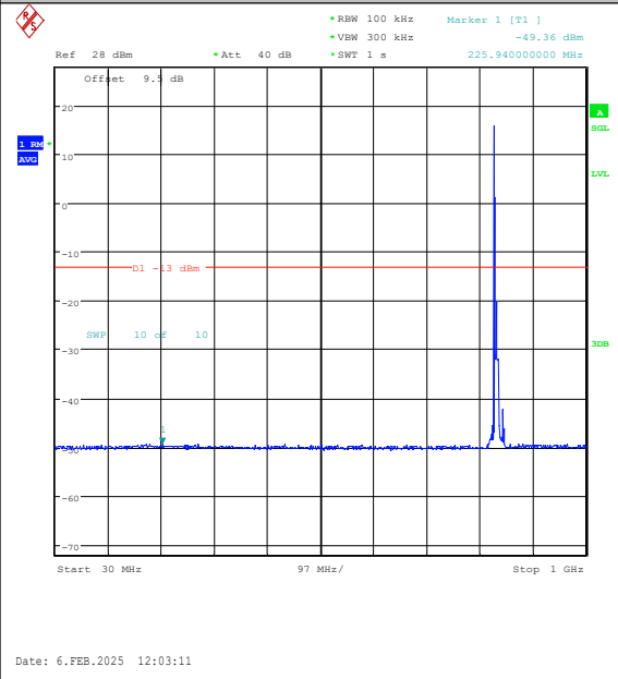
Band26(824-849)-10MHz-16QAM-26915-1RB#0-3 0~1000-PASS
