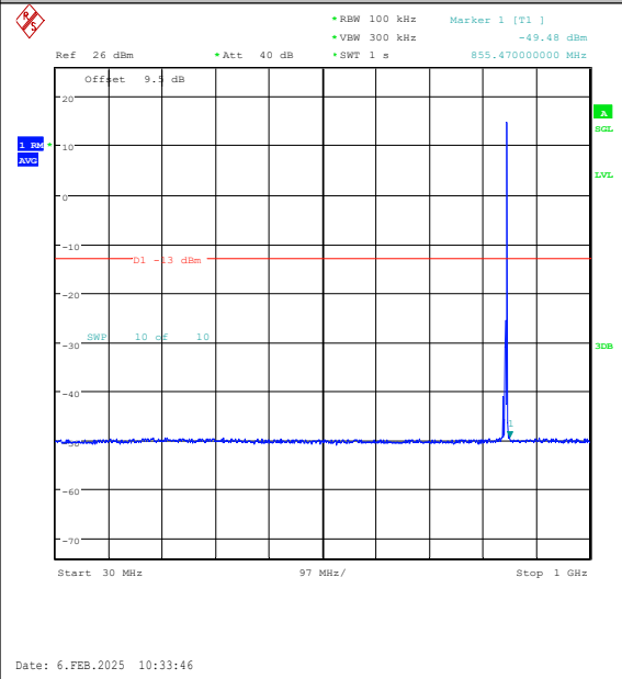
Band26(824-849)-3MHz-QPSK-27025-1RB#14-30 ~1000-PASS
