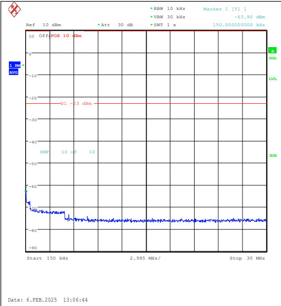
Band26(824-849)-15MHz-16QAM-26965-75RB#0-0.15~30-PASS
