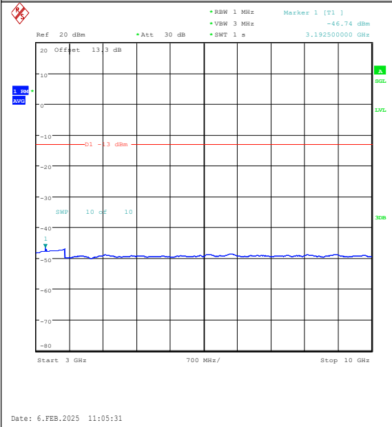
Band26(824-849)-5MHz-QPSK-26815-1RB#0-3000~10000-PASS
