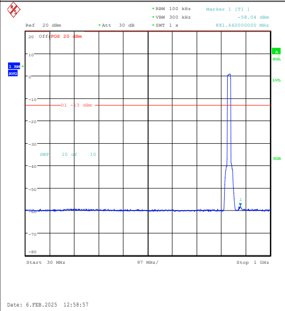
Band26(824-849)-15MHz-16QAM-26915-75RB#0-30~1000-PASS
