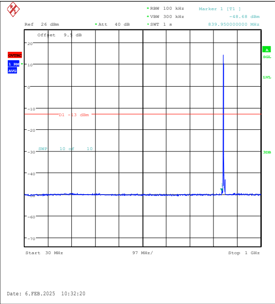
Band26(824-849)-3MHz-16QAM-27025-1RB#0-30 ~1000-PASS
