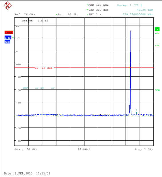
Band26(824-849)-5MHz-QPSK-26915-1RB#24-30 ~1000-PASS
