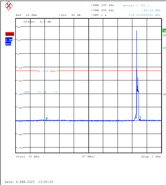
Band26(824-849)-15MHz-QPSK-26965-1RB#0-30 ~1000-PASS
