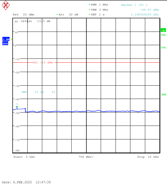
Band26(824-849)-15MHz-QPSK-26865-1RB#74-3 000~10000-PASS
