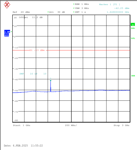
Band26(824-849)-10MHz-16QAM-26840-1RB#0-1 000~3000-PASS
