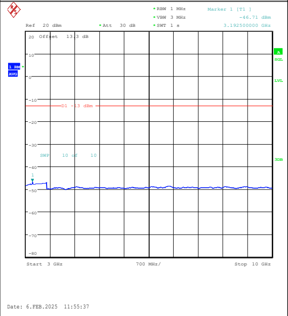
Band26(824-849)-10MHz-16QAM-26840-1RB#0-3 000~10000-PASS
