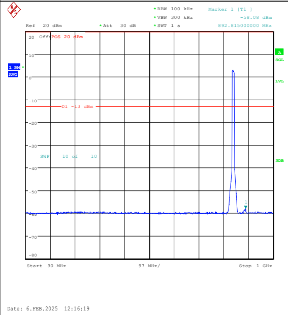
Band26(824-849)-10MHz-16QAM-26990-50RB#0-30~1000-PASS
