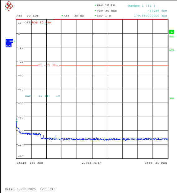
Band26(824-849)-15MHz-16QAM-26915-75RB#0-0.15~30-PASS
