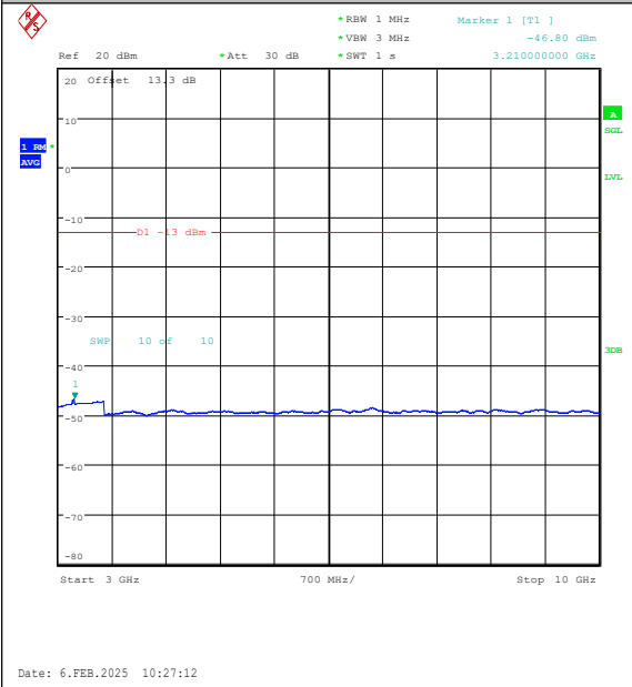
Band26(824-849)-3MHz-16QAM-26915-1RB#14-3 000~10000-PASS
