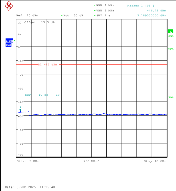
Band26(824-849)-5MHz-16QAM-27015-1RB#24-3 000~10000-PASS
