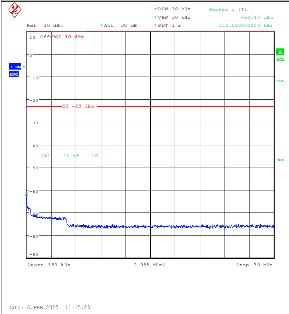
Band26(824-849)-5MHz-QPSK-26915-1RB#24-0. 15~30-PASS
