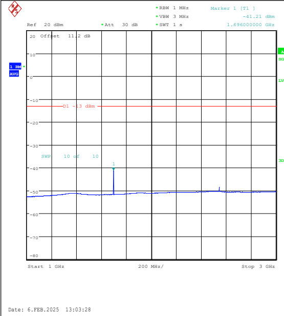
Band26(824-849)-15MHz-QPSK-26965-1RB#74-1 000~3000-PASS
