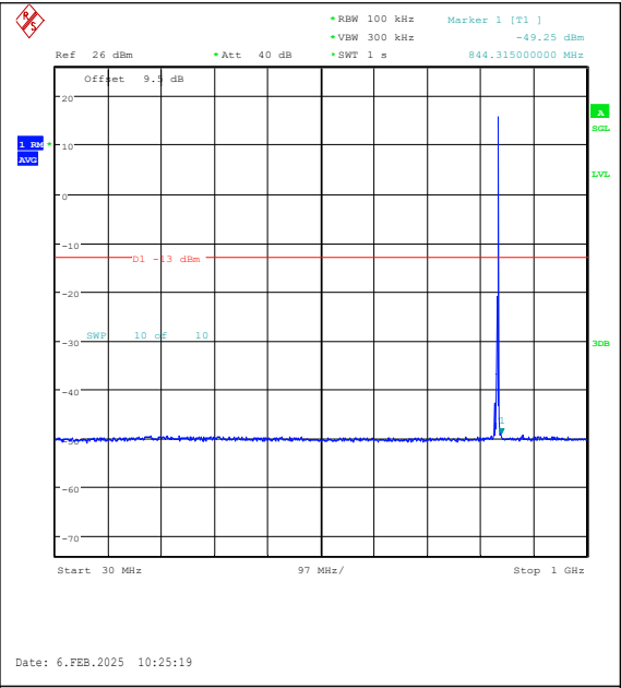
Band26(824-849)-3MHz-QPSK-26915-1RB#14-30 ~1000-PASS
