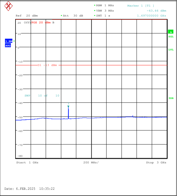
Band26(824-849)-3MHz-16QAM-27025-1RB#14-1 000~3000-PASS
