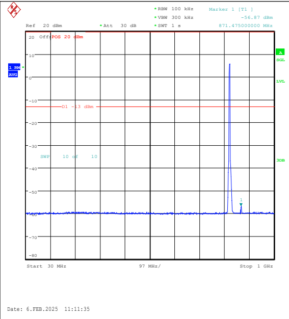
Band26(824-849)-5MHz-16QAM-26815-25RB#0-3 0~1000-PASS
