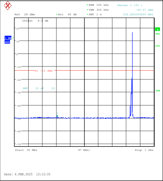
Band26(824-849)-10MHz-QPSK-26990-1RB#49-3 0~1000-PASS
