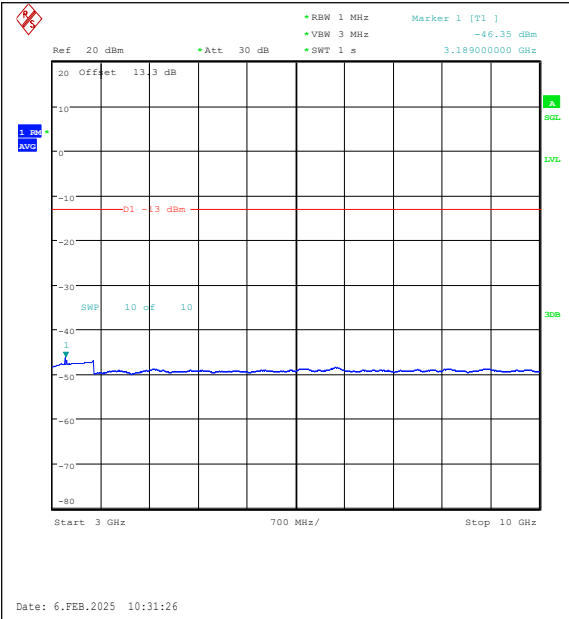
Band26(824-849)-3MHz-QPSK-27025-1RB#0-300 0~10000-PASS
