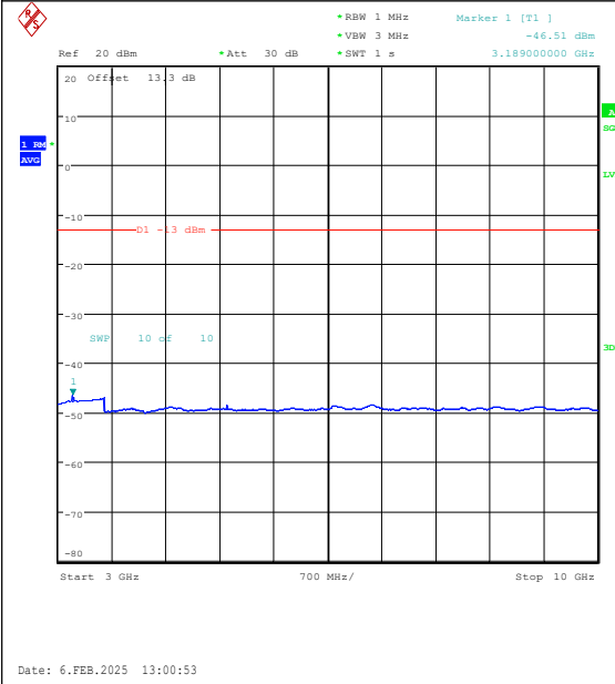
Band26(824-849)-15MHz-QPSK-26965-1RB#0-30 00~10000-PASS
