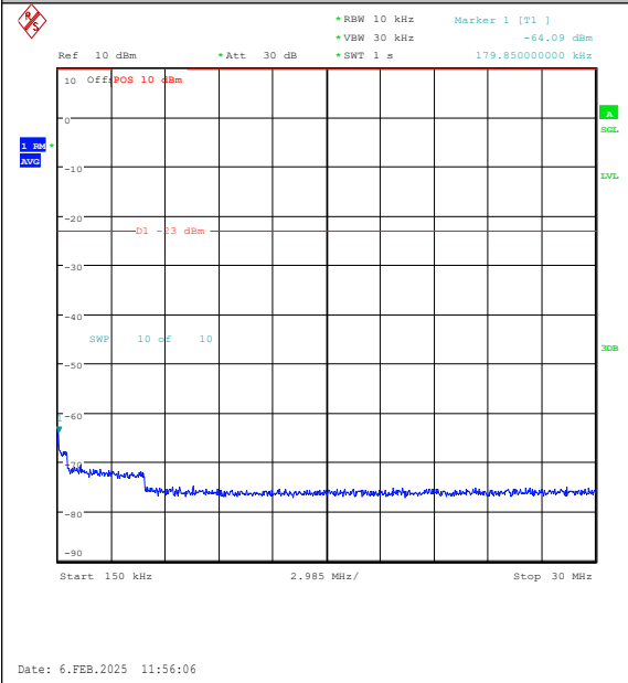
Band26(824-849)-10MHz-QPSK-26840-1RB#49-0 .15~30-PASS
