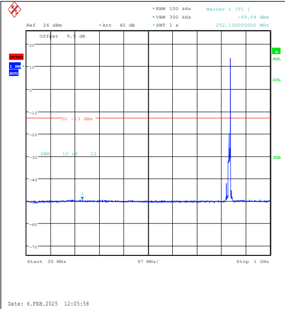
Band26(824-849)-10MHz-16QAM-26915-1RB#49-30~1000-PASS
