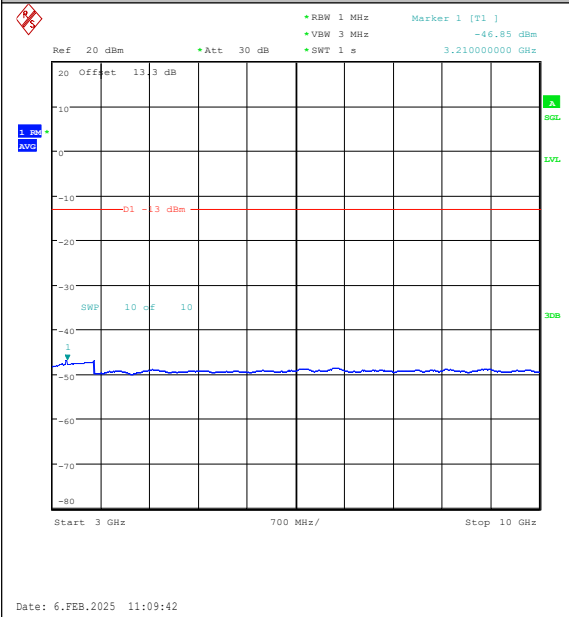
Band26(824-849)-5MHz-16QAM-26815-1RB#24-3 000~10000-PASS
