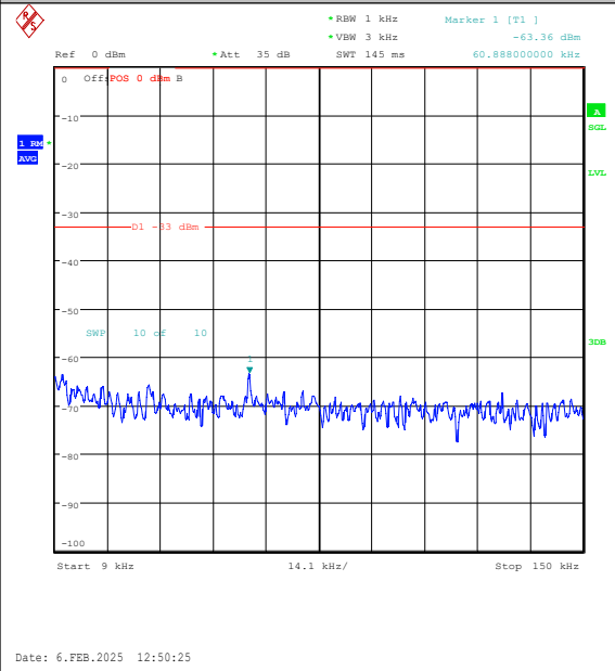
Band26(824-849)-15MHz-16QAM-26865-75RB#0-0.009~0.15-PASS
