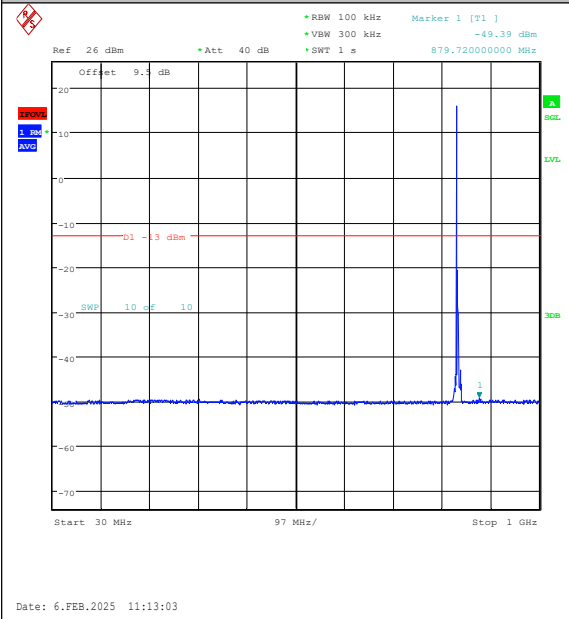
Band26(824-849)-5MHz-QPSK-26915-1RB#0-30~ 1000-PASS
