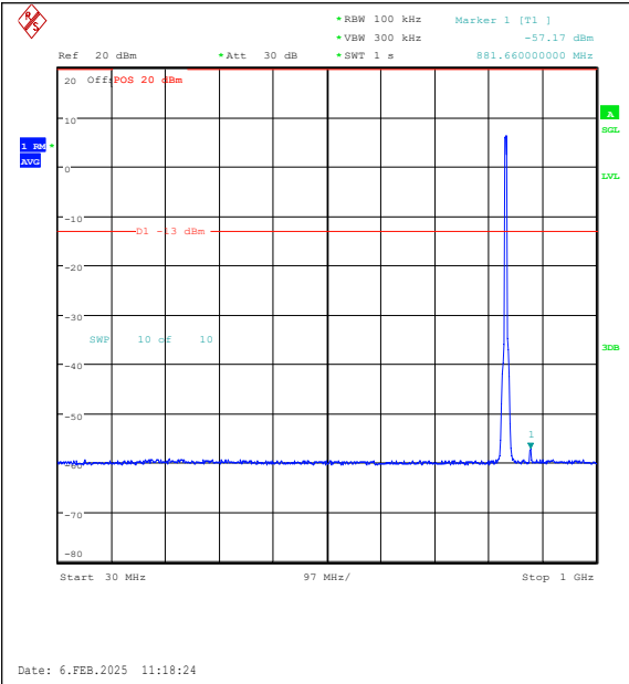
Band26(824-849)-5MHz-QPSK-26915-25RB#0-30 ~1000-PASS
