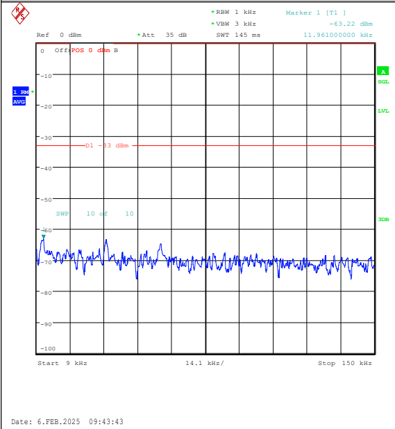
Band26(824-849)-1.4MHz-16QAM-27033-1RB#5- 0.009~0.15-PASS
