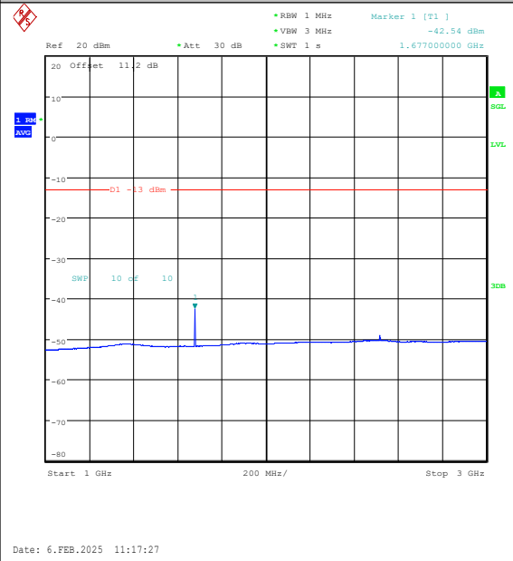
Band26(824-849)-5MHz-16QAM-26915-1RB#24-1 000~3000-PASS
