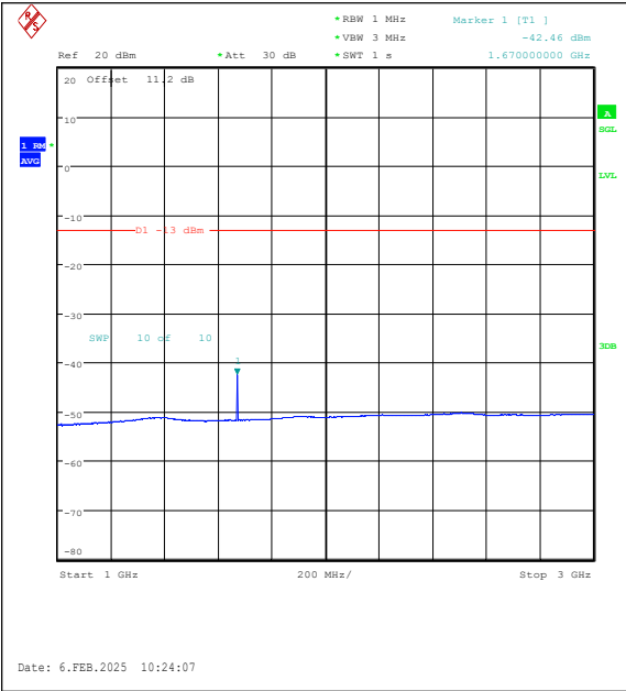
Band26(824-849)-3MHz-16QAM-26915-1RB#0-10 00~3000-PASS
