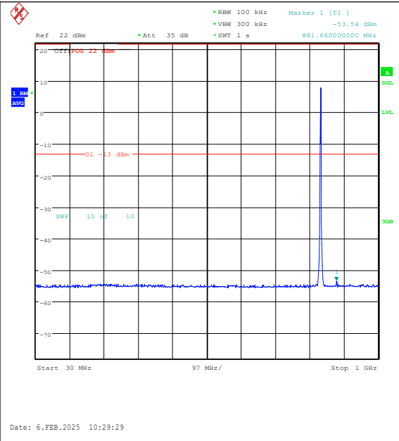
Band26(824-849)-3MHz-16QAM-26915-15RB#0-3 0~1000-PASS
