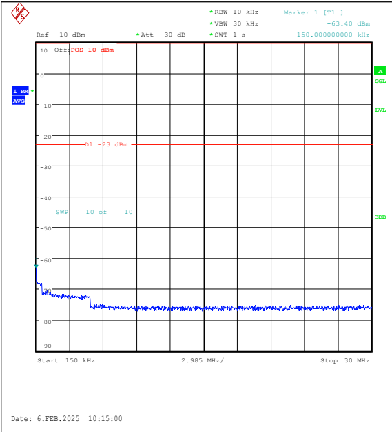
Band26(824-849)-3MHz-16QAM-26805-1RB#0-0. 15~30-PASS
