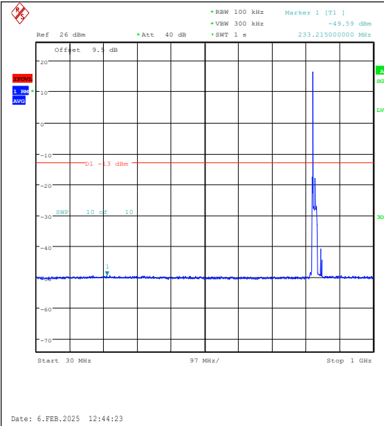
Band26(824-849)-15MHz-QPSK-26865-1RB#0-30 ~1000-PASS
