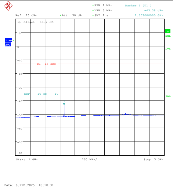
Band26(824-849)-3MHz-16QAM-26805-1RB#14-1 000~3000-PASS
