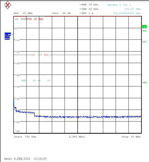
Band26(824-849)-10MHz-16QAM-26990-50RB#0-0.15~30-PASS
