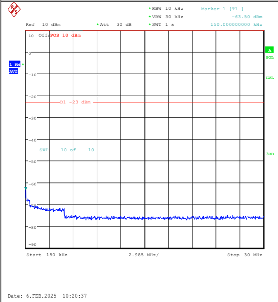
Band26(824-849)-3MHz-16QAM-26805-15RB#0-0 .15~30-PASS
