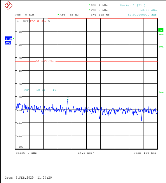
Band26(824-849)-5MHz-16QAM-27015-1RB#24-0 .009~0.15-PASS
