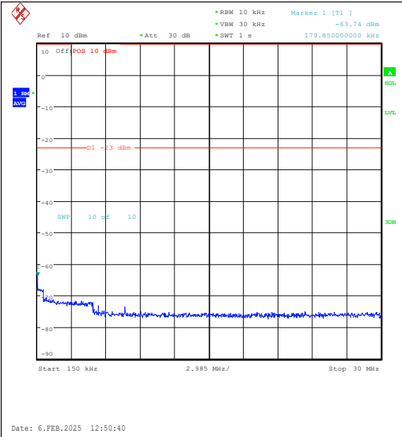
Band26(824-849)-15MHz-16QAM-26865-75RB#0-0.15~30-PASS
