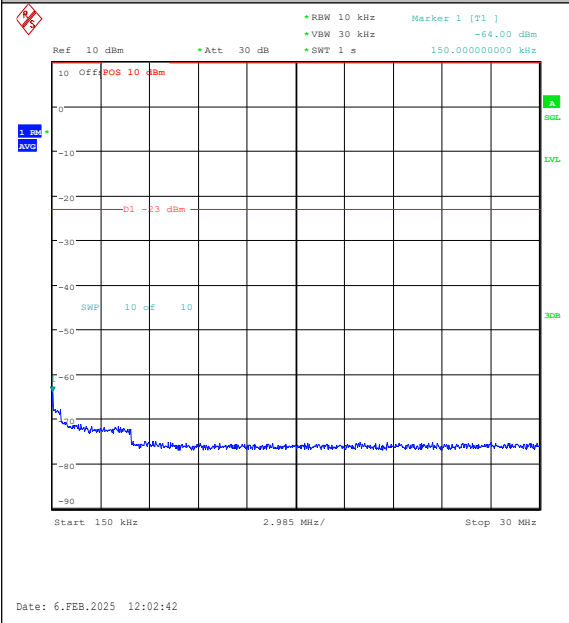
Band26(824-849)-10MHz-16QAM-26915-1RB#0-0 .15~30-PASS
