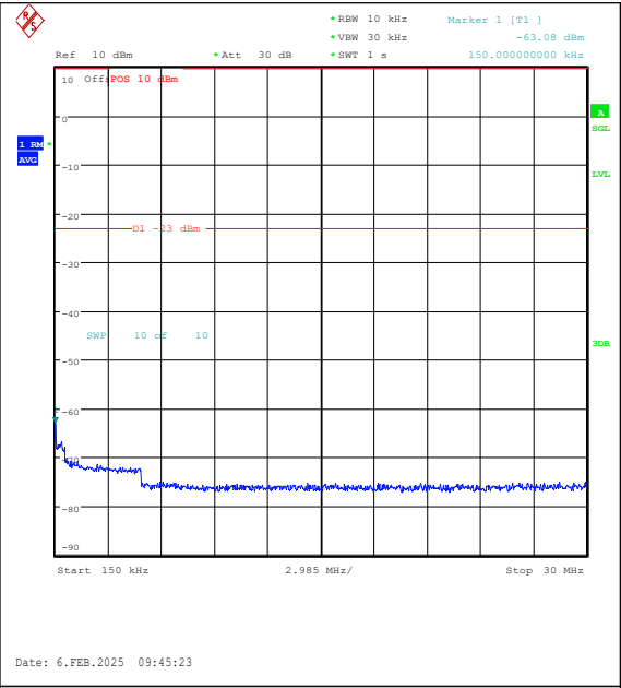
Band26(824-849)-1.4MHz-QPSK-27033-6RB#0-0. 15~30-PASS
