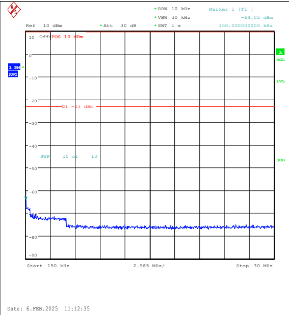
Band26(824-849)-5MHz-QPSK-26915-1RB#0-0.1 5~30-PASS
