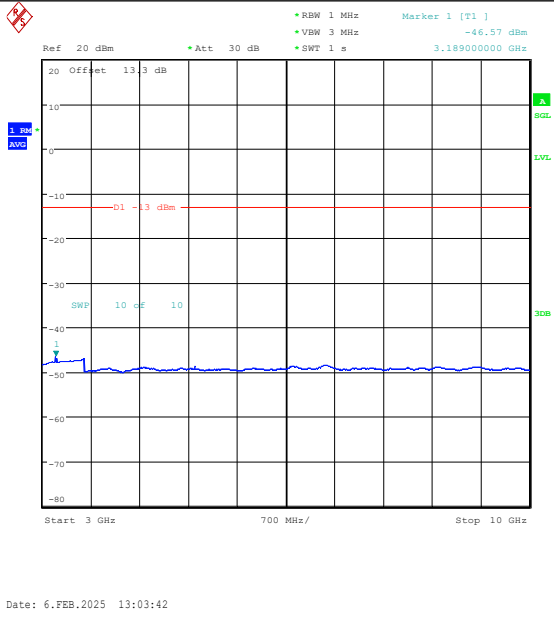
Band26(824-849)-15MHz-QPSK-26965-1RB#74-3 000~10000-PASS
