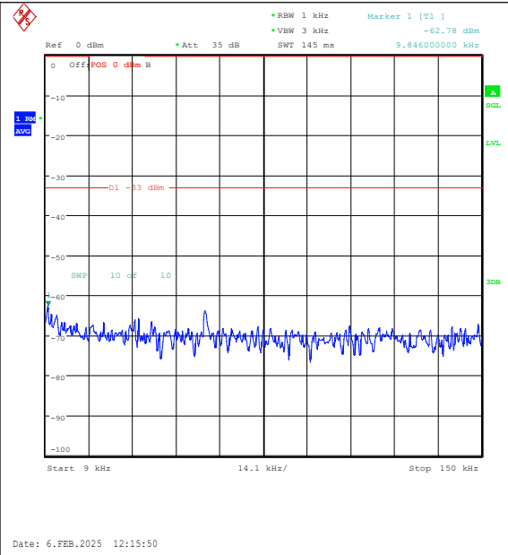
Band26(824-849)-10MHz-16QAM-26990-50RB#0-0.009~0.15-PASS
