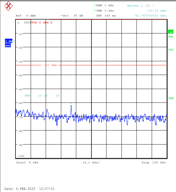
Band26(824-849)-10MHz-16QAM-26915-50RB#0-0.009~0.15-PASS
