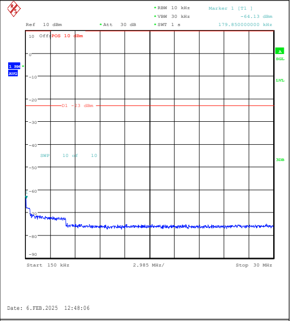
Band26(824-849)-15MHz-16QAM-26865-1RB#74- 0.15~30-PASS
