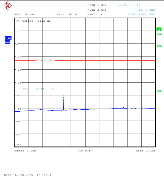
Band26(824-849)-10MHz-16QAM-26990-1RB#49- 1000~3000-PASS
