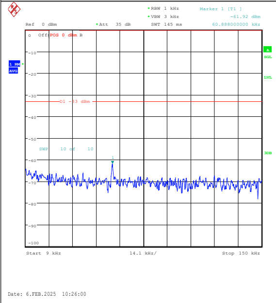
Band26(824-849)-3MHz-16QAM-26915-1RB#14-0 .009~0.15-PASS
