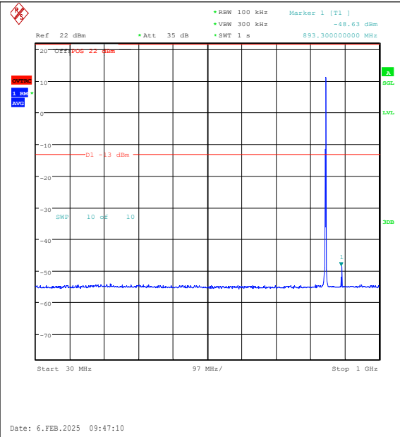
Band26(824-849)-1.4MHz-16QAM-27033-6RB#0-30~1000-PASS
