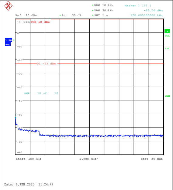
Band26(824-849)-5MHz-16QAM-27015-1RB#24-0 .15~30-PASS
