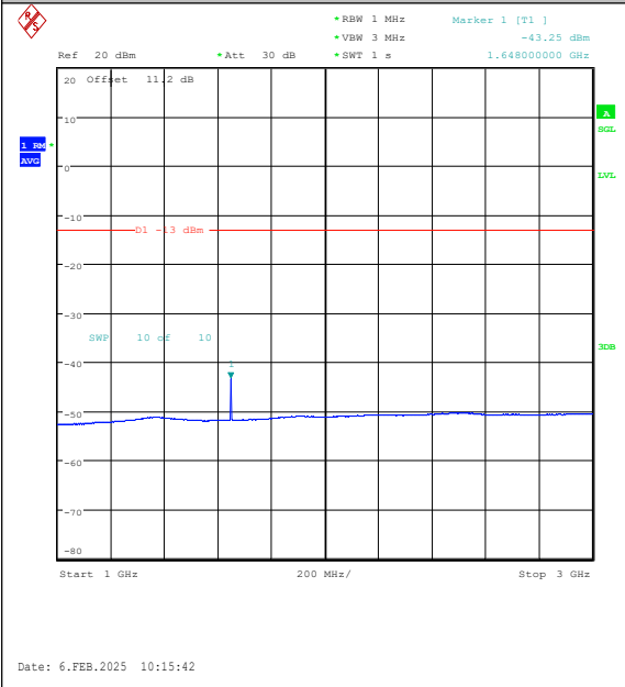
Band26(824-849)-3MHz-16QAM-26805-1RB#0-10 00~3000-PASS
