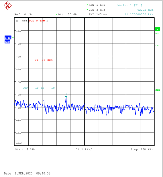
Band26(824-849)-1.4MHz-16QAM-27033-1RB#0- 0.009~0.15-PASS
