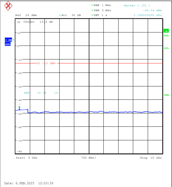
Band26(824-849)-10MHz-16QAM-26915-1RB#0-3 000~10000-PASS
