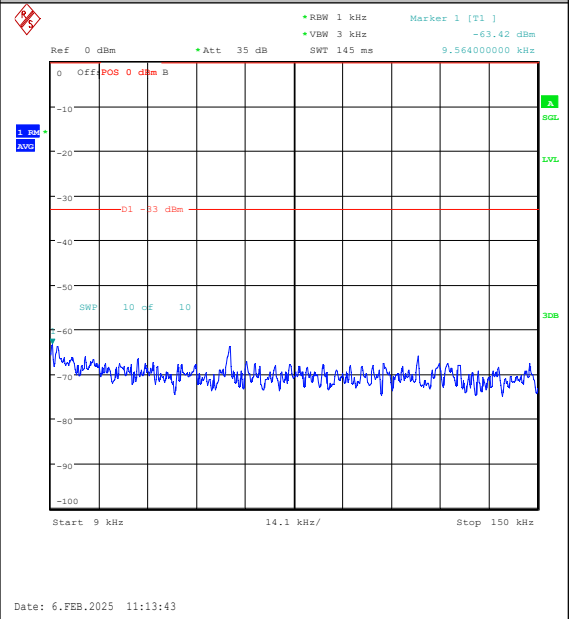
Band26(824-849)-5MHz-16QAM-26915-1RB#0-0. 009~0.15-PASS
