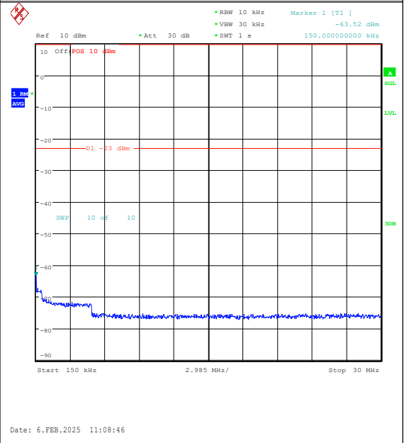
Band26(824-849)-5MHz-16QAM-26815-1RB#24-0 .15~30-PASS
