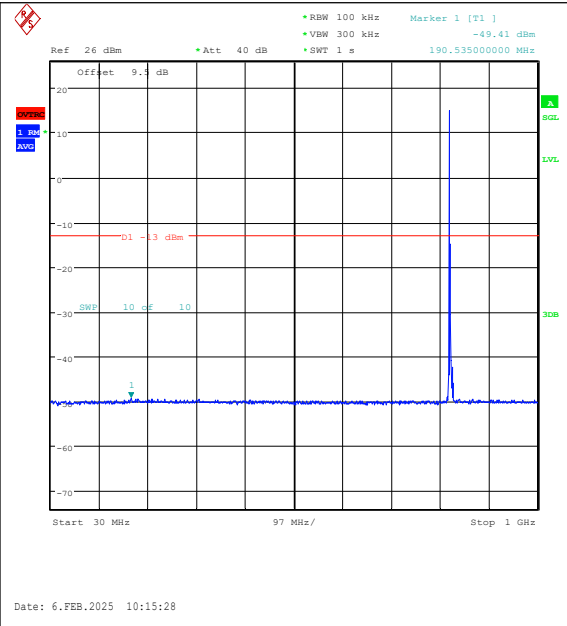
Band26(824-849)-3MHz-16QAM-26805-1RB#0-30 ~1000-PASS
