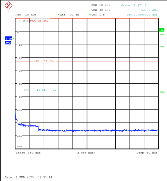
Band26(824-849)-1.4MHz-16QAM-26915-6RB#0-0.15~30-PASS
