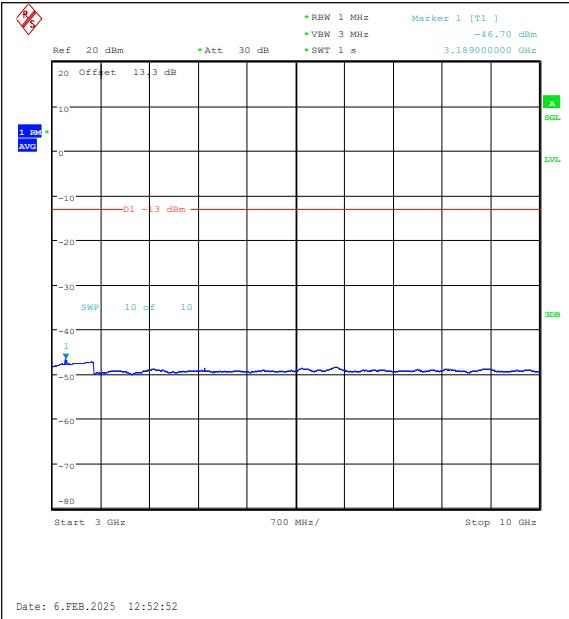
Band26(824-849)-15MHz-QPSK-26915-1RB#0-30 00~10000-PASS
