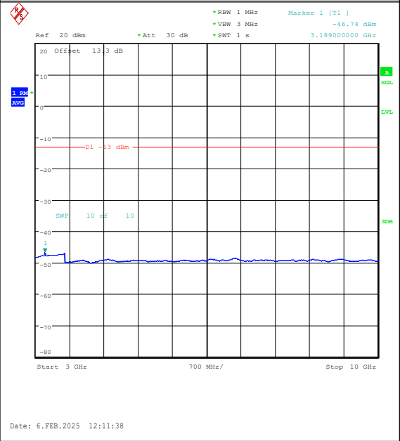
Band26(824-849)-10MHz-16QAM-26990-1RB#0-3 000~10000-PASS
