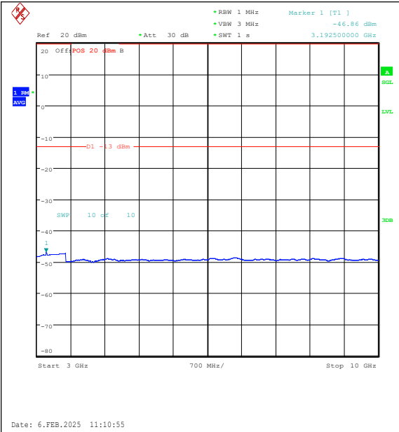
Band26(824-849)-5MHz-QPSK-26815-25RB#0-30 00~10000-PASS
