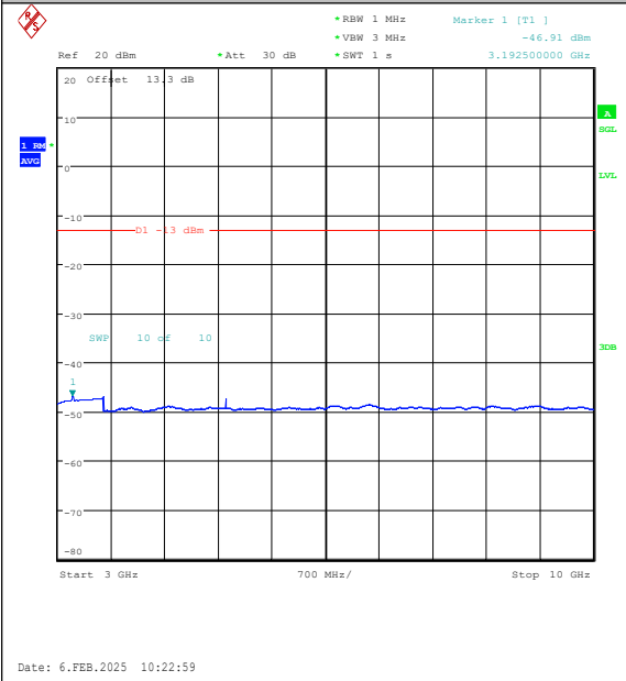
Band26(824-849)-3MHz-QPSK-26915-1RB#0-3000~10000-PASS
