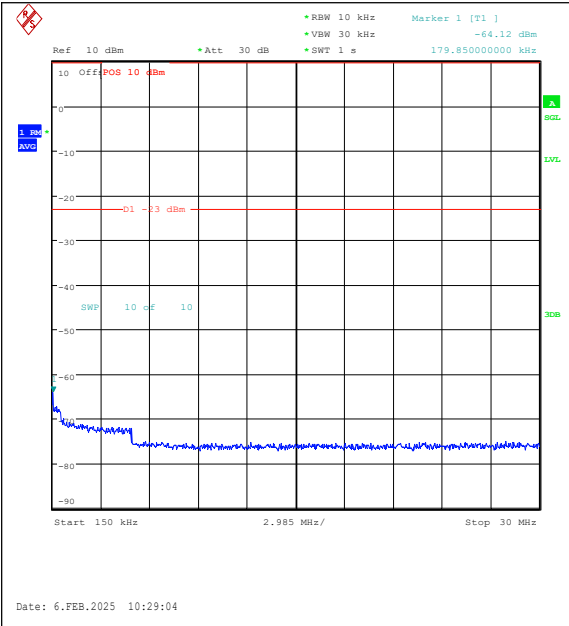
Band26(824-849)-3MHz-16QAM-26915-15RB#0-0 .15~30-PASS
