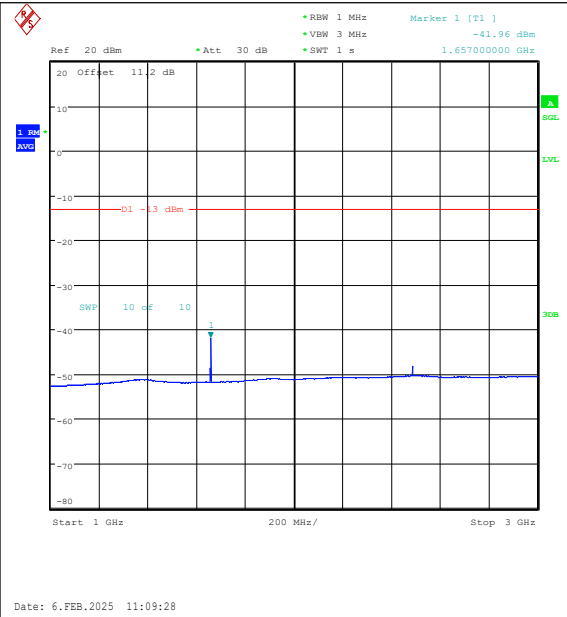
Band26(824-849)-5MHz-16QAM-26815-1RB#24-1 000~3000-PASS
