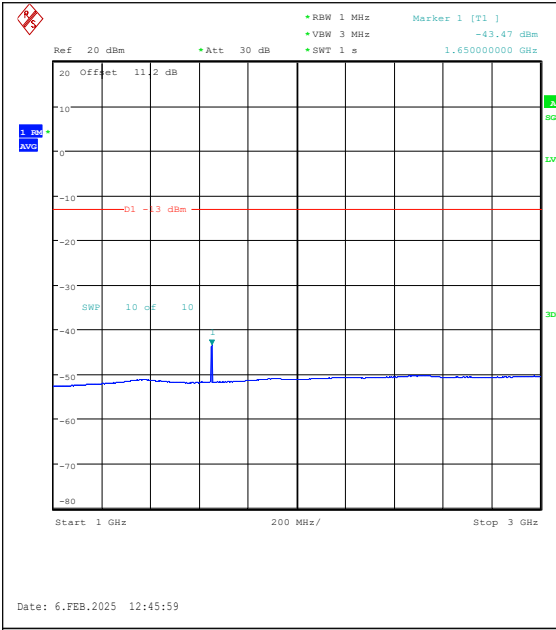
Band26(824-849)-15MHz-16QAM-26865-1RB#0-1 000~3000-PASS
