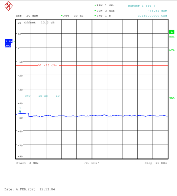
Band26(824-849)-10MHz-QPSK-26990-1RB#49-3 000~10000-PASS
