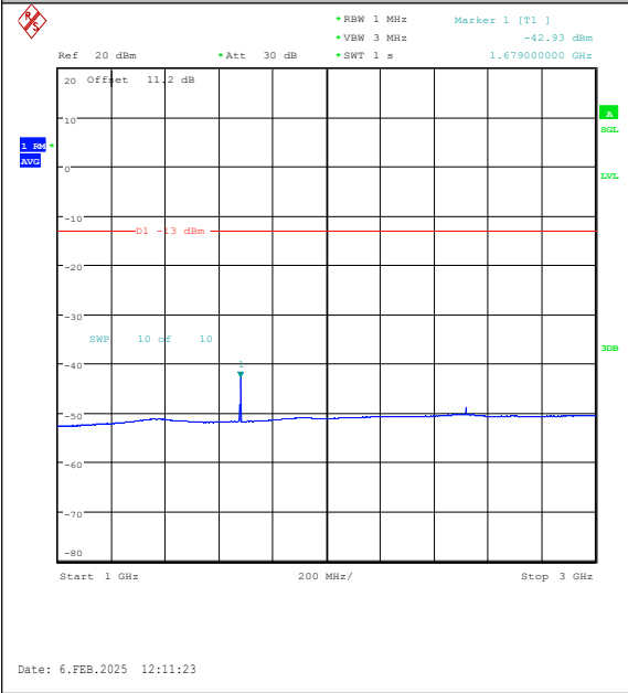
Band26(824-849)-10MHz-16QAM-26990-1RB#0-1 000~3000-PASS
