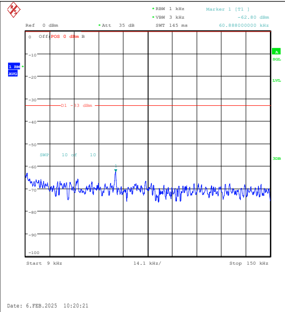
Band26(824-849)-3MHz-16QAM-26805-15RB#0-0 .009~0.15-PASS
