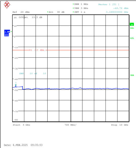
Band26(824-849)-1.4MHz-16QAM-26915-1RB#5-3000~10000-PASS
