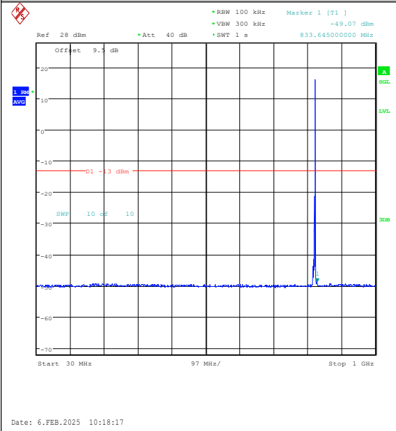
Band26(824-849)-3MHz-16QAM-26805-1RB#14-3 0~1000-PASS
