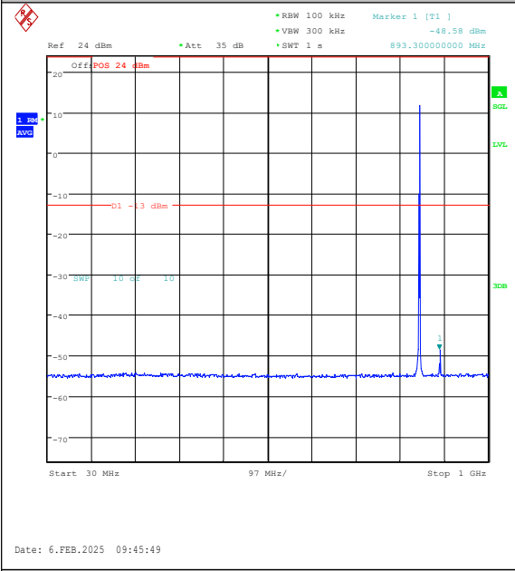
Band26(824-849)-1.4MHz-QPSK-27033-6RB#0-0 0~1000-PASS
