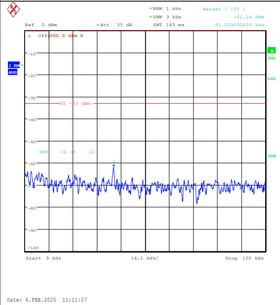
Band26(824-849)-5MHz-16QAM-26815-25RB#0-0 .009~0.15-PASS
