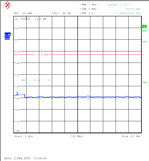
Band26(824-849)-10MHz-16QAM-26915-1RB#49-3000~10000-PASS
