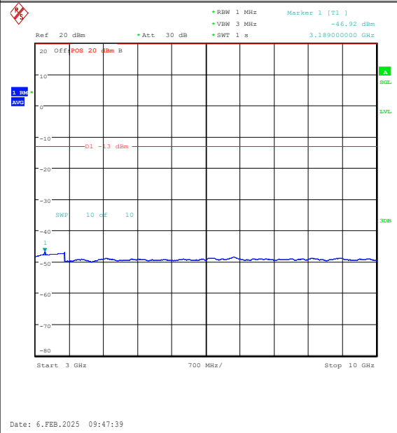
Band26(824-849)-1.4MHz-16QAM-27033-6RB#0-3000~10000-PASS
