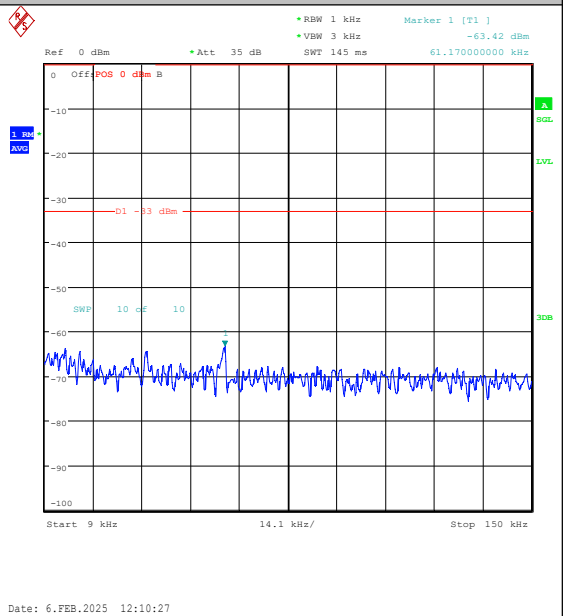
Band26(824-849)-10MHz-16QAM-26990-1RB#0-0 .009~0.15-PASS
