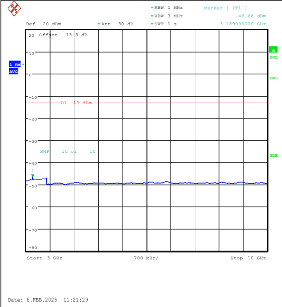
Band26(824-849)-5MHz-QPSK-27015-1RB#0-3000~10000-PASS
