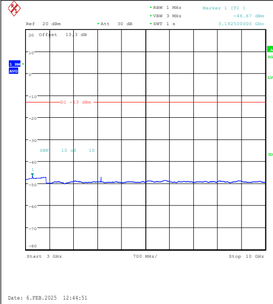
Band26(824-849)-15MHz-QPSK-26865-1RB#0-30 00~10000-PASS
