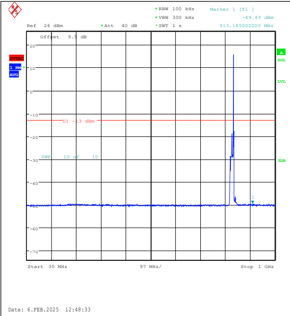
Band26(824-849)-15MHz-16QAM-26865-1RB#74-30~1000-PASS
