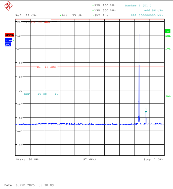
Band26(824-849)-1.4MHz-16QAM-26915-6RB#0-30~1000-PASS
