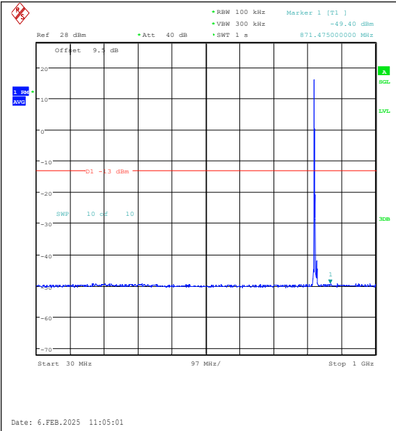
Band26(824-849)-5MHz-QPSK-26815-1RB#0-30~1000-PASS
