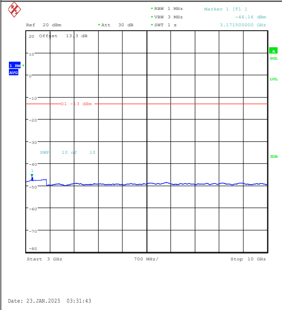
Band26(814-824)-1.4MHz-16QAM-26783-1RB#5-3000~10000-PASS
