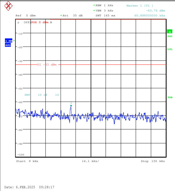
Band26(824-849)-1.4MHz-16QAM-26797-6RB#0-0.009~0.15-PASS
