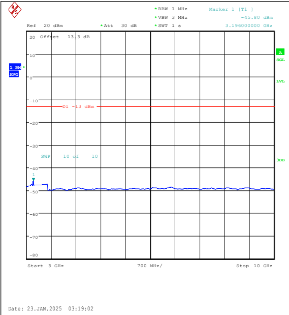
Band26(814-824)-1.4MHz-QPSK-26740-1RB#0-3 000~10000-PASS
