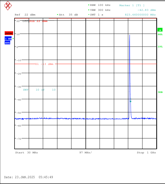
Band26(814-824)-3MHz-16QAM-26705-15RB#0-3 0~1000-PASS
