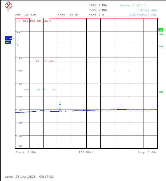
Band26(814-824)-1.4MHz-16QAM-26697-6RB#0-1000~3000-PASS
