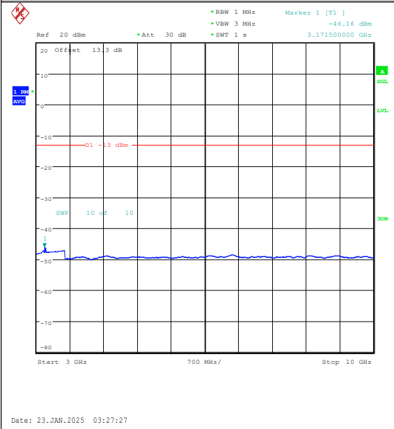
Band26(814-824)-1.4MHz-QPSK-26783-1RB#0-3 000~10000-PASS
