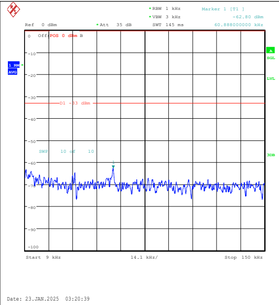
Band26(814-824)-1.4MHz-QPSK-26740-1RB#5-0. 009~0.15-PASS
