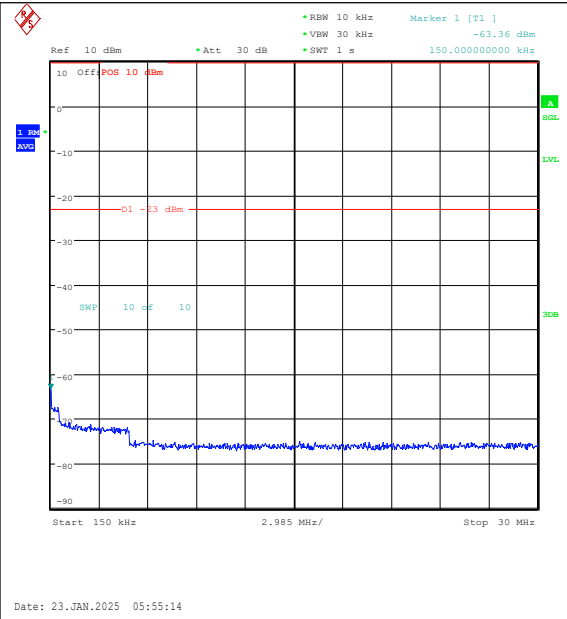
Band26(814-824)-3MHz-QPSK-26775-1RB#0-0.1 5~30-PASS
