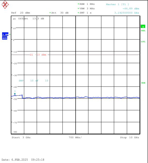
Band26(824-849)-1.4MHz-QPSK-26797-1RB#5-3 000~10000-PASS
