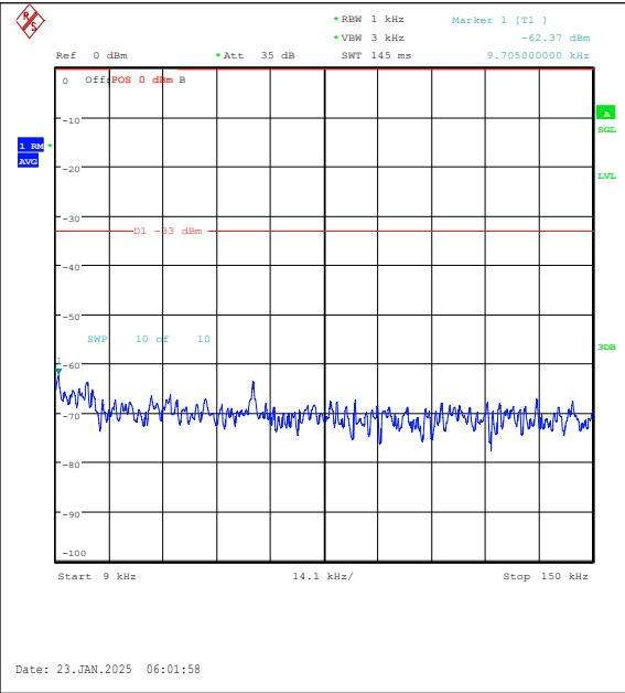
Band26(814-824)-3MHz-16QAM-26775-15RB#0-0 .009~0.15-PASS
