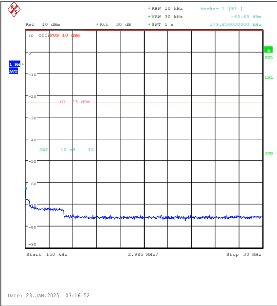
Band26(814-824)-1.4MHz-16QAM-26697-6RB#0-0.15~30-PASS
