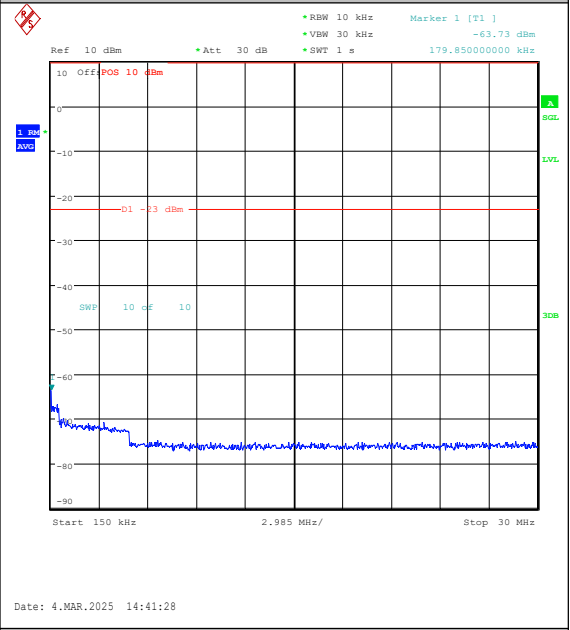
Band26(814-824)-5MHz-QPSK-26740-25RB#0-0. 15~30-PASS
