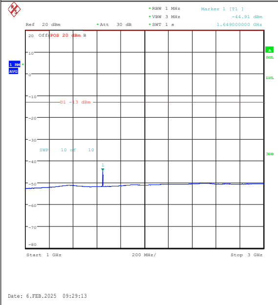
Band26(824-849)-1.4MHz-16QAM-26797-6RB#0-1000~3000-PASS
