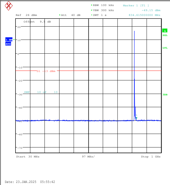
Band26(814-824)-3MHz-QPSK-26775-1RB#0-30~ 1000-PASS
