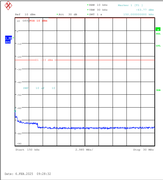
Band26(824-849)-1.4MHz-16QAM-26797-6RB#0-0.15~30-PASS
