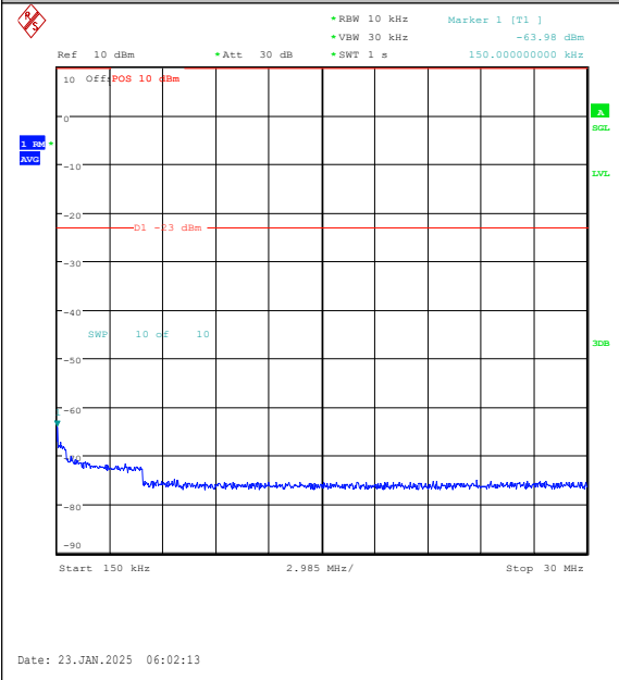
Band26(814-824)-3MHz-16QAM-26775-15RB#0-0 .15~30-PASS
