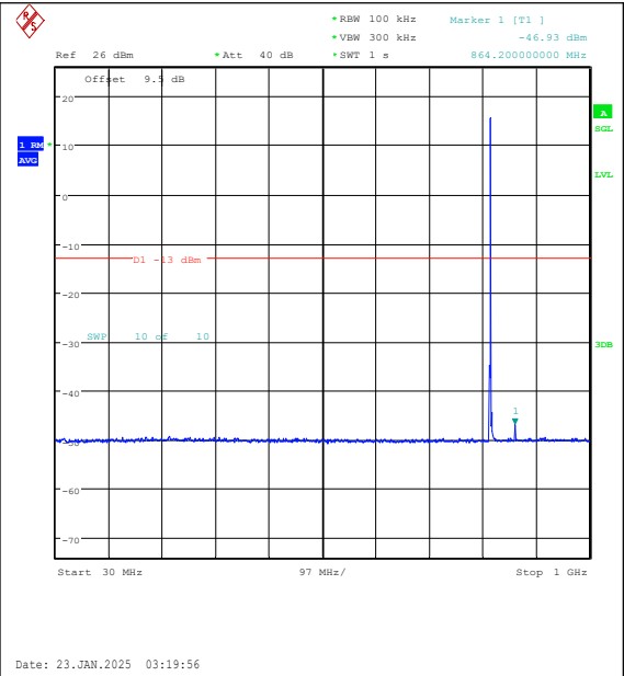
Band26(814-824)-1.4MHz-16QAM-26740-1RB#0-30~1000-PASS
