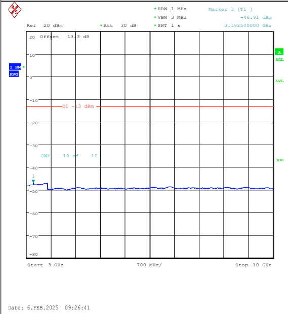
Band26(824-849)-1.4MHz-16QAM-26797-1RB#5-3000~10000-PASS
