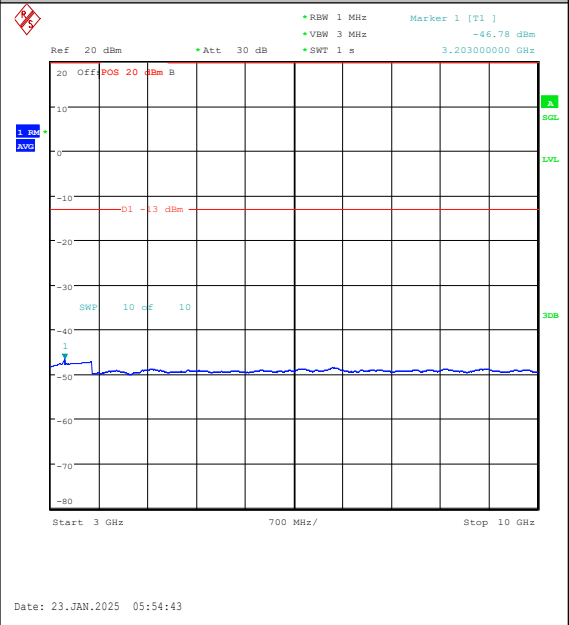
Band26(814-824)-3MHz-16QAM-26740-15RB#0-3 000~10000-PASS
