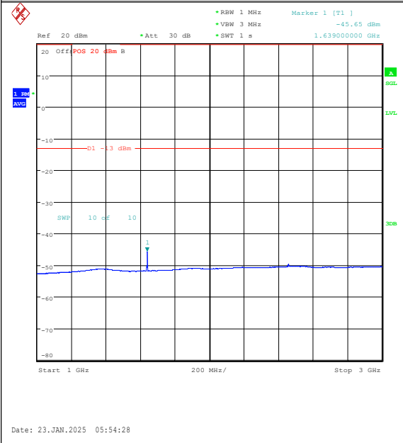
Band26(814-824)-3MHz-16QAM-26740-15RB#0-1 000~3000-PASS
