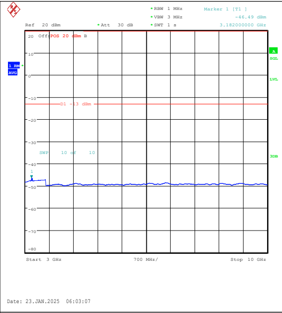
Band26(814-824)-3MHz-16QAM-26775-15RB#0-3 000~10000-PASS
