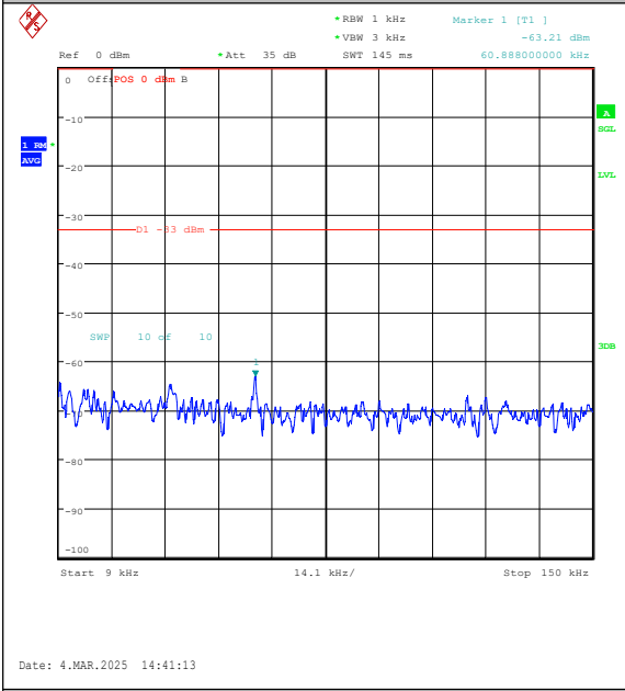
Band26(814-824)-5MHz-QPSK-26740-25RB#0-0. 009~0.15-PASS
