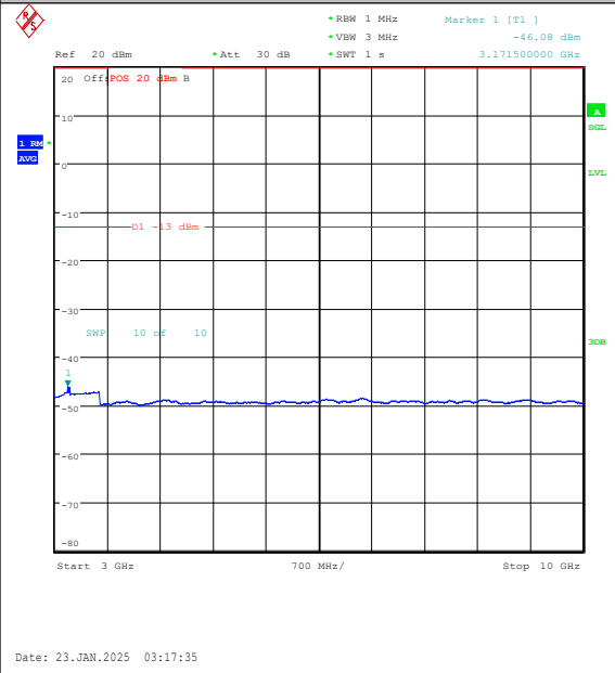
Band26(814-824)-1.4MHz-16QAM-26697-6RB#0-3000~10000-PASS
