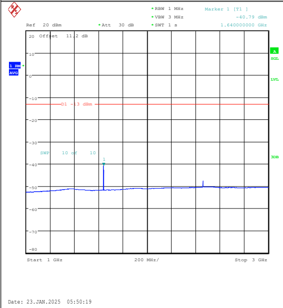
Band26(814-824)-3MHz-QPSK-26740-1RB#14-10 00~3000-PASS
