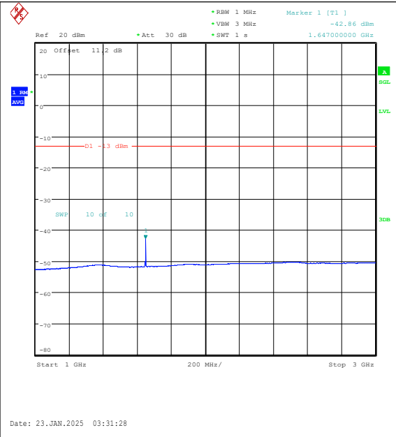
Band26(814-824)-1.4MHz-16QAM-26783-1RB#5-1000~3000-PASS
