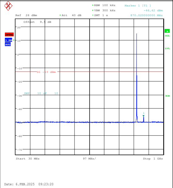
Band26(824-849)-1.4MHz-16QAM-26797-1RB#0- 30~1000-PASS
