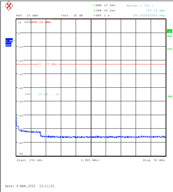
Band26(814-824)-10MHz-16QAM-26740-1RB#0-0 .15~30-PASS
