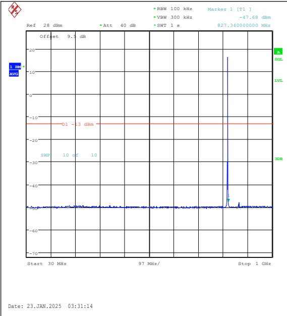
Band26(814-824)-1.4MHz-16QAM-26783-1RB#5-30~1000-PASS
