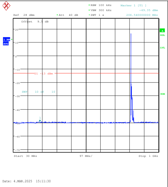
Band26(814-824)-10MHz-16QAM-26740-1RB#0-3 0~1000-PASS
