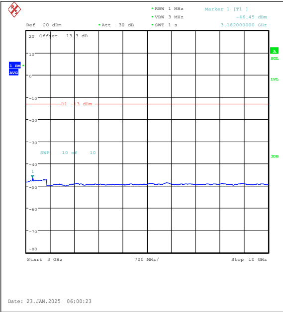
Band26(814-824)-3MHz-16QAM-26775-1RB#14-3 000~10000-PASS
