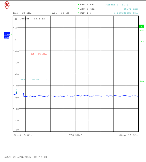
Band26(814-824)-3MHz-QPSK-26705-1RB#14-30 00~10000-PASS
