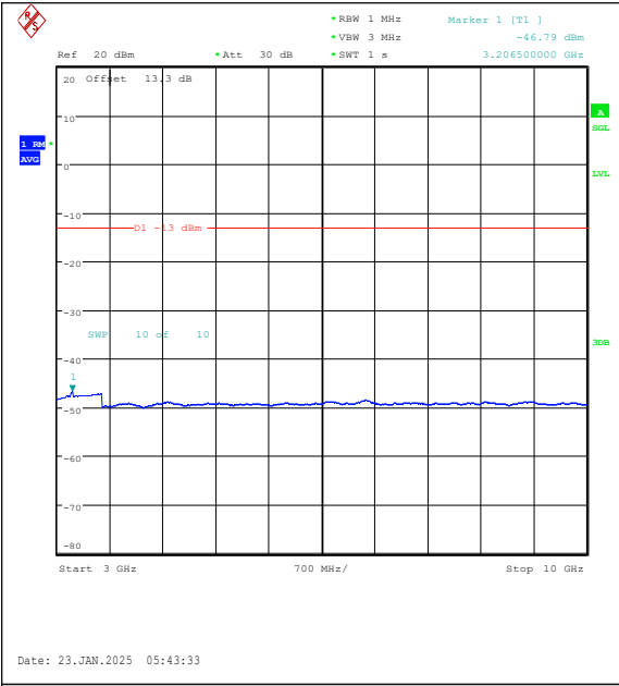
Band26(814-824)-3MHz-16QAM-26705-1RB#14-3 000~10000-PASS
