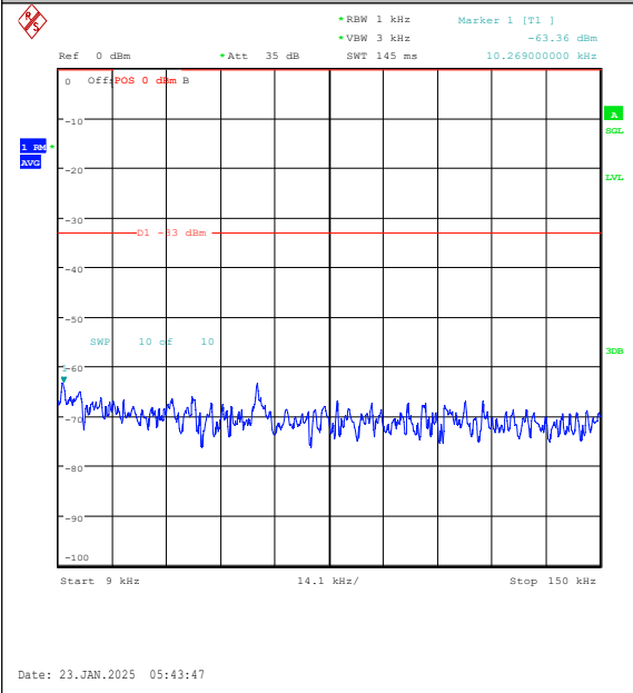
Band26(814-824)-3MHz-QPSK-26705-15RB#0-0. 009~0.15-PASS
