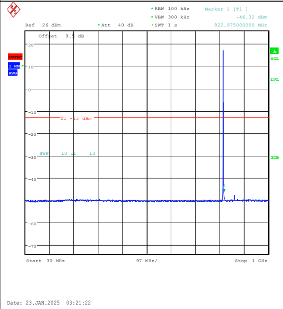
Band26(814-824)-1.4MHz-QPSK-26740-1RB#5-3 0~1000-PASS
