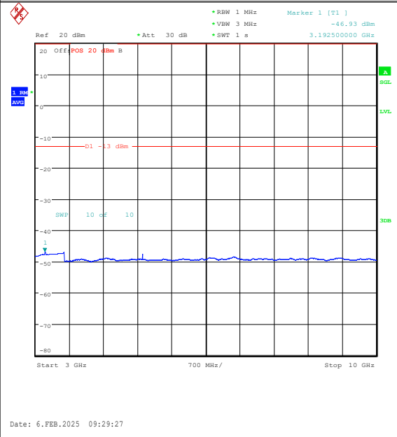
Band26(824-849)-1.4MHz-16QAM-26797-6RB#0-3000~10000-PASS
