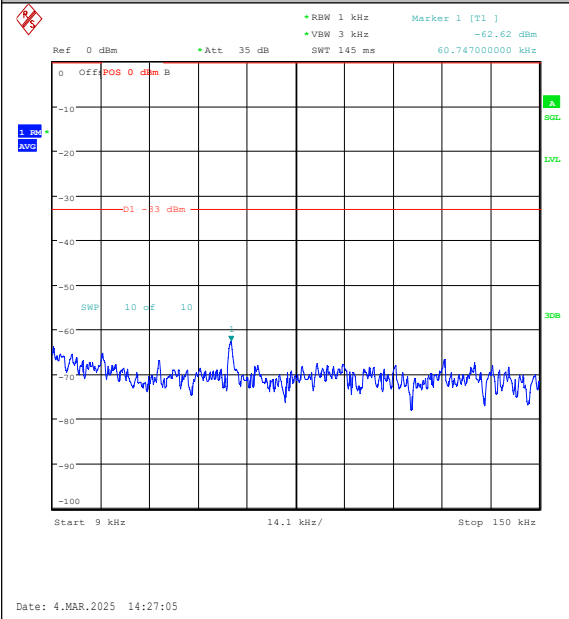
Band26(814-824)-5MHz-QPSK-26715-1RB#0-0.0 09~0.15-PASS
