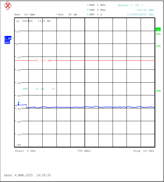
Band26(814-824)-5MHz-QPSK-26740-1RB#24-30 00~10000-PASS
