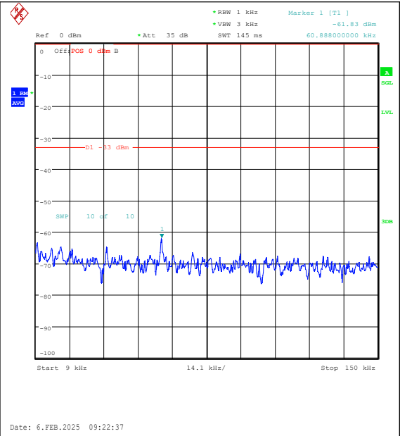
Band26(824-849)-1.4MHz-16QAM-26797-1RB#0- 0.009~0.15-PASS
