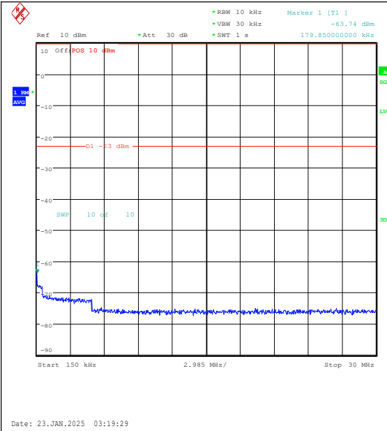
Band26(814-824)-1.4MHz-16QAM-26740-1RB#0-0.15~30-PASS
