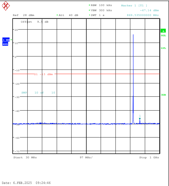
Band26(824-849)-1.4MHz-QPSK-26797-1RB#5-3 0~1000-PASS
