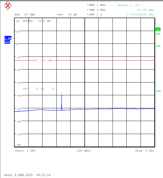
Band26(824-849)-1.4MHz-QPSK-26915-1RB#0-1000~3000-PASS
