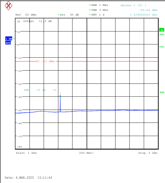
Band26(814-824)-10MHz-16QAM-26740-1RB#0-1 000~3000-PASS
