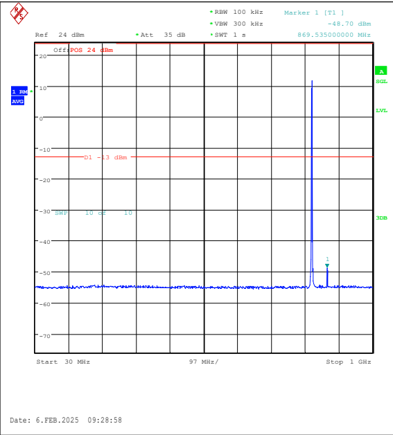
Band26(824-849)-1.4MHz-16QAM-26797-6RB#0-30~1000-PASS
