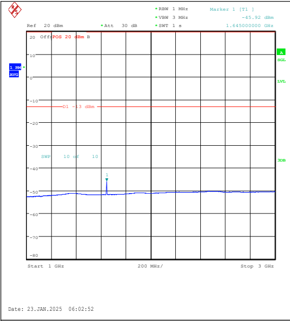
Band26(814-824)-3MHz-16QAM-26775-15RB#0-1 000~3000-PASS
