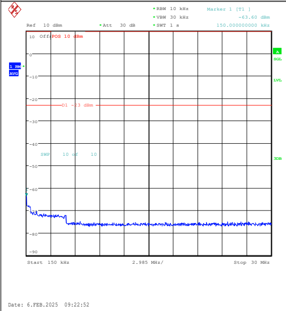
Band26(824-849)-1.4MHz-16QAM-26797-1RB#0- 0.15~30-PASS
