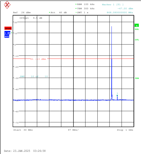
Band26(814-824)-1.4MHz-QPSK-26783-1RB#0-3 0~1000-PASS
