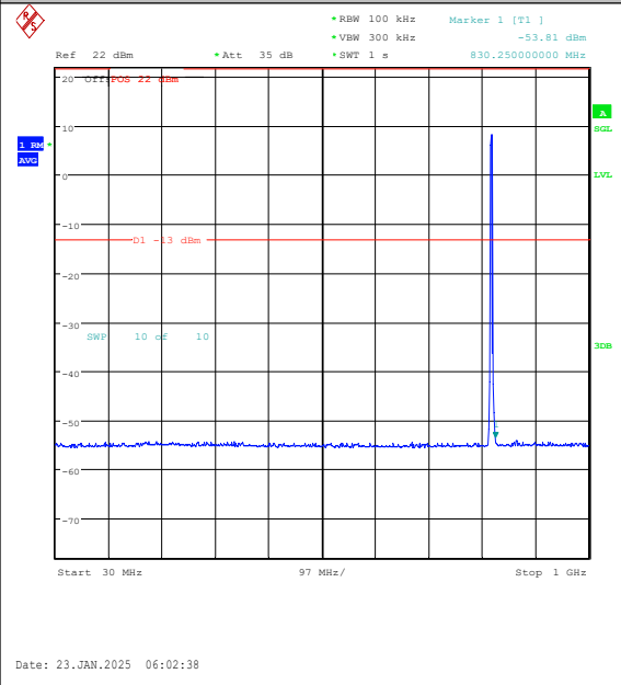
Band26(814-824)-3MHz-16QAM-26775-15RB#0-3 0~1000-PASS
