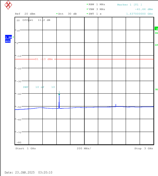
Band26(814-824)-1.4MHz-16QAM-26740-1RB#0-1000~3000-PASS
