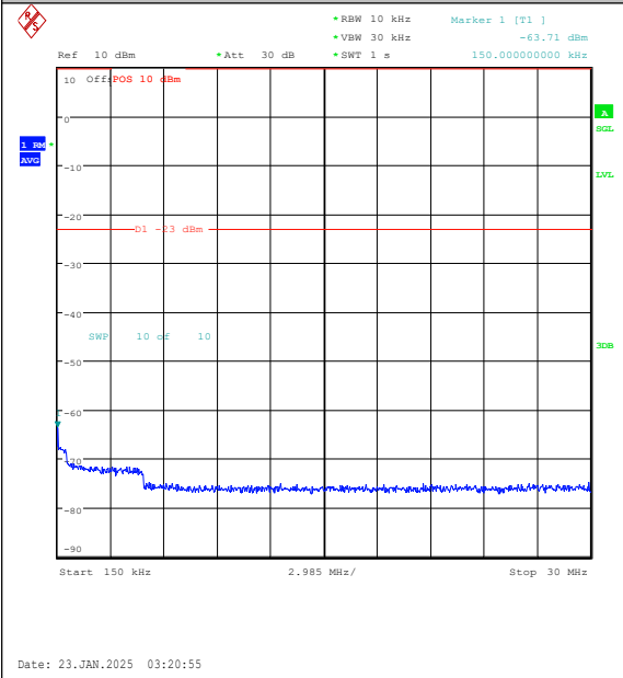
Band26(814-824)-1.4MHz-QPSK-26740-1RB#5-0. 15~30-PASS
