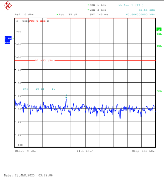
Band26(814-824)-1.4MHz-QPSK-26783-1RB#5-0. 009~0.15-PASS
