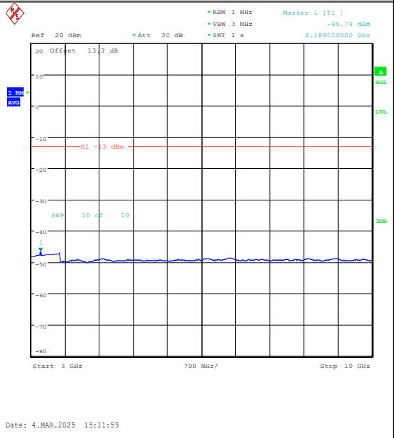
Band26(814-824)-10MHz-16QAM-26740-1RB#0-3 000~10000-PASS
