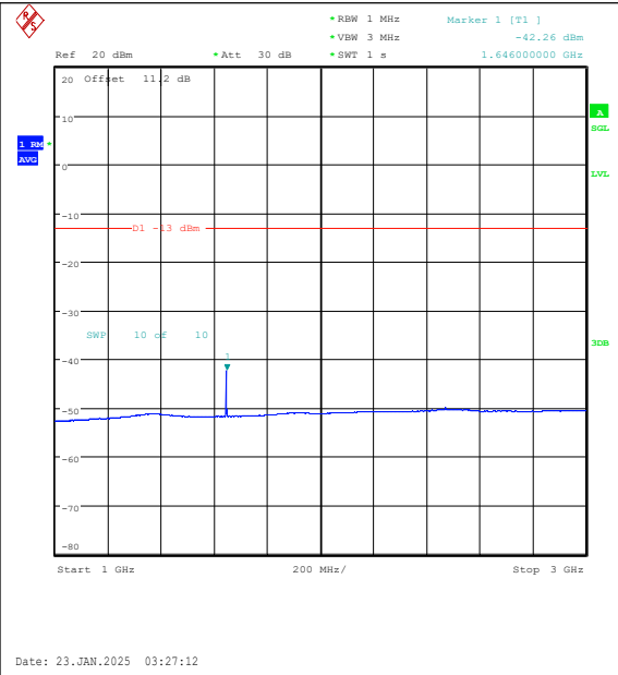
Band26(814-824)-1.4MHz-QPSK-26783-1RB#0-1 000~3000-PASS
