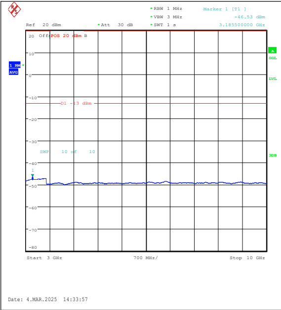
Band26(814-824)-5MHz-QPSK-26715-25RB#0-30 00~10000-PASS
