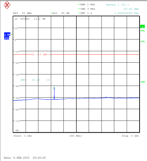
Band26(824-849)-1.4MHz-16QAM-26797-1RB#5-1000~3000-PASS
