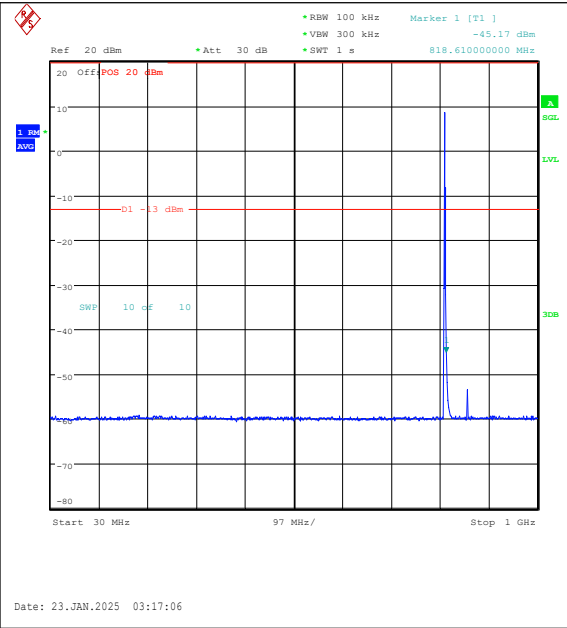
Band26(814-824)-1.4MHz-16QAM-26697-6RB#0-30~1000-PASS
