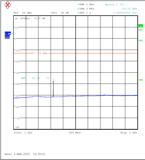
Band26(814-824)-5MHz-QPSK-26740-1RB#24-10 00~3000-PASS
