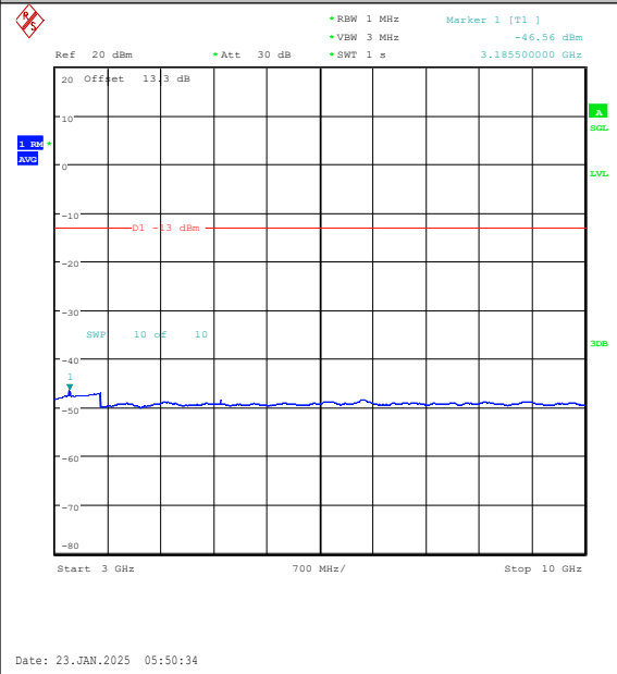
Band26(814-824)-3MHz-QPSK-26740-1RB#14-30 00~10000-PASS
