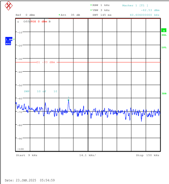
Band26(814-824)-3MHz-QPSK-26775-1RB#0-0.0 09~0.15-PASS
