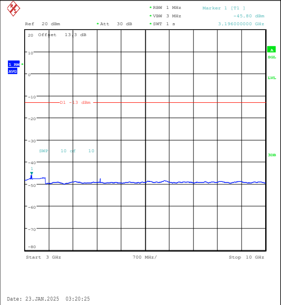
Band26(814-824)-1.4MHz-16QAM-26740-1RB#0-3000~10000-PASS
