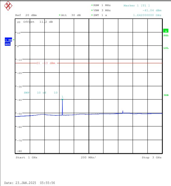
Band26(814-824)-3MHz-QPSK-26775-1RB#0-100 0~3000-PASS
