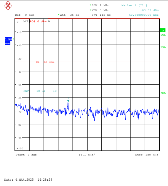
Band26(814-824)-5MHz-16QAM-26715-1RB#0-0. 009~0.15-PASS
