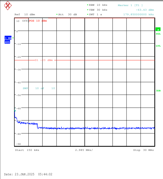
Band26(814-824)-3MHz-QPSK-26705-15RB#0-0. 15~30-PASS
