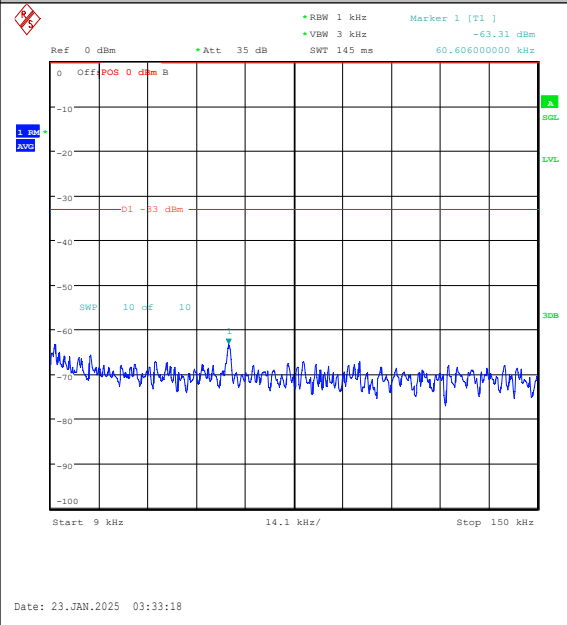
Band26(814-824)-1.4MHz-16QAM-26783-6RB#0-0.009~0.15-PASS
