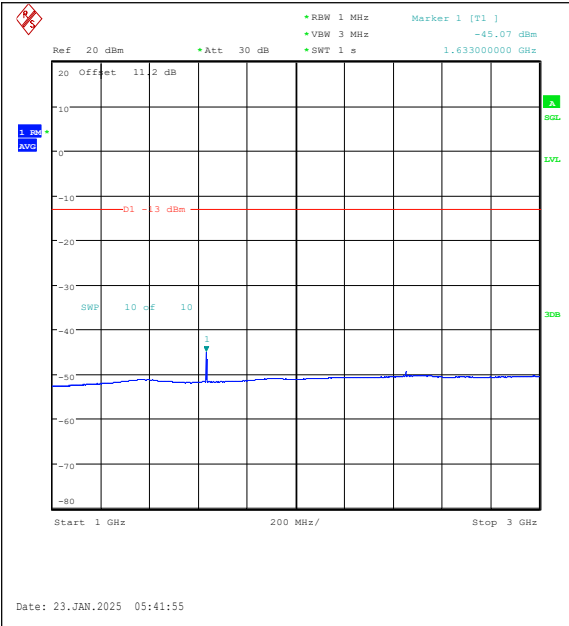
Band26(814-824)-3MHz-QPSK-26705-1RB#14-10 00~3000-PASS
