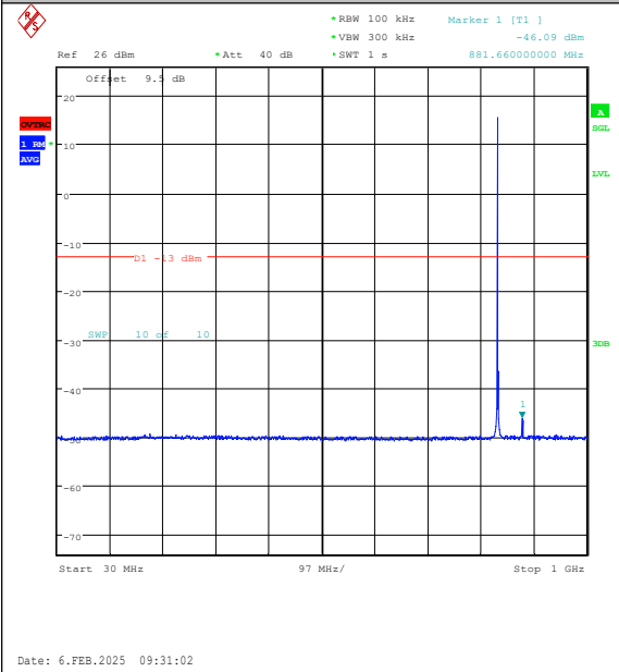
Band26(824-849)-1.4MHz-QPSK-26915-1RB#0-30~1000-PASS
