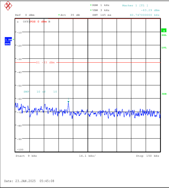
Band26(814-824)-3MHz-16QAM-26705-15RB#0-0 .009~0.15-PASS
