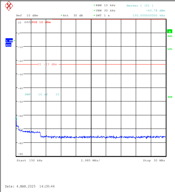
Band26(814-824)-5MHz-16QAM-26715-1RB#0-0. 15~30-PASS
