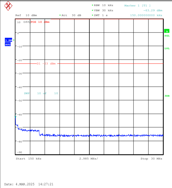
Band26(814-824)-5MHz-QPSK-26715-1RB#0-0.1 5~30-PASS
