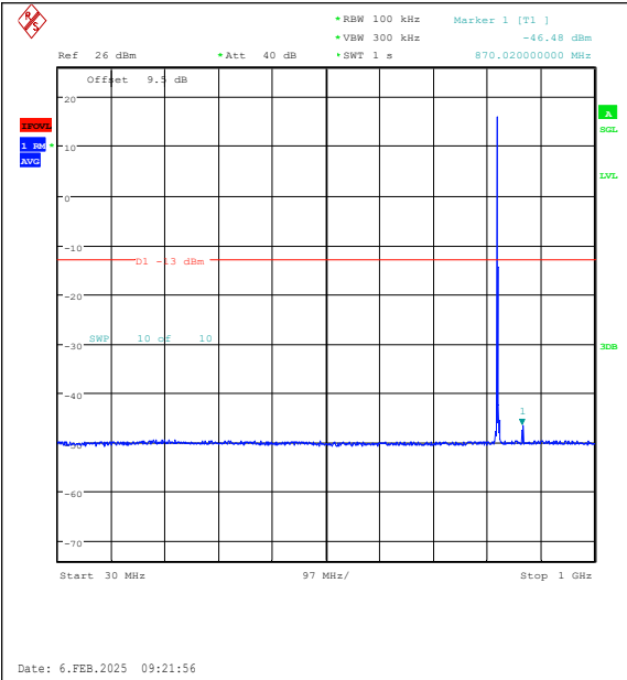
Band26(824-849)-1.4MHz-QPSK-26797-1RB#0-3 0~1000-PASS
