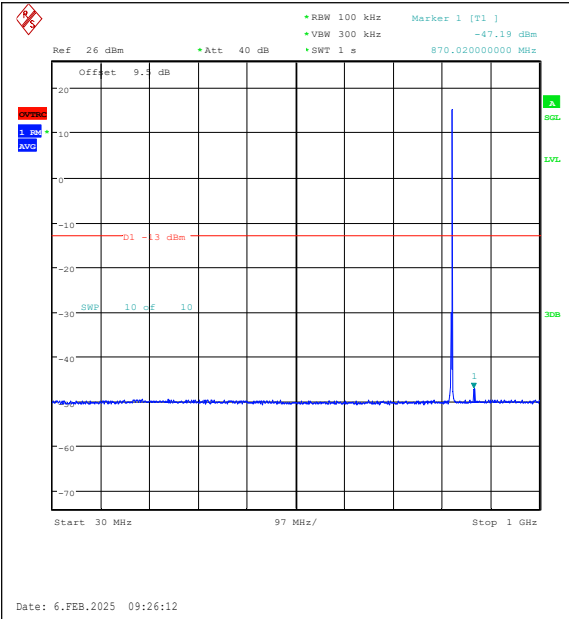
Band26(824-849)-1.4MHz-16QAM-26797-1RB#5-30~1000-PASS
