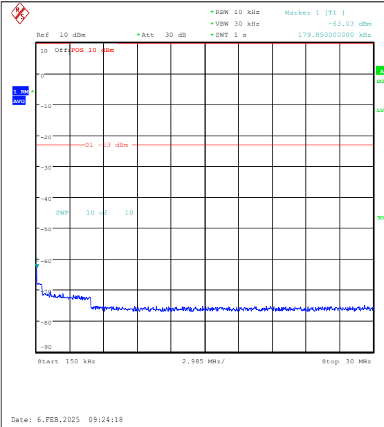
Band26(824-849)-1.4MHz-QPSK-26797-1RB#5-0. 15~30-PASS
