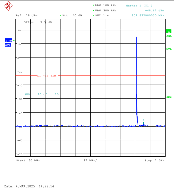
Band26(814-824)-5MHz-16QAM-26715-1RB#0-30 ~1000-PASS
