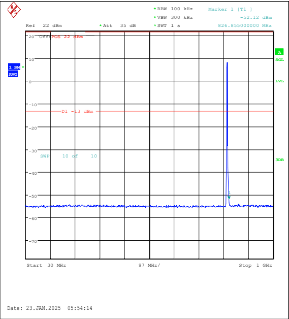
Band26(814-824)-3MHz-16QAM-26740-15RB#0-3 0~1000-PASS
