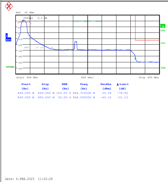
Band26(824-849)-5MHz-QPSK-27015-1RB#0-PA SS
