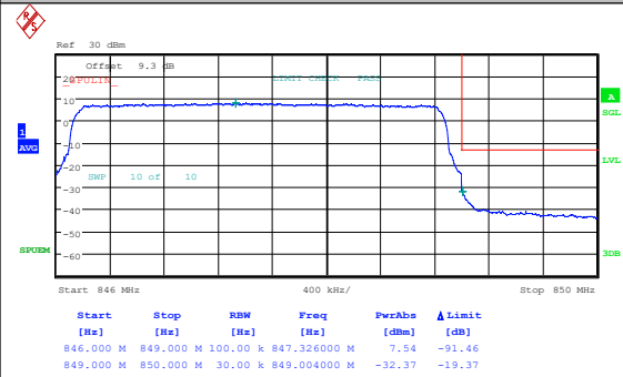
Band26(824-849)-3MHz-16QAM-27025-1RB#0-P ASS
