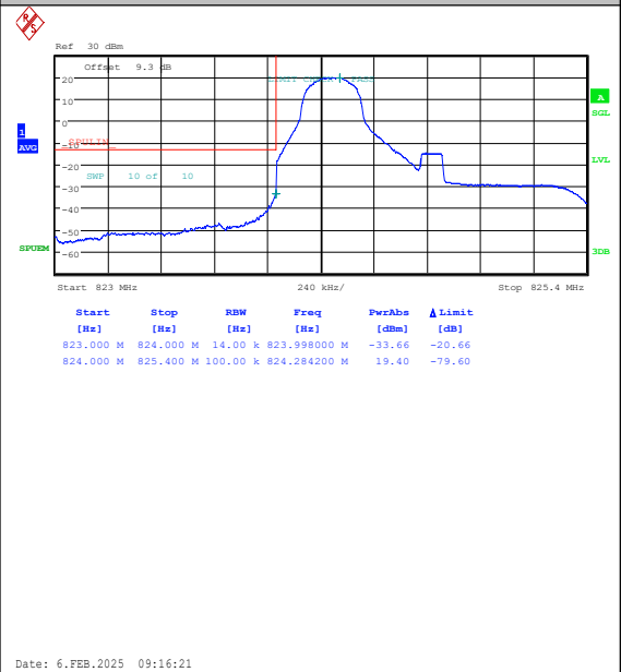
Band26(824-849)-1.4MHz-16QAM-26797-1RB#0-P PASS
