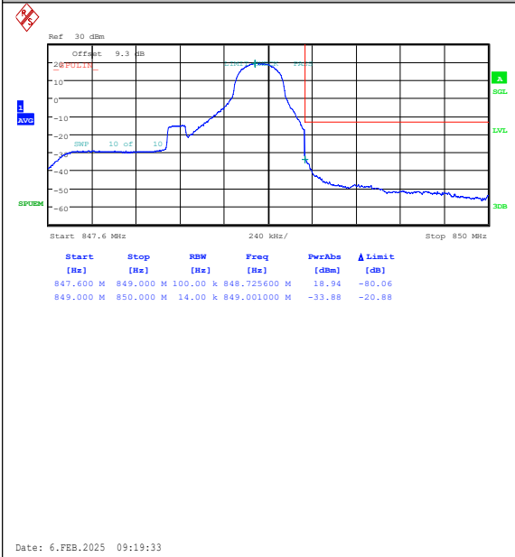
Band26(824-849)-1.4MHz-16QAM-27033-1RB#5-P PASS
