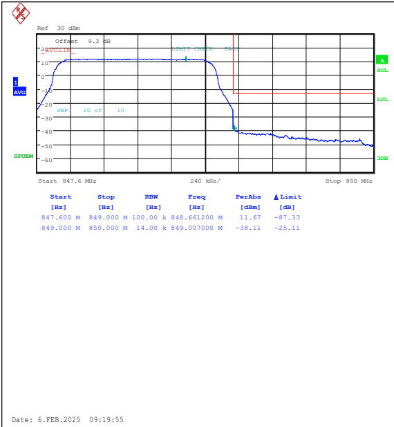
Band26(824-849)-1.4MHz-QPSK-27033-6RB#0-P ASS
