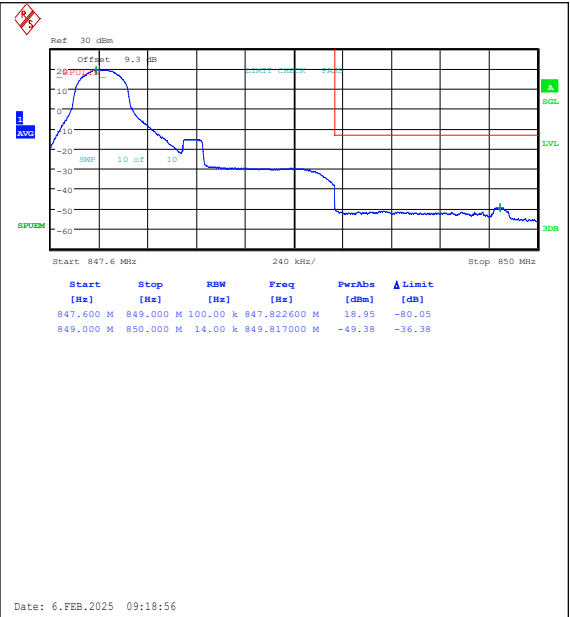
Band26(824-849)-1.4MHz-16QAM-27033-1RB#0-P PASS
