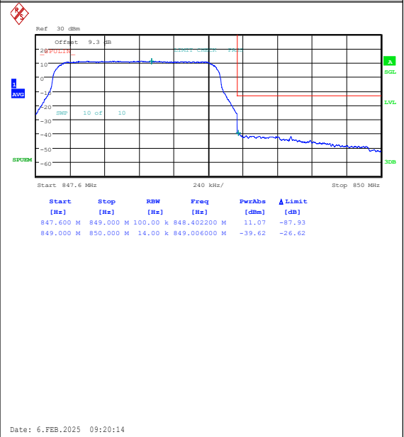
Band26(824-849)-1.4MHz-16QAM-27033-6RB#0-P PASS
