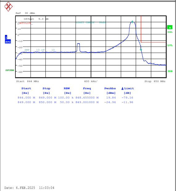
Band26(824-849)-5MHz-QPSK-27015-1RB#24-P ASS
