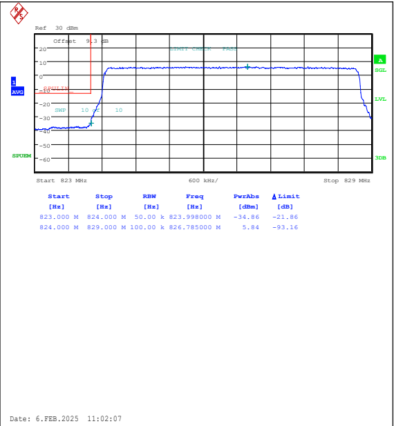
Band26(824-849)-5MHz-16QAM-26815-25RB#0-P ASS
