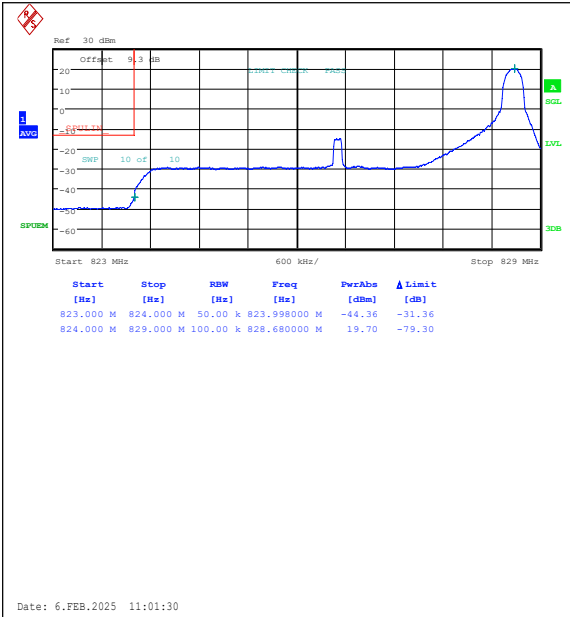
Band26(824-849)-5MHz-16QAM-26815-1RB#24-P ASS
