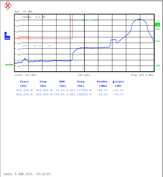
Band26(824-849)-1.4MHz-QPSK-26797-1RB#5-P ASS
