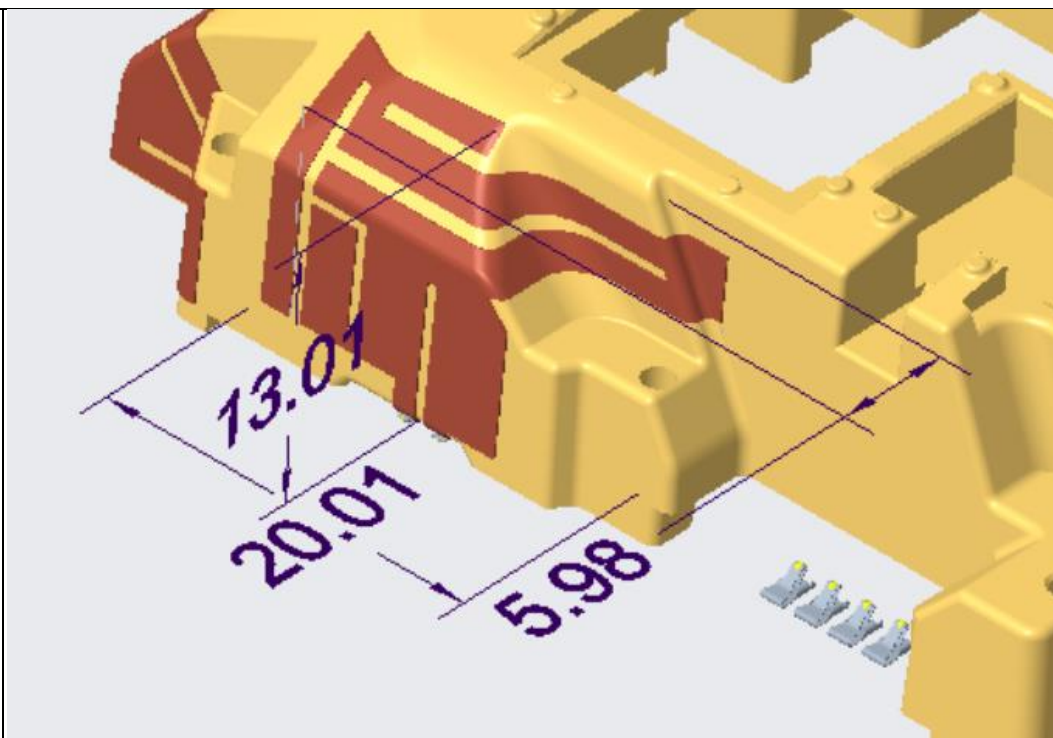
ANT7:20.01*13.01*5.98mm PIFA
