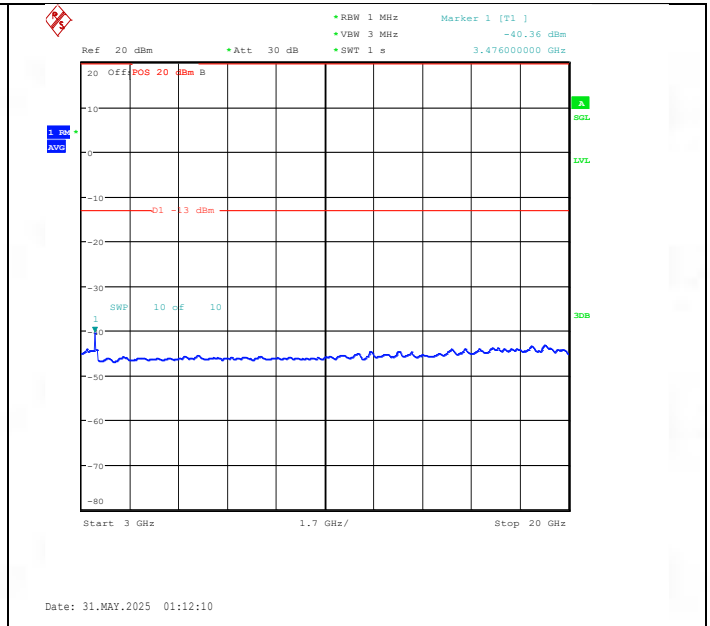
Band66-10MHz-16QAM-132322-1RB#0-3000~20000-PASS
