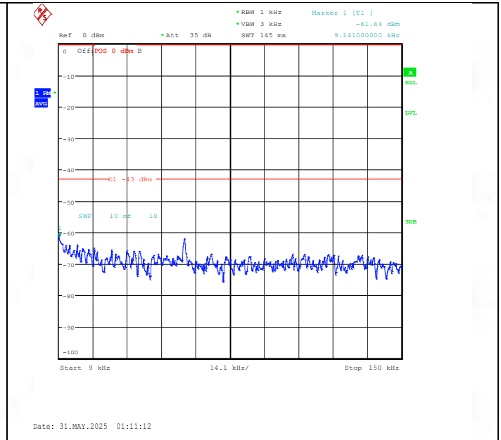
Band66-10MHz-16QAM-132322-1RB#0-0.009~0.15-PASS
