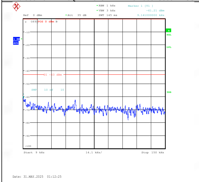
Band66-10MHz-QPSK-132622-1RB#0-0.009~0.15-PASS
