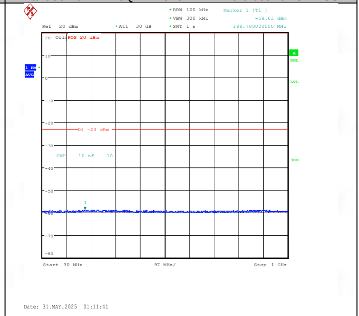
Band66-10MHz-16QAM-132322-1RB#0-30~1000-PASS
