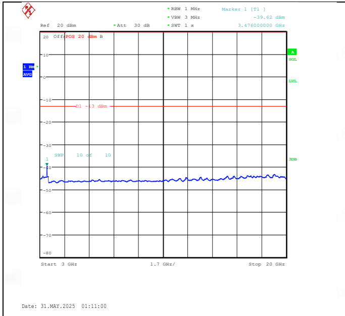
Band66-10MHz-QPSK-132322-1RB#0-3000~20000-PASS
