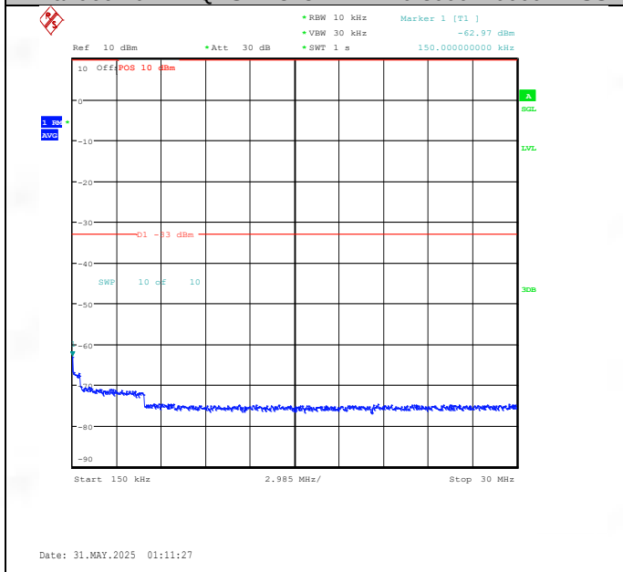
Band66-10MHz-16QAM-132322-1RB#0-0.15~30-PASS
