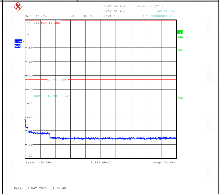
Band66-10MHz-QPSK-132622-1RB#0-0.15~30-PASS
