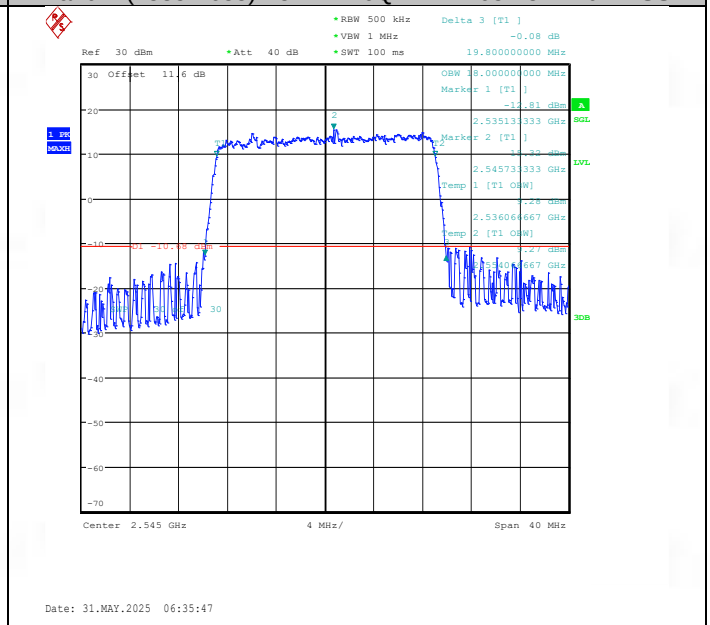
Band41(2535-2655)-20MHz-16QAM-40140-100RB#0-PASS
