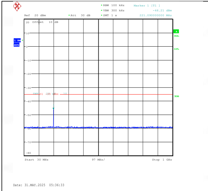
Band41(2535-2655)-10MHz-QPSK-40090-1RB#0-30~1000-PASS
