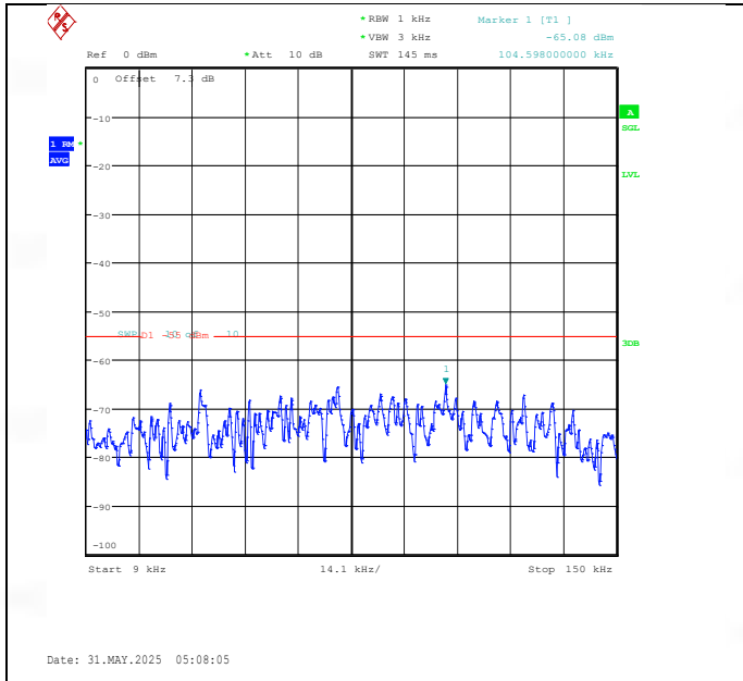
Band41(2535-2655)-5MHz-QPSK-41215-1RB#0-0.009~0.15-PASS
