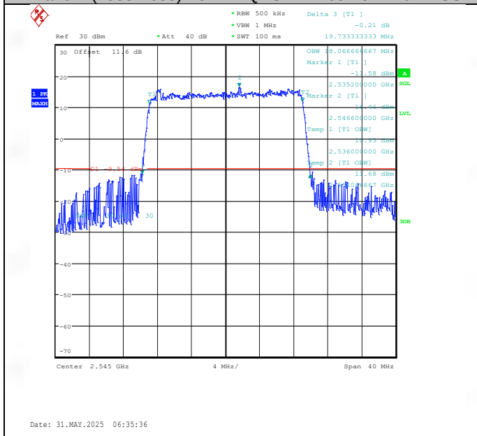
Band41(2535-2655)-20MHz-QPSK-40140-100RB#0-PASS
