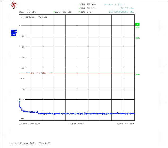
Band41(2535-2655)-5MHz-QPSK-41215-1RB#0-0.15~30-PASS
