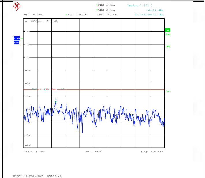
Band41(2535-2655)-10MHz-16QAM-40090-1RB#0-0.009~0.15-PASS
