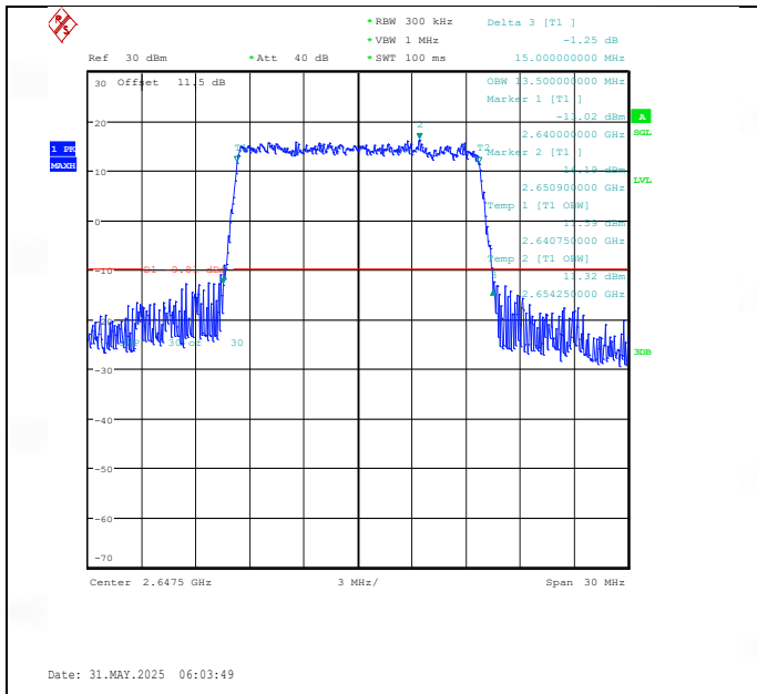
Band41(2535-2655)-15MHz-QPSK-41165-75RB#0-PASS
