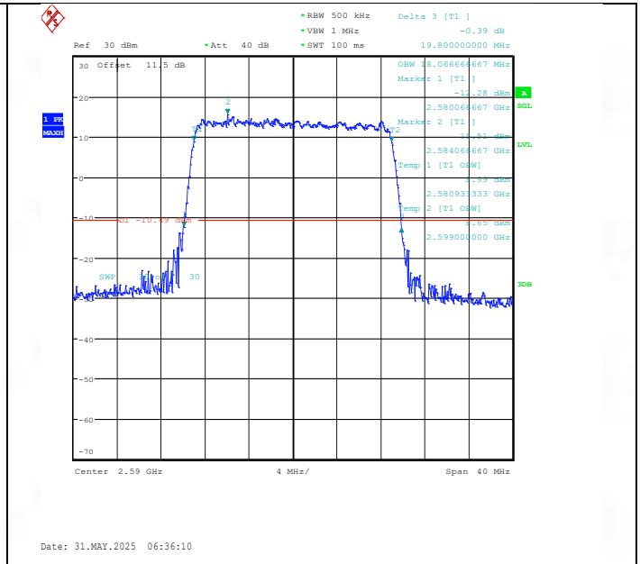
Band41(2535-2655)-20MHz-16QAM-40590-100RB#0-PASS
