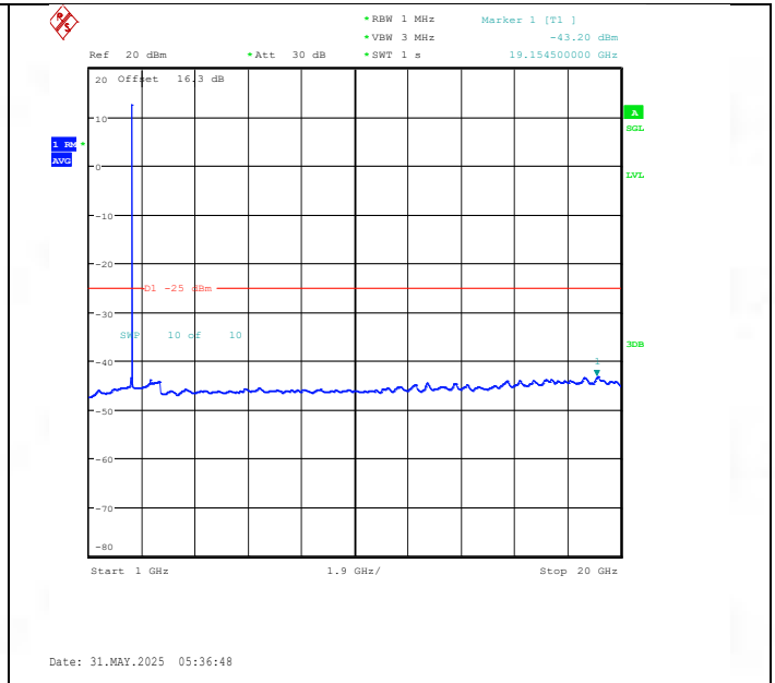
Band41(2535-2655)-10MHz-QPSK-40090-1RB#0-1000~20000-PASS
