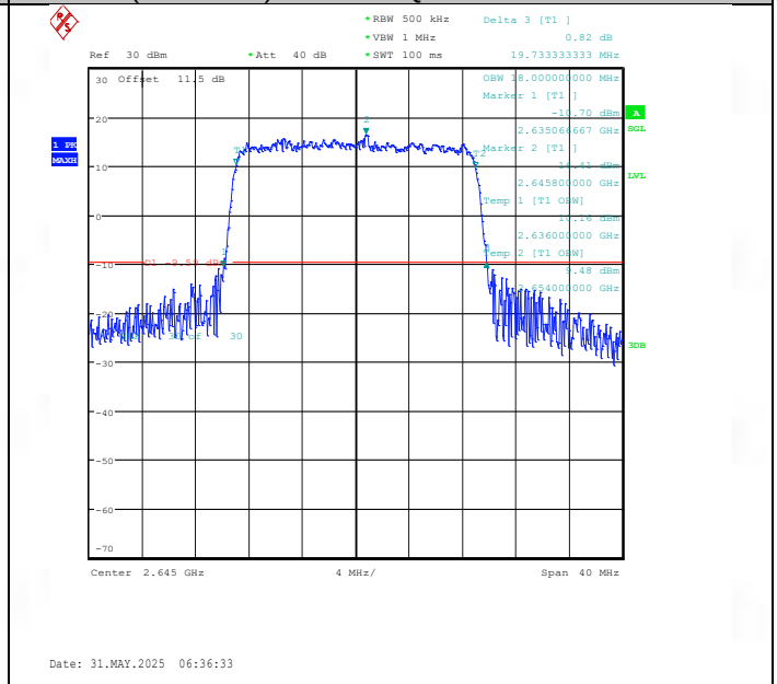
Band41(2535-2655)-20MHz-16QAM-41140-100RB#0-PASS
