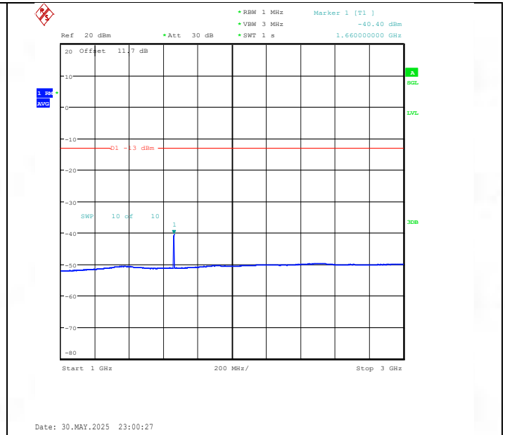
Band26(824-849)-15MHz-QPSK-26915-1RB#0-1000~3000-PASS
