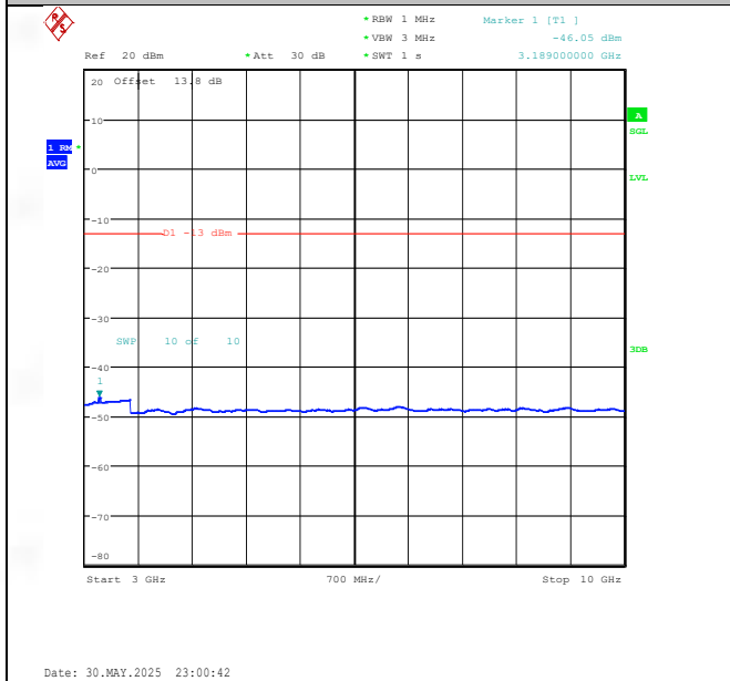
Band26(824-849)-15MHz-QPSK-26915-1RB#0-3000~10000-PASS
