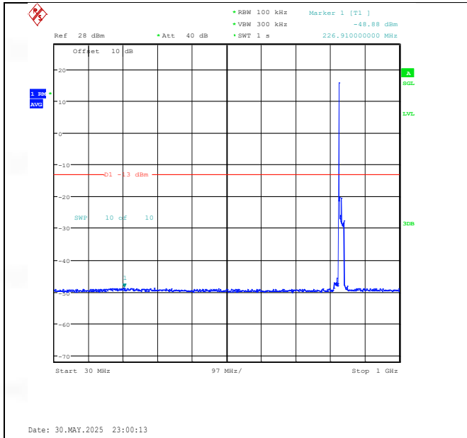
Band26(824-849)-15MHz-QPSK-26915-1RB#0-30~1000-PASS
