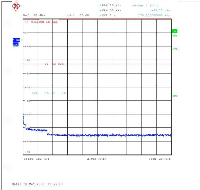
Band26(824-849)-3MHz-16QAM-27025-1RB#0-0.15~30-PASS
