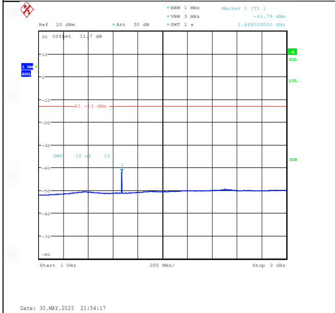
Band26(824-849)-5MHz-16QAM-26915-1RB#0-1000~3000-PASS
