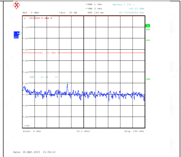
Band26(824-849)-5MHz-16QAM-27015-1RB#0-0.009~0.15-PASS
