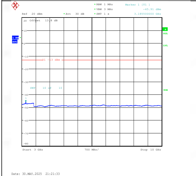
Band26(824-849)-3MHz-QPSK-27025-1RB#0-3000~10000-PASS
