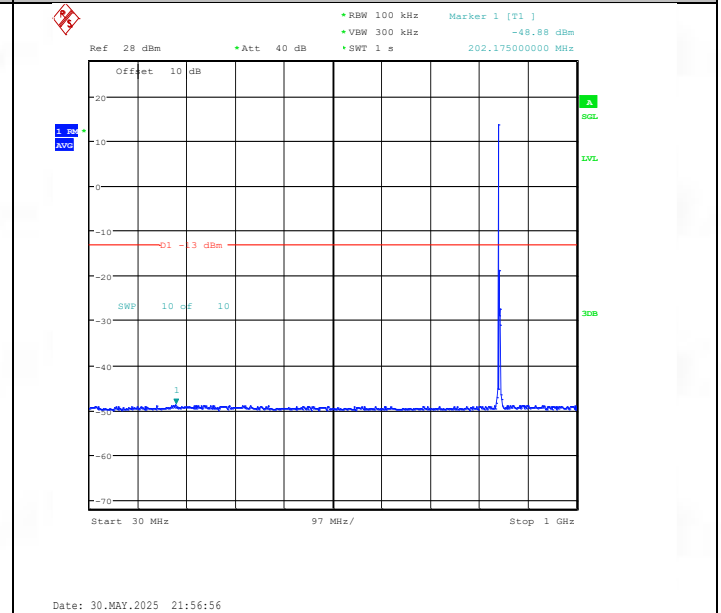
Band26(824-849)-5MHz-16QAM-27015-1RB#0-30~1000-PASS
