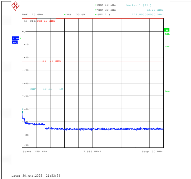
Band26(824-849)-5MHz-16QAM-26915-1RB#0-0.15~30-PASS
