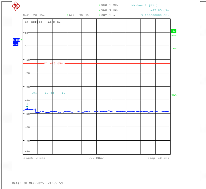
Band26(824-849)-5MHz-QPSK-27015-1RB#0-3000~10000-PASS
