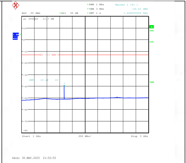
Band26(824-849)-5MHz-QPSK-26915-1RB#0-1000~3000-PASS
