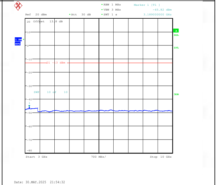
Band26(824-849)-5MHz-16QAM-26915-1RB#0-3000~10000-PASS
