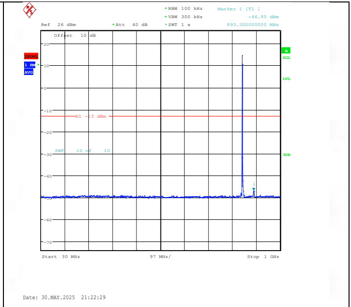
Band26(824-849)-3MHz-16QAM-27025-1RB#0-30~1000-PASS
