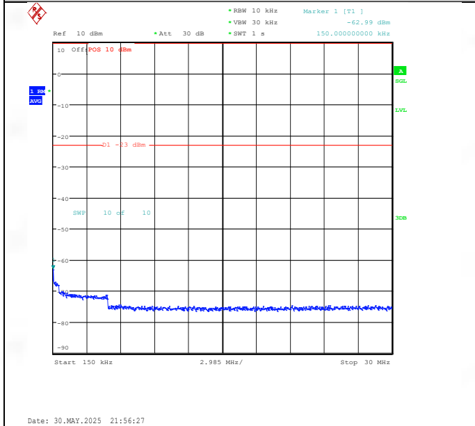
Band26(824-849)-5MHz-16QAM-27015-1RB#0-0.15~30-PASS
