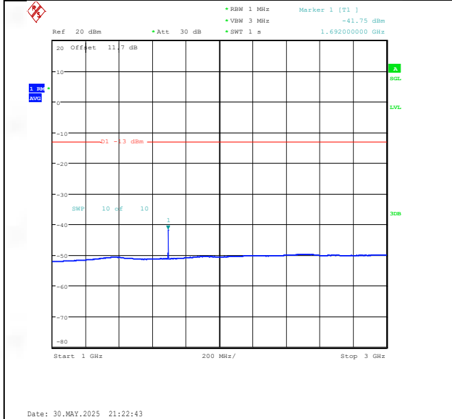
Band26(824-849)-3MHz-16QAM-27025-1RB#0-1000~3000-PASS
