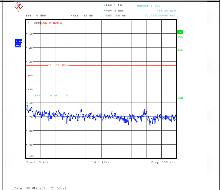
Band26(824-849)-5MHz-16QAM-26915-1RB#0-0.009~0.15-PASS
