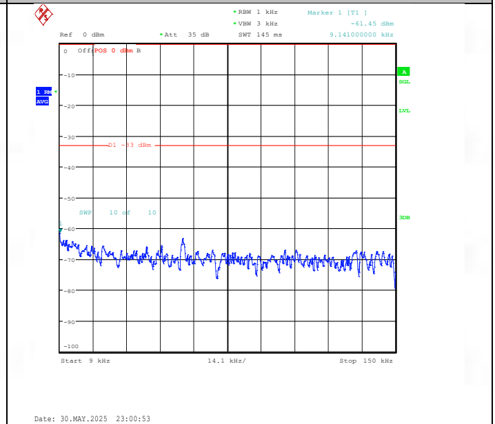
Band26(824-849)-15MHz-16QAM-26915-1RB#0-0.009~0.15-PASS
