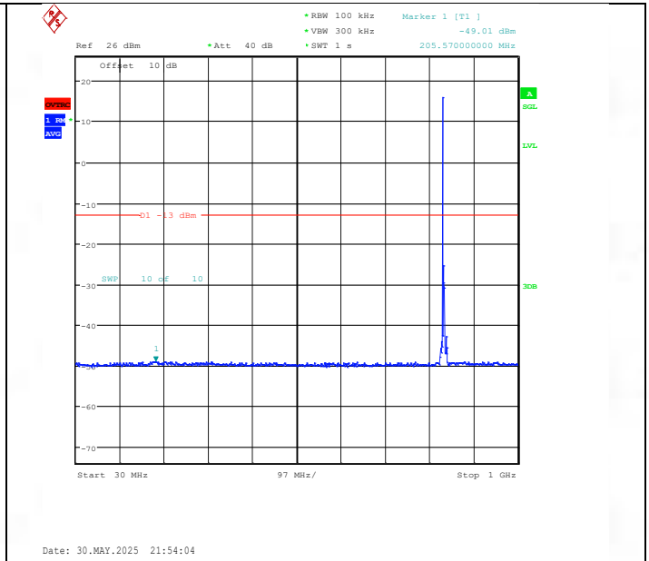
Band26(824-849)-5MHz-16QAM-26915-1RB#0-30~1000-PASS
