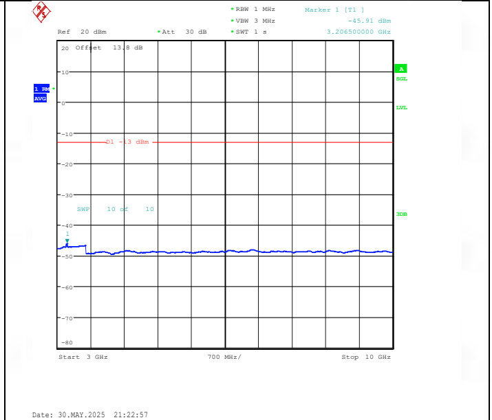
Band26(824-849)-3MHz-16QAM-27025-1RB#0-3000~10000-PASS
