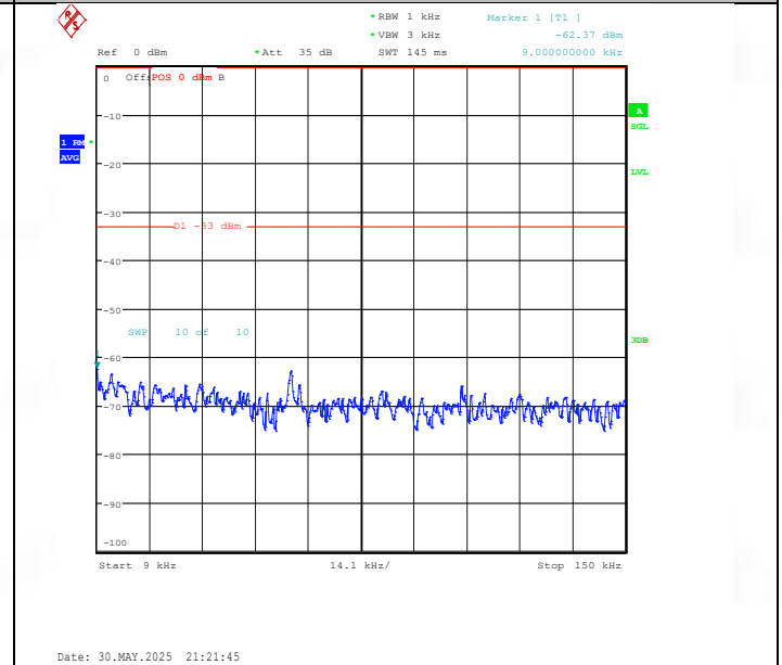
Band26(824-849)-3MHz-16QAM-27025-1RB#0-0.009~0.15-PASS
