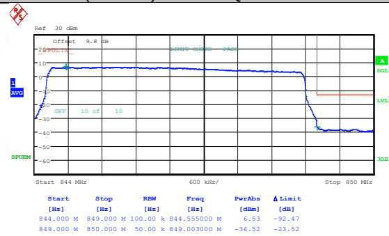
Band26(824-849)-5MHz-16QAM-27015-1RB#0-PASS
