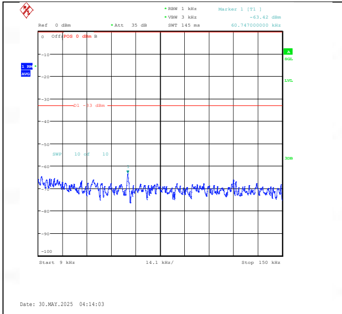
Band26(824-849)-1.4MHz-QPSK-27033-1RB#0-0.009~0.15-PASS
