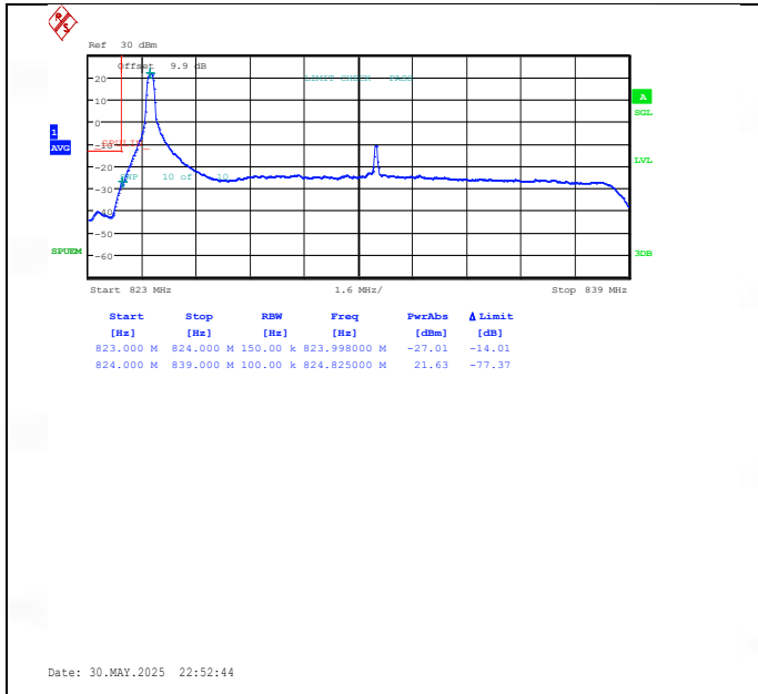
Band26(824-849)-15MHz-QPSK-26865-1RB#0-PASS
