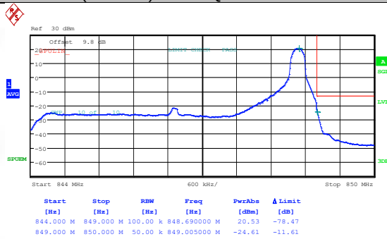
Band26(824-849)-5MHz-QPSK-27015-25RB#0-PASS
