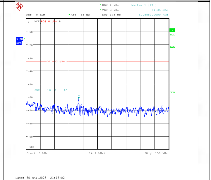
Band26(824-849)-3MHz-16QAM-26805-1RB#0-0.009~0.15-PASS
