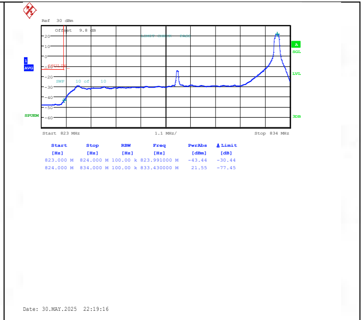
Band26(824-849)-10MHz-QPSK-26840-1RB#49-PASS
