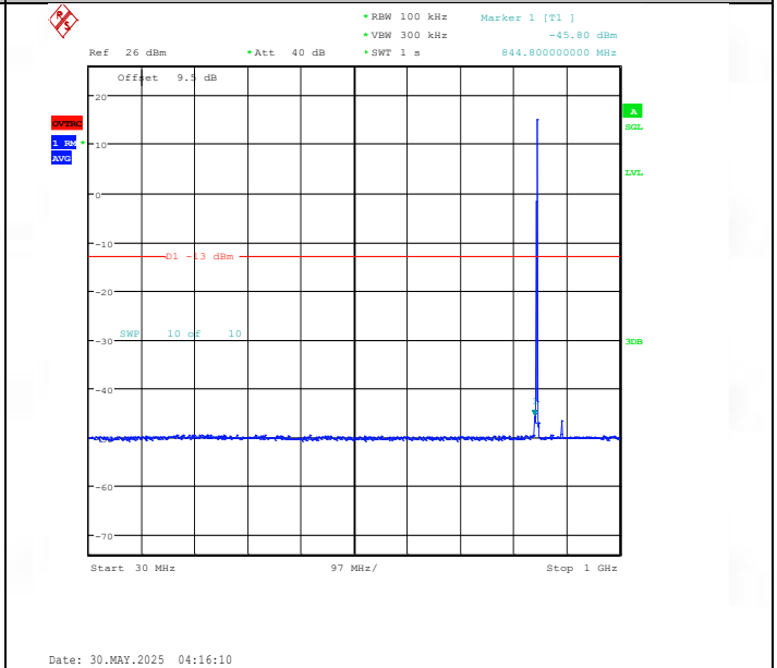
Band26(824-849)-1.4MHz-16QAM-27033-1RB#0-30~1000-PASS
