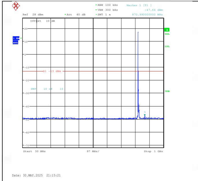
Band26(824-849)-3MHz-QPSK-26805-1RB#0-30~1000-PASS
