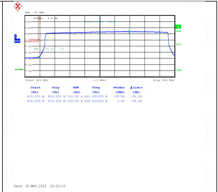
Band26(824-849)-10MHz-16QAM-26840-50RB#0-PASS
