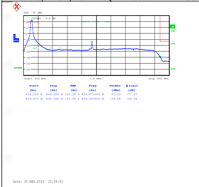
Band26(824-849)-15MHz-QPSK-26965-1RB#0-PASS
