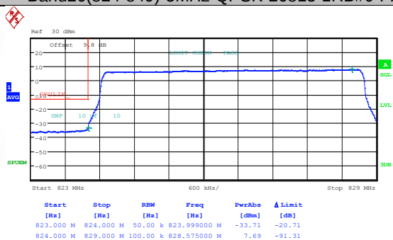
Band26(824-849)-5MHz-OPSK-26815-1RB#0-PASS
