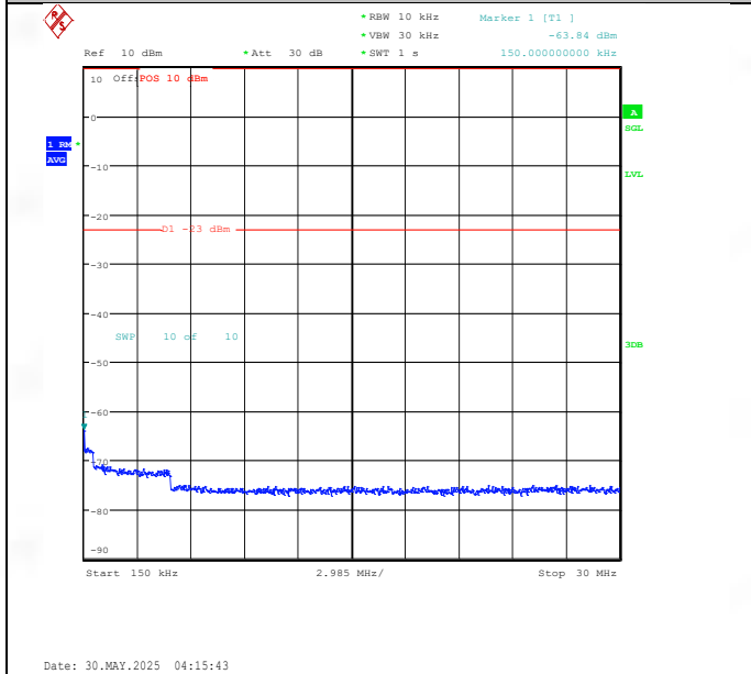
Band26(824-849)-1.4MHz-16QAM-27033-1RB#0-0.15~30-PASS
