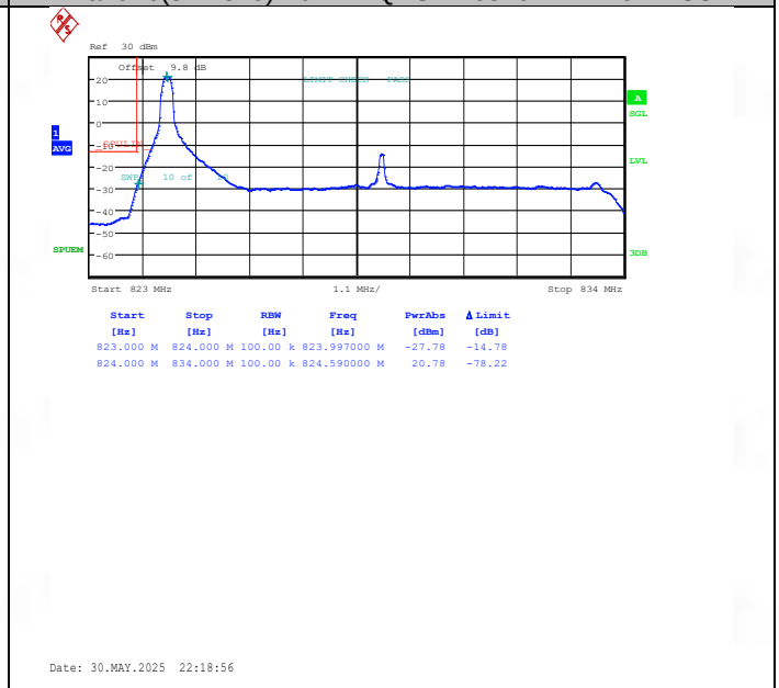
Band26(824-849)-10MHz-16QAM-26840-1RB#0-PASS
