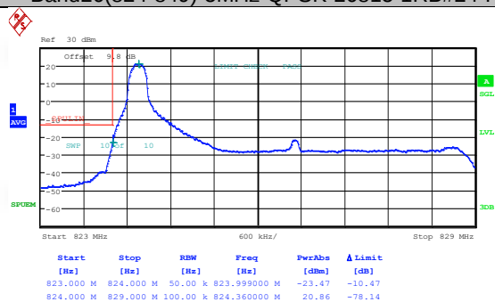
Band26(824-849)-5MHz-OPSK-26815-1RB#24-PASS
