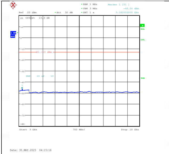
Band26(824-849)-1.4MHz-QPSK-27033-1RB#0-3000~10000-PASS
