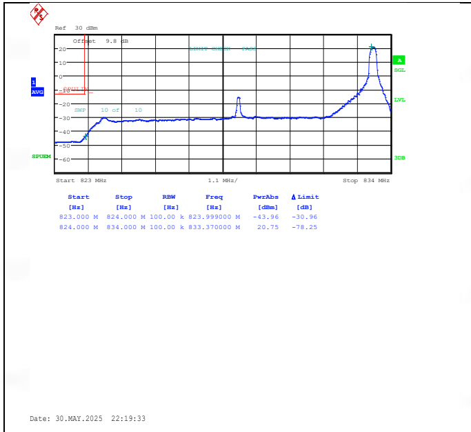
Band26(824-849)-10MHz-16QAM-26840-1RB#49-PASS
