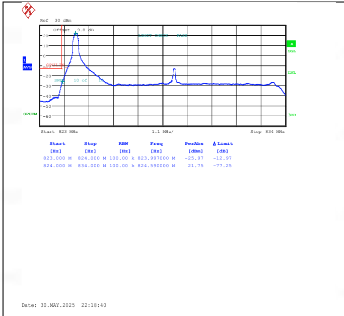
Band26(824-849)-10MHz-QPSK-26840-1RB#0-PASS
