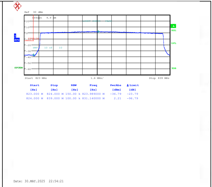
Band26(824-849)-15MHz-16QAM-26865-75RB#0-PASS
