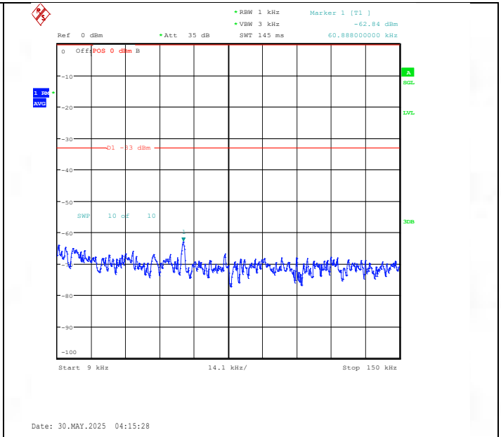
Band26(824-849)-1.4MHz-16QAM-27033-1RB#0-0.009~0.15-PASS
