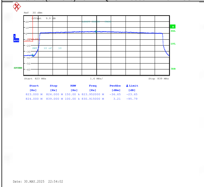
Band26(824-849)-15MHz-QPSK-26865-75RB#0-PASS
