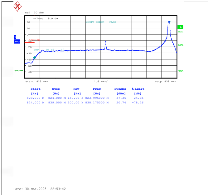
Band26(824-849)-15MHz-16QAM-26865-1RB#74-PASS
