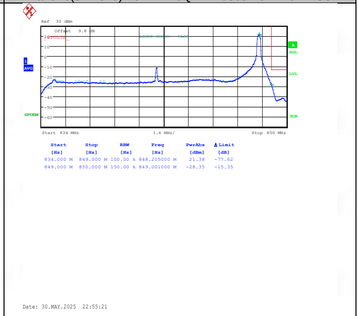
Band26(824-849)-15MHz-QPSK-26965-1RB#74-PASS
