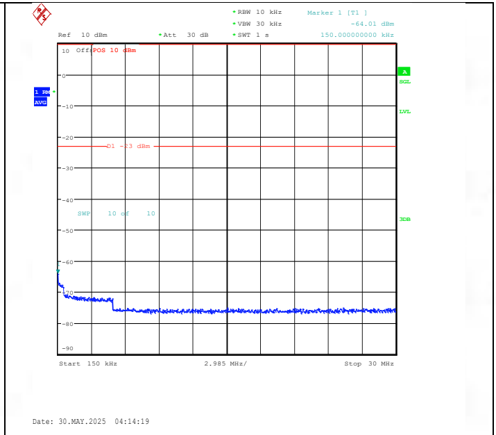
Band26(824-849)-1.4MHz-QPSK-27033-1RB#0-0.15~30-PASS
