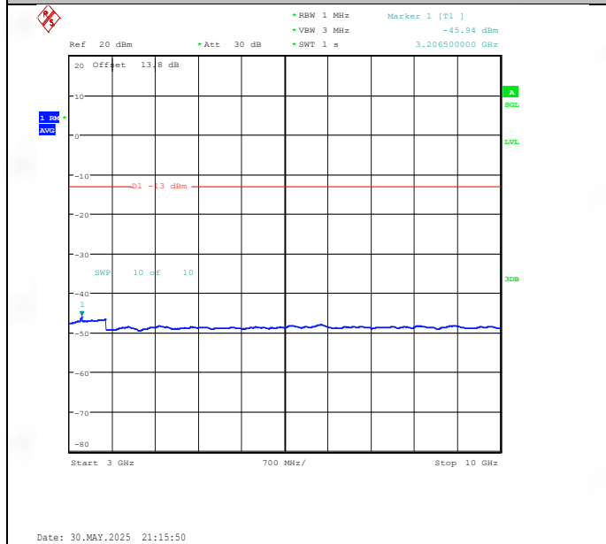
Band26(824-849)-3MHz-QPSK-26805-1RB#0-3000~10000-PASS
