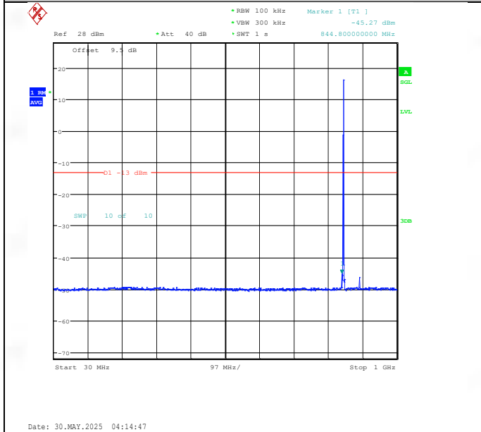
Band26(824-849)-1.4MHz-QPSK-27033-1RB#0-30~1000-PASS
