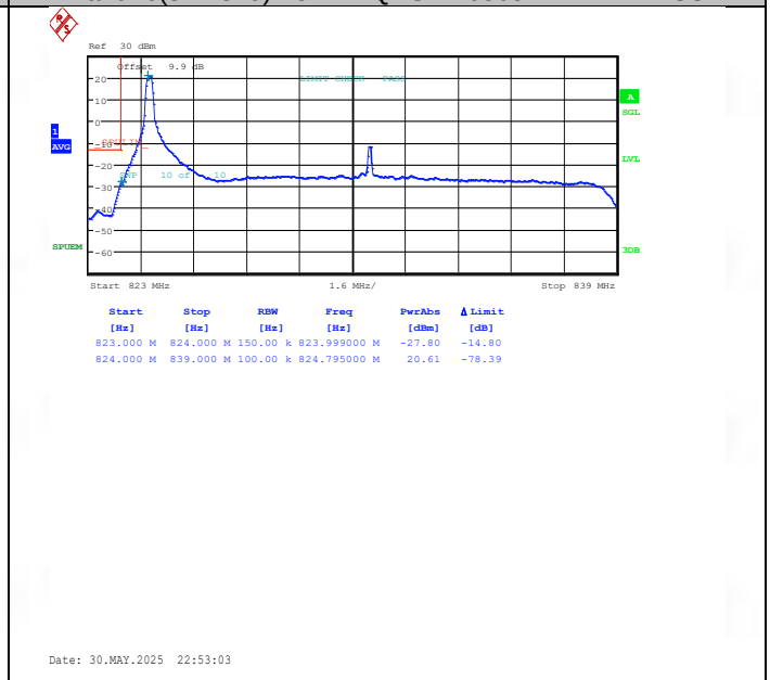
Band26(824-849)-15MHz-16QAM-26865-1RB#0-PASS
