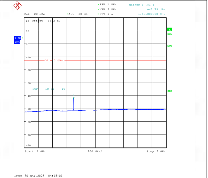
Band26(824-849)-1.4MHz-QPSK-27033-1RB#0-1000~3000-PASS
