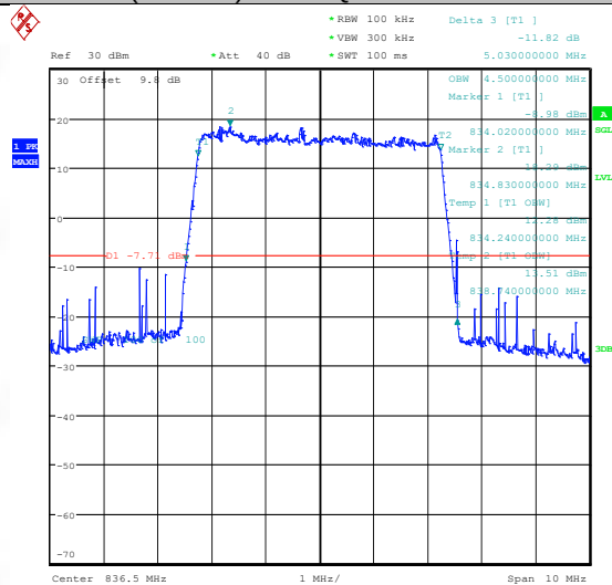
Band26(824-849)-5MHz-QPSK-26815-25RB#0-PASS
