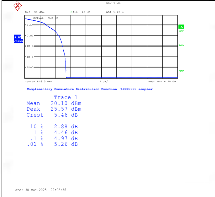
Band26(824-849)-5MHz-16QAM-27015-1RB#0-PASS
