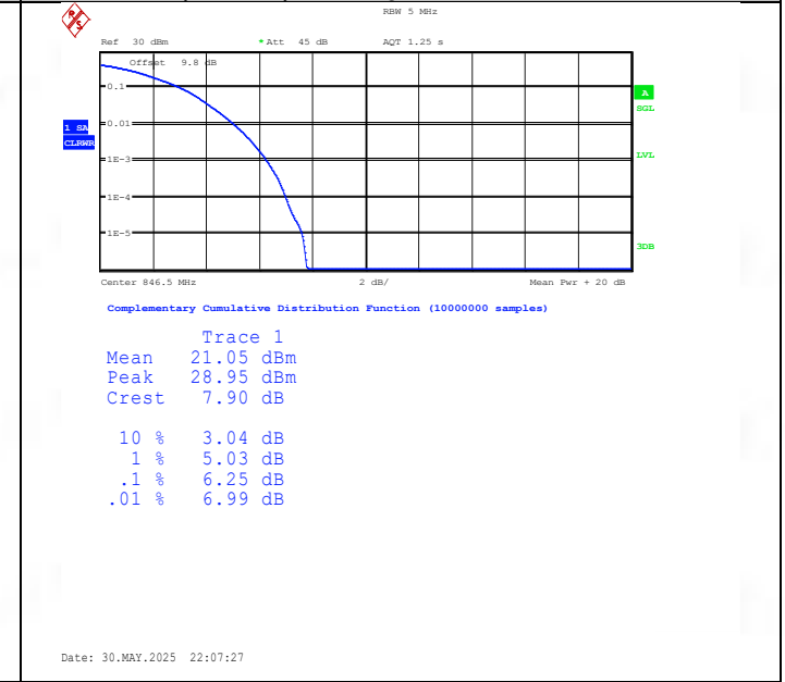
Band26(824-849)-5MHz-16QAM-27015-25RB#0-PASS
