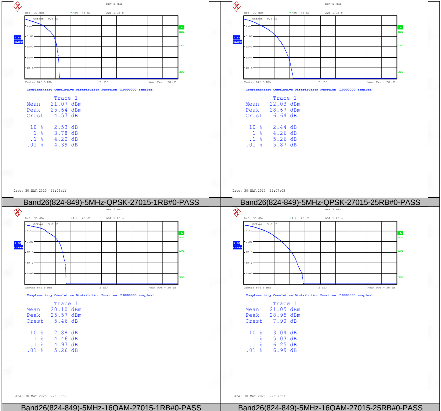
Band26(824-849)-5MHz-16QAM-27015-1RB#0-PASS
