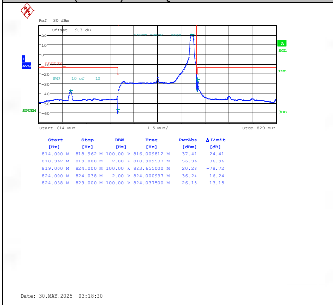
Band26(814-824)-5MHz-16QAM-26765-1RB#24-PASS
