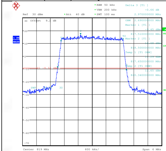
Band26(814-824)-3MHz-QPSK-26705-15RB#0-PASS
