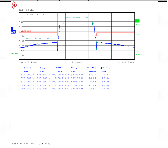
Band26(814-824)-5MHz-16QAM-26765-25RB#0-PASS
