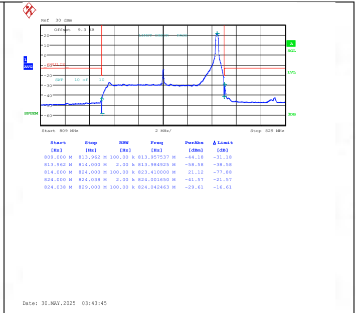
Band26(814-824)-10MHz-QPSK-26740-1RB#49-PASS
