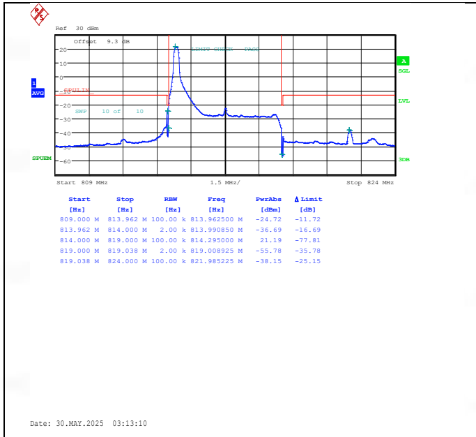
Band26(814-824)-5MHz-QPSK-26715-1RB#0-PASS
