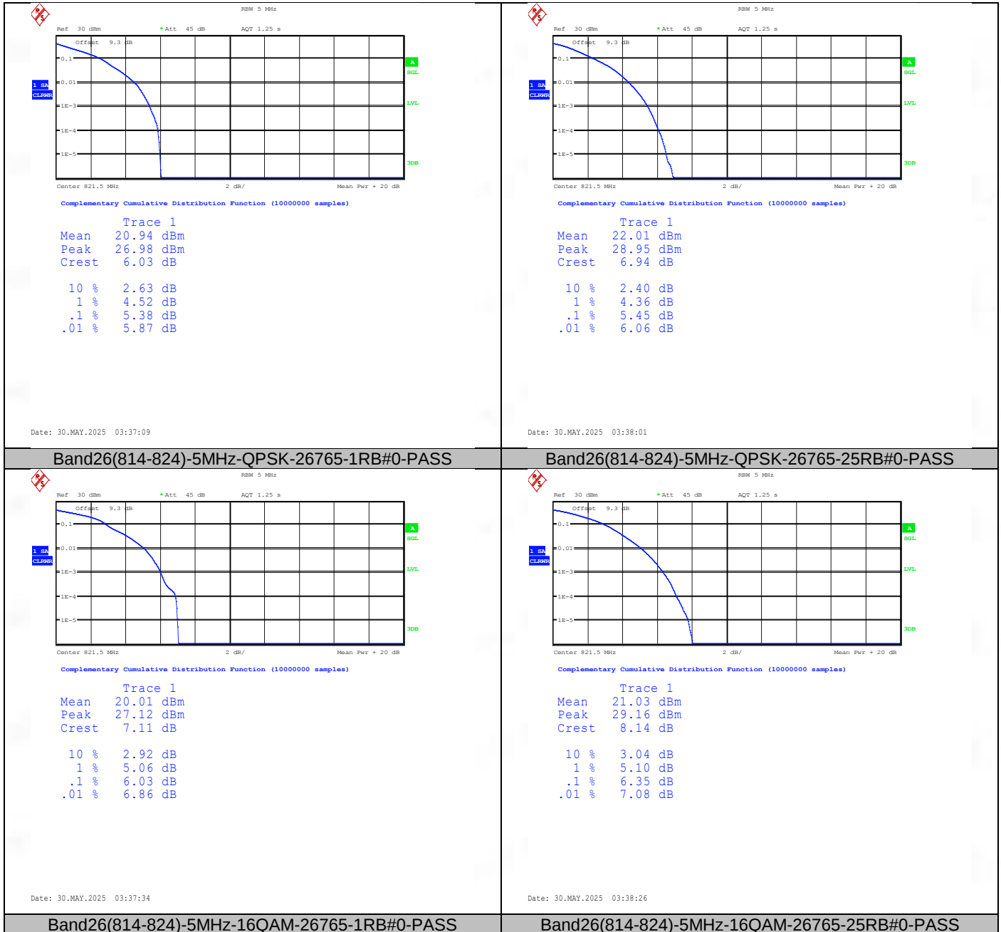
Band26(814-824)-5MHz-16QAM-26765-1RB#0-PASS
