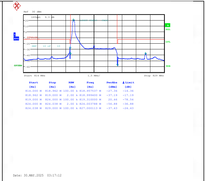
Band26(814-824)-5MHz-16QAM-26765-1RB#0-PASS
