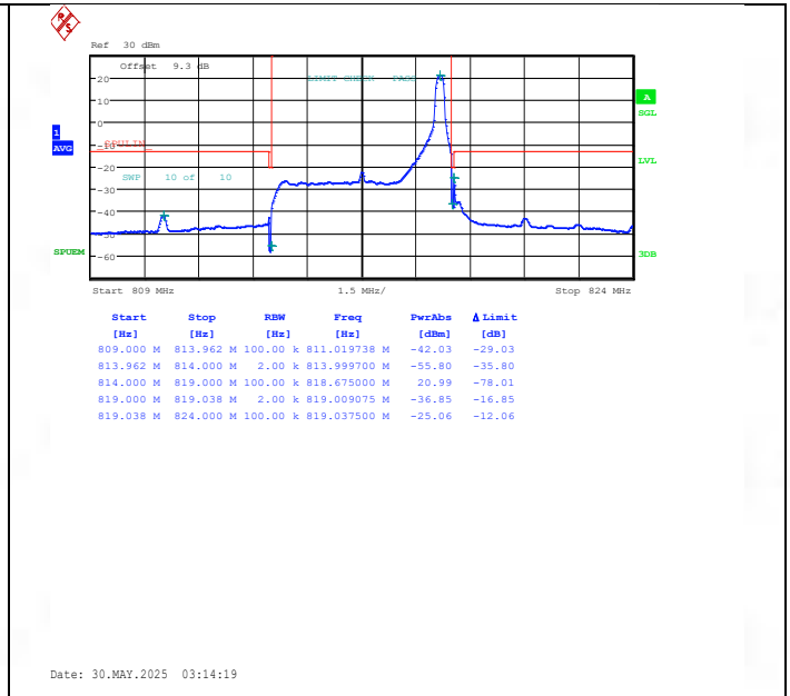
Band26(814-824)-5MHz-QPSK-26715-1RB#24-PASS
