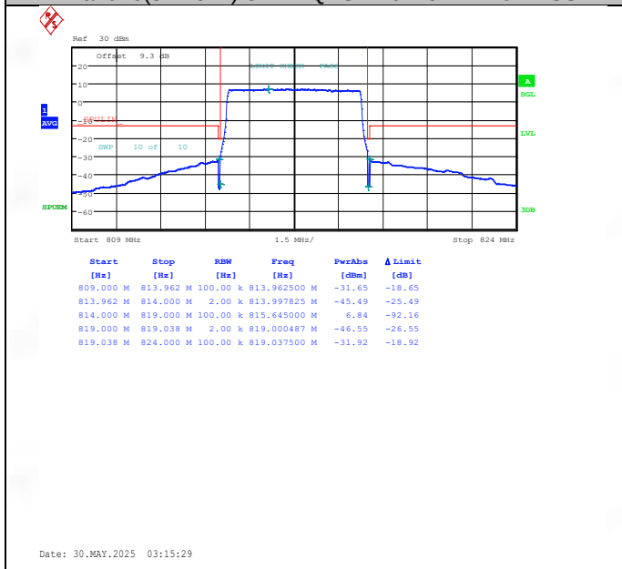
Band26(814-824)-5MHz-QPSK-26715-25RB#0-PASS
