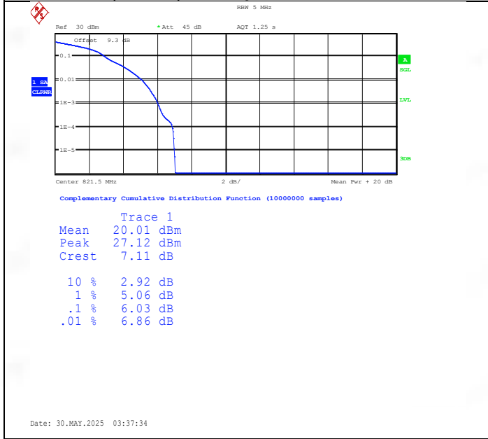
Band26(814-824)-5MHz-16QAM-26765-1RB#0-PASS
