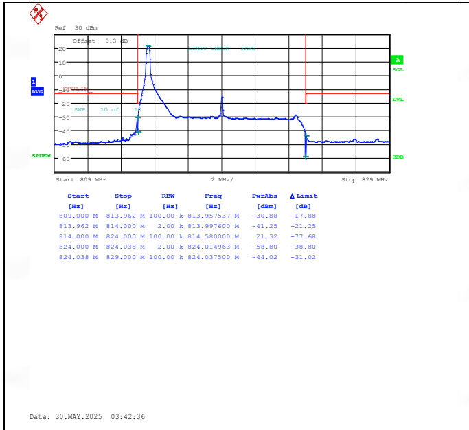
Band26(814-824)-10MHz-QPSK-26740-1RB#0-PASS
