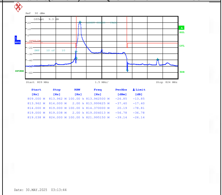
Band26(814-824)-5MHz-16QAM-26715-1RB#0-PASS
