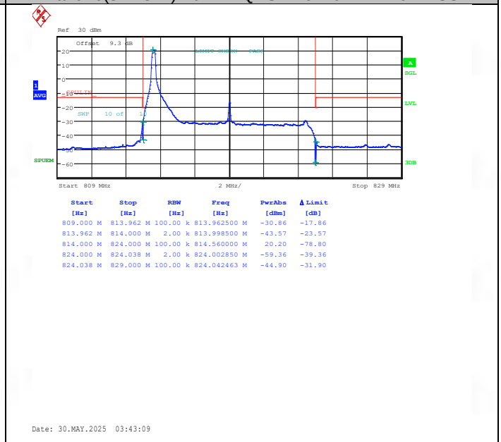
Band26(814-824)-10MHz-16QAM-26740-1RB#0-PASS
