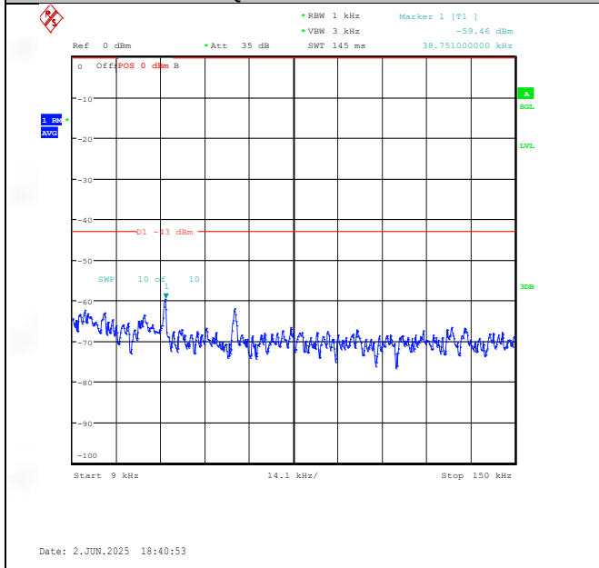
Band25-20MHz-QPSK-26590-1RB#0-0.009-0.15-PASS
