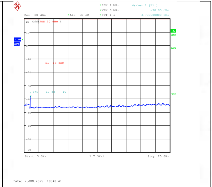
Band25-20MHz-16QAM-26365-1RB#0-3000-20000-PASS
