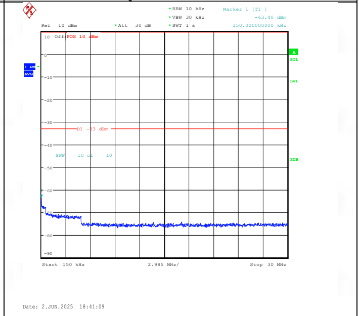
Band25-20MHz-QPSK-26590-1RB#0-0.15-30-PASS
