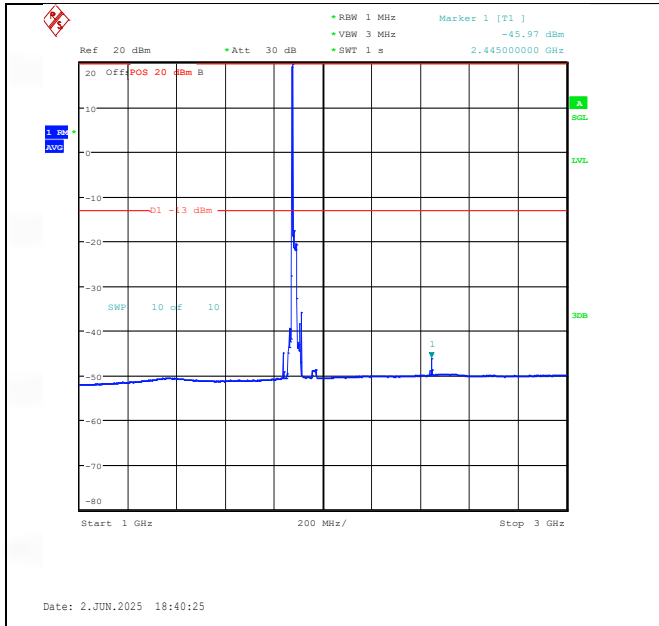
Band25-20MHz-16QAM-26365-1RB#0-1000-3000-PASS
