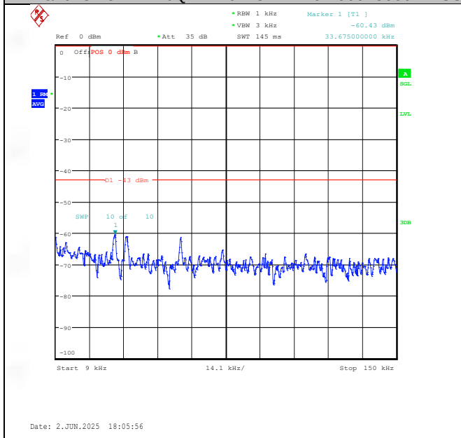
Band25-15MHz-QPSK-26365-1RB#0-0.009~0.15-PASS
