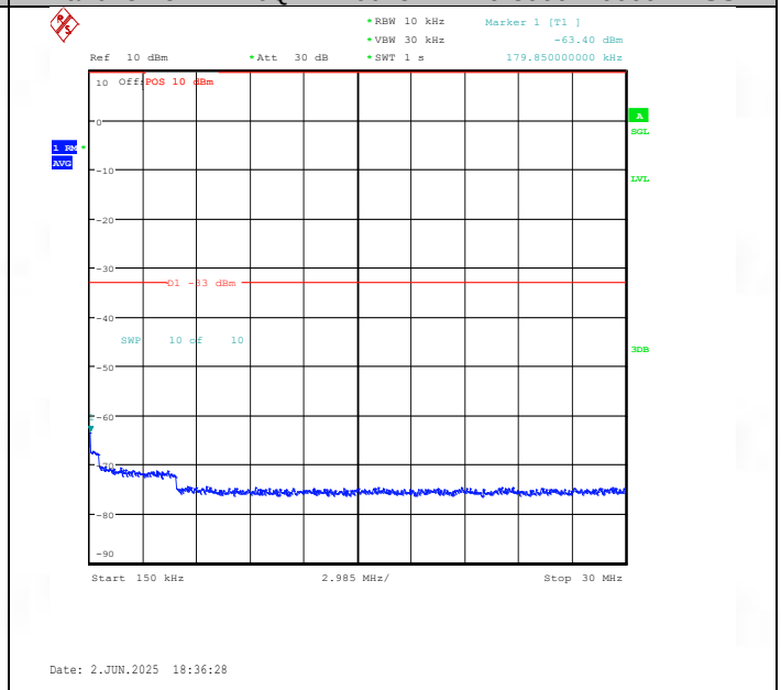
Band25-20MHz-QPSK-26140-1RB#0-0.15~30-PASS
