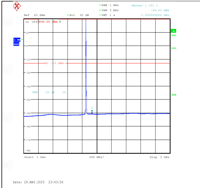
Band25-5MHz-16QAM-26065-1RB#0-1000~3000-PASS
