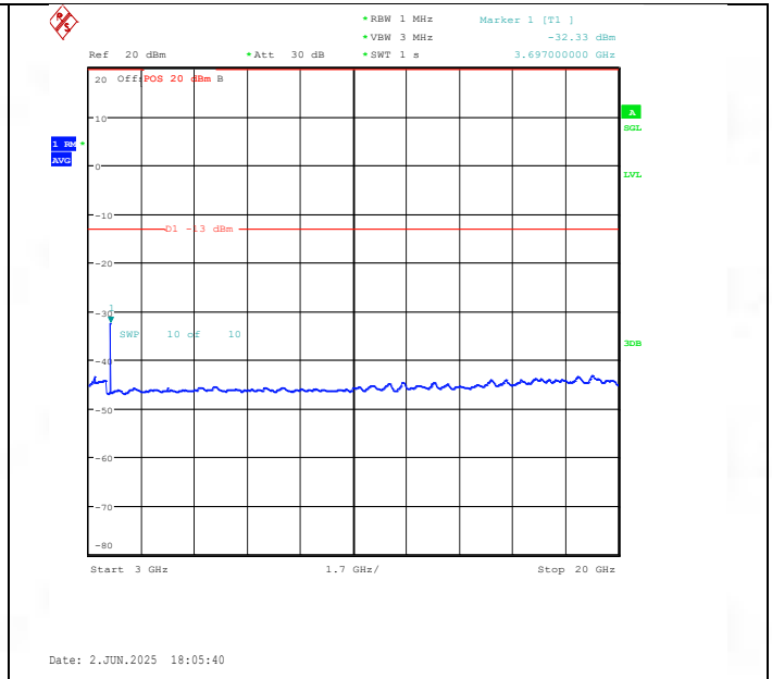
Band25-15MHz-16QAM-26115-1RB#0-3000~20000-PASS
