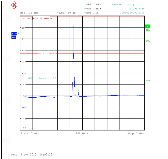
Band25-15MHz-16QAM-26115-1RB#0-1000~3000-PASS
