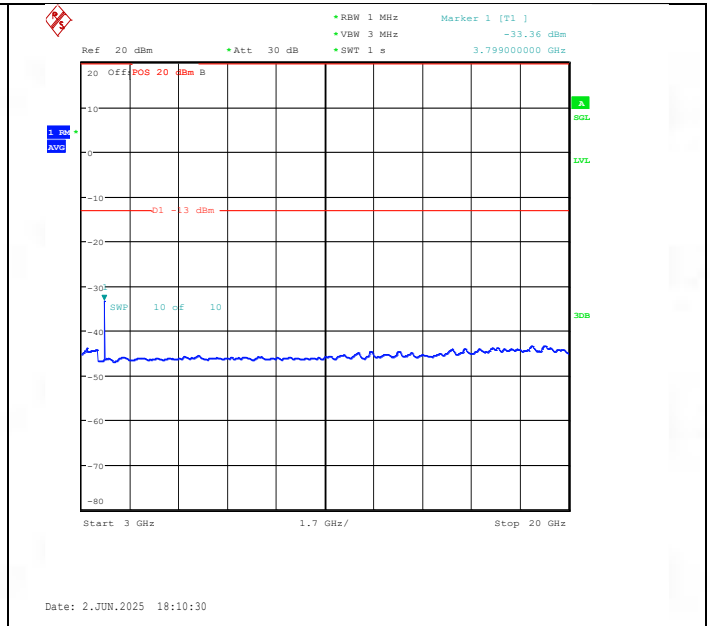
Band25-15MHz-16QAM-26615-1RB#0-3000~20000-PASS
