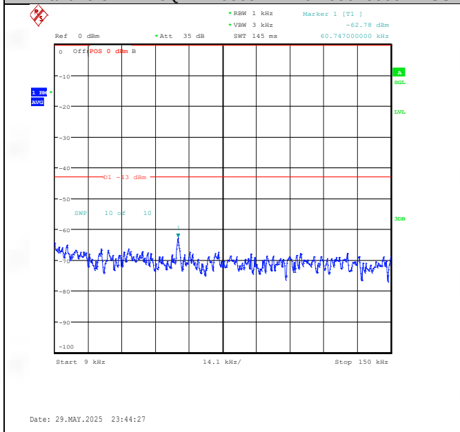
Band25-5MHz-QPSK-26365-1RB#0-0.009~0.15-PASS
