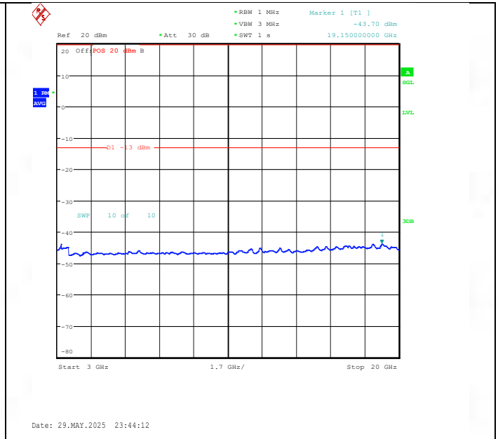
Band25-5MHz-16QAM-26065-1RB#0-3000~20000-PASS
