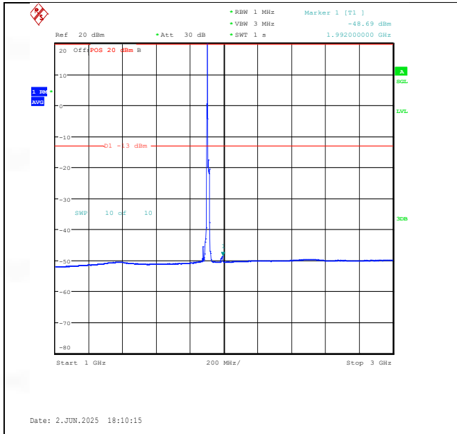
Band25-15MHz-16QAM-26615-1RB#0-1000~3000-PASS
