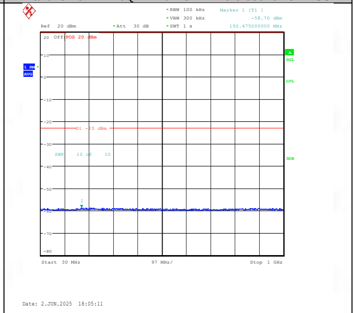
Band25-15MHz-16QAM-26115-1RB#0-30~1000-PASS
