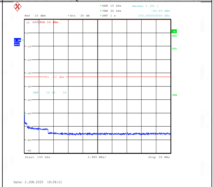
Band25-15MHz-QPSK-26365-1RB#0-0.15~30-PASS
