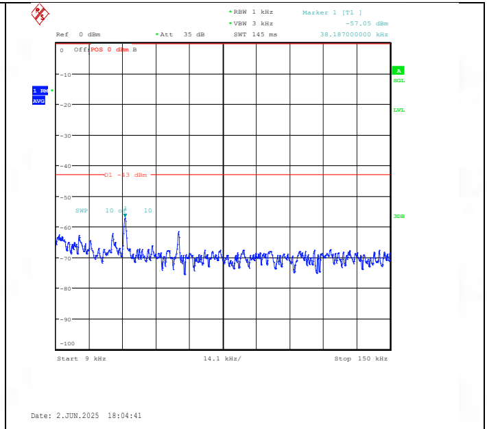
Band25-15MHz-16QAM-26115-1RB#0-0.009~0.15-PASS
