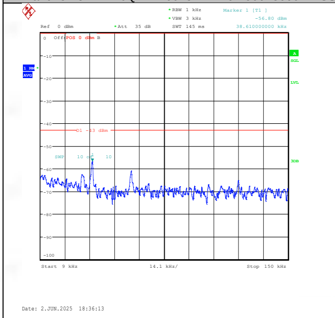
Band25-20MHz-QPSK-26140-1RB#0-0.009~0.15-PASS
