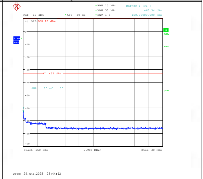
Band25-5MHz-QPSK-26365-1RB#0-0.15~30-PASS
