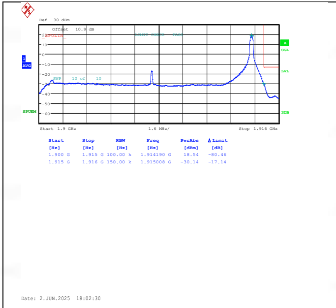
Band25-15MHz-16QAM-26615-1RB#74-PASS
