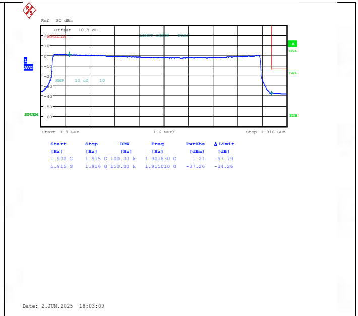
Band25-15MHz-16QAM-26615-75RB#0-PASS
