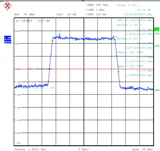
Band25-15MHz-16QAM-26115-75RB#0-PASS
