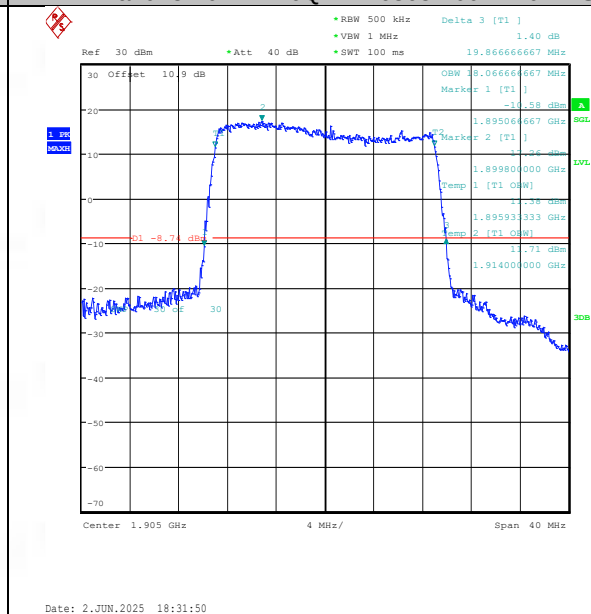
Band25-20MHz-16QAM-26590-100RB#0-PASS
