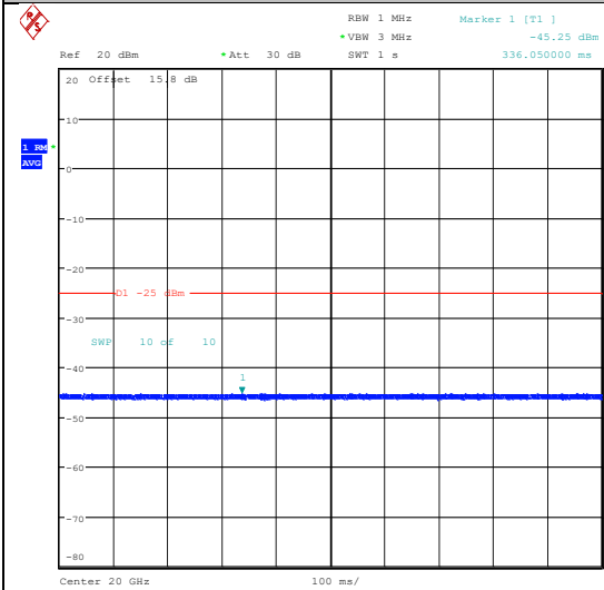
Band41(2535-2655)-5MHz-QPSK-40590-1RB#0-3 0~1000-PASS
