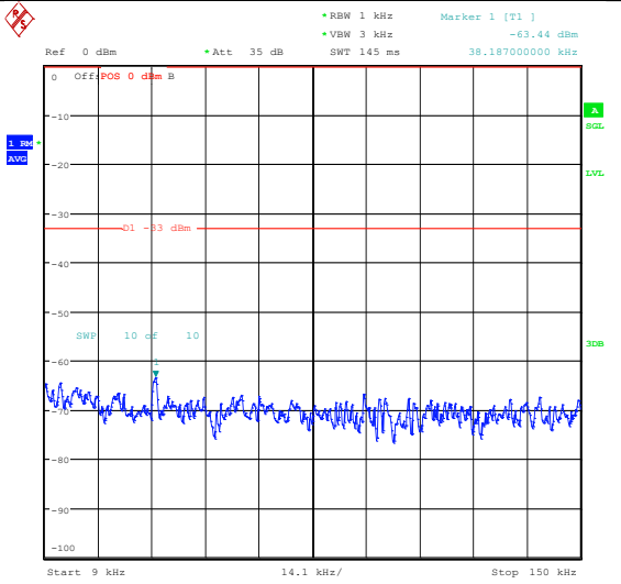
Band26(824-849)-1.4MHz-QPSK-26915-1RB#0-10 00~3000-PASS
