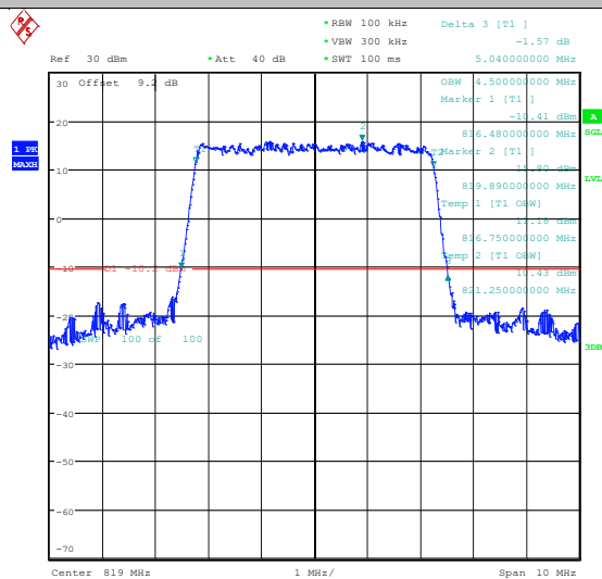
Band26(814-824)-5MHz-16QAM-26715-25RB#0-P
