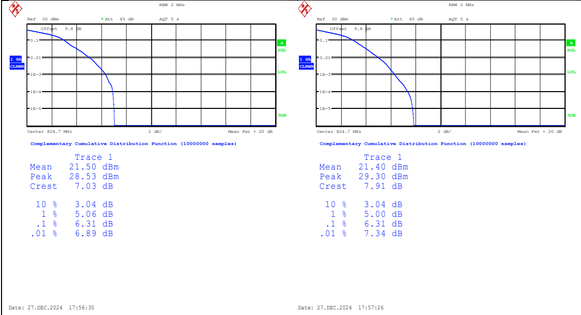
Band26(824-849)-1.4MHz-16QAM-26797-1RB#0-P PASS Band26(824-849)-1.4MHz-16QAM-26797-6RB#0-P PASS
