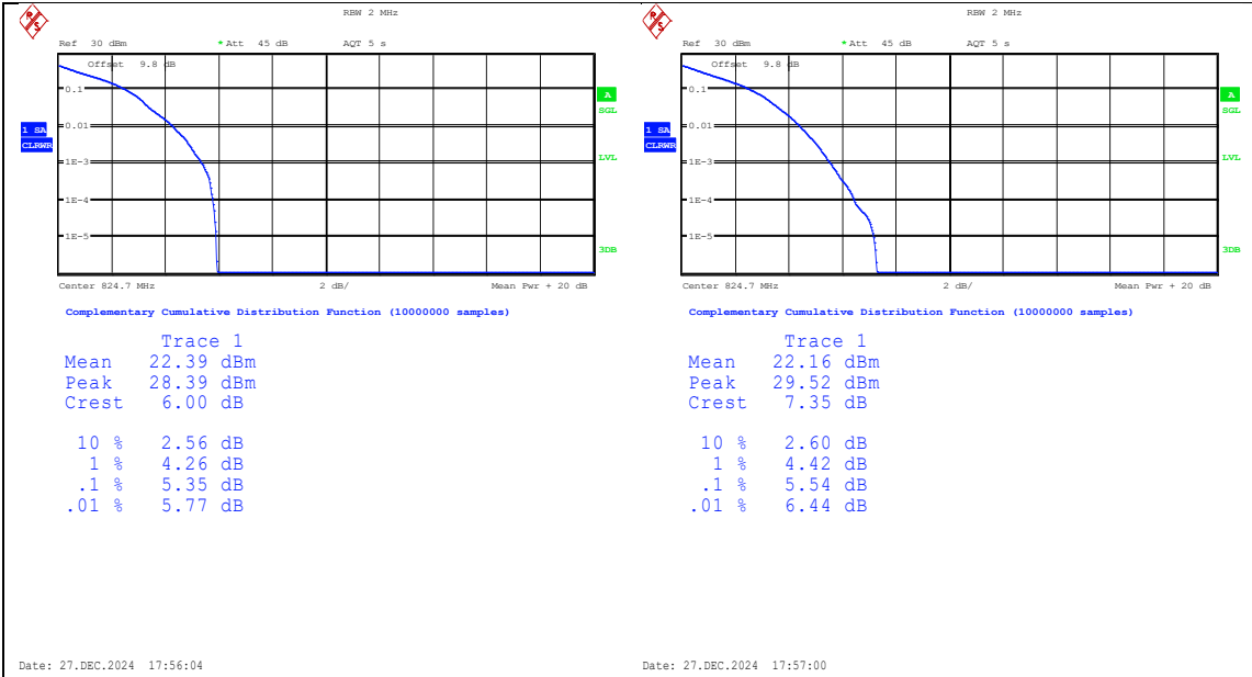
Band26(824-849)-1.4MHz-QPSK-26797-1RB#0-P ASS Band26(824-849)-1.4MHz-QPSK-26797-6RB#0-P ASS
