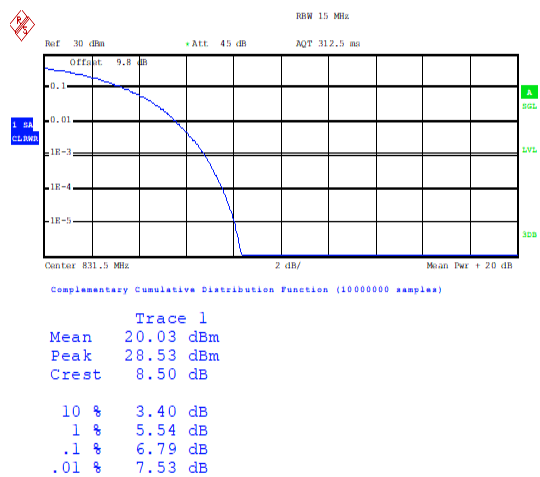
Band26(824-849)-15MHz-QPSK-26865-75RB#0-P ASS
