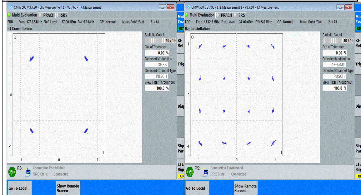
Band4-5MHz-QPSK-20175-25RB#0-PASS
