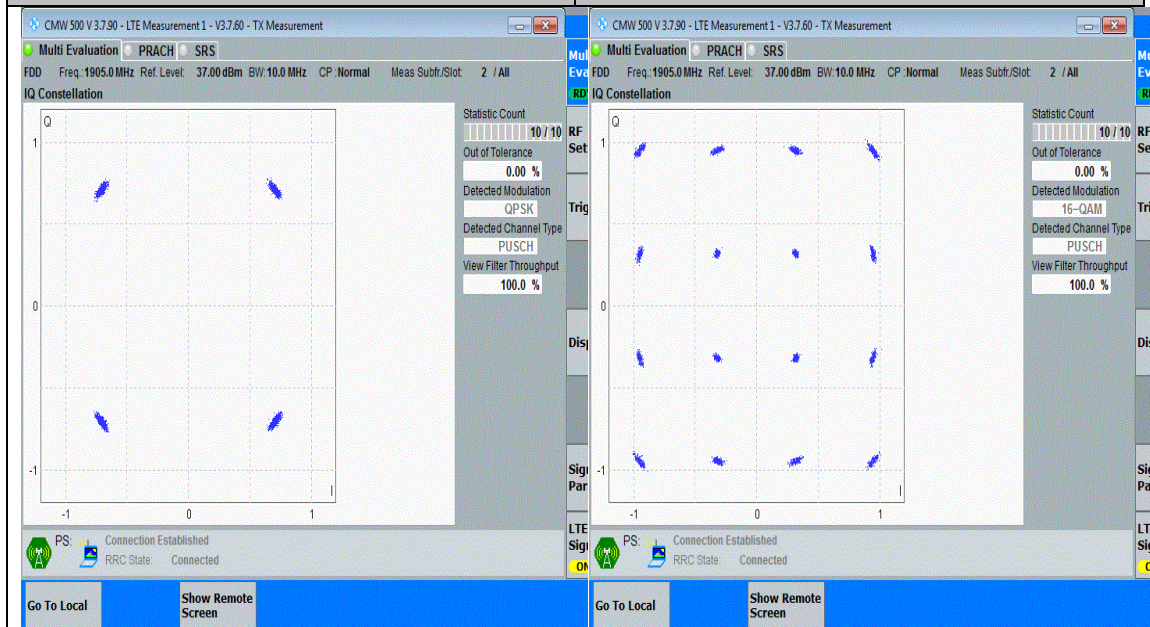
Band2-10MHz-QPSK-19150-50RB#0-PASS
