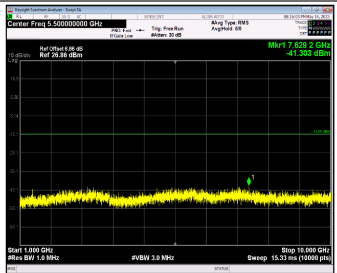
Band5-10MHz-16QAM-20525-1RB#0-Range2:1000~ 10000MHz
