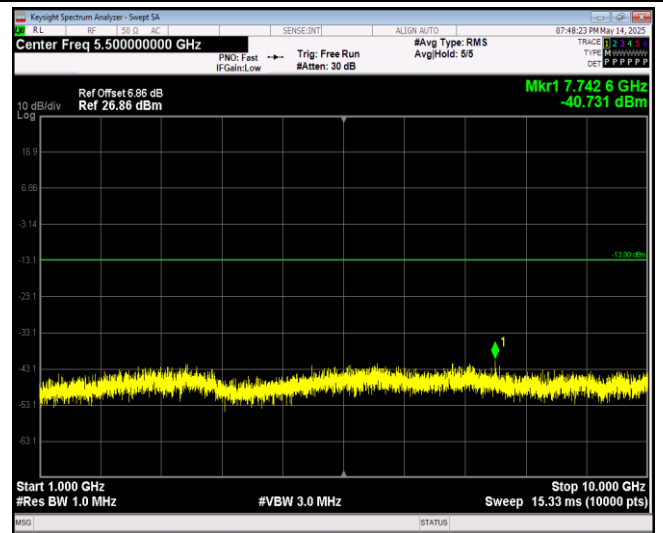
Band5-1.4MHz-QPSK-20643-1RB#0-Range2:1000~1 0000MHz
