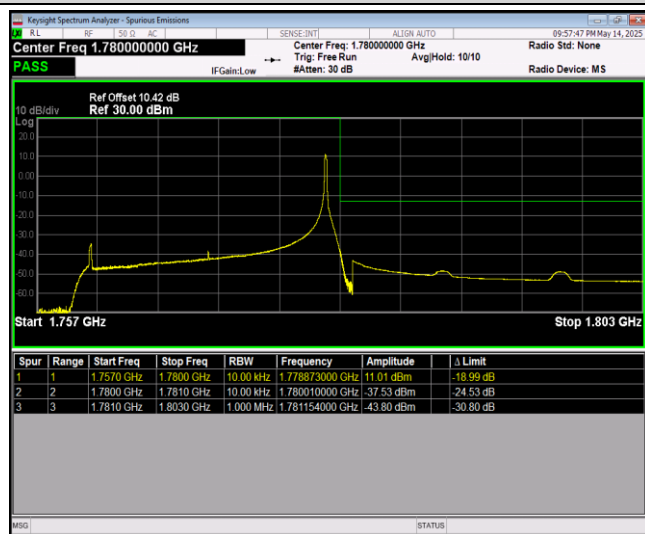
Band66-20MHz-16QAM-132572-1RB#99
