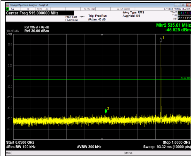
Band5-1.4MHz-QPSK-20643-1RB#0-Range1:30~100 0MHz
