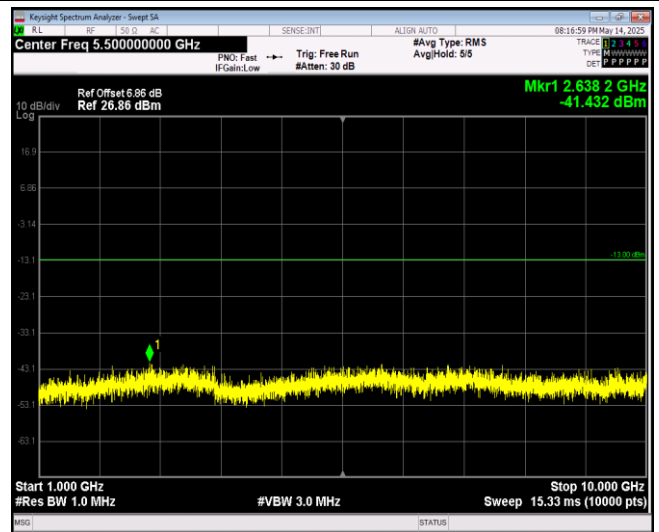
Band5-10MHz-16QAM-20450-1RB#0-Range2:1000~ 10000MHz
