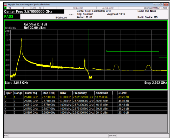
Band7-20MHz-QPSK-21350-100RB#0
