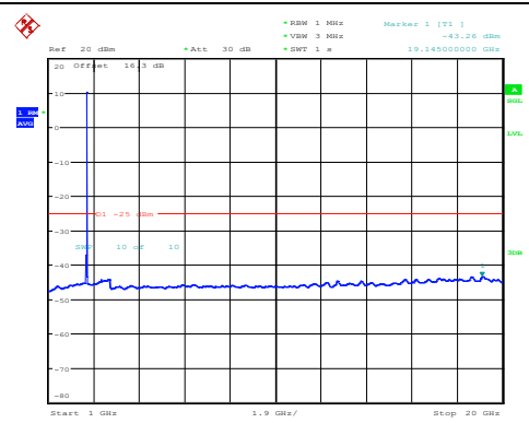
Band38-15MHz-QPSK-38000-1RB#0-1000~20000 -PASS
