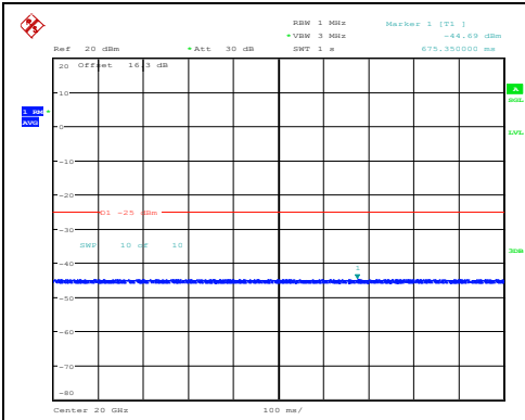
Band38-10MHz-QPSK-38200-1RB#0-20000~270 00-PASS
