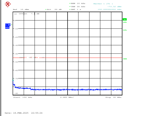
Band38-15MHz-16QAM-38175-1RB#0-0.15~30-P ASS
