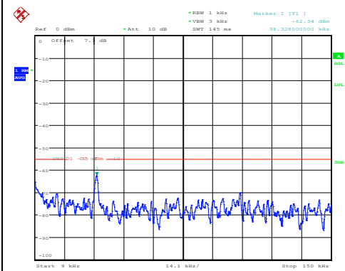
Band38-15MHz-16QAM-38000-1RB#0-1000~200 00-PASS
