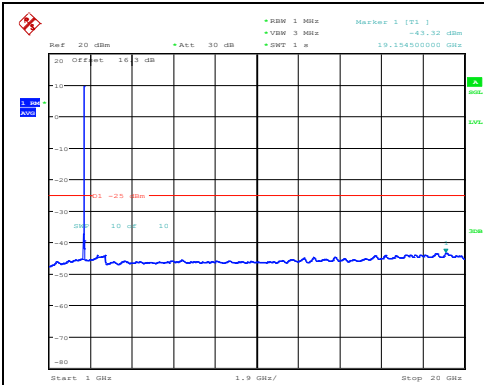
Band38-15MHz-16QAM-38000-1RB#0-1000~200 00-PASS
