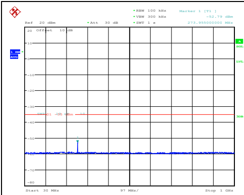
Band38-15MHz-QPSK-38000-1RB#0-30~1000-P ASS
