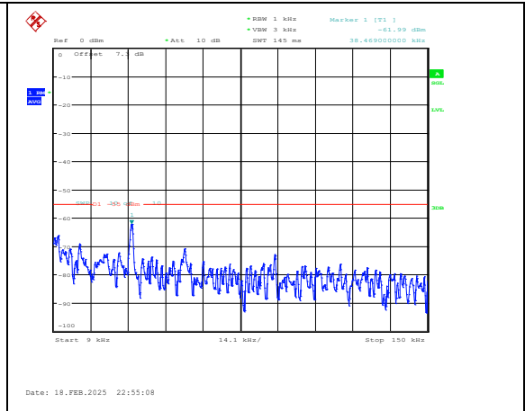
Band38-15MHz-16QAM-38175-1RB#0-0.009~0.15 -PASS
