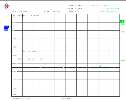
Band38-10MHz-16QAM-38000-1RB#0-20000~270 00-PASS
