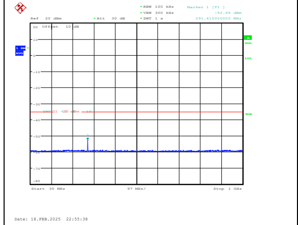
Band38-15MHz-16QAM-38175-1RB#0-30~1000-P ASS
