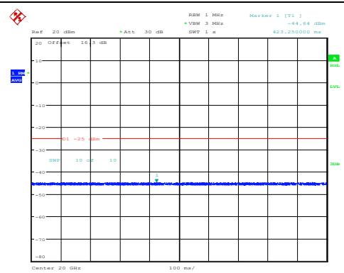
Band38-15MHz-16QAM-38000-1RB#0-20000~270 00-PASS
