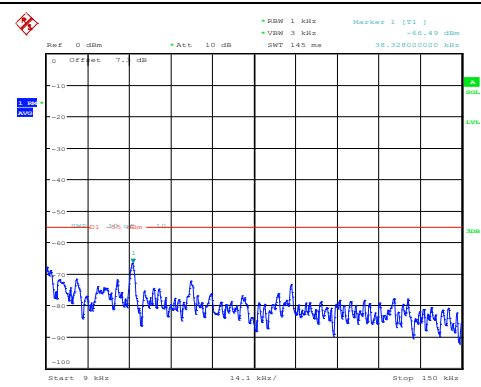
Band38-10MHz-16QAM-38200-1RB#0-0.009~0.15 -PASS
