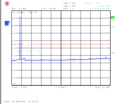
Band38-15MHz-16QAM-38175-1RB#0-1000~200 00-PASS
