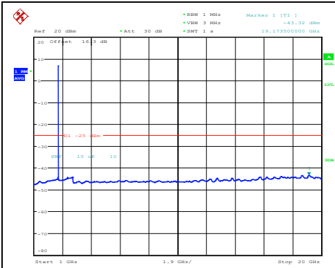
Band38-10MHz-16QAM-38000-1RB#0-1000~200 00-PASS
