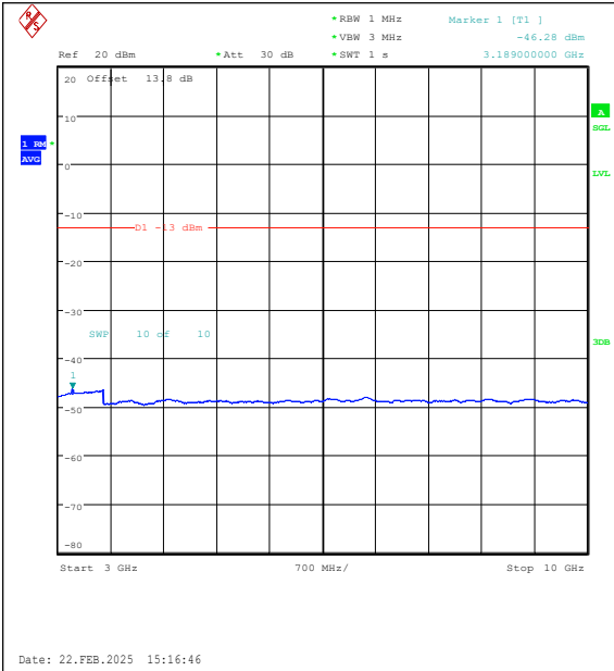
Band26(824-849)-15MHz-QPSK-26965-1RB#0-3 000~10000-PASS
