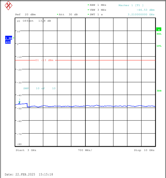
Band26(824-849)-15MHz-16QAM-26915-1RB#0-3 000~10000-PASS
