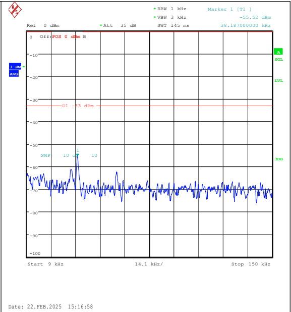
Band26(824-849)-15MHz-16QAM-26965-1RB#0-0 .009~0.15-PASS
