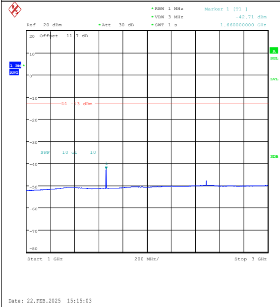
Band26(824-849)-15MHz-16QAM-26915-1RB#0-1000~3000-PASS
