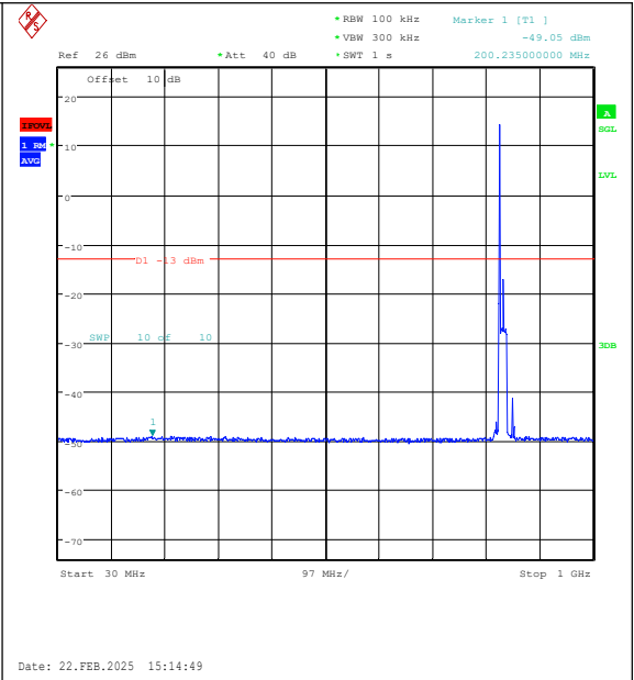
Band26(824-849)-15MHz-16QAM-26915-1RB#0-3 0~1000-PASS
