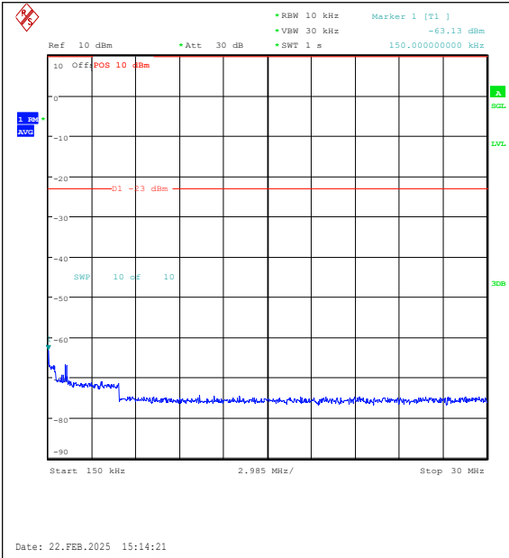
Band26(824-849)-15MHz-16QAM-26915-1RB#0-0.15~30-PASS
