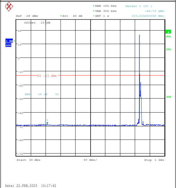
Band26(824-849)-15MHz-16QAM-26965-1RB#0-3 0~1000-PASS
