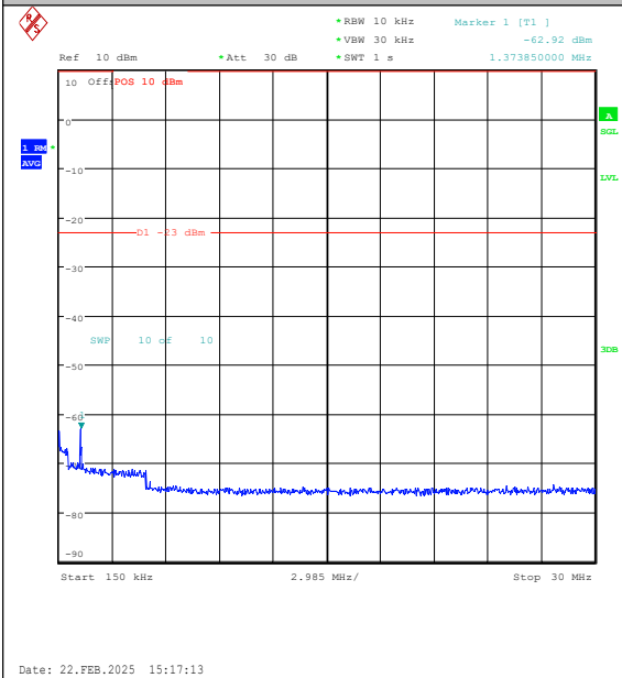
Band26(824-849)-15MHz-16QAM-26965-1RB#0-0 0.15~30-PASS
