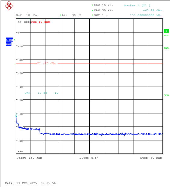
Band26(824-849)-1.4MHz-16QAM-26797-1RB#0- 0.15~30-PASS
