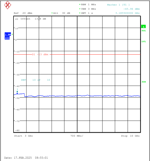
Band26(824-849)-5MHz-16QAM-27015-1RB#0-30 00~10000-PASS
