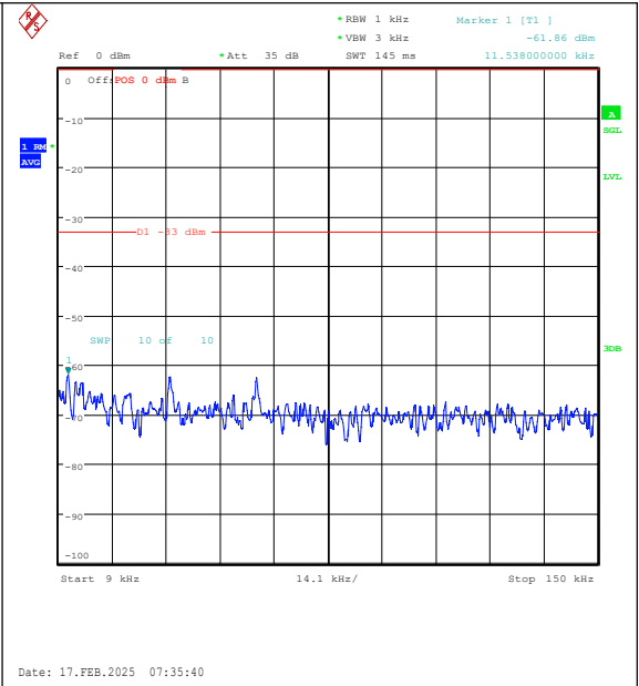
Band26(824-849)-1.4MHz-16QAM-26797-1RB#0- 0.009~0.15-PASS
