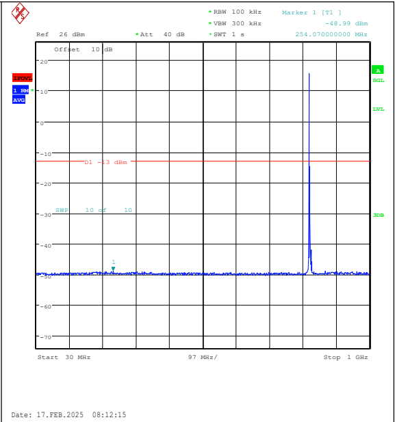
Band26(824-849)-3MHz-16QAM-26805-1RB#0-30 ~1000-PASS
