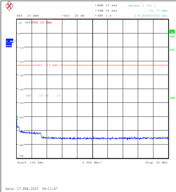
Band26(824-849)-3MHz-16QAM-26805-1RB#0-0. 15~30-PASS
