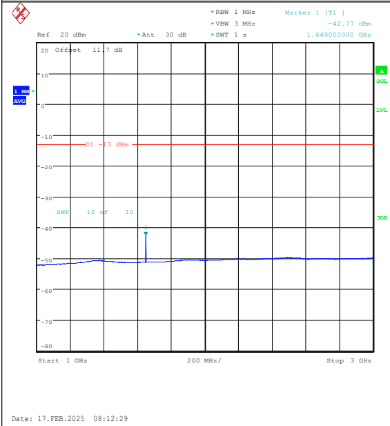
Band26(824-849)-3MHz-16QAM-26805-1RB#0-1 000~3000-PASS
