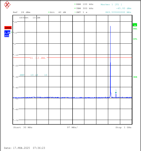
Band26(824-849)-1.4MHz-16QAM-26797-1RB#0- 30~1000-PASS
