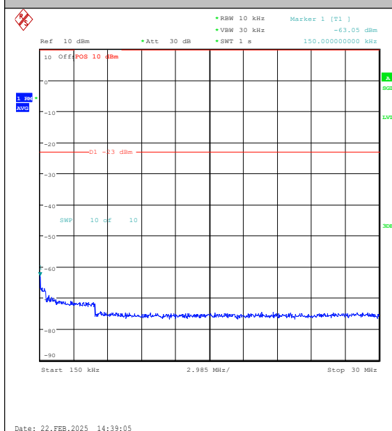
Band26(824-849)-10MHz-16QAM-26915-1RB#0- 0.15~30-PASS
