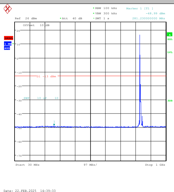
Band26(824-849)-10MHz-16QAM-26915-1RB#0-3 0~1000-PASS
