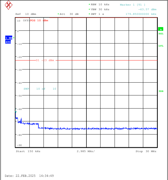
Band26(824-849)-10MHz-QPSK-26840-1RB#0-0.1 5~30-PASS
