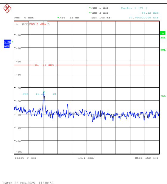
Band26(824-849)-10MHz-16QAM-26915-1RB#0-0 .009~0.15-PASS
