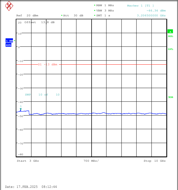
Band26(824-849)-3MHz-16QAM-26805-1RB#0-30 00~10000-PASS
