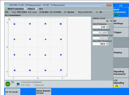
Band25-15MHz-16QAM-26615-75RB#0-PASS
