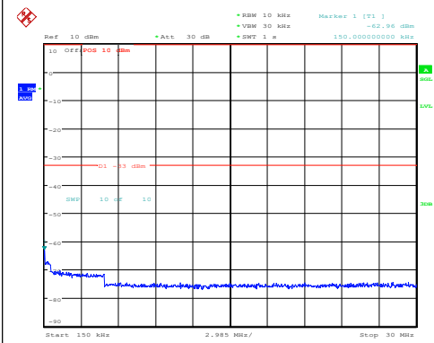
Band25-15MHz-QPSK-26615-1RB#0-3000~2000 0-PASS
