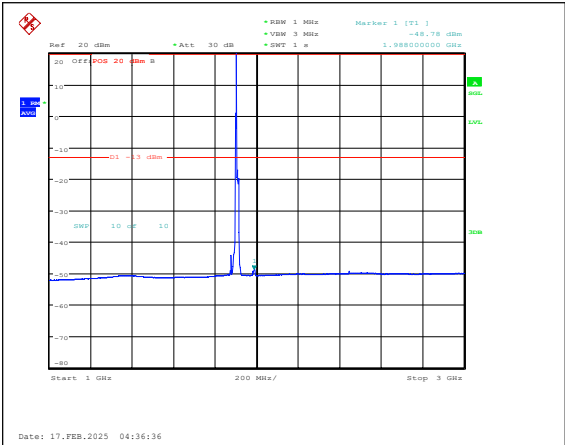
Band25-15MHz-16QAM-26615-1RB#0-1000~300 0-PASS
