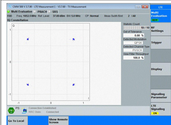
Band25-5MHz-QPSK-26065-25RB#0-PASS
