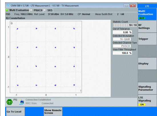
Band25-3MHz-16QAM-26365-15RB#0-PASS
