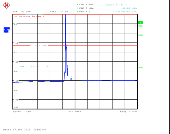
Band25-20MHz-QPSK-26140-1RB#0-1000~3000-PASS
