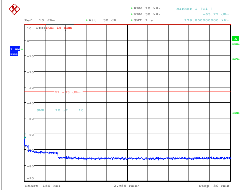
Band25-20MHz-QPSK-26590-1RB#0-3000~2000 0-PASS
