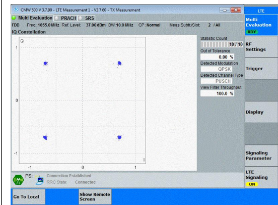
Band25-10MHz-QPSK-26090-50RB#0-PASS
