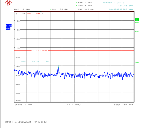
Band25-15MHz-QPSK-26615-1RB#0-0.009~0.15 -PASS
