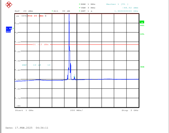
Band25-15MHz-16QAM-26365-1RB#0-1000~300 0-PASS
