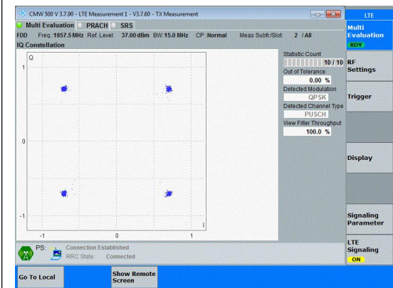
Band25-15MHz-QPSK-26115-75RB#0-PASS
