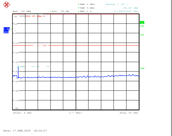
Band25-15MHz-16QAM-26365-1RB#0-3000~2000 0-PASS
