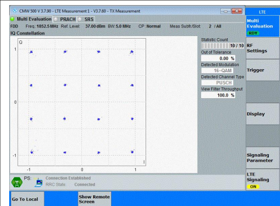
Band25-5MHz-16QAM-26065-25RB#0-PASS
