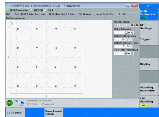
Band25-5MHz-16QAM-26665-25RB#0-PASS
