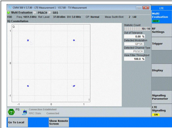
Band25-3MHz-QPSK-26055-15RB#0-PASS
