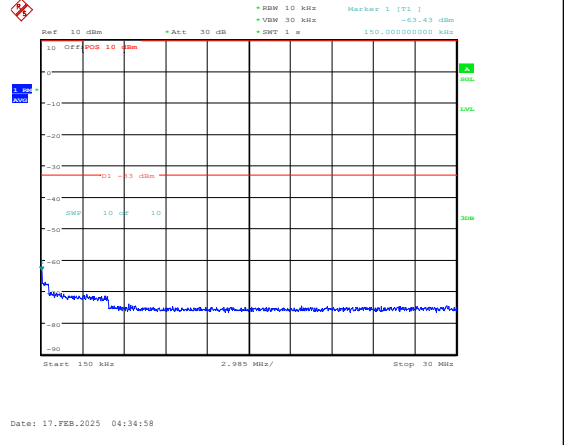
Band25-15MHz-QPSK-26615-1RB#0-0.15~30-PA SS
