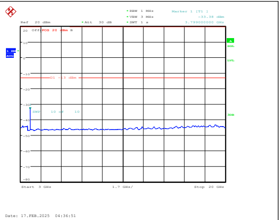
Band25-15MHz-16QAM-26615-1RB#0-3000~2000 0-PASS
