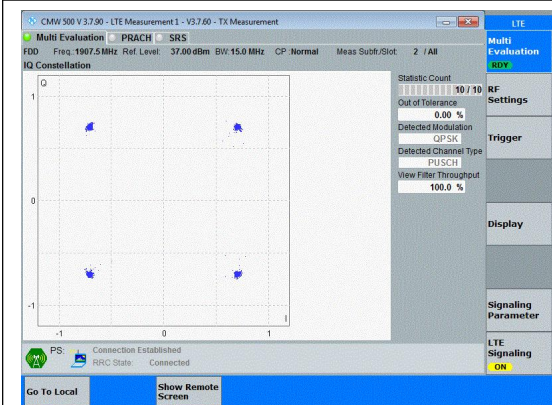
Band25-15MHz-QPSK-26615-75RB#0-PASS
