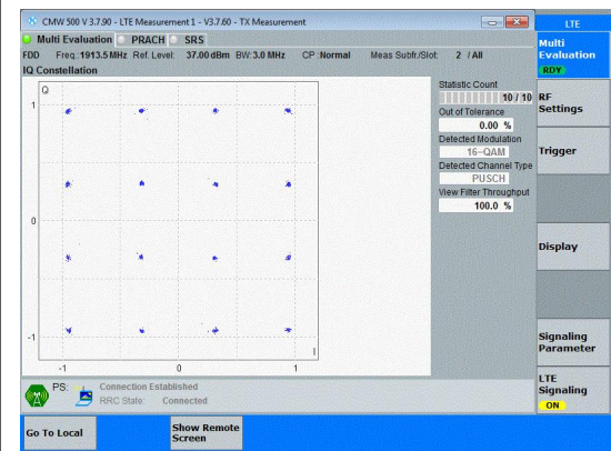
Band25-3MHz-16QAM-26675-15RB#0-PASS
