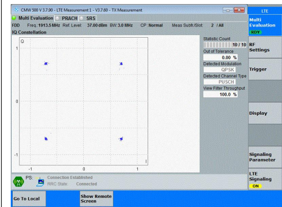
Band25-3MHz-QPSK-26675-15RB#0-PASS
