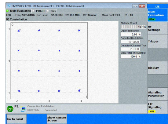
Band25-10MHz-16QAM-26090-50RB#0-PASS
