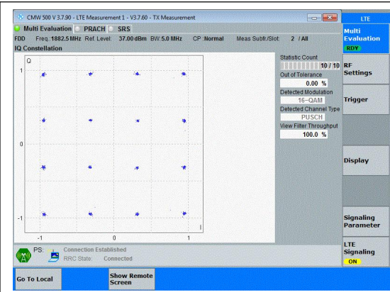
Band25-5MHz-16QAM-26365-25RB#0-PASS
