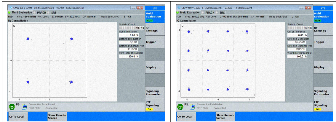
Band25-20MHz-QPSK-26140-100RB#0-PASS
