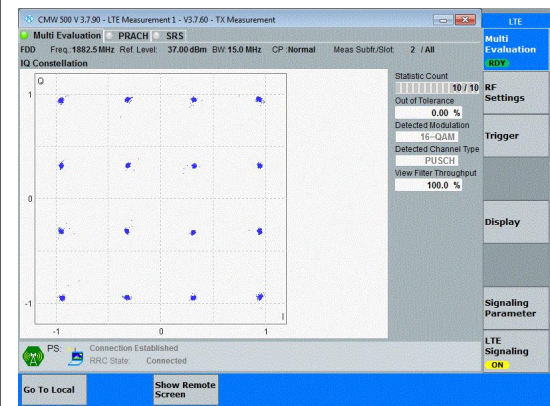
Band25-15MHz-16QAM-26365-75RB#0-PASS
