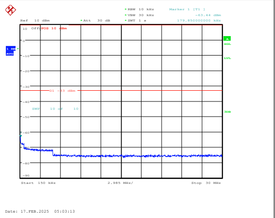
Band25-20MHz-QPSK-26140-1RB#0-0.15~30-PA SS
