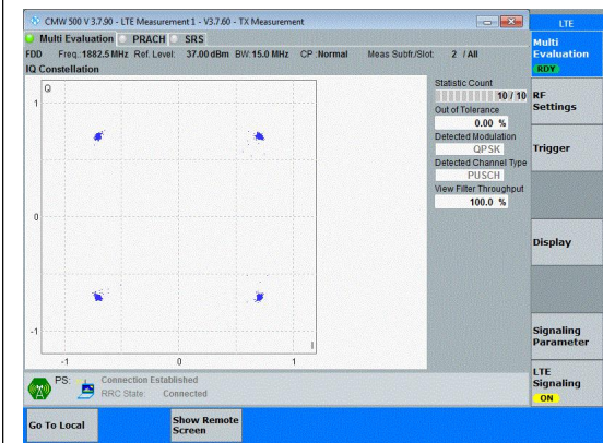
Band25-15MHz-QPSK-26365-75RB#0-PASS
