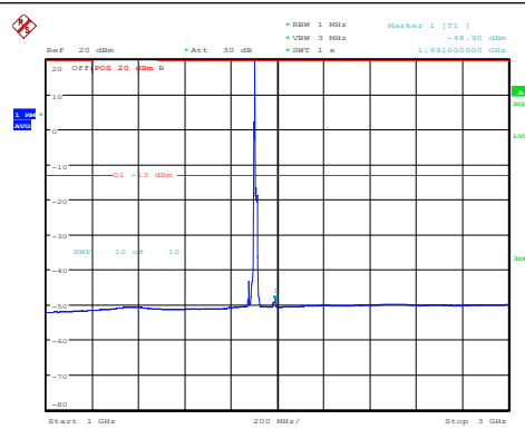
Band25-15MHz-QPSK-26615-1RB#0-1000~3000- PASS
