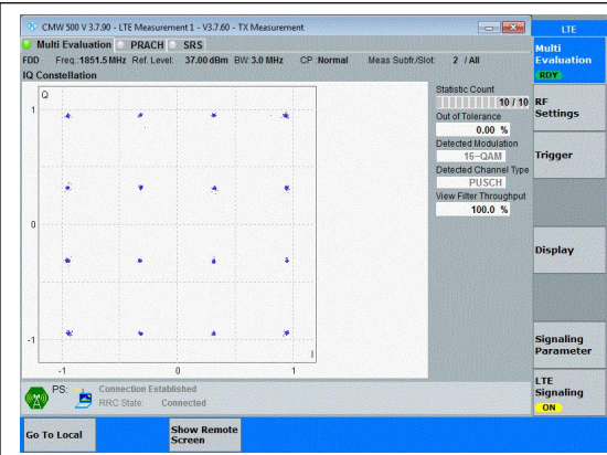
Band25-3MHz-16QAM-26055-15RB#0-PASS
