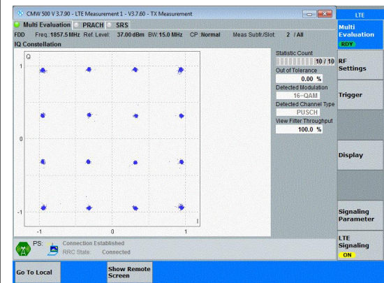
Band25-15MHz-16QAM-26115-75RB#0-PASS
