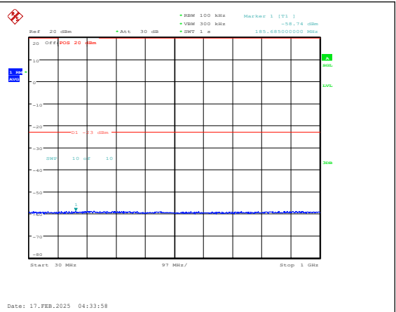
Band25-15MHz-16QAM-26365-1RB#0-30~1000-P ASS
