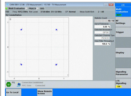
Band25-5MHz-QPSK-26665-25RB#0-PASS
