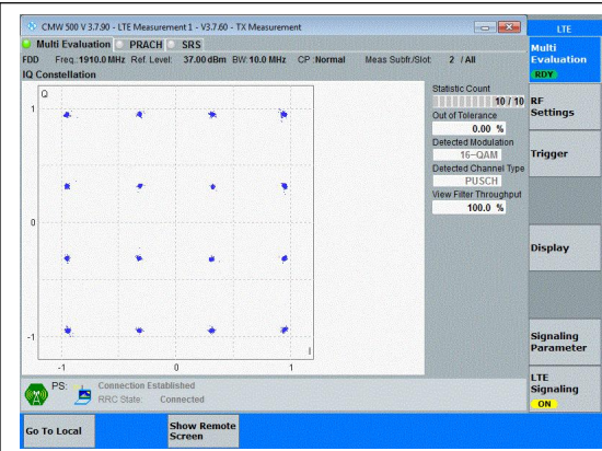
Band25-10MHz-16QAM-26640-50RB#0-PASS
