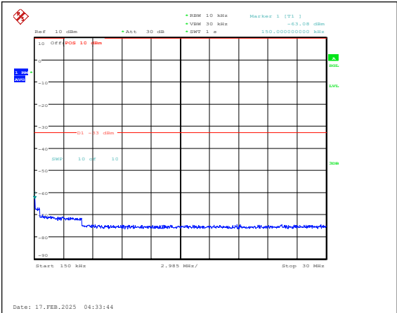
Band25-15MHz-16QAM-26365-1RB#0-0.15~30-P ASS
