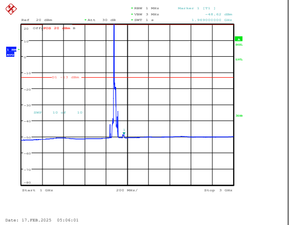
Band25-20MHz-QPSK-26365-1RB#0-1000~3000-P PASS
