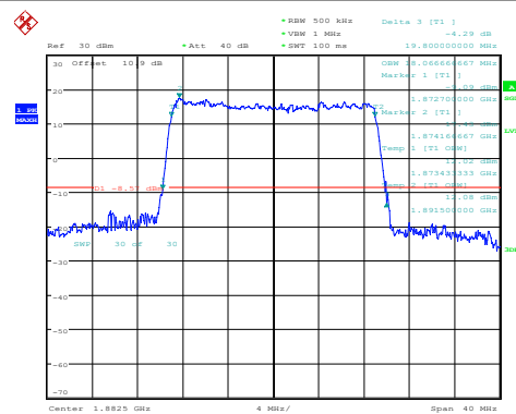
Band25-20MHz-16QAM-26140-100RB#0-PASS
