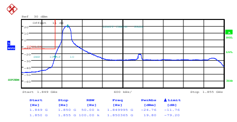
Band25-5MHz-QPSK-26065-1RB#24-PASS
