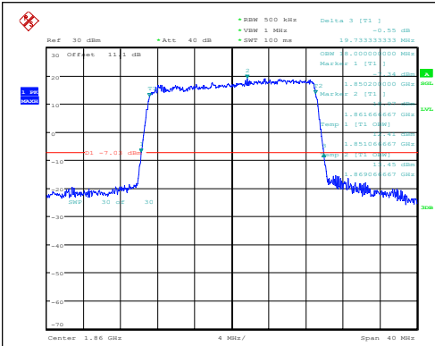
Band25-20MHz-QPSK-26140-100RB#0-PASS
