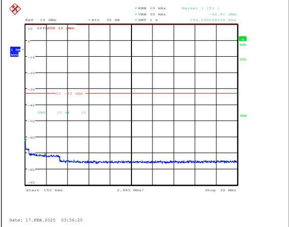
Band25-10MHz-16QAM-26090-1RB#0-0.15~30-P ASS
