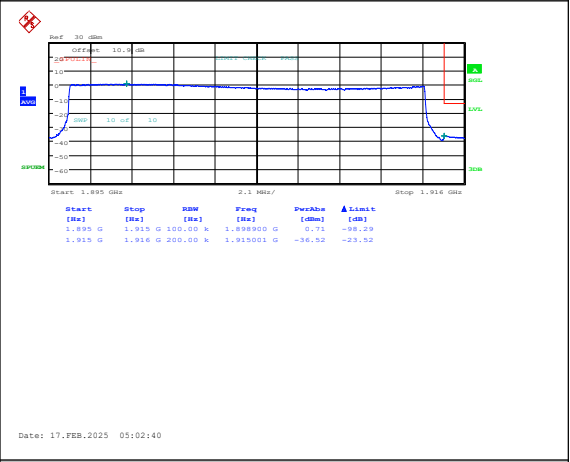
Band25-20MHz-16QAM-26590-100RB#0-PASS
