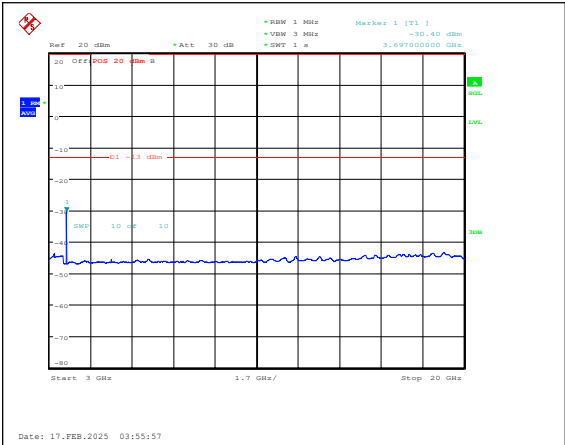
Band25-10MHz-QPSK-26090-1RB#0-3000~2000 0-PASS
