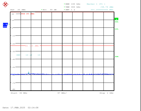
Band25-1.4MHz-16QAM-26047-1RB#0-30~1000-P ASS
