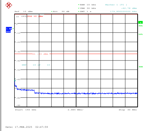
Band25-3MHz-16QAM-26055-1RB#0-0.15~30-PA SS
