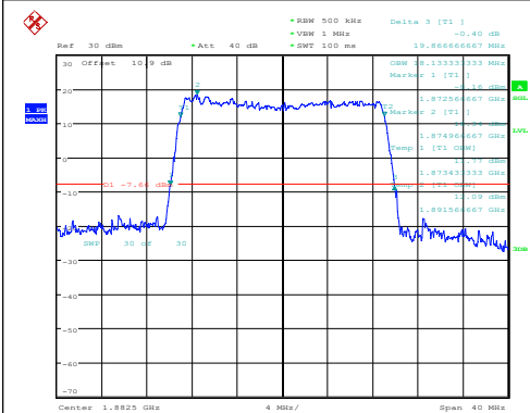
Band25-20MHz-QPSK-26140-100RB#0-PASS
