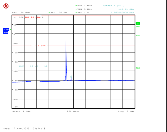
Band25-5MHz-QPSK-26365-1RB#0-1000~3000-P
