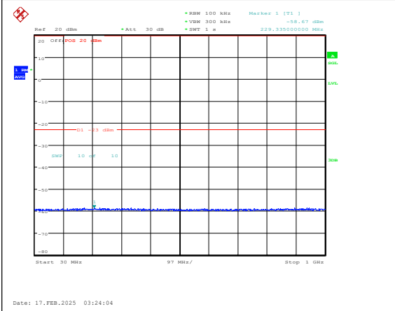
Band25-5MHz-QPSK-26365-1RB#0-30~1000-PA
