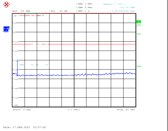
Band25-10MHz-16QAM-26090-1RB#0-3000~2000 0-PASS
