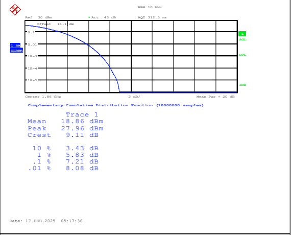
Band25-20MHz-16QAM-26140-100RB#0-PASS
