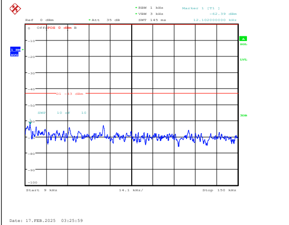
Band25-5MHz-QPSK-26665-1RB#0-0.009~0.15- PASS
