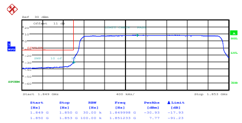
Band25-3MHz-16QAM-26055-1RB#0-PASS
