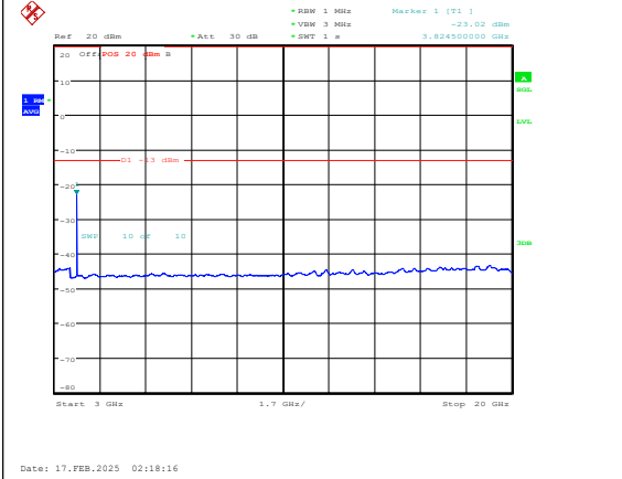
Band25-1.4MHz-QPSK-26683-1RB#0-3000~2000 0-PASS
