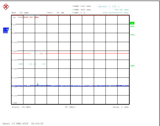
Band25-1.4MHz-16QAM-26365-1RB#0-30~1000-PASS
