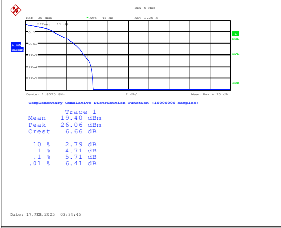
Band25-5MHz-16QAM-26065-1RB#0-PASS
