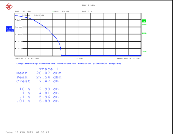
Band25-1.4MHz-16QAM-26683-6RB#0-PASS
