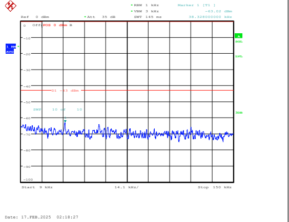
Band25-1.4MHz-16QAM-26683-1RB#0-0.009~0.1 5-PASS
