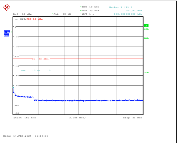
Band25-1.4MHz-QPSK-26365-1RB#0-0.15~30-PA SS
