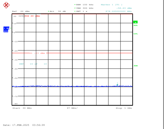
Band25-10MHz-16QAM-26090-1RB#0-30~1000-P ASS
