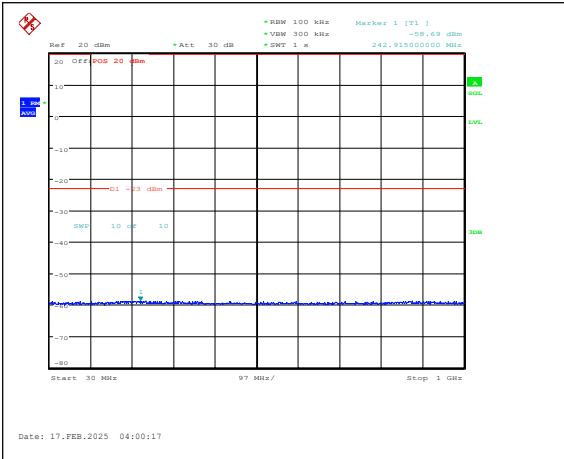
Band25-10MHz-QPSK-26640-1RB#0-30~1000-P ASS
