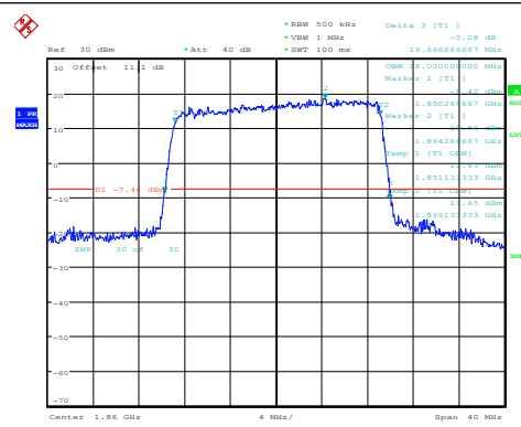
Band25-20MHz-16QAM-26140-100RB#0-PASS
