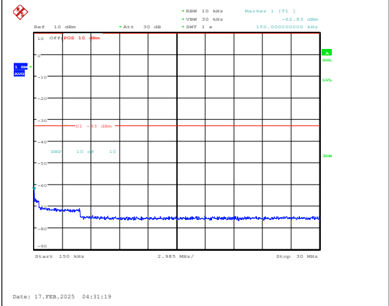
Band25-15MHz-16QAM-26115-1RB#0-0.15~30-P ASS
