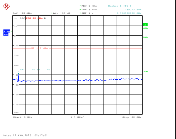
Band25-1.4MHz-16QAM-26365-1RB#0-3000~20000-PASS
