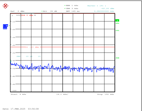
Band25-10MHz-16QAM-26090-1RB#0-0.009~0.15 -PASS
