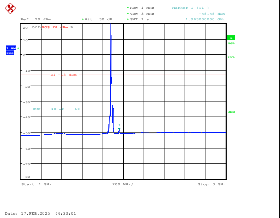
Band25-15MHz-QPSK-26365-1RB#0-1000~3000-P PASS
