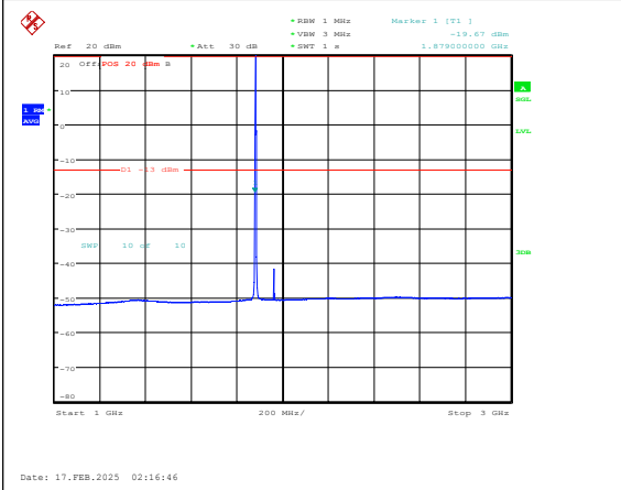
Band25-1.4MHz-16QAM-26365-1RB#0-1000~3000-PASS
