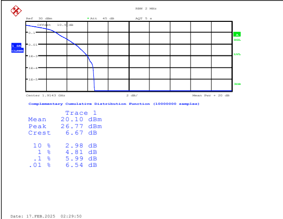
Band25-1.4MHz-16QAM-26683-1RB#0-PASS
