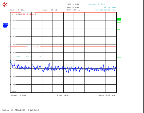
Band25-10MHz-16QAM-26640-1RB#0-0.009~0.15 -PASS
