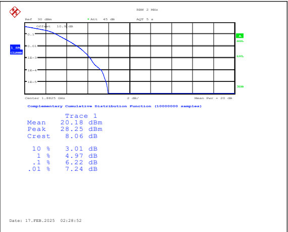
Band25-1.4MHz-16QAM-26365-6RB#0-PASS
