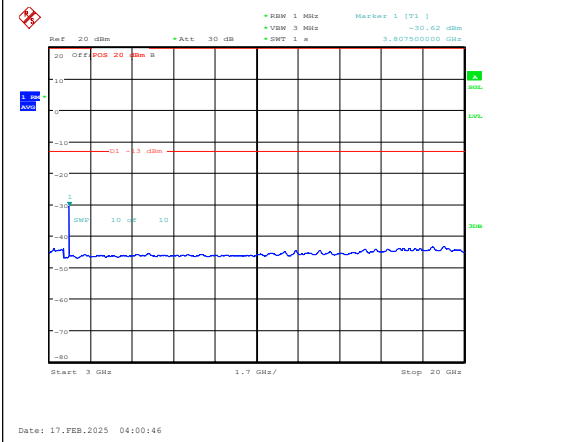
Band25-10MHz-QPSK-26640-1RB#0-3000~2000 0-PASS
