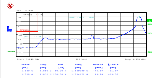
Band25-5MHz-QPSK-26065-25RB#0-PASS
