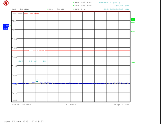
Band25-1.4MHz-16QAM-26683-1RB#0-30~1000-P ASS
