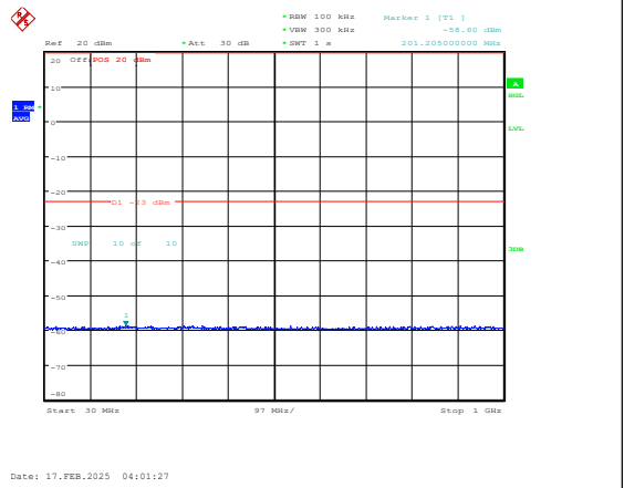
Band25-10MHz-16QAM-26640-1RB#0-30~1000-P ASS
