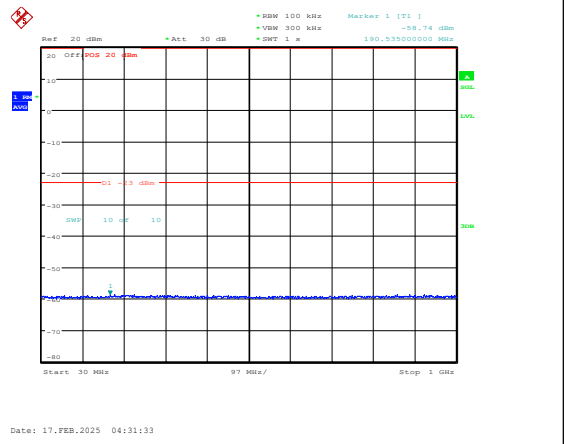
Band25-15MHz-16QAM-26115-1RB#0-30~1000-P ASS
