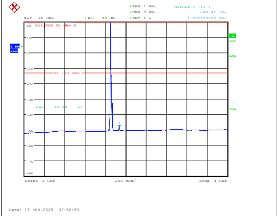
Band25-10MHz-16QAM-26090-1RB#0-1000~300 0-PASS
