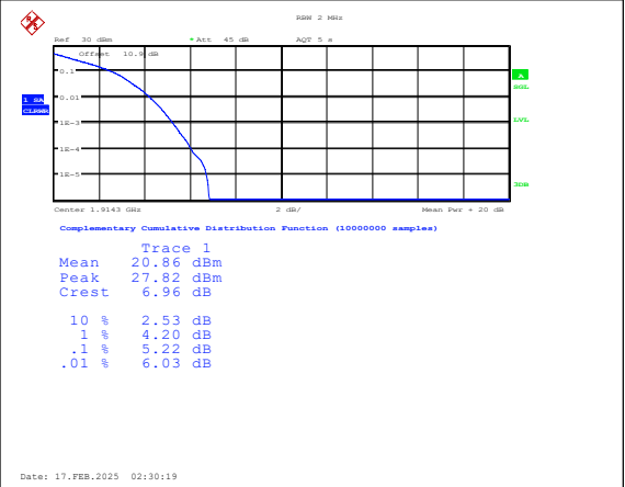
Band25-1.4MHz-QPSK-26683-6RB#0-PASS
