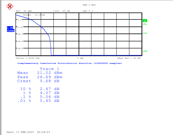
Band25-1.4MHz-QPSK-26683-1RB#0-PASS
