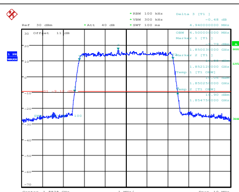
Band25-5MHz-16QAM-26065-25RB#0-PASS
