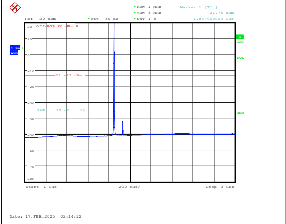
Band25-1.4MHz-16QAM-26047-1RB#0-1000~30 00-PASS
