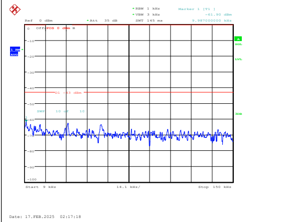
Band25-1.4MHz-QPSK-26683-1RB#0-0.009~0.15-PASS
