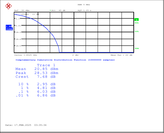
Band25-5MHz-16QAM-26065-25RB#0-PASS
