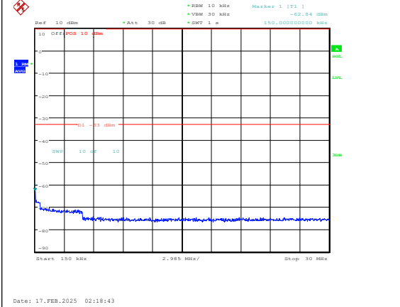
Band25-1.4MHz-16QAM-26683-1RB#0-0.15~30- PASS
