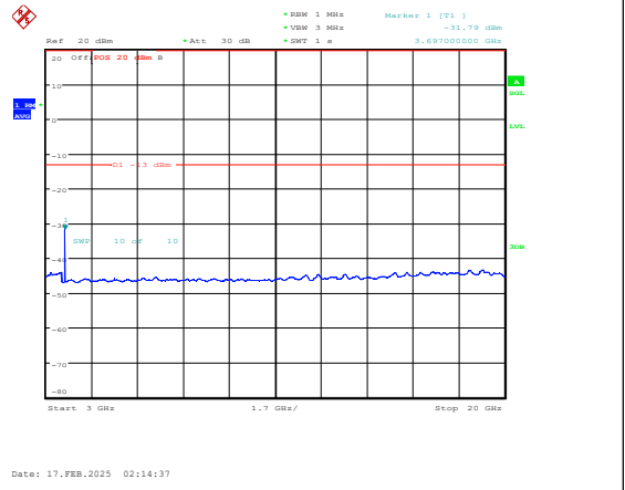
Band25-1.4MHz-16QAM-26047-1RB#0-3000~200 00-PASS
