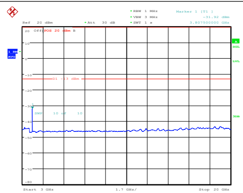
Band25-10MHz-16QAM-26640-1RB#0-3000~2000 0-PASS
