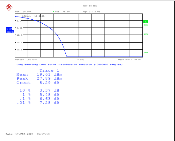
Band25-20MHz-QPSK-26140-100RB#0-PASS
