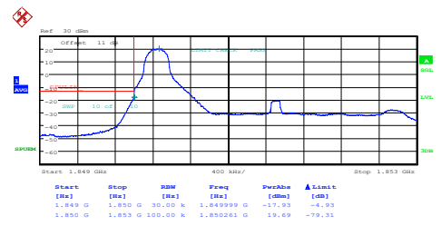
Band25-3MHz-QPSK-26055-1RB#14-PASS
