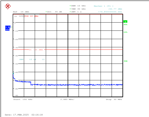
Band25-1.4MHz-16QAM-26365-1RB#0-0.15~30-PASS
