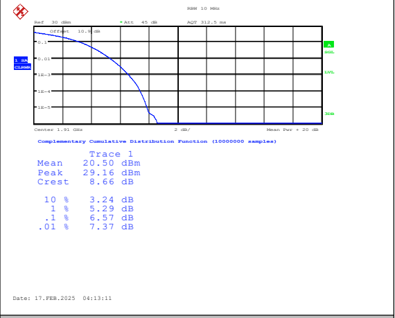
Band25-10MHz-16QAM-26640-50RB#0-PASS
