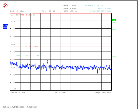
Band25-1.4MHz-16QAM-26047-1RB#0-0.009~0.1 5-PASS
