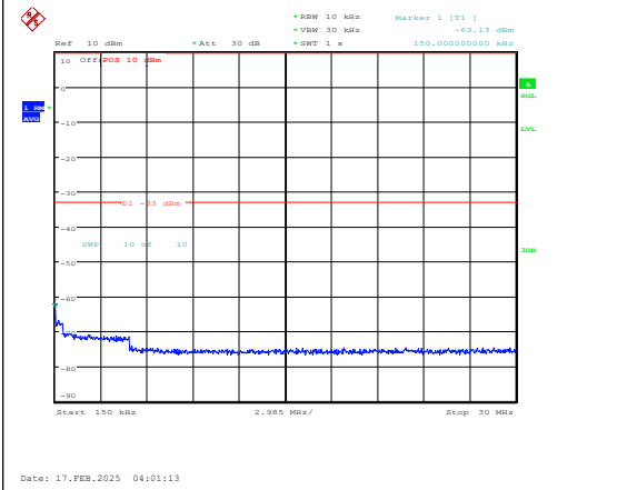
Band25-10MHz-16QAM-26640-1RB#0-0.15~30-P ASS
