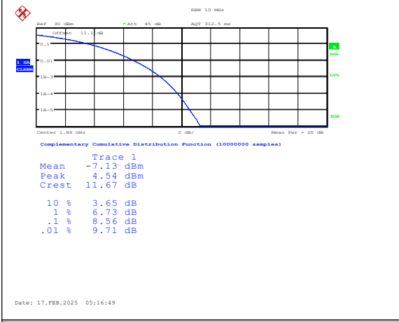
Band25-20MHz-16QAM-26140-1RB#0-PASS
