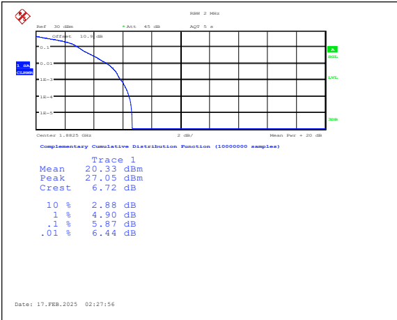
Band25-1.4MHz-16QAM-26365-1RB#0-PASS
