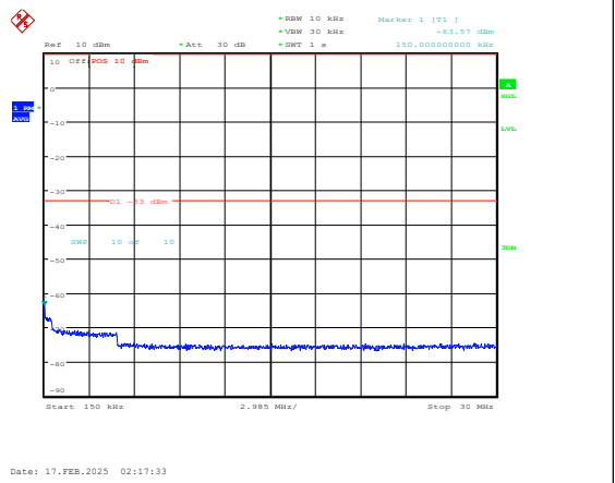
Band25-1.4MHz-QPSK-26683-1RB#0-0.15~30-PASS
