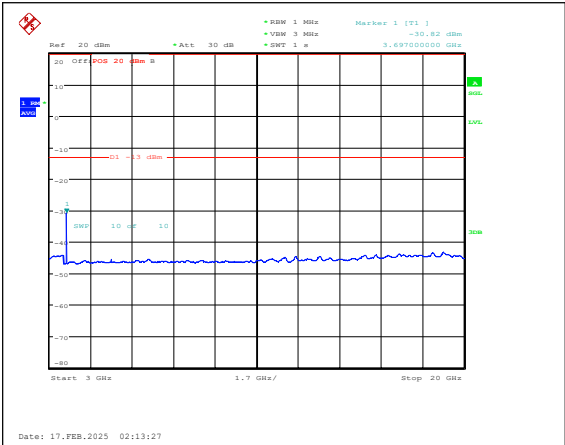
Band25-1.4MHz-QPSK-26047-1RB#0-3000~2000 0-PASS
