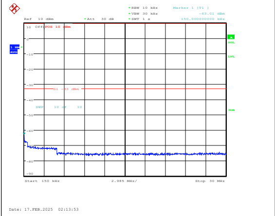
Band25-1.4MHz-16QAM-26047-1RB#0-0.15~30-PASS
