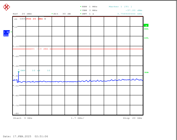
Band25-3MHz-16QAM-26365-1RB#0-3000~20000 -PASS
