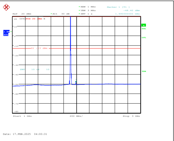
Band25-10MHz-QPSK-26640-1RB#0-1000~3000- PASS
