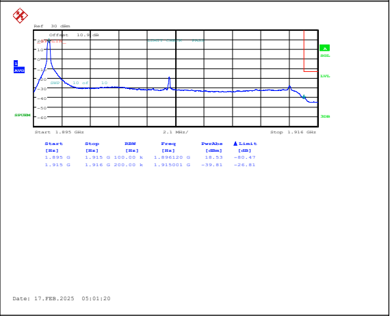
Band25-20MHz-16QAM-26590-1RB#0-PASS
