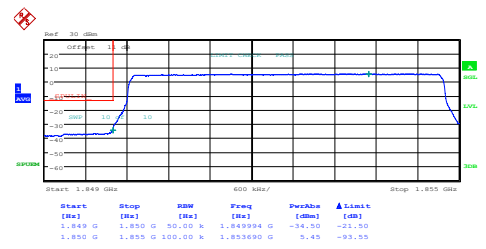
Band25-5MHz-16QAM-26065-1RB#0-PASS
