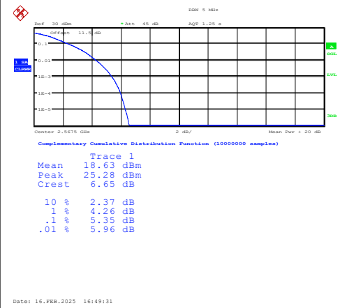
Band7-5MHz-QPSK-21425-25RB#0-PASS
