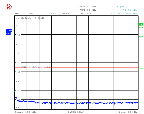
Band7-5MHz-16QAM-20775-1RB#0-0.15~30-PA SS
