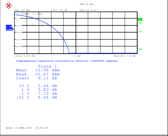
Band7-20MHz-16QAM-20850-100RB#0-PASS
