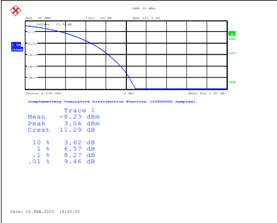
Band7-20MHz-QPSK-21100-1RB#0-PASS
