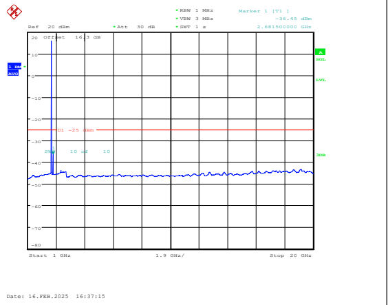
Band7-5MHz-QPSK-21425-1RB#0-1000~20000-P ASS
