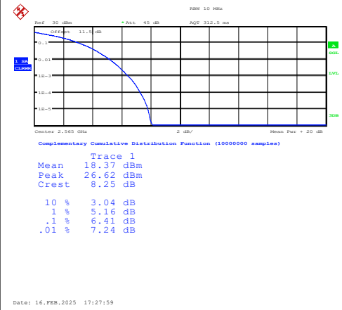
Band7-10MHz-16QAM-21400-50RB#0-PASS
