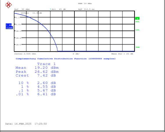
Band7-10MHz-QPSK-21100-50RB#0-PASS
