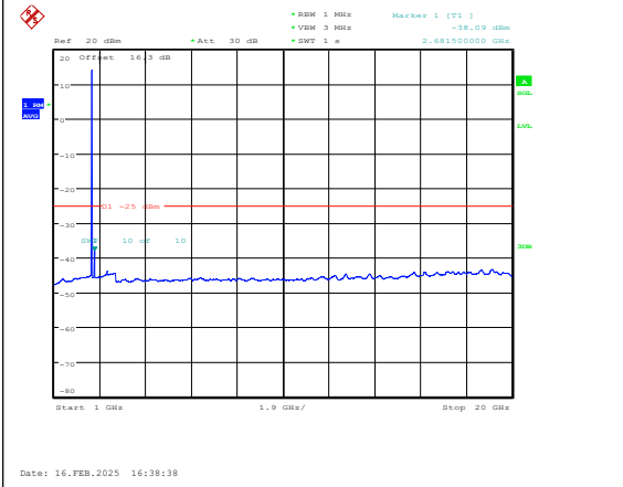
Band7-5MHz-16QAM-21425-1RB#0-1000~20000 -PASS
