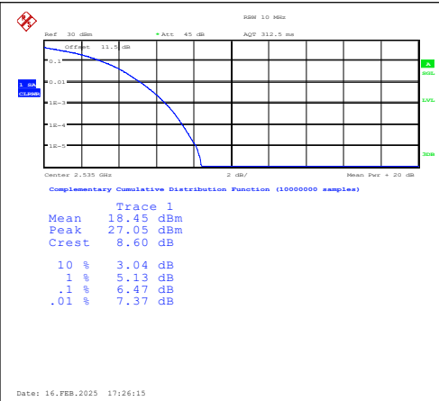
Band7-10MHz-16QAM-21100-50RB#0-PASS
