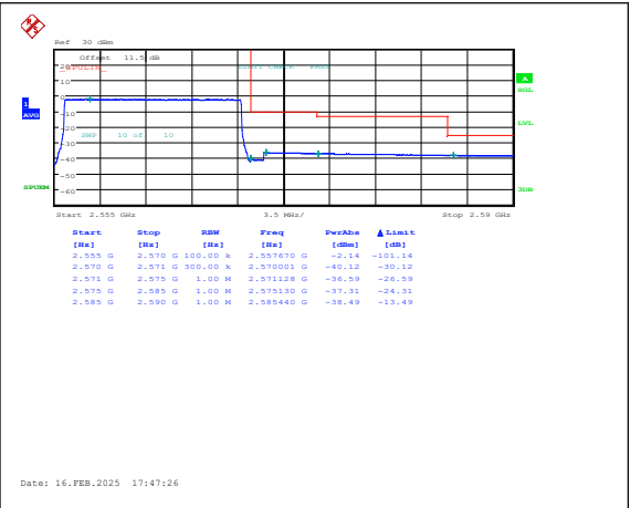
Band7-15MHz-16QAM-21375-75RB#0-PASS
