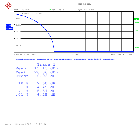
Band7-10MHz-QPSK-21400-50RB#0-PASS
