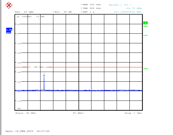
Band7-5MHz-QPSK-21425-1RB#0-30~1000-PAS S
