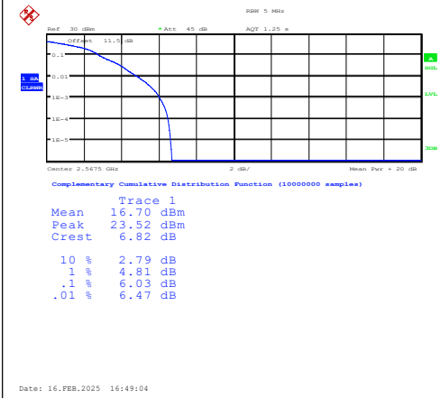
Band7-5MHz-16QAM-21425-1RB#0-PASS
