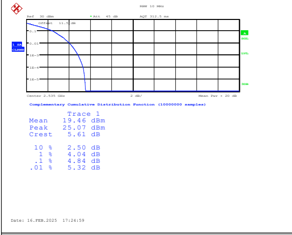
Band7-10MHz-QPSK-21100-1RB#0-PASS
