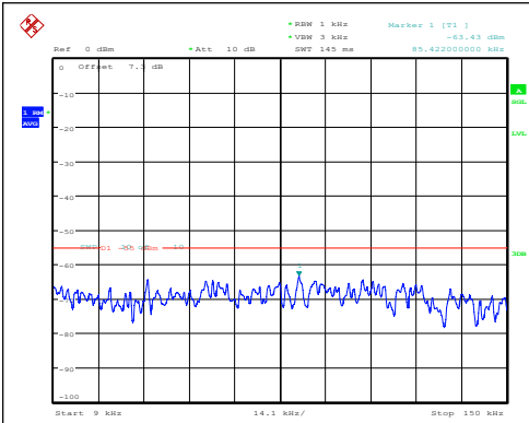
Band7-10MHz-QPSK-20800-1RB#0-0.009~0.15-PASS
