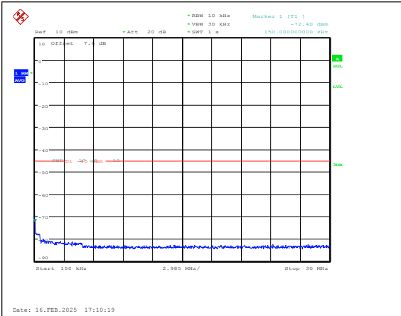
Band7-10MHz-16QAM-20800-1RB#0-0.15~30-PA SS
