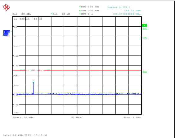
Band7-10MHz-16QAM-20800-1RB#0-30~1000-PA SS
