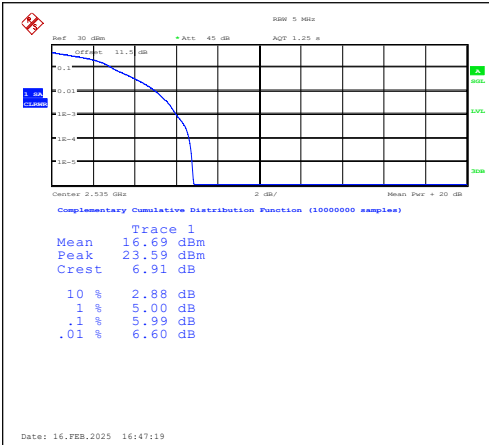
Band7-5MHz-16QAM-21100-1RB#0-PASS
