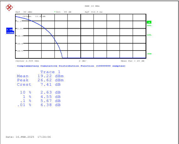
Band7-10MHz-QPSK-20800-50RB#0-PASS
