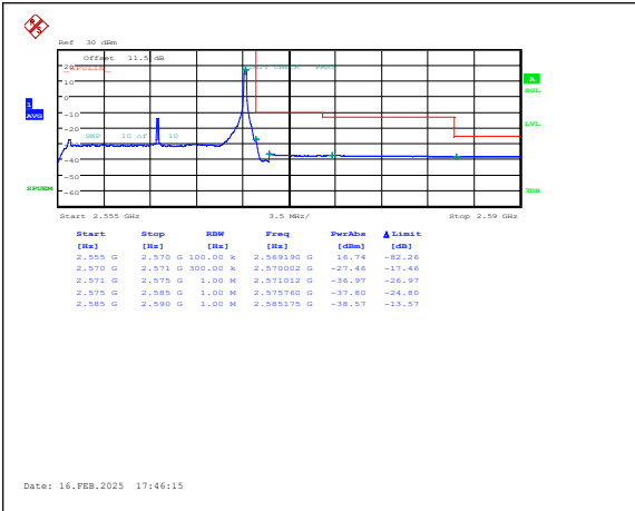
Band7-15MHz-16QAM-21375-1RB#74-PASS
