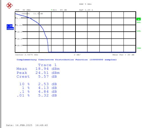
Band7-5MHz-QPSK-21425-1RB#0-PASS
