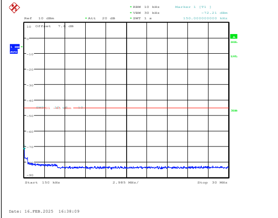
Band7-5MHz-16QAM-21425-1RB#0-0.15~30-PA SS
