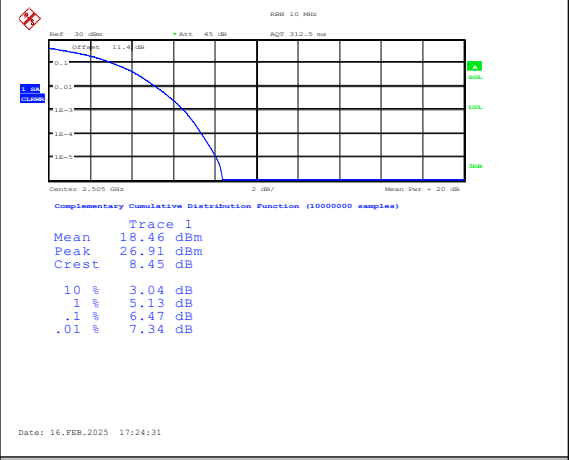
Band7-10MHz-16QAM-20800-50RB#0-PASS
