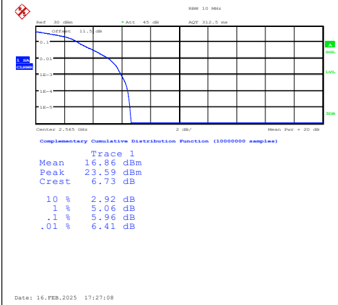
Band7-10MHz-16QAM-21400-1RB#0-PASS
