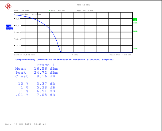
Band7-20MHz-QPSK-21100-100RB#0-PASS
