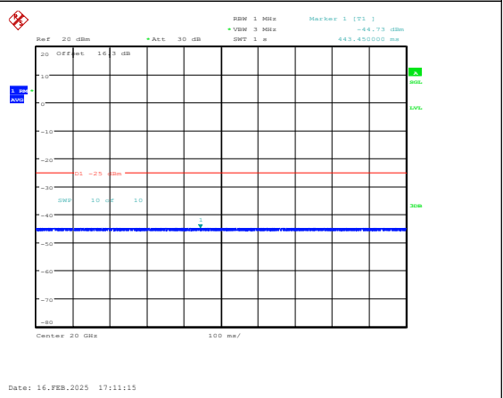
Band7-10MHz-16QAM-20800-1RB#0-20000~2700 0-PASS
