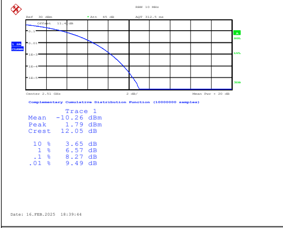
Band7-20MHz-16QAM-20850-1RB#0-PASS
