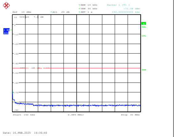
Band7-5MHz-QPSK-21425-1RB#0-0.15~30-PASS
