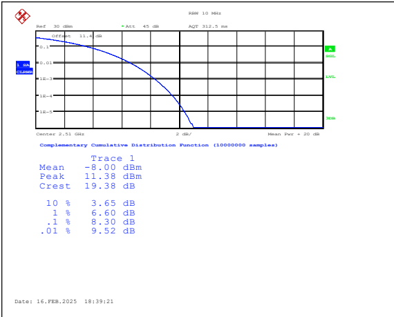
Band7-20MHz-QPSK-20850-1RB#0-PASS
