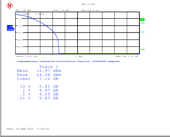
Band7-10MHz-16QAM-20800-1RB#0-PASS
