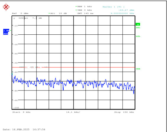
Band7-5MHz-16QAM-21425-1RB#0-0.009~0.15-P ASS
