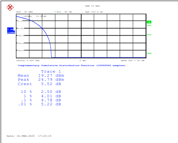
Band7-10MHz-QPSK-20800-1RB#0-PASS
