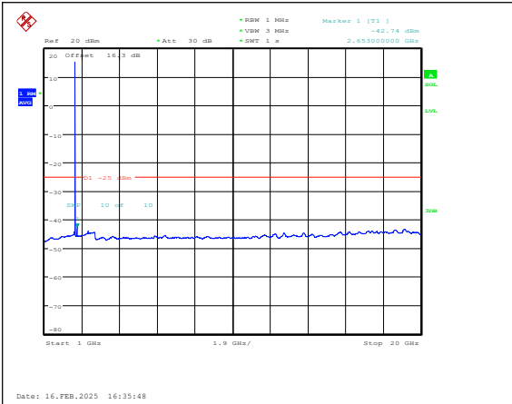
Band7-5MHz-16QAM-21100-1RB#0-1000~20000 -PASS
