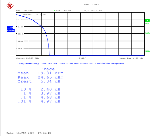
Band7-10MHz-QPSK-21400-1RB#0-PASS
