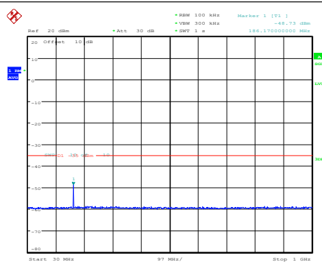
Band7-5MHz-16QAM-20775-1RB#0-30~1000-PAS S
