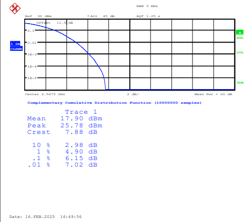
Band7-5MHz-16QAM-21425-25RB#0-PASS
