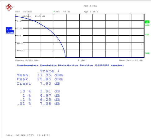
Band7-5MHz-16QAM-21100-25RB#0-PASS
