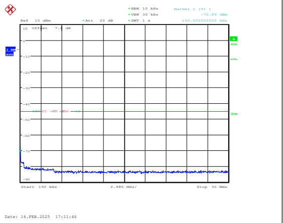
Band7-10MHz-QPSK-21100-1RB#0-0.15~30-PAS S
