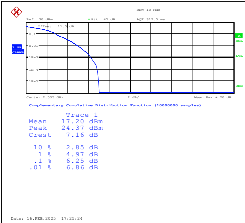
Band7-10MHz-16QAM-21100-1RB#0-PASS
