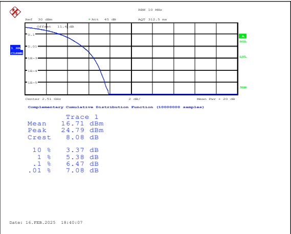
Band7-20MHz-QPSK-20850-100RB#0-PASS
