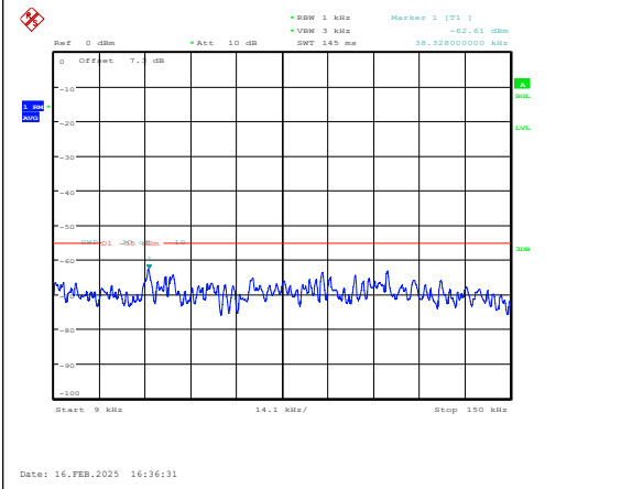
Band7-5MHz-QPSK-21425-1RB#0-0.009~0.15-P ASS
