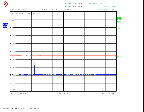
Band7-5MHz-16QAM-21425-1RB#0-30~1000-PAS S
