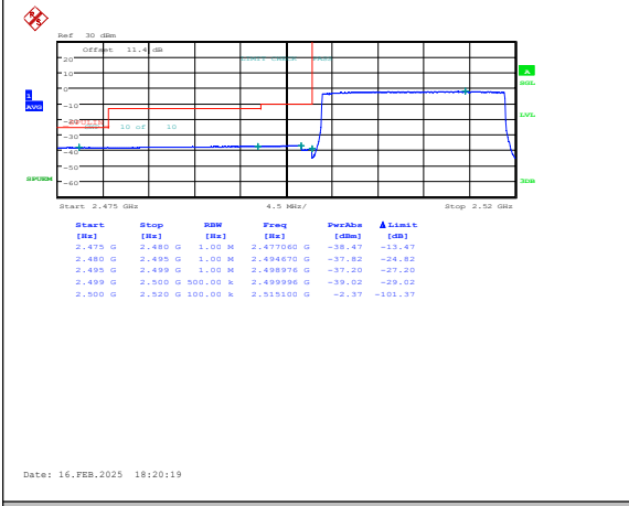
Band7-20MHz-QPSK-20850-100RB#0-PASS
