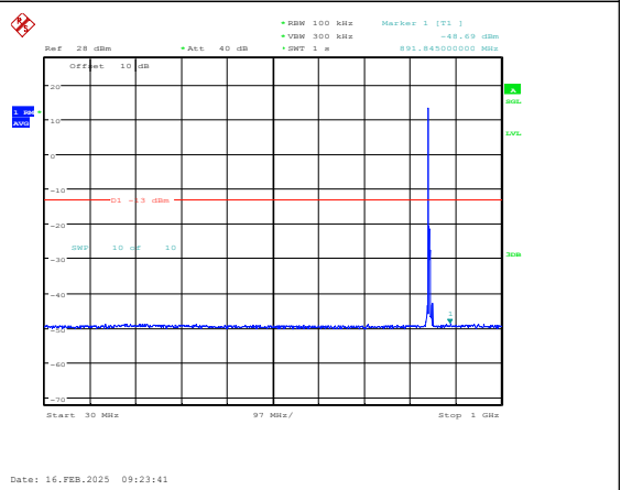
Band5-5MHz-16QAM-20625-1RB#0-30~1000-PAS S
