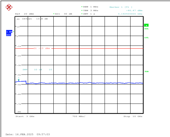
Band5-10MHz-QPSK-20600-1RB#0-3000~10000 -PASS
