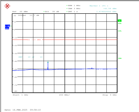
Band5-10MHz-16QAM-20600-1RB#0-1000~3000 -PASS
