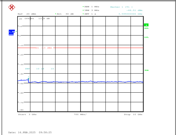
Band5-10MHz-16QAM-20600-1RB#0-3000~10000 -PASS
