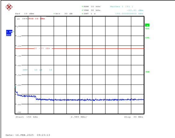
Band5-5MHz-16QAM-20625-1RB#0-0.15~30-PA SS
