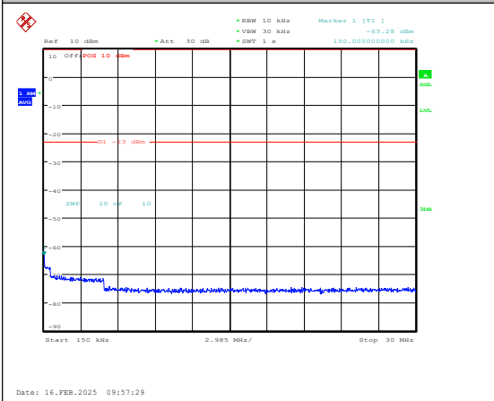
Band5-10MHz-16QAM-20600-1RB#0-0.15~30-PA SS
