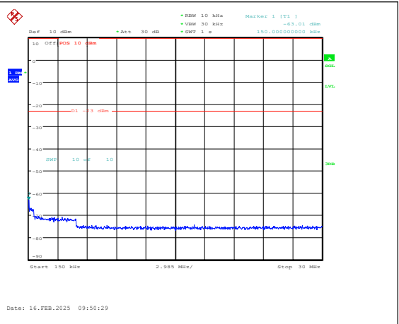
Band5-10MHz-QPSK-20450-1RB#0-0.15~30-PAS
