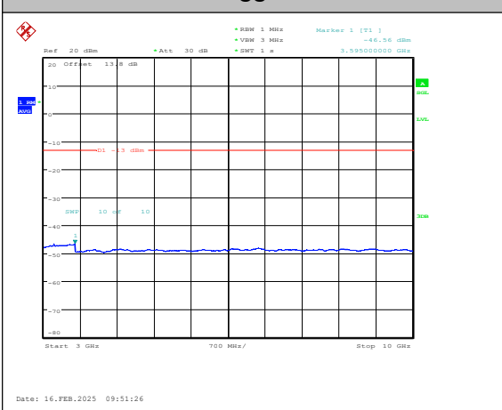
Band5-10MHz-QPSK-20450-1RB#0-3000~10000
