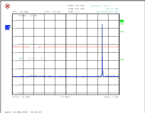
Band5-3MHz-QPSK-20635-1RB#0-30~1000-PASS
