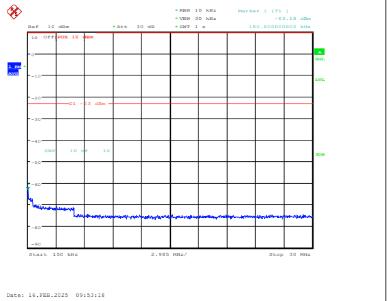
Band5-10MHz-QPSK-20525-1RB#0-0.15~30-PAS S
