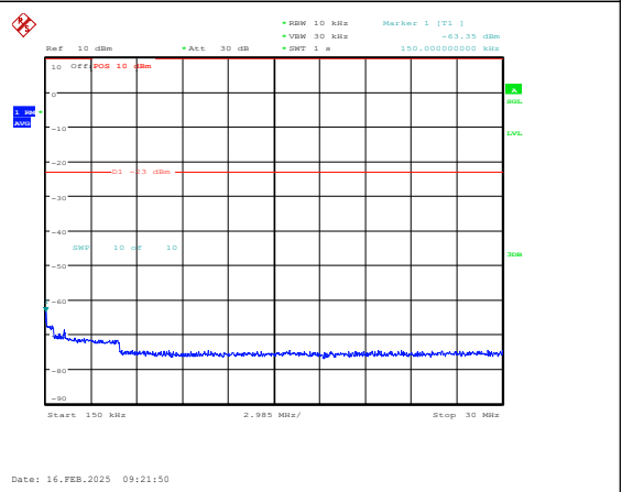
Band5-5MHz-QPSK-20625-1RB#0-0.15~30-PASS
