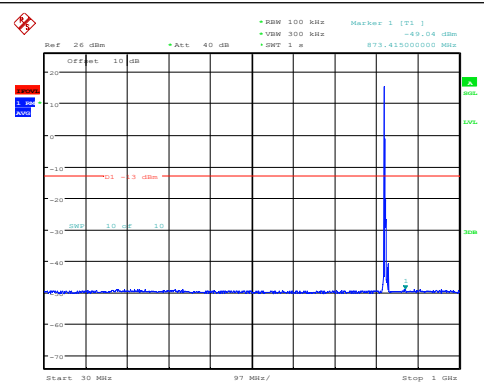
Band5-5MHz-16QAM-20425-1RB#0-30~1000-PAS S
