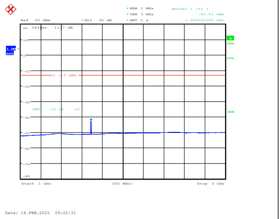
Band5-5MHz-QPSK-20625-1RB#0-1000~3000-PASS
