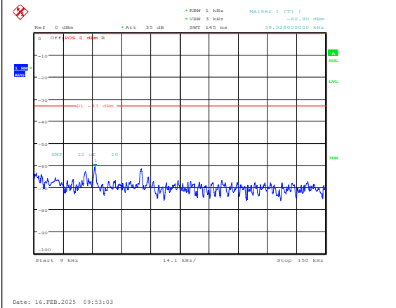
Band5-10MHz-QPSK-20525-1RB#0-0.009~0.15- PASS
