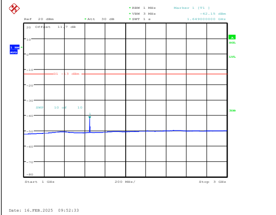
Band5-10MHz-16QAM-20450-1RB#0-1000~3000 -PASS
