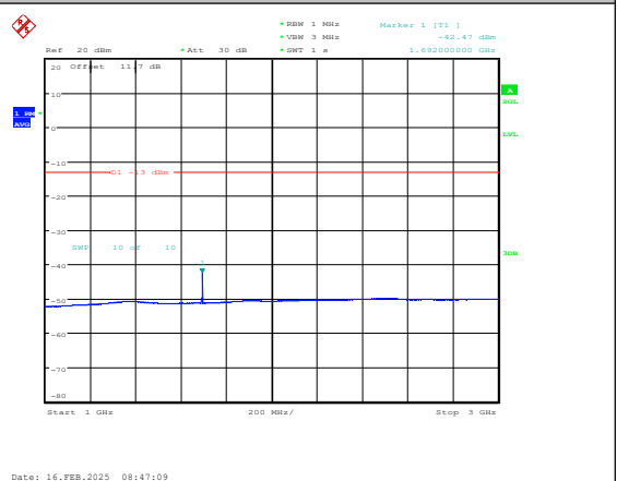
Band5-3MHz-QPSK-20635-1RB#0-1000~3000-PASS
