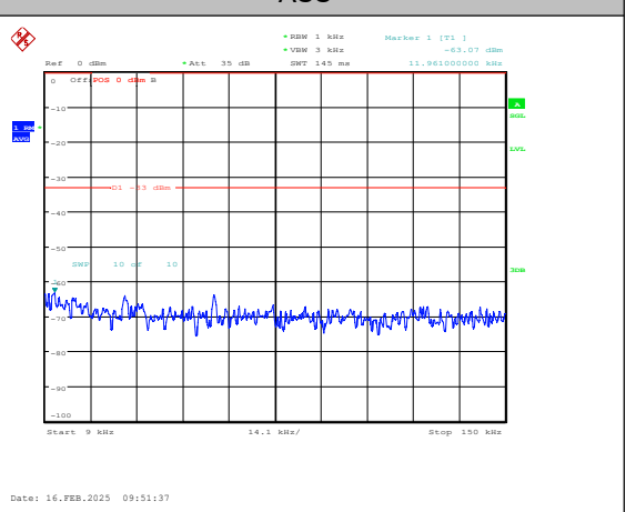
Band5-10MHz-16QAM-20450-1RB#0-0.009~0.15-PASS
