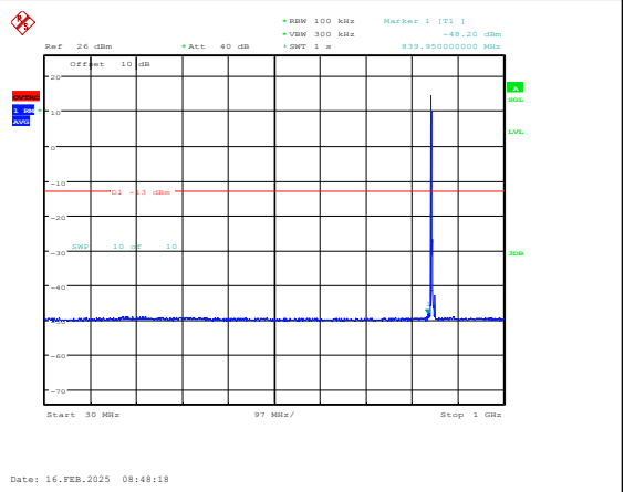
Band5-3MHz-16QAM-20635-1RB#0-30~1000-PASS
