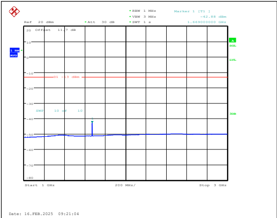
Band5-5MHz-16QAM-20525-1RB#0-1000~3000-PASS
