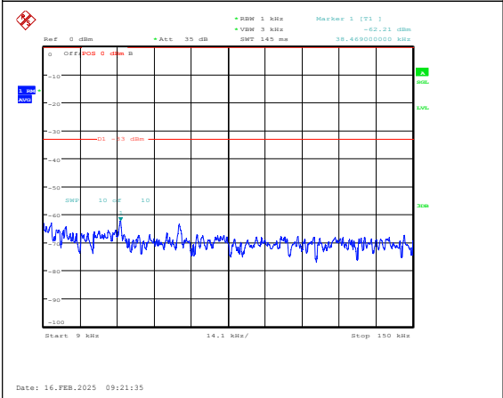
Band5-5MHz-QPSK-20625-1RB#0-0.009~0.15-PASS
