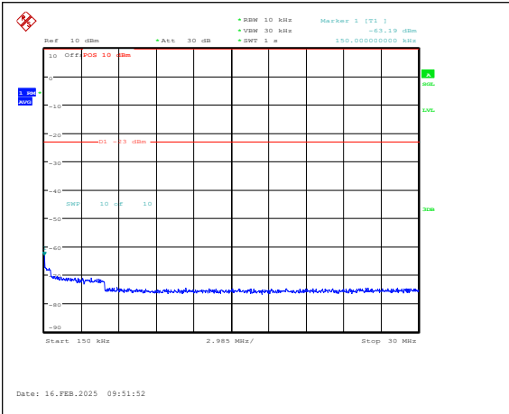
Band5-10MHz-16QAM-20450-1RB#0-0.15~30-PA SS
