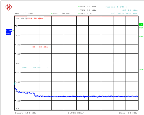
Band5-5MHz-16QAM-20425-1RB#0-0.15~30-PA SS
