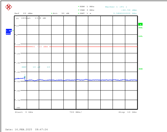
Band5-3MHz-QPSK-20635-1RB#0-3000~10000-PASS
