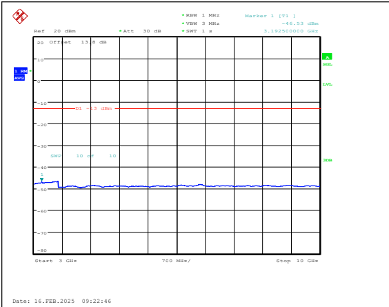
Band5-5MHz-QPSK-20625-1RB#0-3000~10000-PASS
