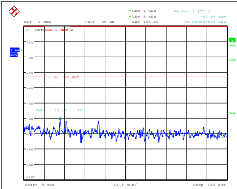
Band5-5MHz-QPSK-20425-1RB#0-0.009~0.15-P ASS
