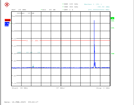
Band5-5MHz-QPSK-20625-1RB#0-30~1000-PASS
