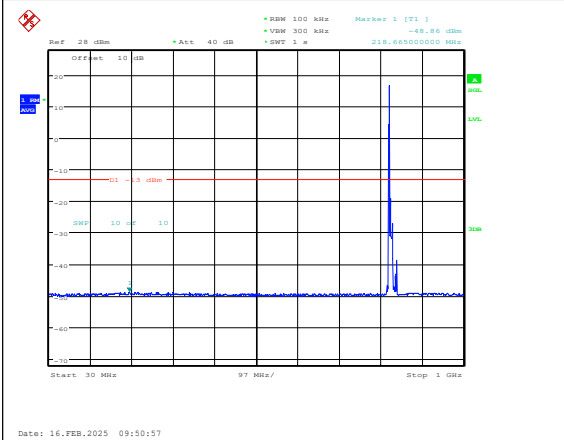
Band5-10MHz-QPSK-20450-1RB#0-30~1000-PA
