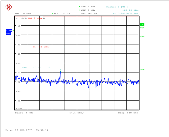
Band5-10MHz-QPSK-20450-1RB#0-0.009~0.15-PASS
