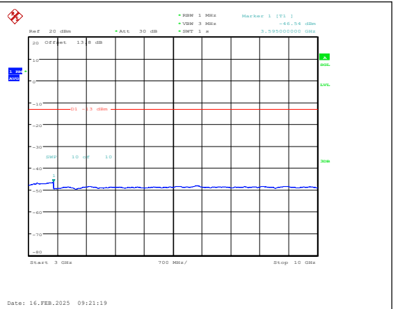
Band5-5MHz-16QAM-20525-1RB#0-3000~10000-PASS
