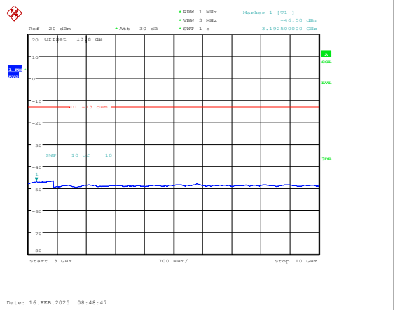
Band5-3MHz-16QAM-20635-1RB#0-3000~10000-PASS
