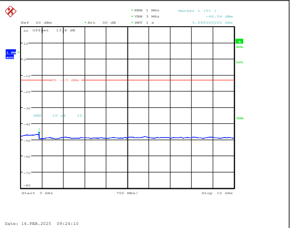
Band5-5MHz-16QAM-20625-1RB#0-3000~10000-PASS
