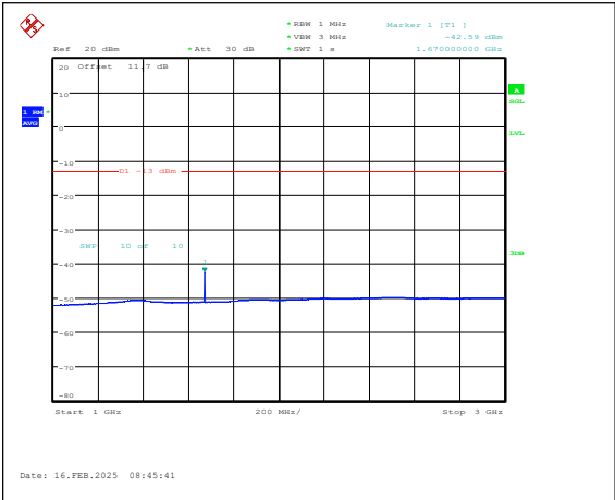
Band5-3MHz-16QAM-20525-1RB#0-1000~3000-PASS
