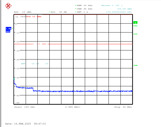
Band5-3MHz-16QAM-20635-1RB#0-0.15~30-PA
