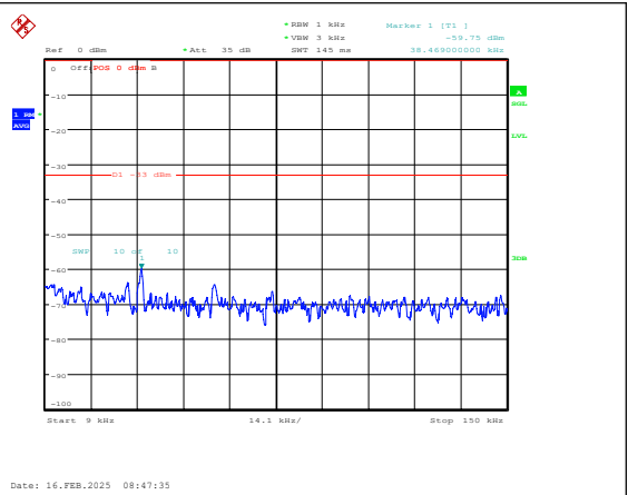
Band5-3MHz-16QAM-20635-1RB#0-0.009~0.15-PASS
