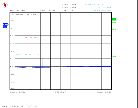
Band5-10MHz-QPSK-20450-1RB#0-1000~3000-P
