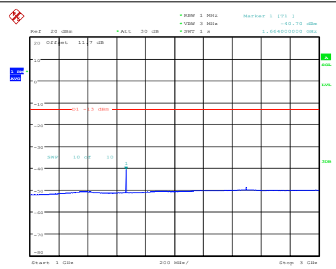
Band5-10MHz-QPSK-20525-1RB#0-1000~3000-P ASS
