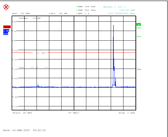
Band5-10MHz-16QAM-20450-1RB#0-30~1000-PA SS
