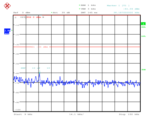
Band5-5MHz-QPSK-20425-1RB#0-1000~3000-PASS
