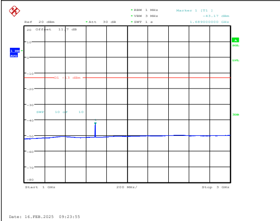
Band5-5MHz-16QAM-20625-1RB#0-1000~3000-PASS
