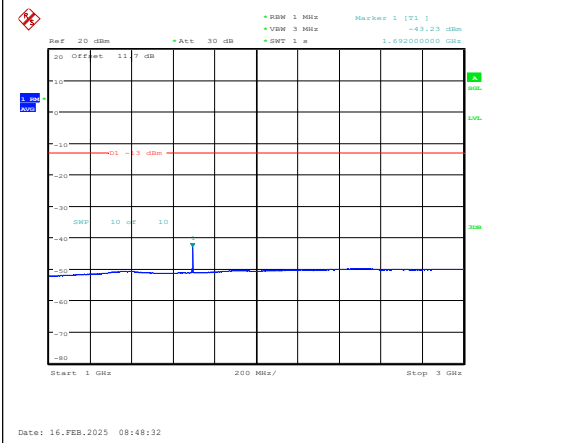
Band5-3MHz-16QAM-20635-1RB#0-1000~3000-PASS
