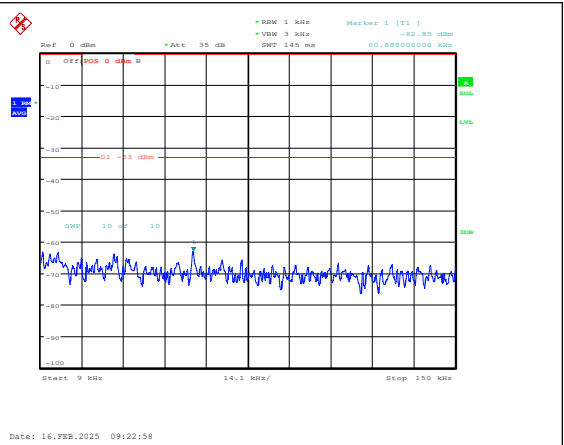
Band5-5MHz-16QAM-20625-1RB#0-0.009~0.15-P ASS
