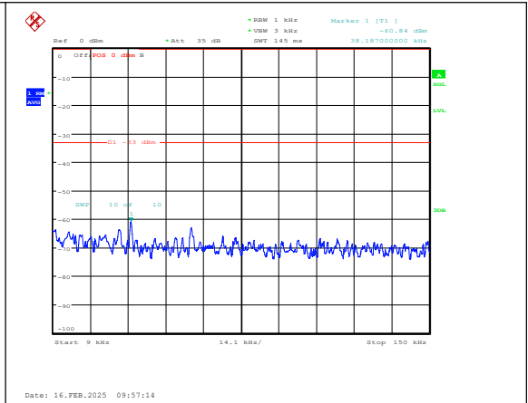
Band5-10MHz-16QAM-20600-1RB#0-0.009~0.15- PASS
