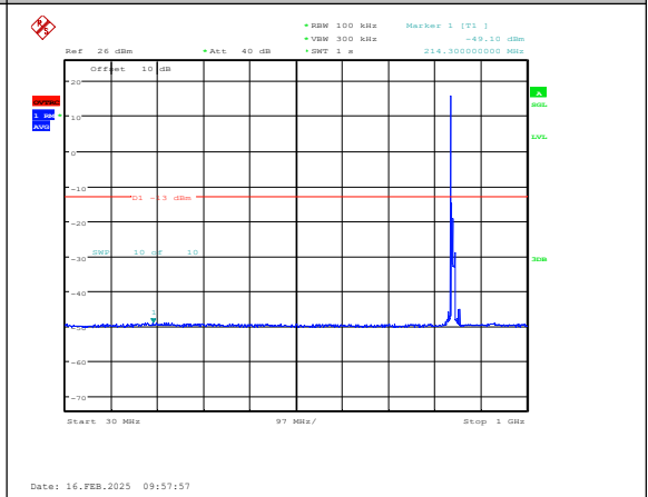
Band5-10MHz-16QAM-20600-1RB#0-30~1000-PA SS
