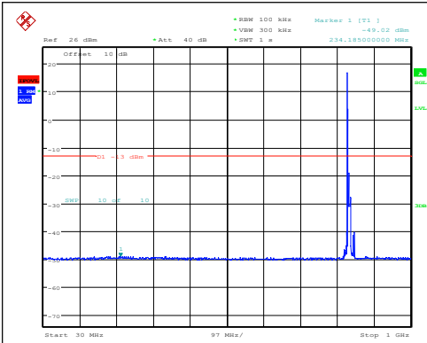
Band5-10MHz-QPSK-20525-1RB#0-30~1000-PA SS
